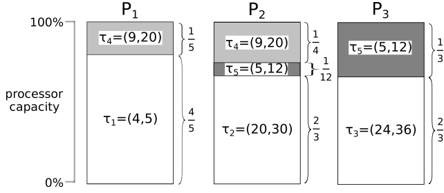
Figure 13: Counterexample to show that EDF-os is not optimal for non-preemptive task systems.
