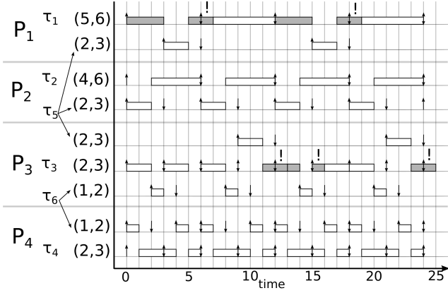
Figure 11: EDF-os schedule for Ex. 2. f_{5,1} = \frac{1}{4} , f_{5,2} = \frac{1}{2} and f_{5,3} = \frac{1}{4} . f_{6,3} = \frac{1}{3} and f_{6,4} = \frac{2}{3} .
