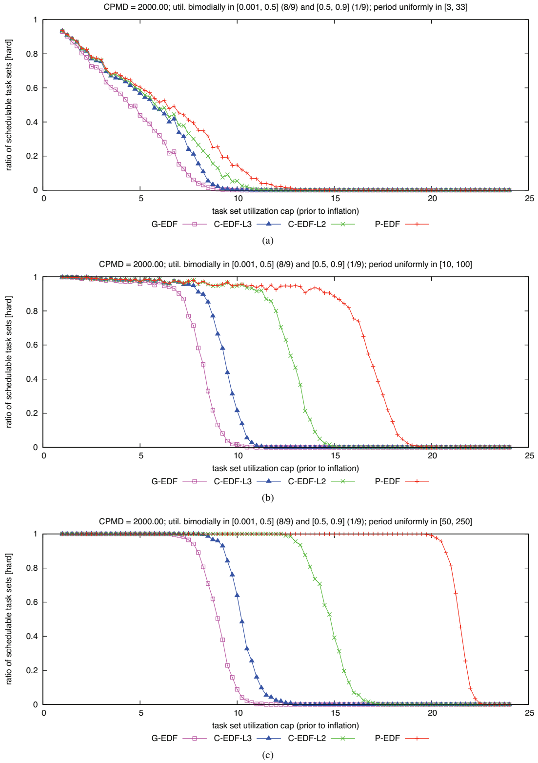
Figure 267: CPMD = 2000.00. Hard W(D) schedulability of task sets with bimodal light per-task utilizations and (a) short, (b) moderate, and (c) long periods.
