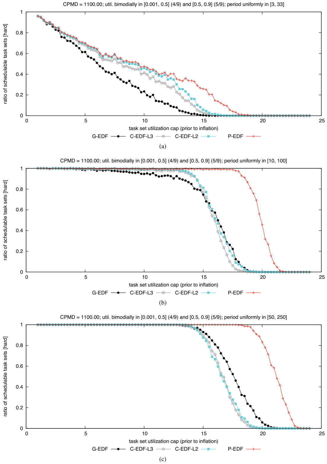
Figure 168: CPMD = 1100.00. Hard BF schedulability of task sets with bimodal heavy per-task utilizations and (a) short, (b) moderate, and (c) long periods.
