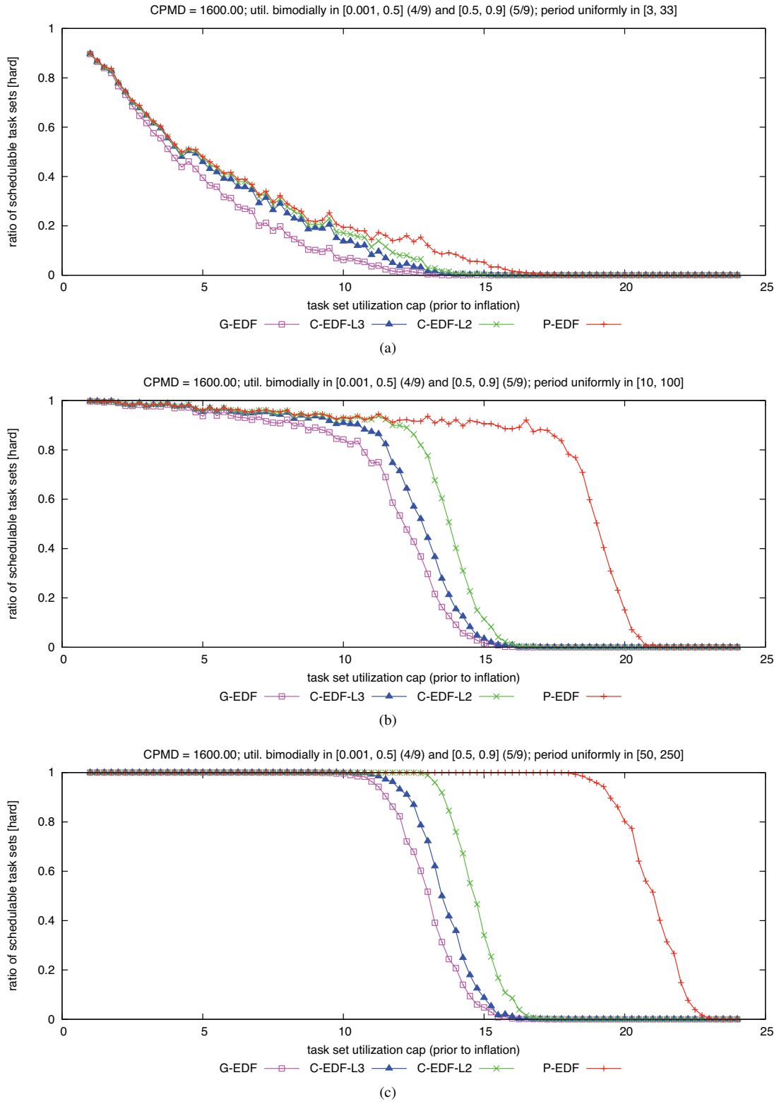
Figure 227: CPMD = 1600.00. Hard W(D) schedulability of task sets with bimodal heavy per-task utilizations and (a) short, (b) moderate, and (c) long periods.
