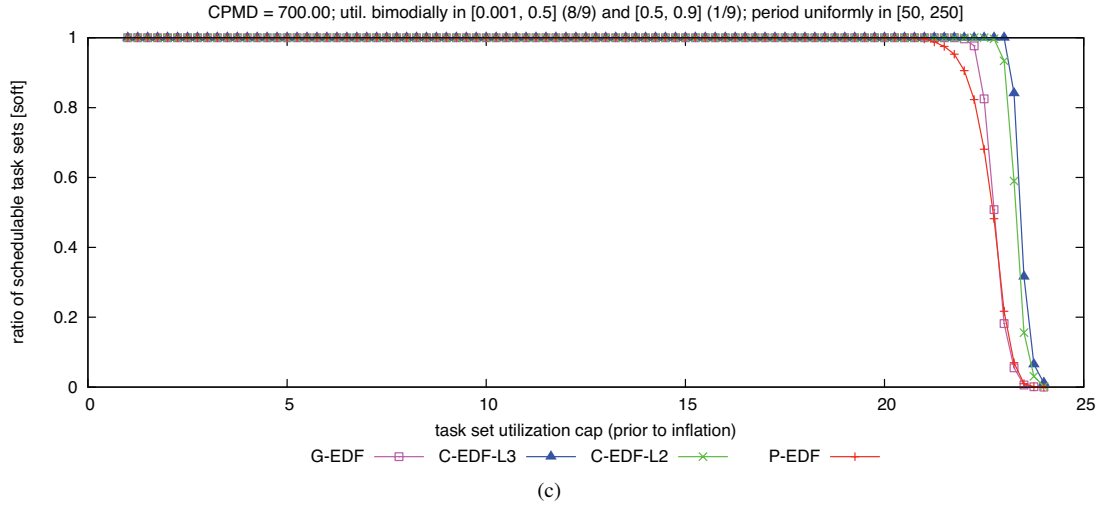
Figure 320: CPMD = 700.00. Soft schedulability of task sets with bimodal light per-task utilizations and (a) short, (b) moderate, and (c) long periods.
