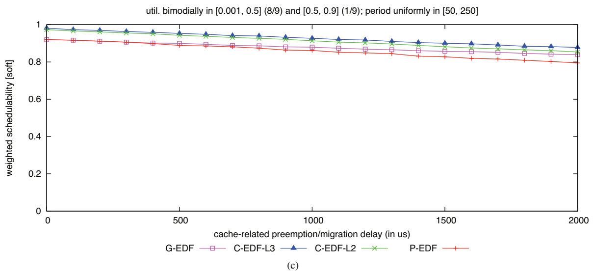
Figure 20: Soft weighted schedulability of task sets with bimodal light per-task utilizations and (a) short, (b) moderate, and (c) long periods.
