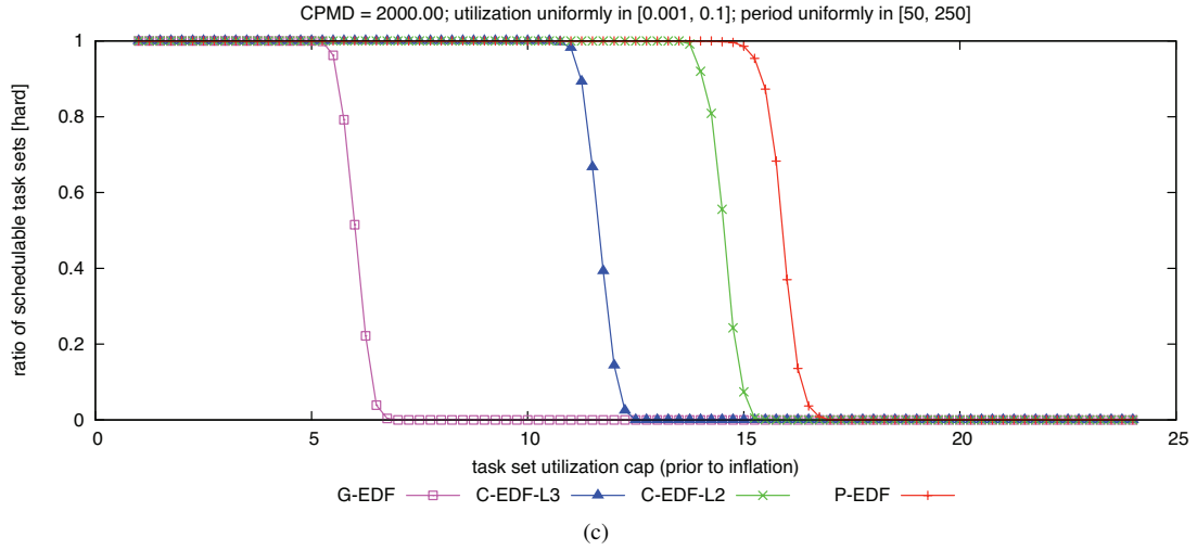
Figure 265: CPMD = 2000.00. Hard W(D) schedulability of task sets with uniform light per-task utilizations and (a) short, (b) moderate, and (c) long periods.
