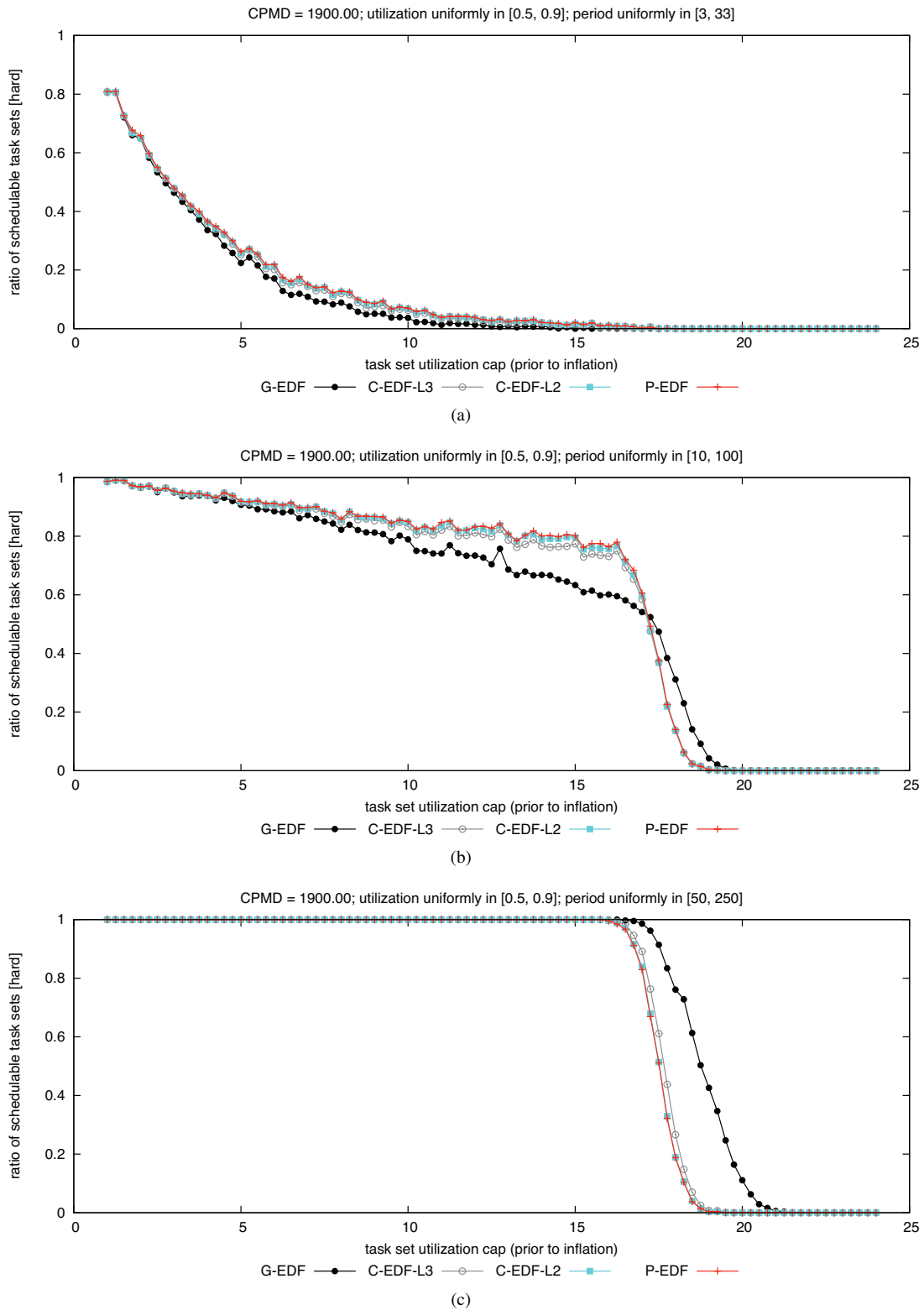
Figure 262: CPMD = 1900.00. Hard BF schedulability of task sets with uniform heavy per-task utilizations and (a) short, (b) moderate, and (c) long periods.
