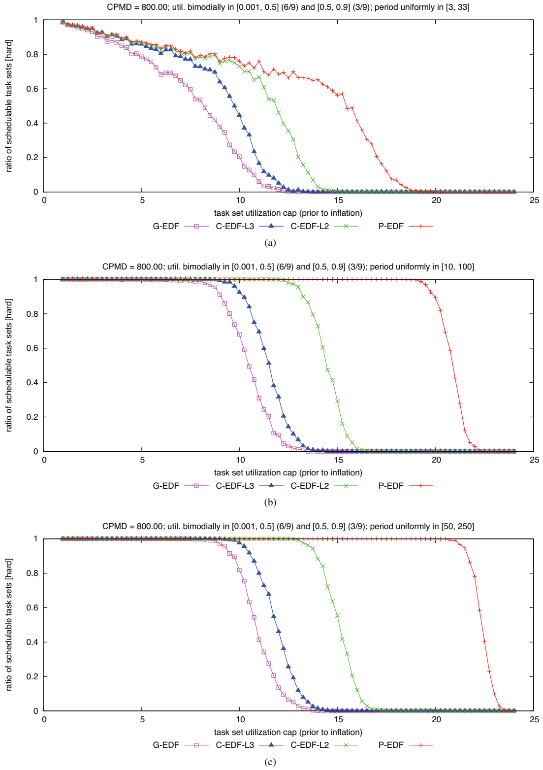
Figure 127: CPMD = 800.00. Hard W(D) schedulability of task sets with bimodal medium per-task utilizations and (a) short, (b) moderate, and (c) long periods.
