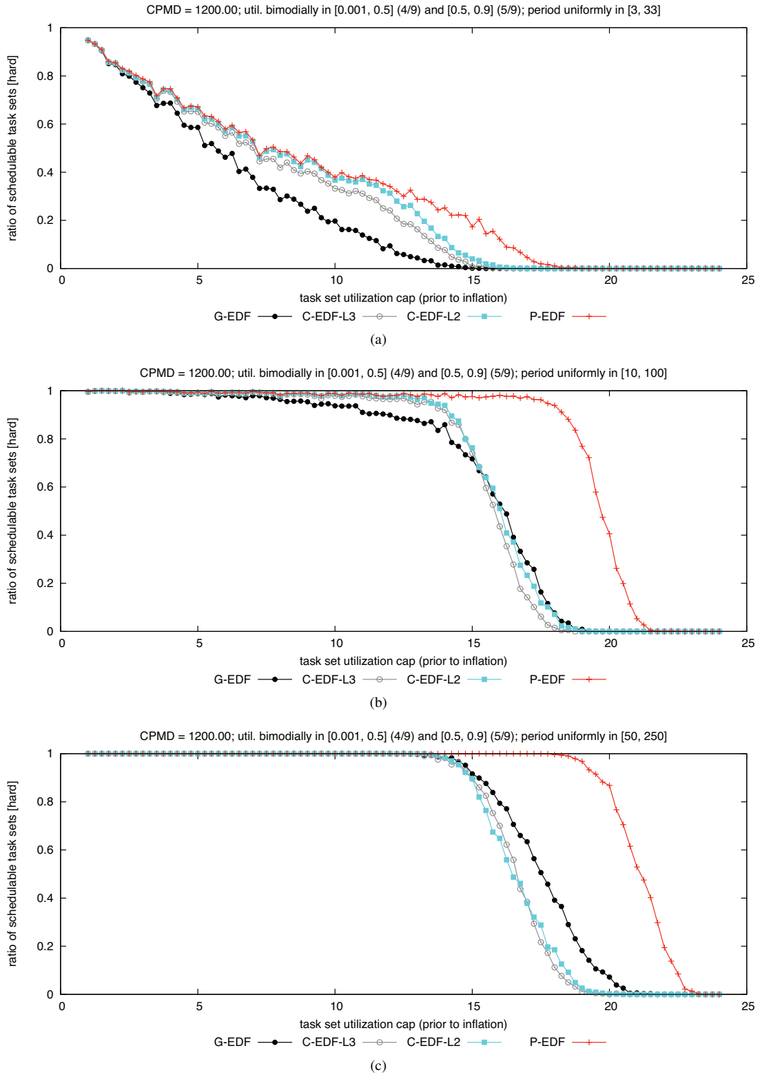
Figure 180: CPMD = 1200.00. Hard BF schedulability of task sets with bimodal heavy per-task utilizations and (a) short, (b) moderate, and (c) long periods.
