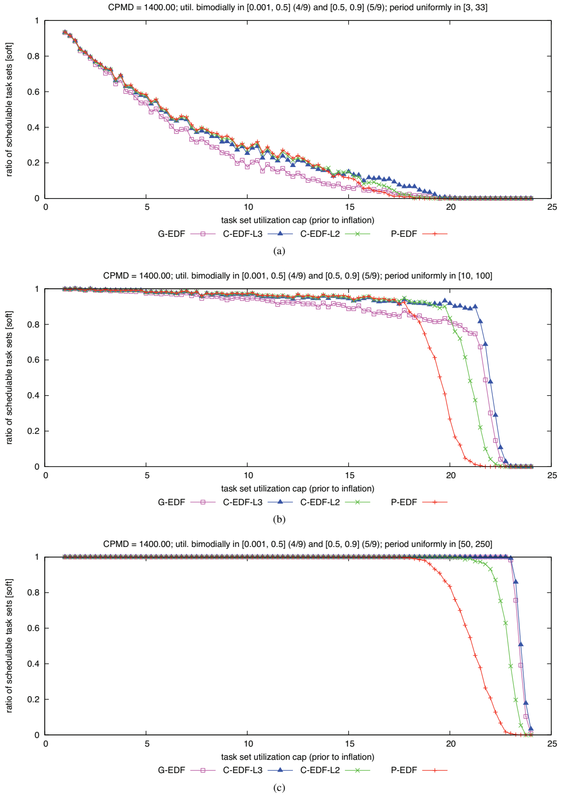
Figure 366: CPMD = 1400.00. Soft schedulability of task sets with bimodal heavy per-task utilizations and (a) short, (b) moderate, and (c) long periods.
