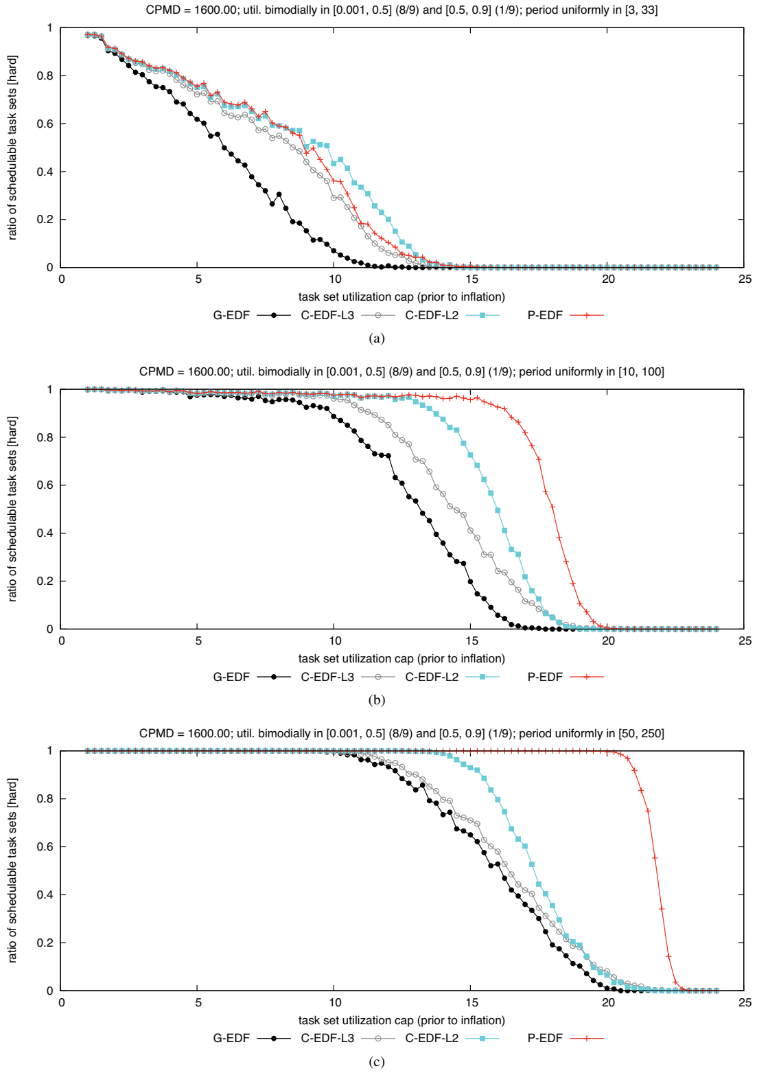
Figure 220: CPMD = 1600.00. Hard BF schedulability of task sets with bimodal light per-task utilizations and (a) short, (b) moderate, and (c) long periods.
