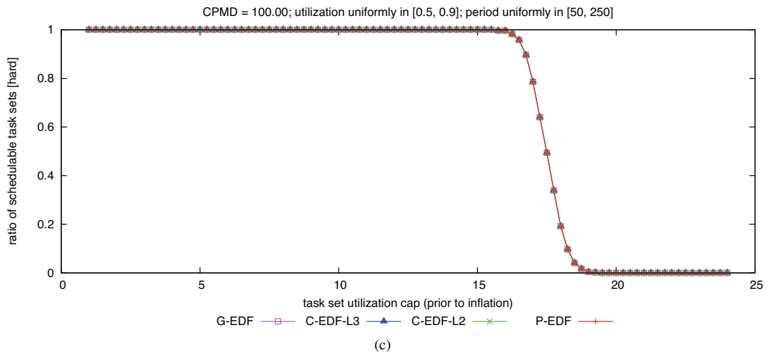
Figure 45: CPMD = 100.00. Hard W(D) schedulability of task sets with uniform heavy per-task utilizations and (a) short, (b) moderate, and (c) long periods.
