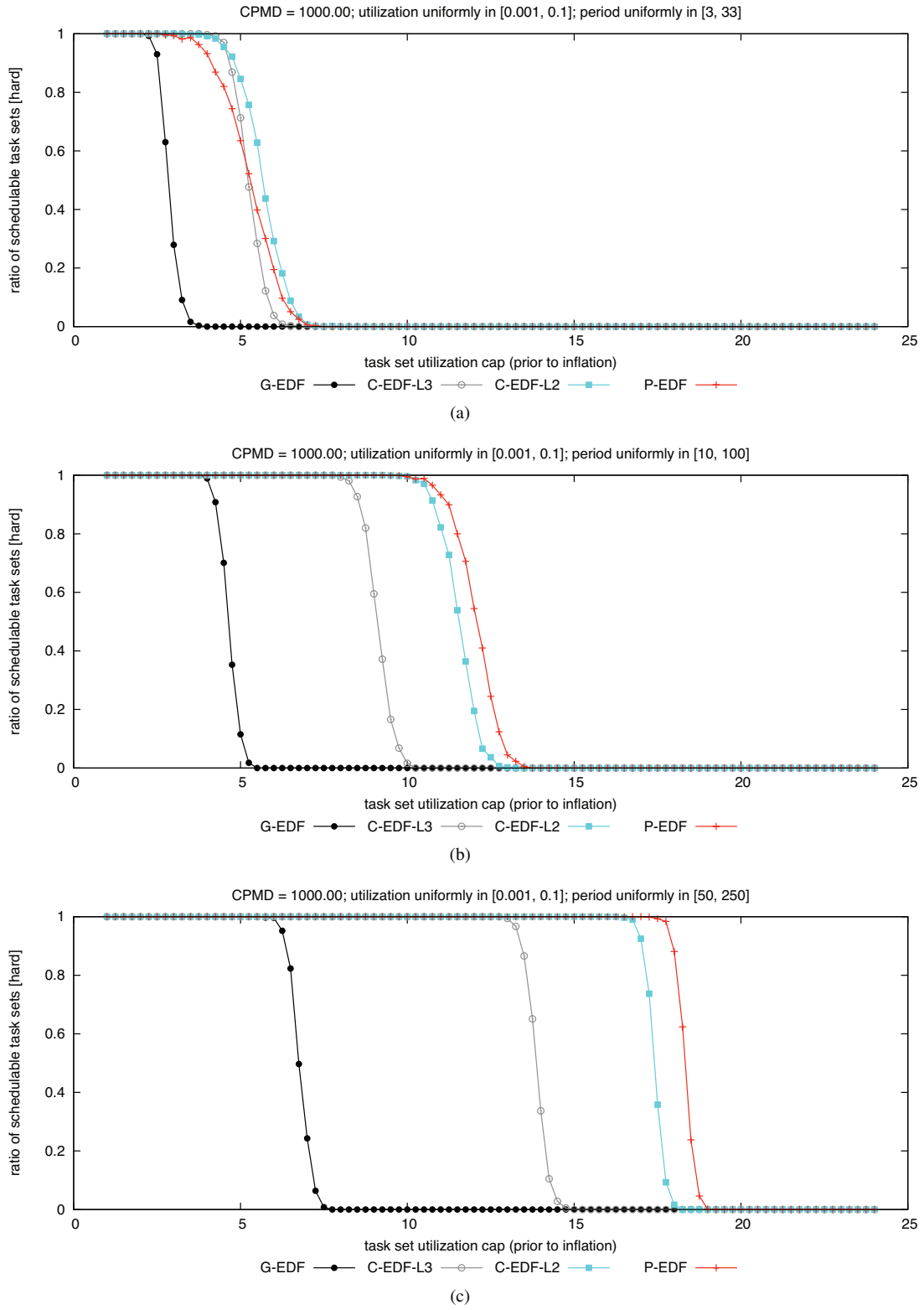
Figure 146: CPMD = 1000.00. Hard BF schedulability of task sets with uniform light per-task utilizations and (a) short, (b) moderate, and (c) long periods.
