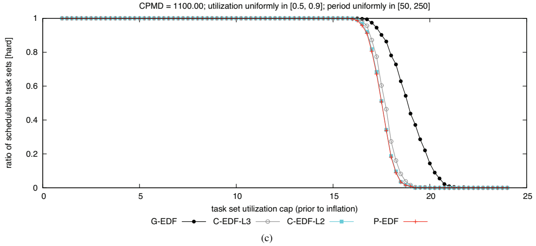
Figure 166: CPMD = 1100.00. Hard BF schedulability of task sets with uniform heavy per-task utilizations and (a) short, (b) moderate, and (c) long periods.
