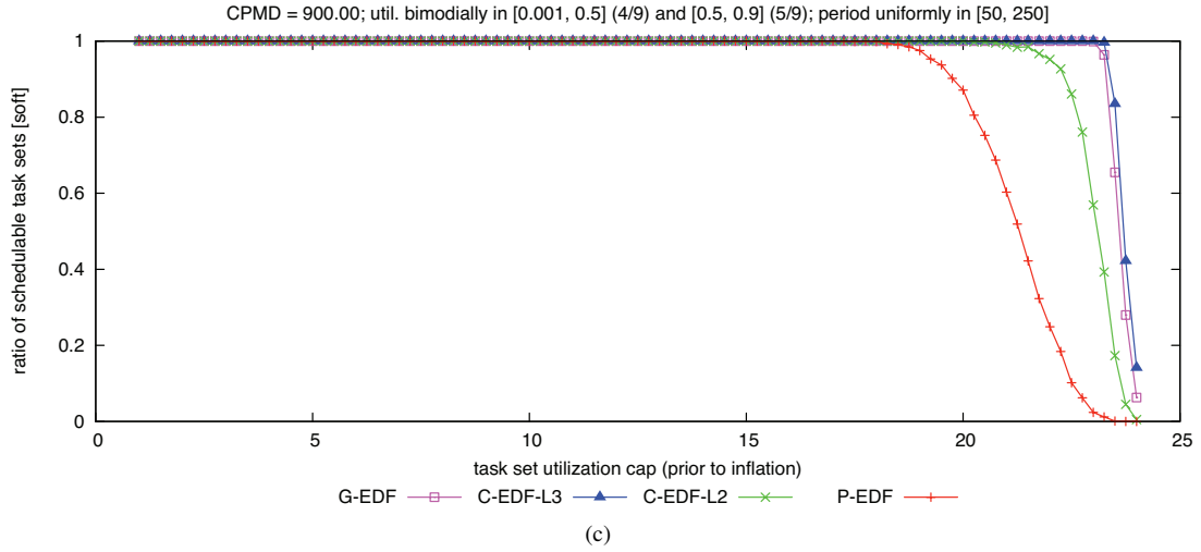
Figure 336: CPMD = 900.00. Soft schedulability of task sets with bimodal heavy per-task utilizations and (a) short, (b) moderate, and (c) long periods.
