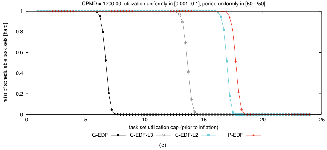
Figure 170: CPMD = 1200.00. Hard BF schedulability of task sets with uniform light per-task utilizations and (a) short, (b) moderate, and (c) long periods.
