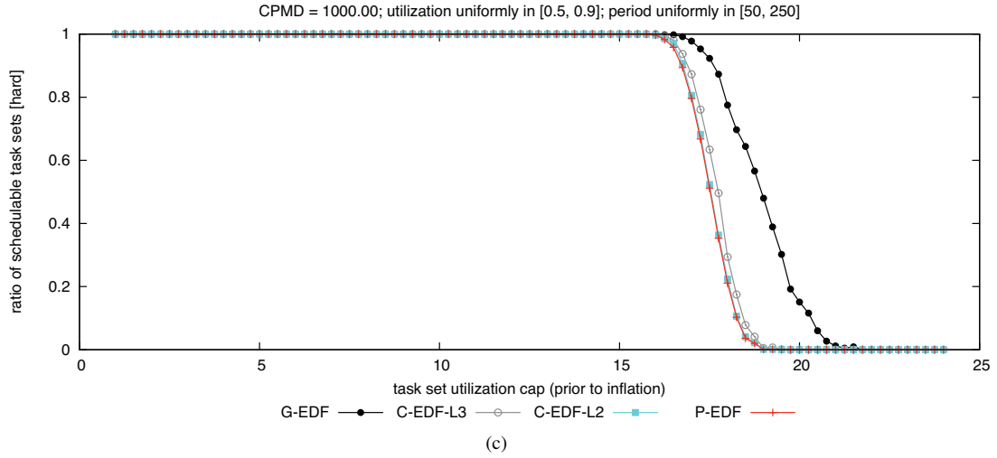
Figure 154: CPMD = 1000.00. Hard BF schedulability of task sets with uniform heavy per-task utilizations and (a) short, (b) moderate, and (c) long periods.
