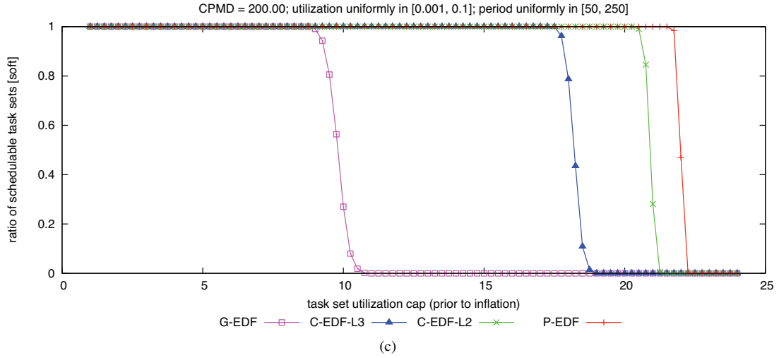
Figure 289: CPMD = 200.00. Soft schedulability of task sets with uniform light per-task utilizations and (a) short, (b) moderate, and (c) long periods.
