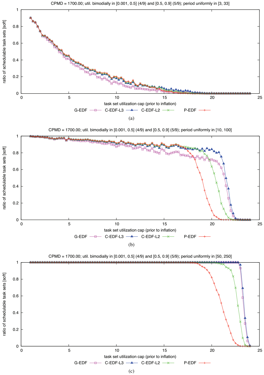
Figure 384: CPMD = 1700.00. Soft schedulability of task sets with bimodal heavy per-task utilizations and (a) short, (b) moderate, and (c) long periods.
