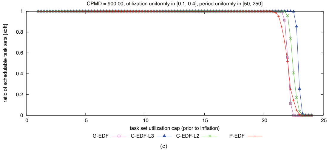
Figure 333: CPMD = 900.00. Soft schedulability of task sets with uniform medium per-task utilizations and (a) short, (b) moderate, and (c) long periods.
