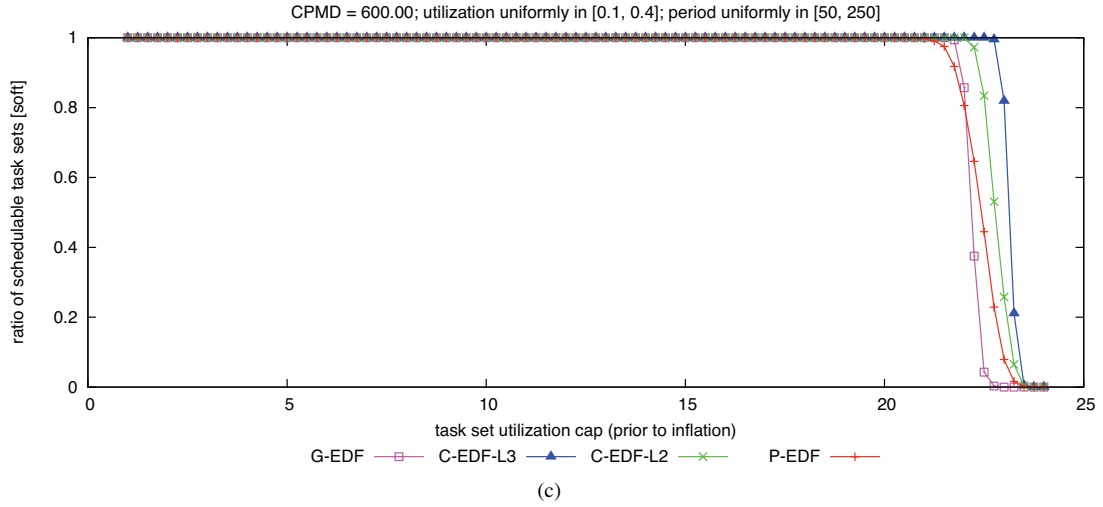
Figure 315: CPMD = 600.00. Soft schedulability of task sets with uniform medium per-task utilizations and (a) short, (b) moderate, and (c) long periods.
