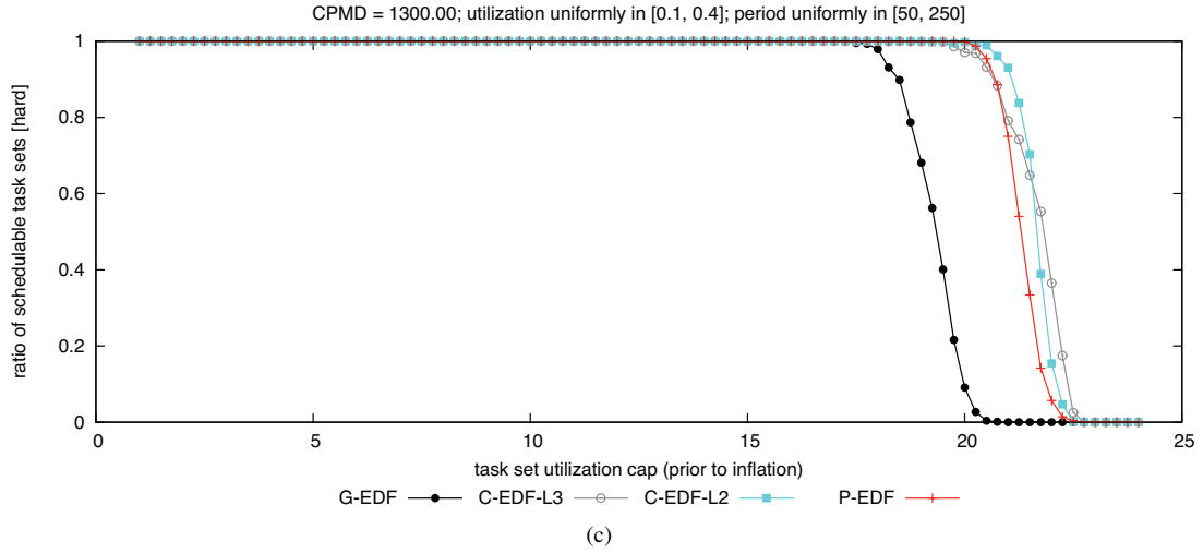
Figure 186: CPMD = 1300.00. Hard BF schedulability of task sets with uniform medium per-task utilizations and (a) short, (b) moderate, and (c) long periods.
