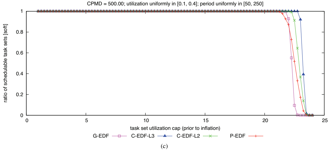
Figure 309: CPMD = 500.00. Soft schedulability of task sets with uniform medium per-task utilizations and (a) short, (b) moderate, and (c) long periods.
