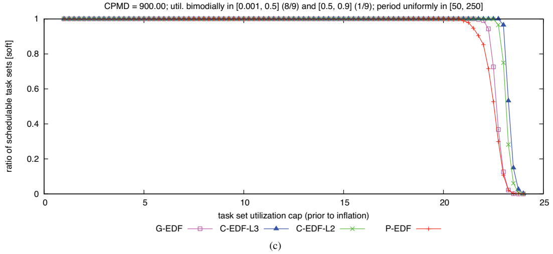
Figure 332: CPMD = 900.00. Soft schedulability of task sets with bimodal light per-task utilizations and (a) short, (b) moderate, and (c) long periods.
