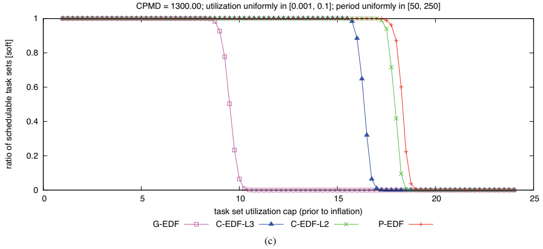
Figure 355: CPMD = 1300.00. Soft schedulability of task sets with uniform light per-task utilizations and (a) short, (b) moderate, and (c) long periods.
