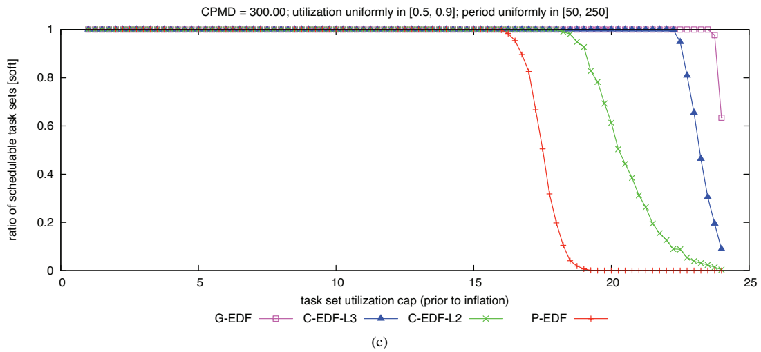
Figure 299: CPMD = 300.00. Soft schedulability of task sets with uniform heavy per-task utilizations and (a) short, (b) moderate, and (c) long periods.
