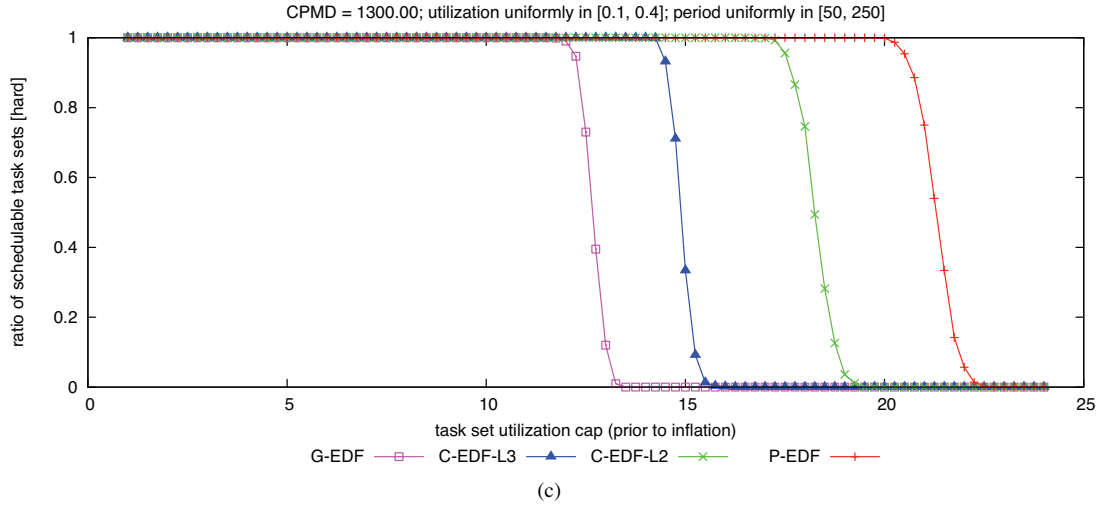
Figure 185: CPMD = 1300.00. Hard W(D) schedulability of task sets with uniform medium per-task utilizations and (a) short, (b) moderate, and (c) long periods.
