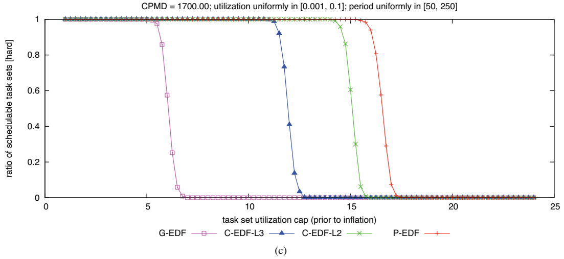
Figure 229: CPMD = 1700.00. Hard W(D) schedulability of task sets with uniform light per-task utilizations and (a) short, (b) moderate, and (c) long periods.
