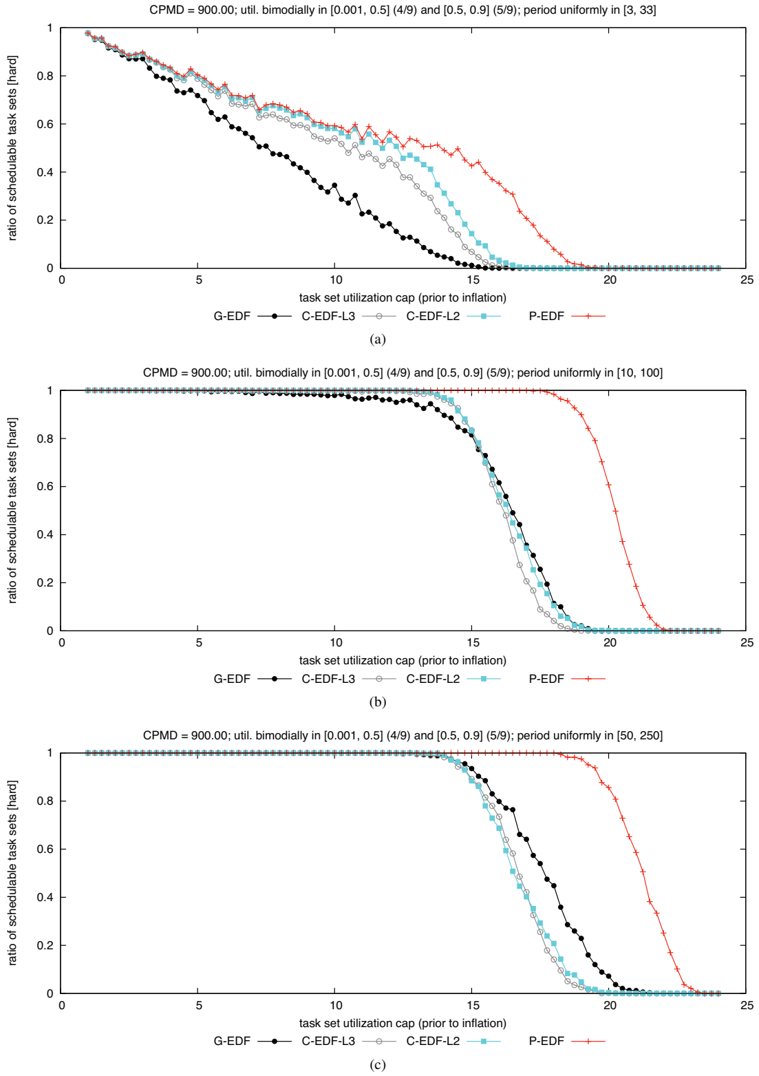
Figure 144: CPMD = 900.00. Hard BF schedulability of task sets with bimodal heavy per-task utilizations and (a) short, (b) moderate, and (c) long periods.
