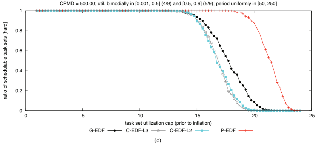
Figure 96: CPMD = 500.00. Hard BF schedulability of task sets with bimodal heavy per-task utilizations and (a) short, (b) moderate, and (c) long periods.
