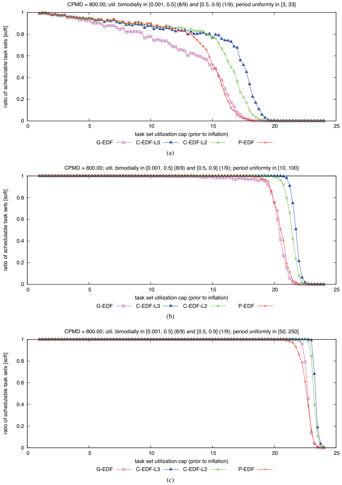
Figure 326: CPMD = 800.00. Soft schedulability of task sets with bimodal light per-task utilizations and (a) short, (b) moderate, and (c) long periods.
