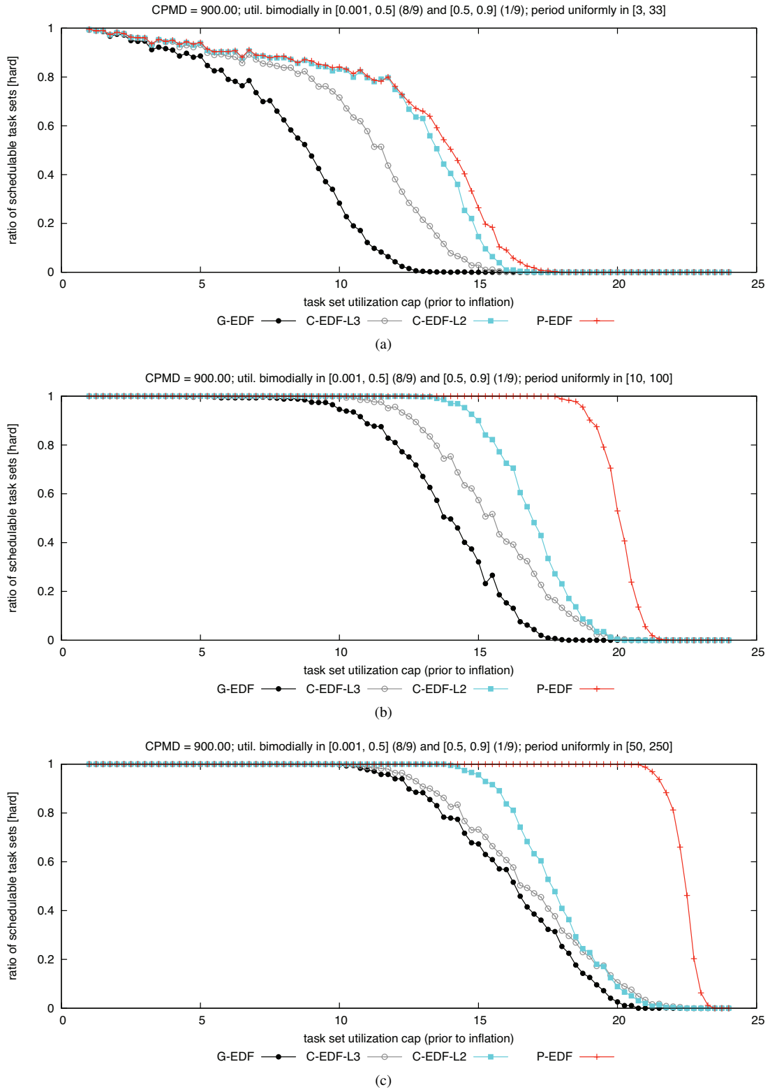
Figure 136: CPMD = 900.00. Hard BF schedulability of task sets with bimodal light per-task utilizations and (a) short, (b) moderate, and (c) long periods.
