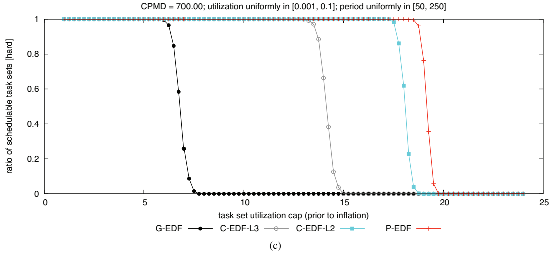
Figure 110: CPMD = 700.00. Hard BF schedulability of task sets with uniform light per-task utilizations and (a) short, (b) moderate, and (c) long periods.
