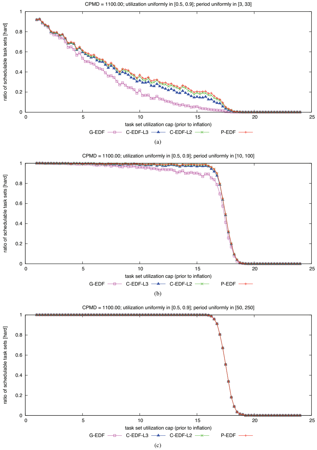
Figure 165: CPMD = 1100.00. Hard W(D) schedulability of task sets with uniform heavy per-task utilizations and (a) short, (b) moderate, and (c) long periods.
