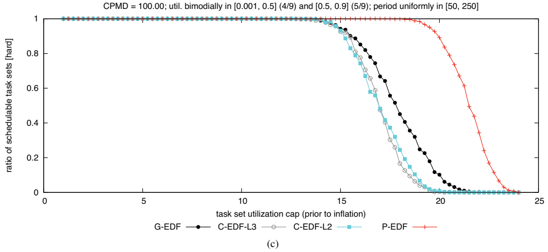
Figure 48: CPMD = 100.00. Hard BF schedulability of task sets with bimodal heavy per-task utilizations and (a) short, (b) moderate, and (c) long periods.
