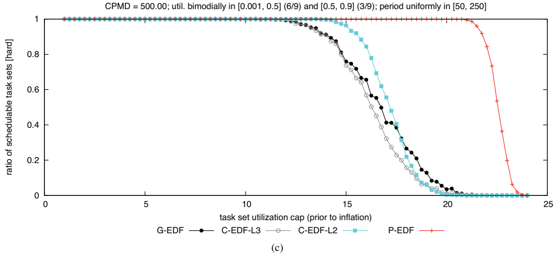
Figure 92: CPMD = 500.00. Hard BF schedulability of task sets with bimodal medium per-task utilizations and (a) short, (b) moderate, and (c) long periods.
