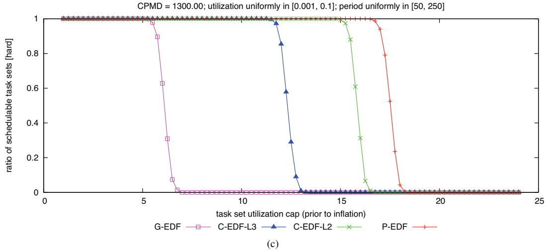
Figure 181: CPMD = 1300.00. Hard W(D) schedulability of task sets with uniform light per-task utilizations and (a) short, (b) moderate, and (c) long periods.
