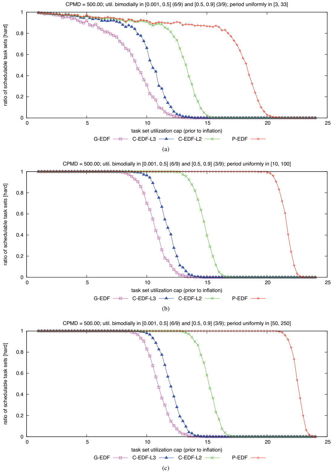
Figure 91: CPMD = 500.00. Hard W(D) schedulability of task sets with bimodal medium per-task utilizations and (a) short, (b) moderate, and (c) long periods.
