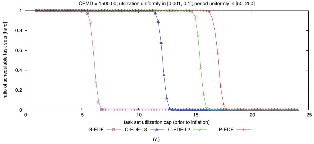
Figure 205: CPMD = 1500.00. Hard W(D) schedulability of task sets with uniform light per-task utilizations and (a) short, (b) moderate, and (c) long periods.
