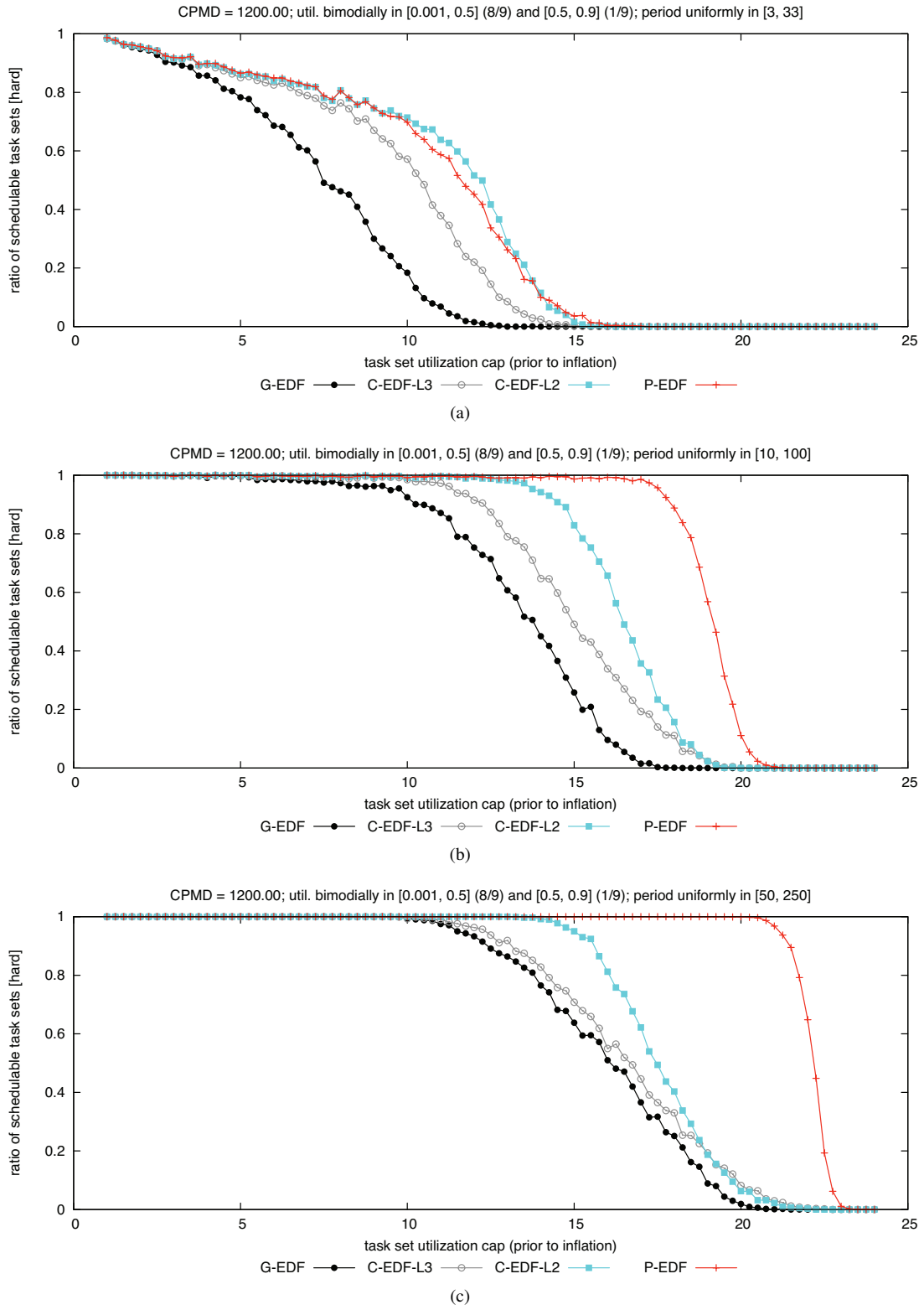
Figure 172: CPMD = 1200.00. Hard BF schedulability of task sets with bimodal light per-task utilizations and (a) short, (b) moderate, and (c) long periods.
