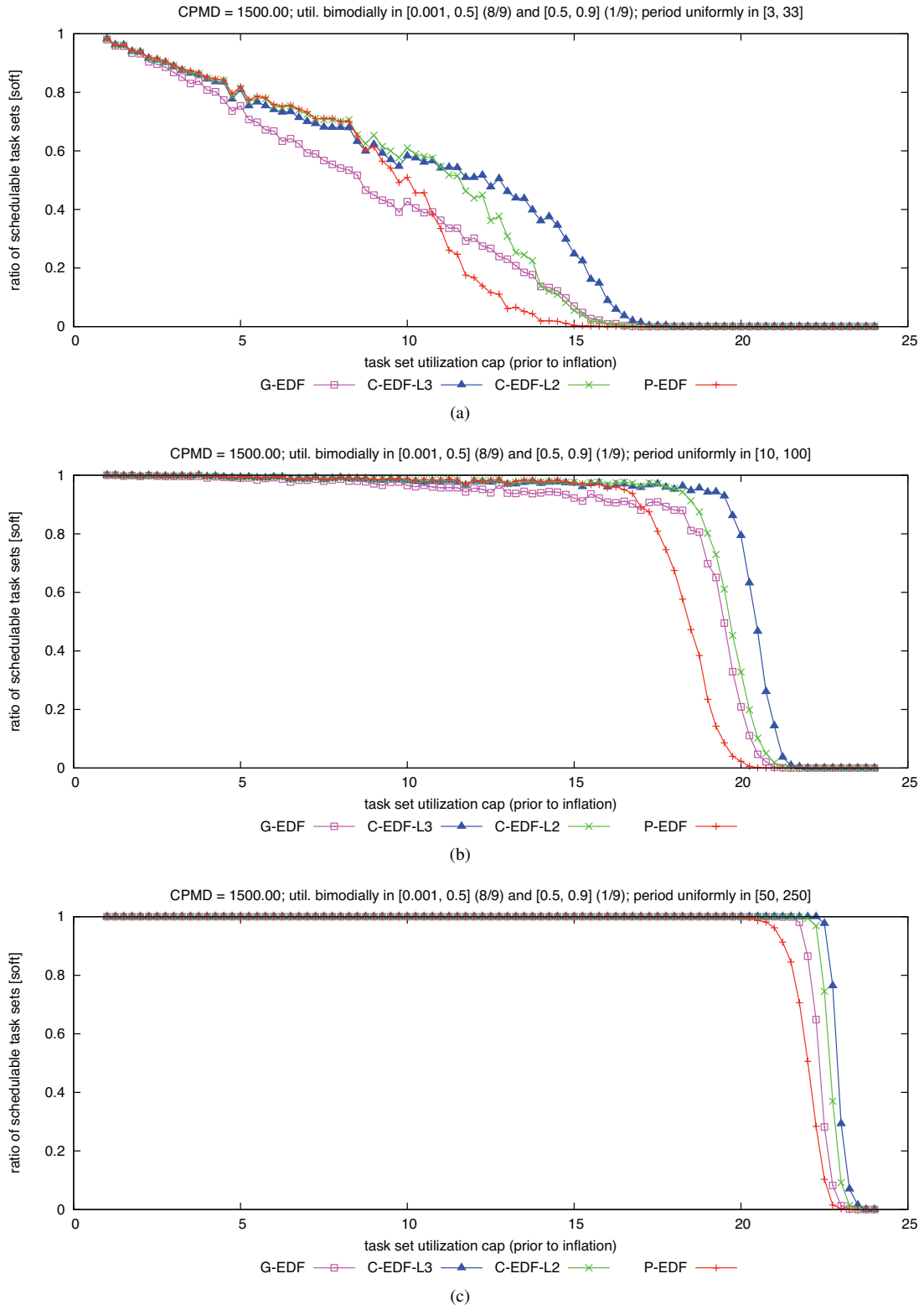
Figure 368: CPMD = 1500.00. Soft schedulability of task sets with bimodal light per-task utilizations and (a) short, (b) moderate, and (c) long periods.
