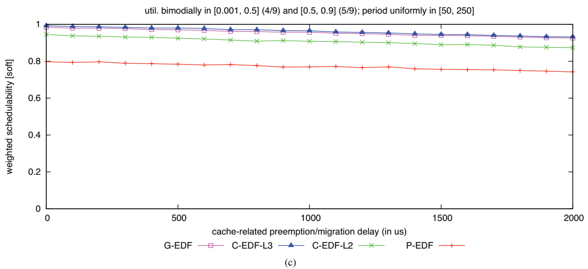
Figure 24: Soft weighted schedulability of task sets with bimodal heavy per-task utilizations and (a) short, (b) moderate, and (c) long periods.
