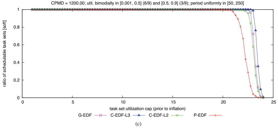
Figure 352: CPMD = 1200.00. Soft schedulability of task sets with bimodal medium per-task utilizations and (a) short, (b) moderate, and (c) long periods.
