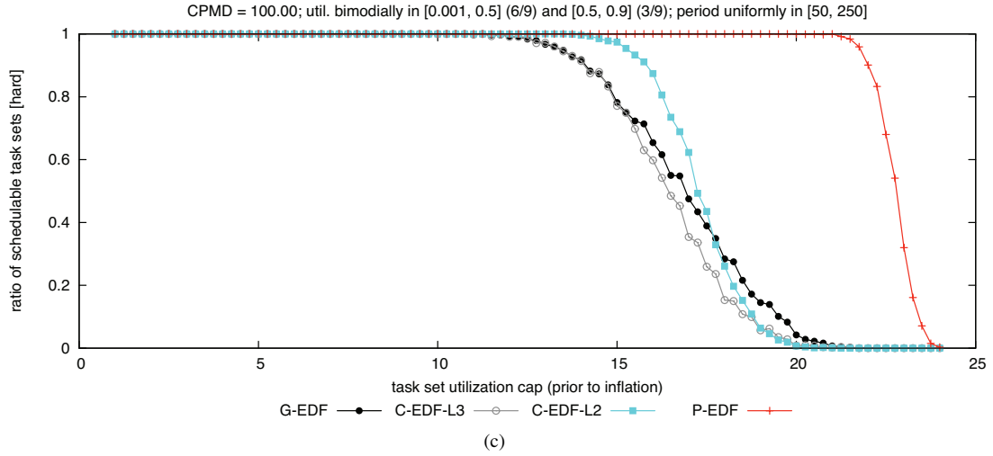
Figure 44: CPMD = 100.00. Hard BF schedulability of task sets with bimodal medium per-task utilizations and (a) short, (b) moderate, and (c) long periods.
