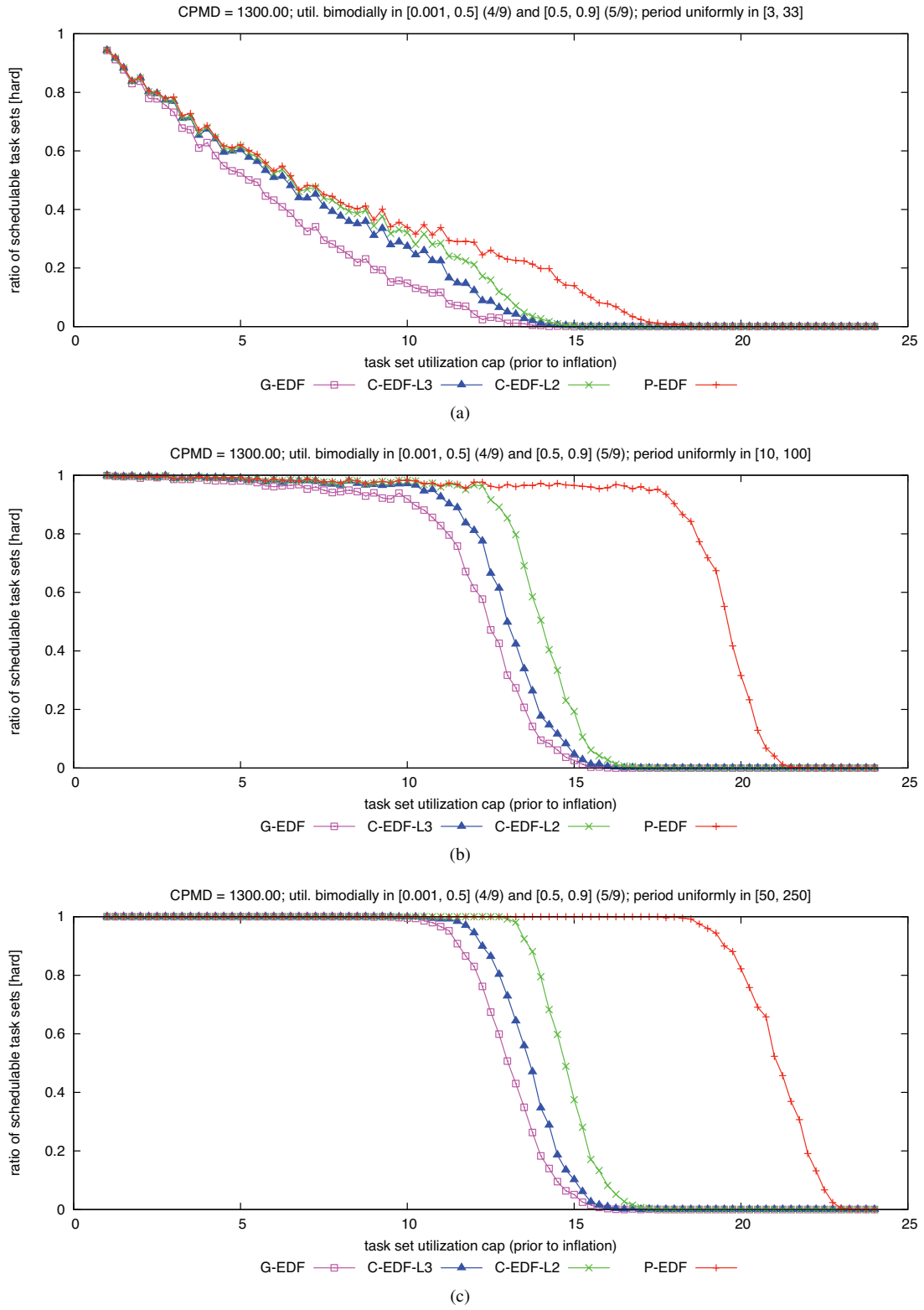
Figure 191: CPMD = 1300.00. Hard W(D) schedulability of task sets with bimodal heavy per-task utilizations and (a) short, (b) moderate, and (c) long periods.
