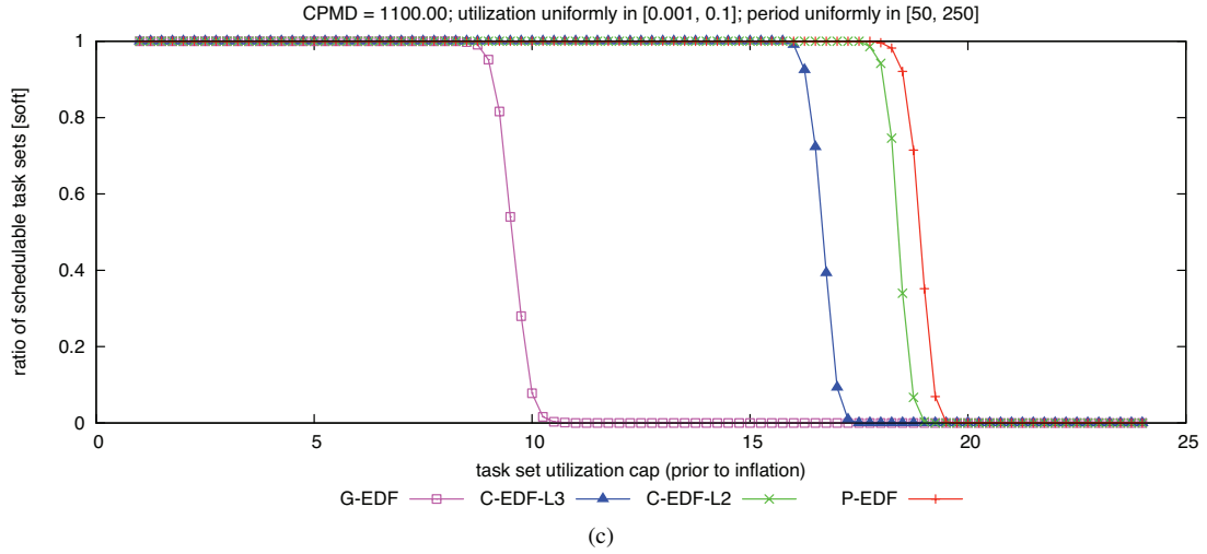
Figure 343: CPMD = 1100.00. Soft schedulability of task sets with uniform light per-task utilizations and (a) short, (b) moderate, and (c) long periods.
