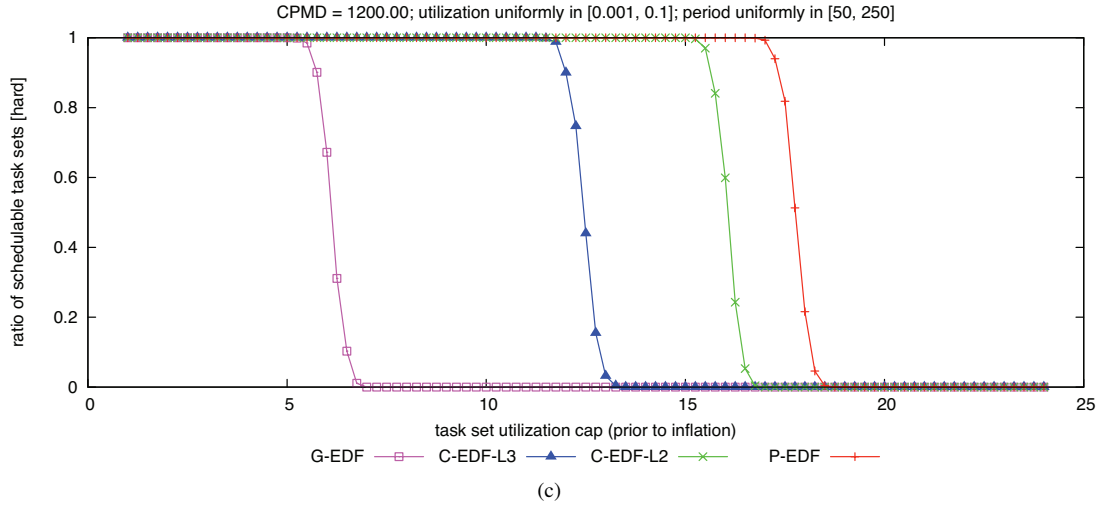
Figure 169: CPMD = 1200.00. Hard W(D) schedulability of task sets with uniform light per-task utilizations and (a) short, (b) moderate, and (c) long periods.
