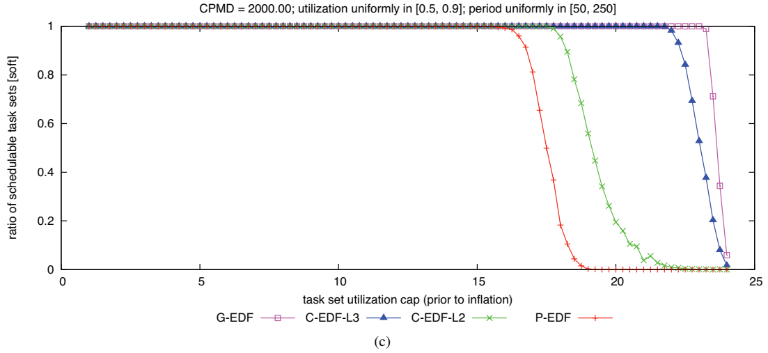
Figure 401: CPMD = 2000.00. Soft schedulability of task sets with uniform heavy per-task utilizations and (a) short, (b) moderate, and (c) long periods.
