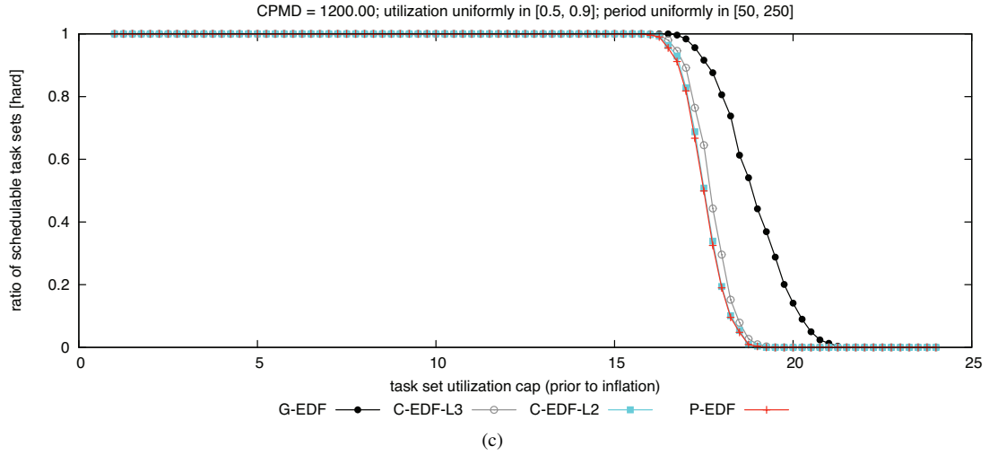
Figure 178: CPMD = 1200.00. Hard BF schedulability of task sets with uniform heavy per-task utilizations and (a) short, (b) moderate, and (c) long periods.
