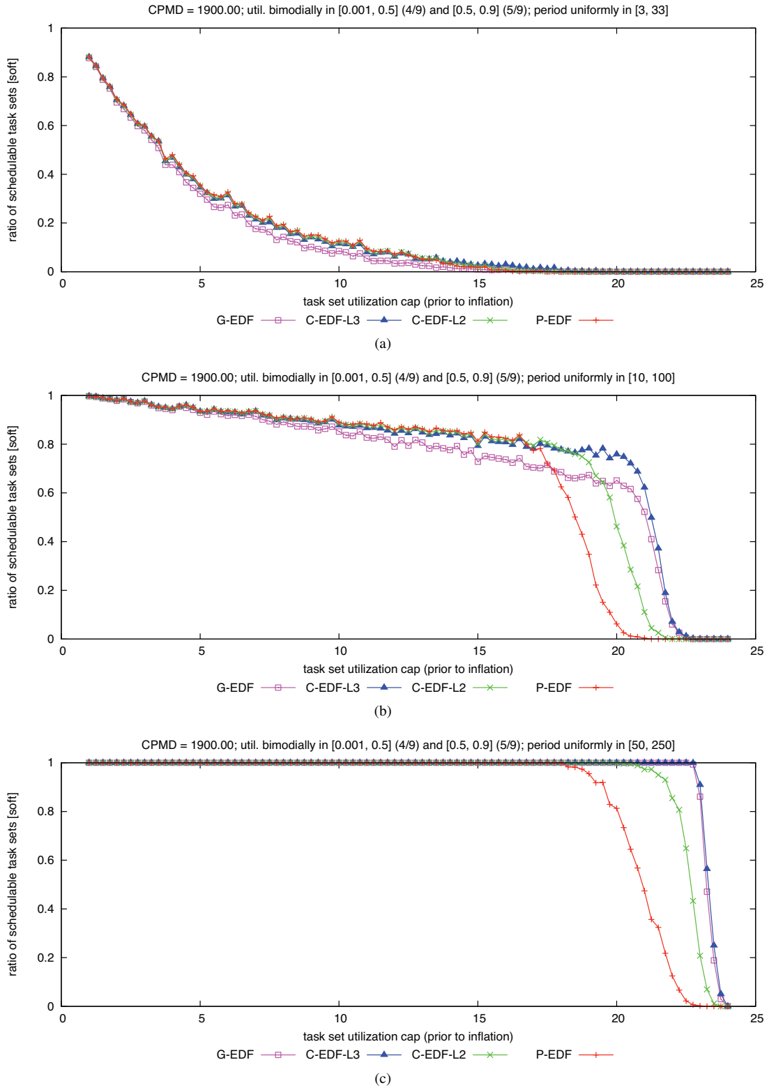
Figure 396: CPMD = 1900.00. Soft schedulability of task sets with bimodal heavy per-task utilizations and (a) short, (b) moderate, and (c) long periods.
