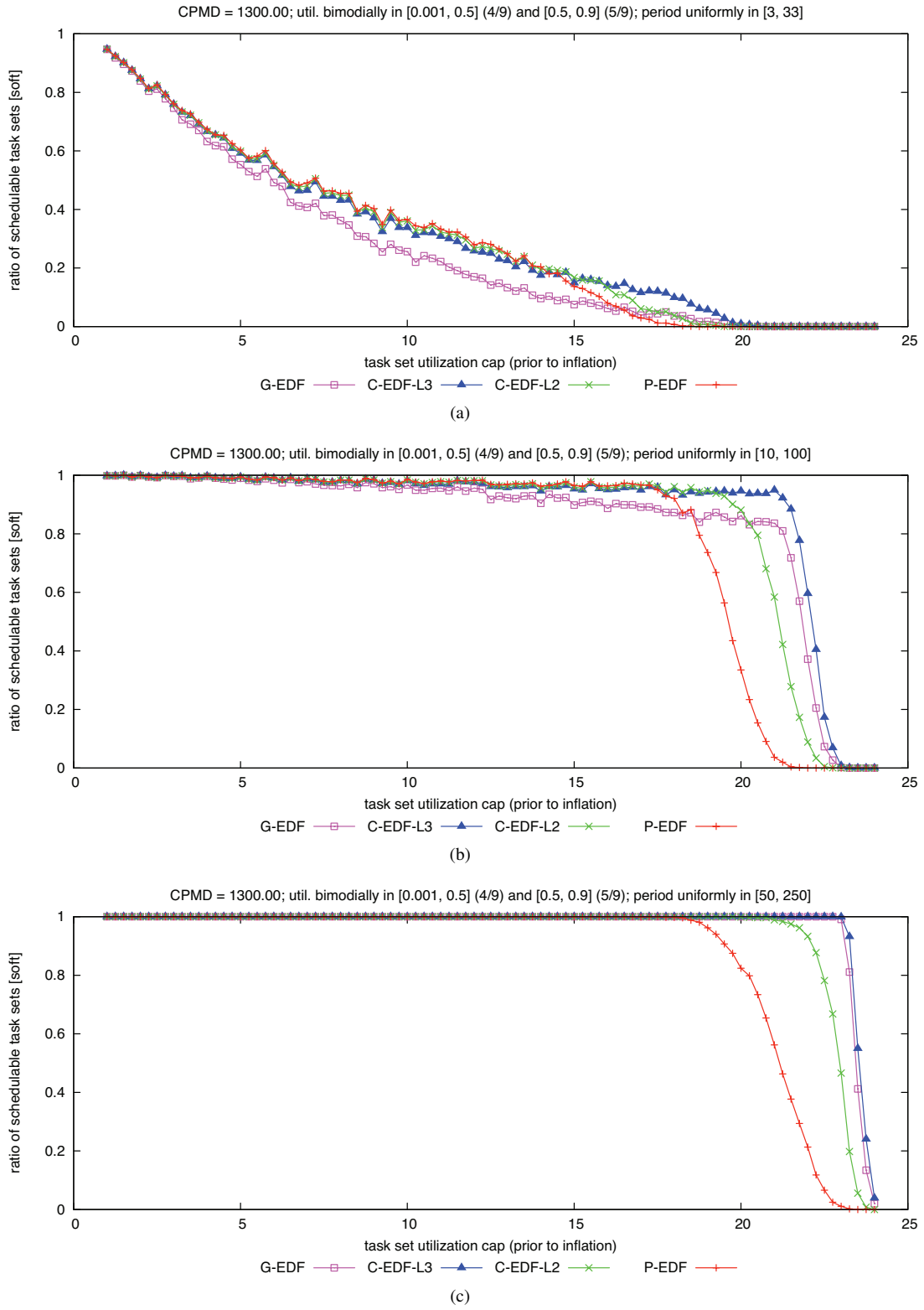
Figure 360: CPMD = 1300.00. Soft schedulability of task sets with bimodal heavy per-task utilizations and (a) short, (b) moderate, and (c) long periods.
