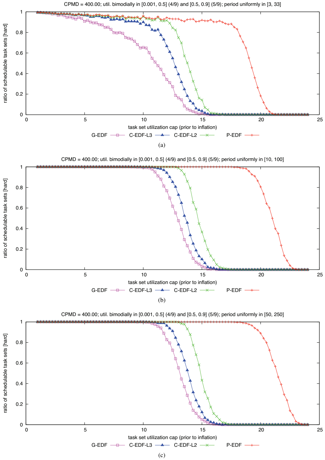
Figure 83: CPMD = 400.00. Hard W(D) schedulability of task sets with bimodal heavy per-task utilizations and (a) short, (b) moderate, and (c) long periods.
