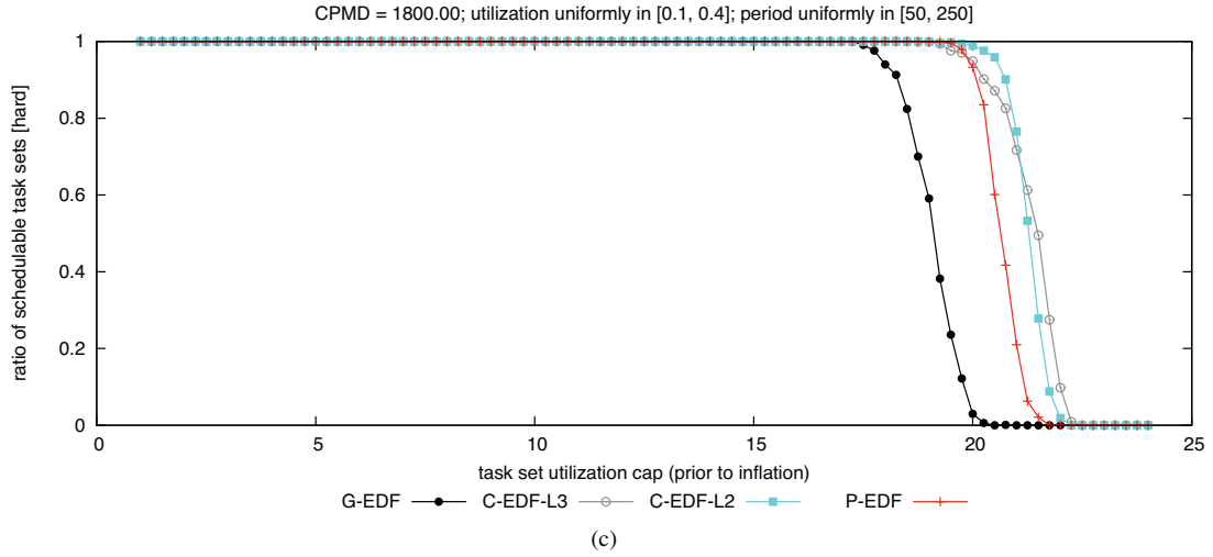
Figure 246: CPMD = 1800.00. Hard BF schedulability of task sets with uniform medium per-task utilizations and (a) short, (b) moderate, and (c) long periods.
