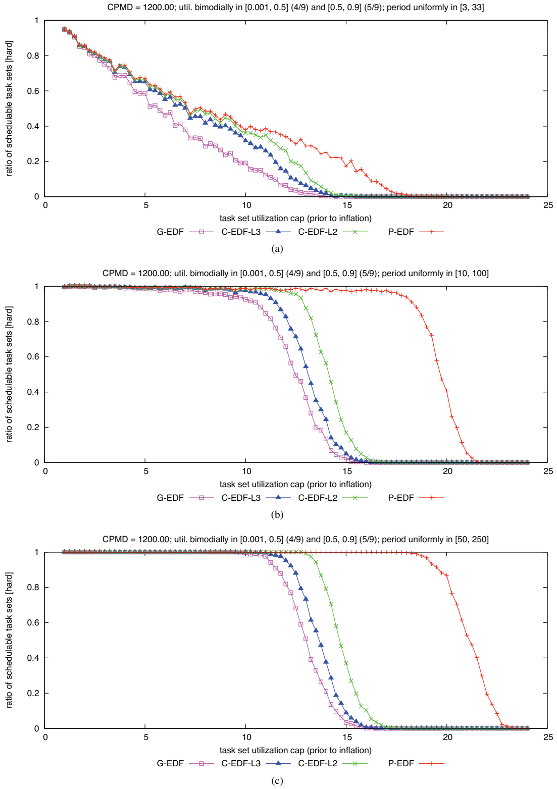
Figure 179: CPMD = 1200.00. Hard W(D) schedulability of task sets with bimodal heavy per-task utilizations and (a) short, (b) moderate, and (c) long periods.
