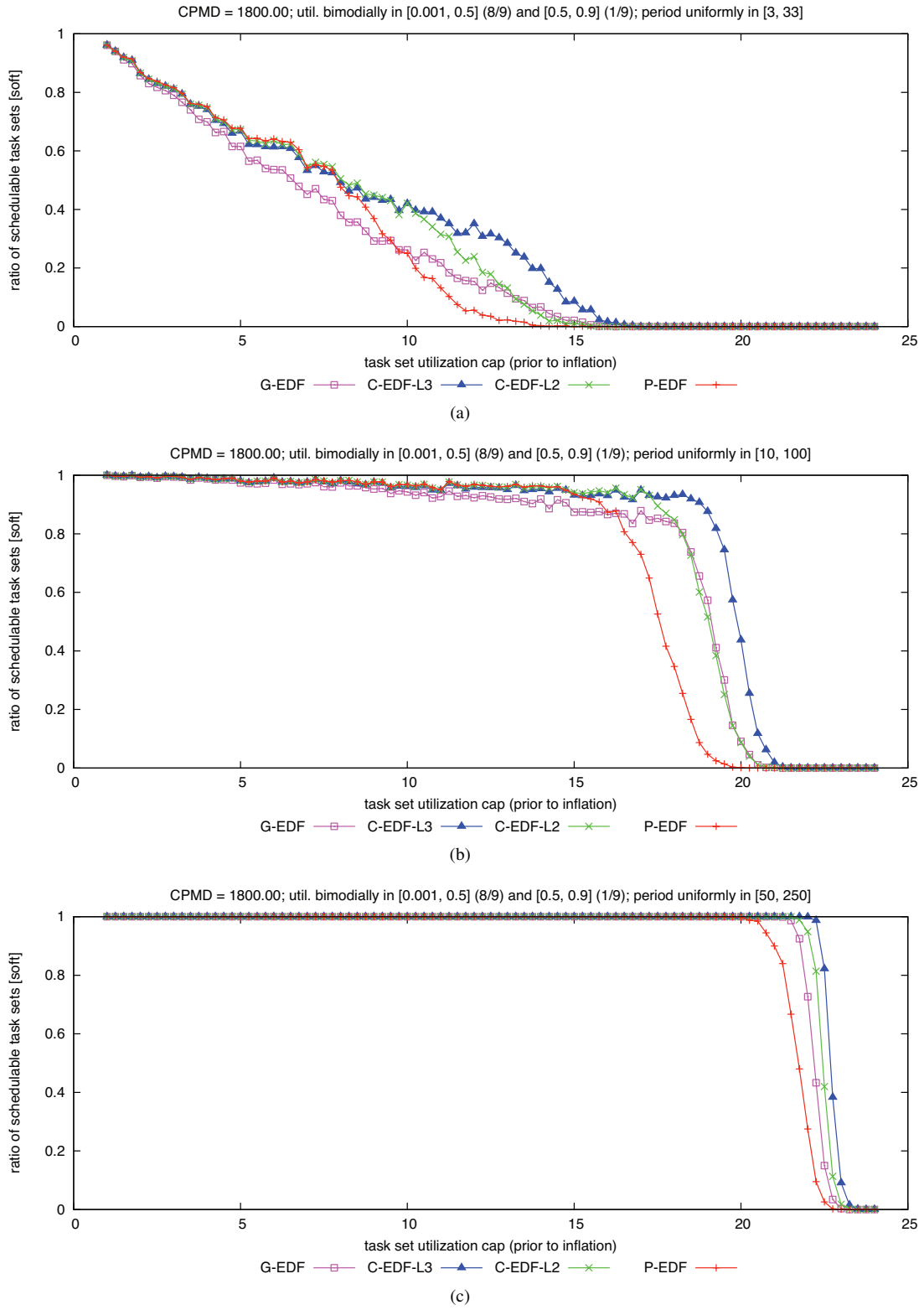
Figure 386: CPMD = 1800.00. Soft schedulability of task sets with bimodal light per-task utilizations and (a) short, (b) moderate, and (c) long periods.
