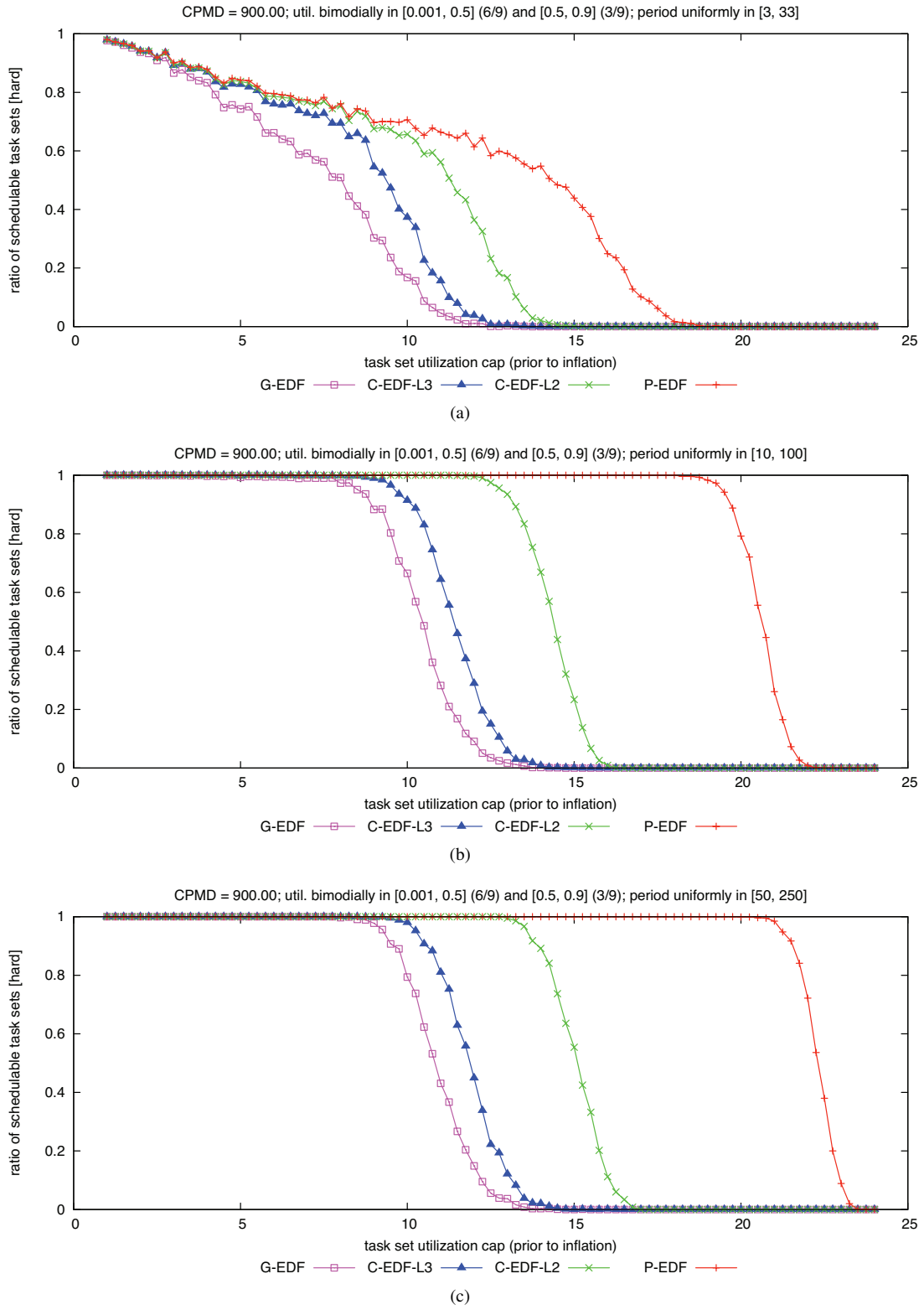
Figure 139: CPMD = 900.00. Hard W(D) schedulability of task sets with bimodal medium per-task utilizations and (a) short, (b) moderate, and (c) long periods.
