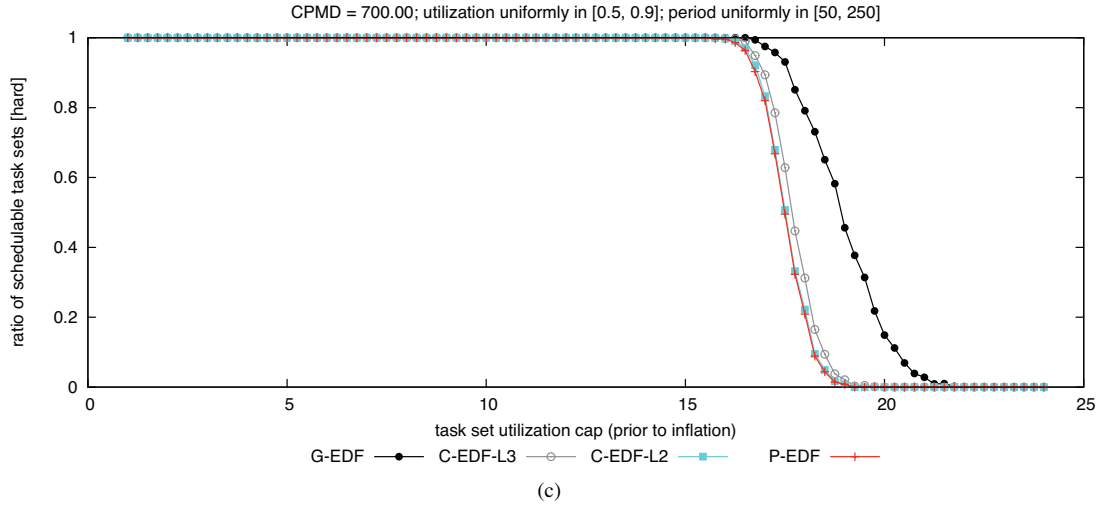
Figure 118: CPMD = 700.00. Hard BF schedulability of task sets with uniform heavy per-task utilizations and (a) short, (b) moderate, and (c) long periods.
