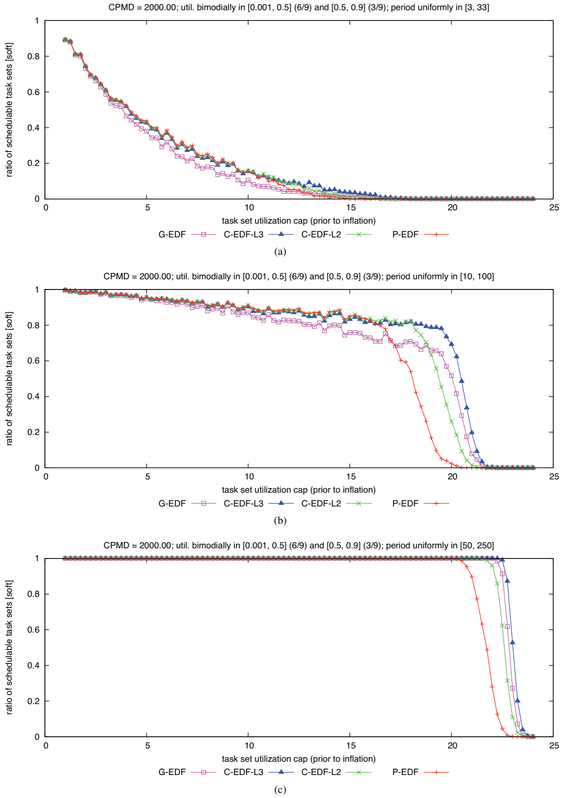
Figure 400: CPMD = 2000.00. Soft schedulability of task sets with bimodal medium per-task utilizations and (a) short, (b) moderate, and (c) long periods.
