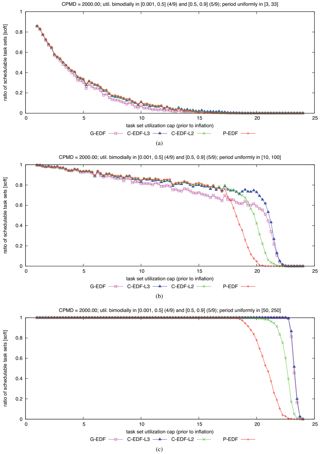
Figure 402: CPMD = 2000.00. Soft schedulability of task sets with bimodal heavy per-task utilizations and (a) short, (b) moderate, and (c) long periods.
