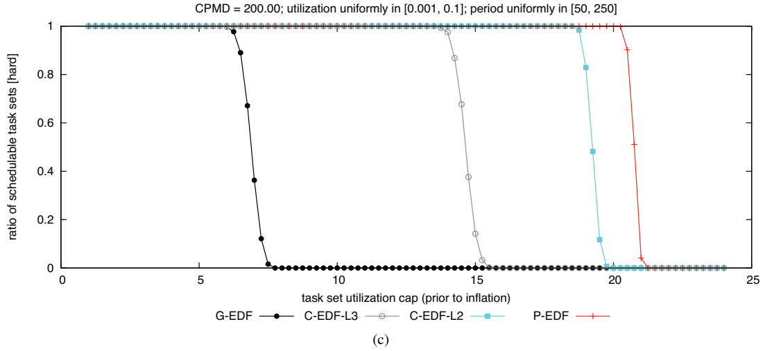
Figure 50: CPMD = 200.00. Hard BF schedulability of task sets with uniform light per-task utilizations and (a) short, (b) moderate, and (c) long periods.
