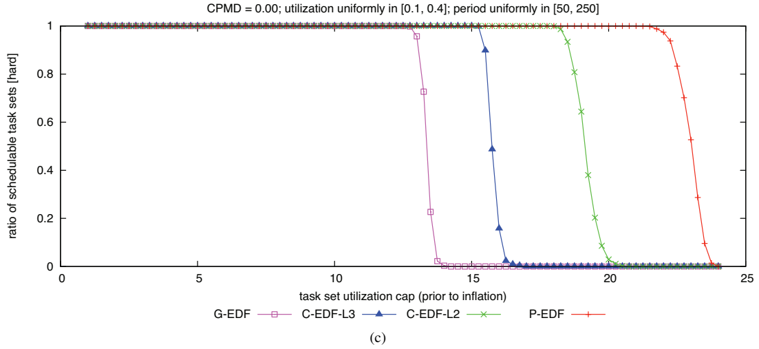
Figure 29: CPMD = 0.00. Hard W(D) schedulability of task sets with uniform medium per-task utilizations and (a) short, (b) moderate, and (c) long periods.
