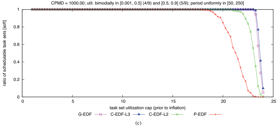
Figure 342: CPMD = 1000.00. Soft schedulability of task sets with bimodal heavy per-task utilizations and (a) short, (b) moderate, and (c) long periods.
