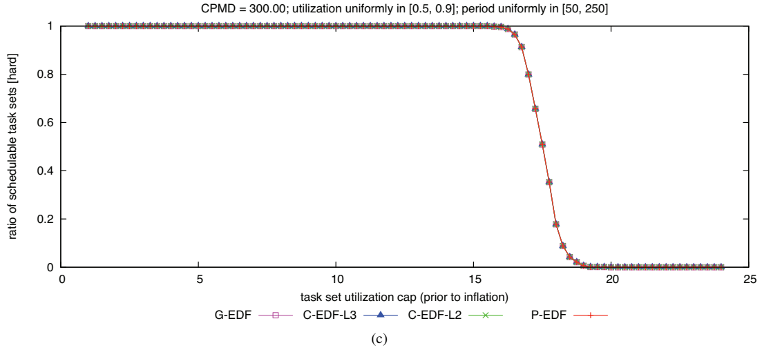
Figure 69: CPMD = 300.00. Hard W(D) schedulability of task sets with uniform heavy per-task utilizations and (a) short, (b) moderate, and (c) long periods.
