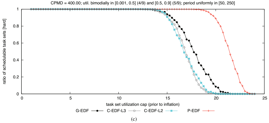
Figure 84: CPMD = 400.00. Hard BF schedulability of task sets with bimodal heavy per-task utilizations and (a) short, (b) moderate, and (c) long periods.
