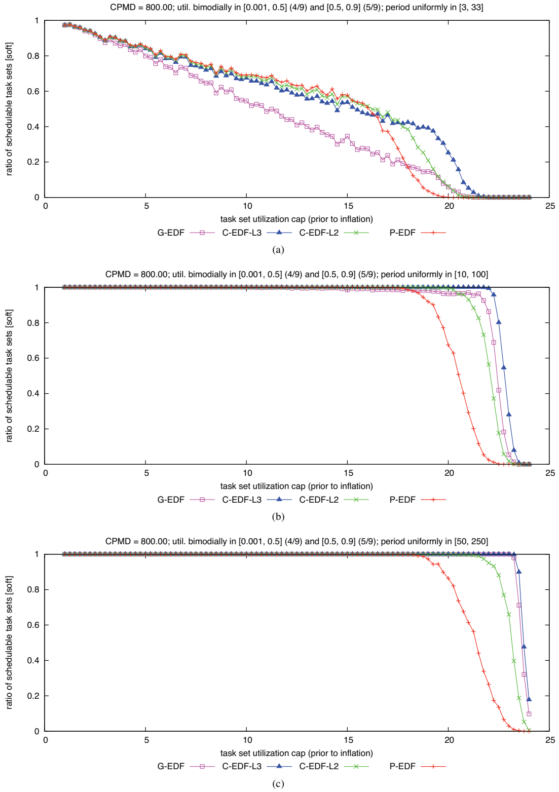
Figure 330: CPMD = 800.00. Soft schedulability of task sets with bimodal heavy per-task utilizations and (a) short, (b) moderate, and (c) long periods.
