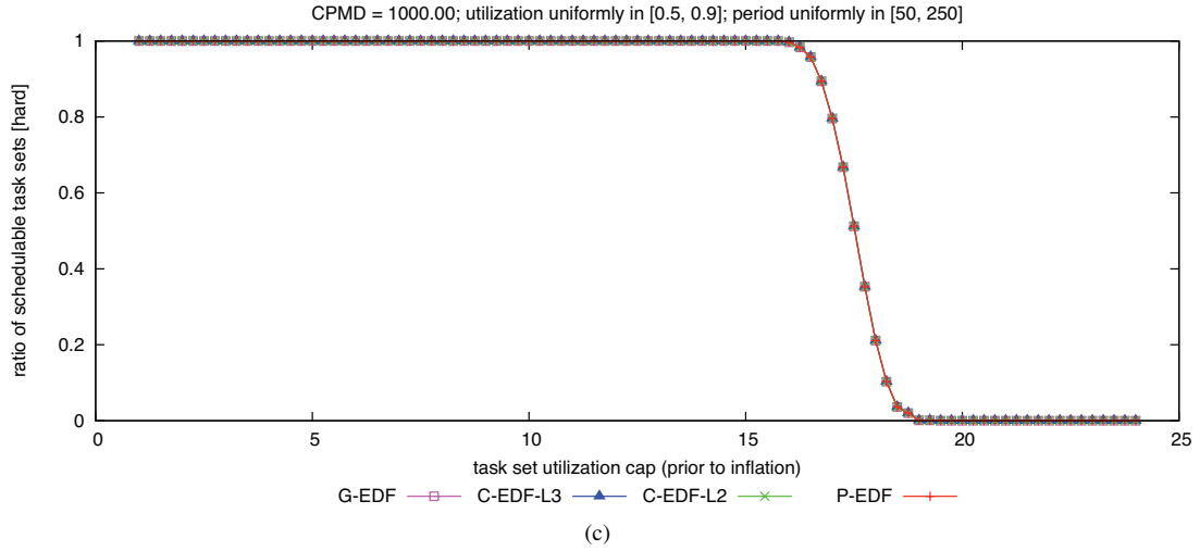
Figure 153: CPMD = 1000.00. Hard W(D) schedulability of task sets with uniform heavy per-task utilizations and (a) short, (b) moderate, and (c) long periods.
