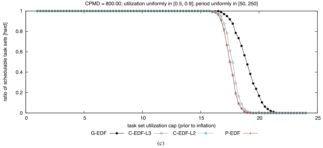
Figure 130: CPMD = 800.00. Hard BF schedulability of task sets with uniform heavy per-task utilizations and (a) short, (b) moderate, and (c) long periods.
