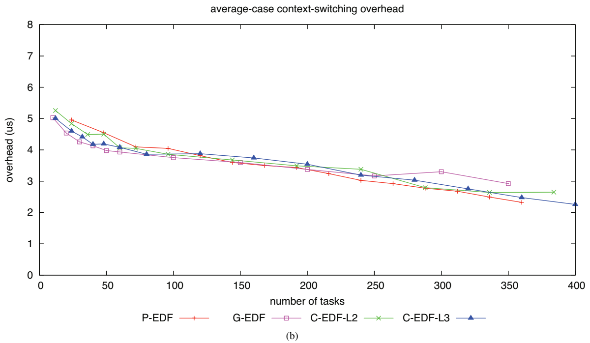
Figure 10: Measured context-switching overhead. (a) Measured worst case. (b) Measured average case.
