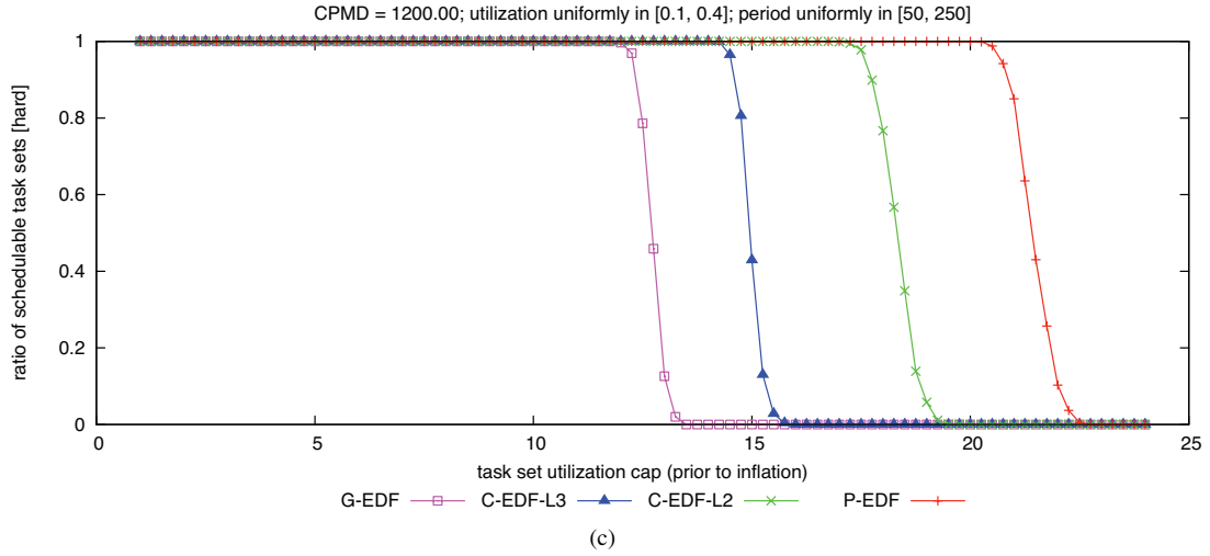
Figure 173: CPMD = 1200.00. Hard W(D) schedulability of task sets with uniform medium per-task utilizations and (a) short, (b) moderate, and (c) long periods.
