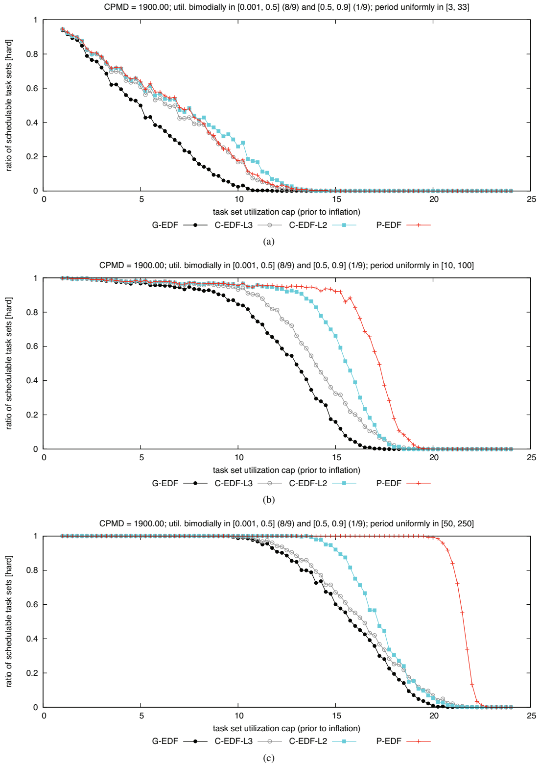
Figure 256: CPMD = 1900.00. Hard BF schedulability of task sets with bimodal light per-task utilizations and (a) short, (b) moderate, and (c) long periods.
