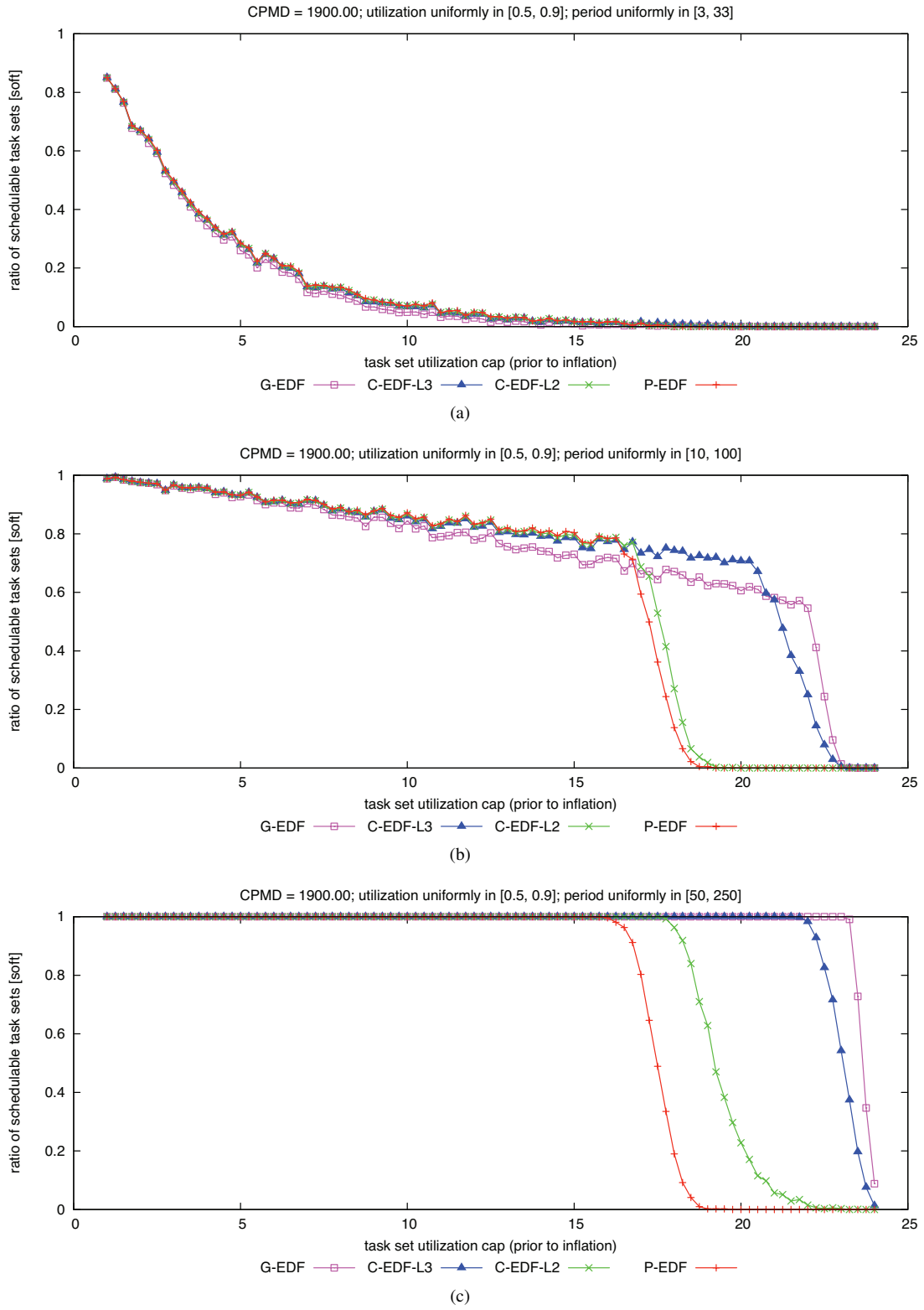
Figure 395: CPMD = 1900.00. Soft schedulability of task sets with uniform heavy per-task utilizations and (a) short, (b) moderate, and (c) long periods.
