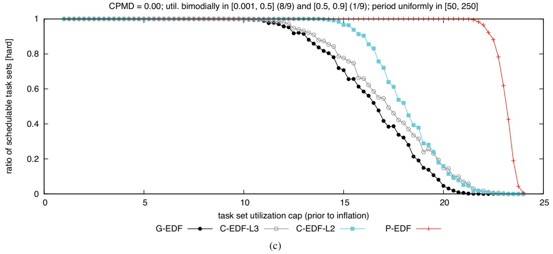
Figure 28: CPMD = 0.00. Hard BF schedulability of task sets with bimodal light per-task utilizations and (a) short, (b) moderate, and (c) long periods.
