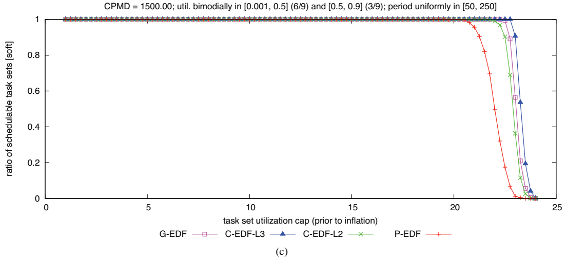
Figure 370: CPMD = 1500.00. Soft schedulability of task sets with bimodal medium per-task utilizations and (a) short, (b) moderate, and (c) long periods.
