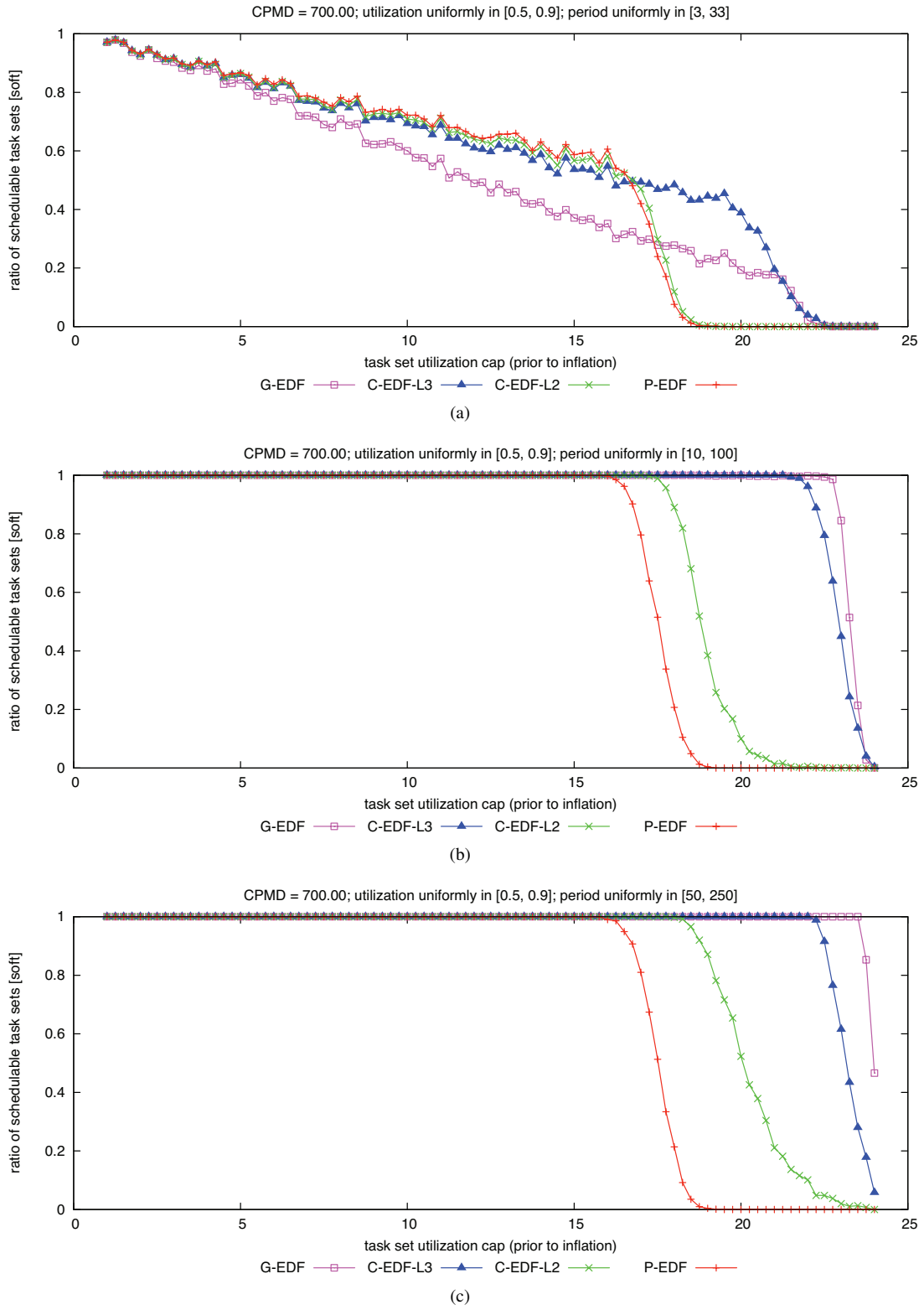
Figure 323: CPMD = 700.00. Soft schedulability of task sets with uniform heavy per-task utilizations and (a) short, (b) moderate, and (c) long periods.
