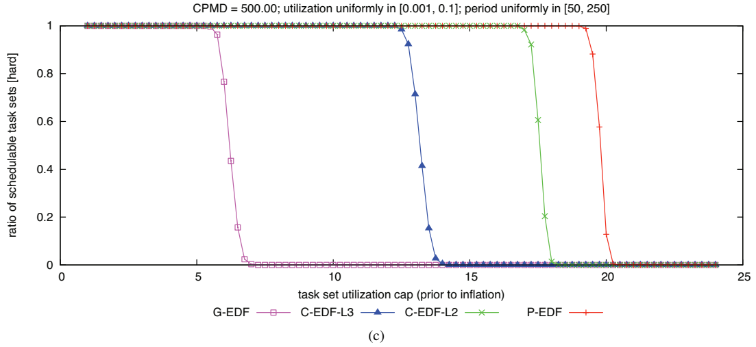
Figure 85: CPMD = 500.00. Hard W(D) schedulability of task sets with uniform light per-task utilizations and (a) short, (b) moderate, and (c) long periods.
