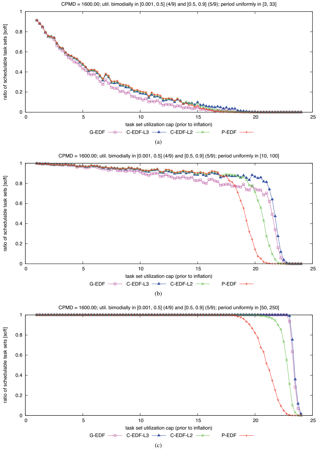
Figure 378: CPMD = 1600.00. Soft schedulability of task sets with bimodal heavy per-task utilizations and (a) short, (b) moderate, and (c) long periods.
