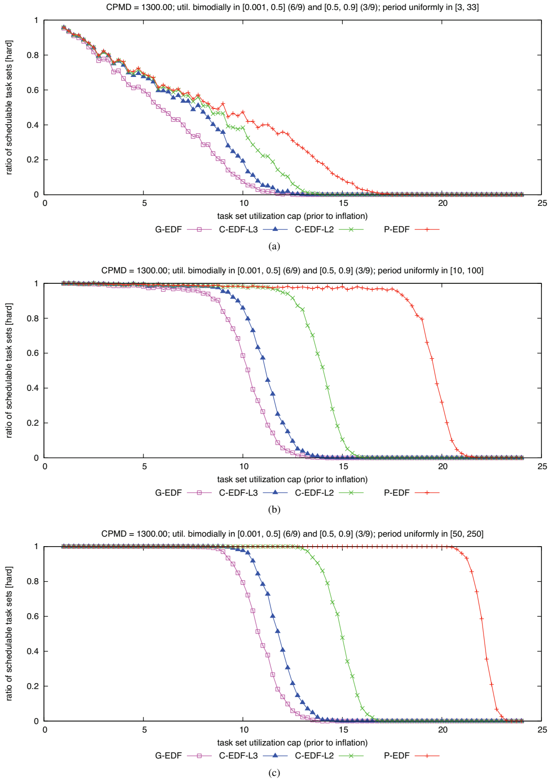
Figure 187: CPMD = 1300.00. Hard W(D) schedulability of task sets with bimodal medium per-task utilizations and (a) short, (b) moderate, and (c) long periods.
