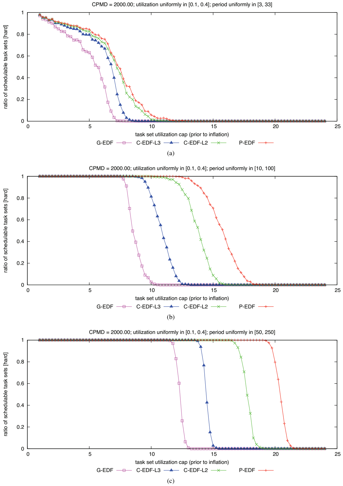
Figure 269: CPMD = 2000.00. Hard W(D) schedulability of task sets with uniform medium per-task utilizations and (a) short, (b) moderate, and (c) long periods.
