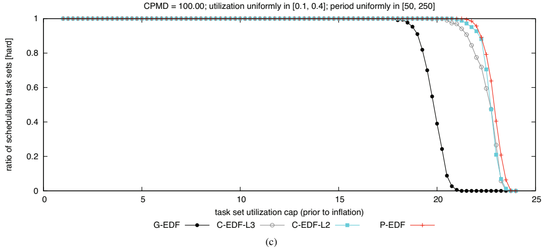
Figure 42: CPMD = 100.00. Hard BF schedulability of task sets with uniform medium per-task utilizations and (a) short, (b) moderate, and (c) long periods.
