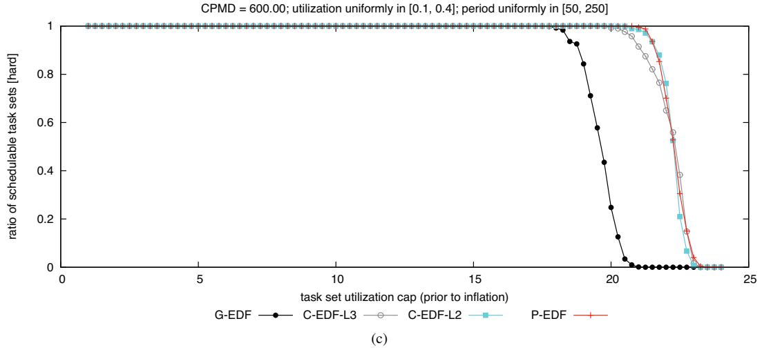
Figure 102: CPMD = 600.00. Hard BF schedulability of task sets with uniform medium per-task utilizations and (a) short, (b) moderate, and (c) long periods.
