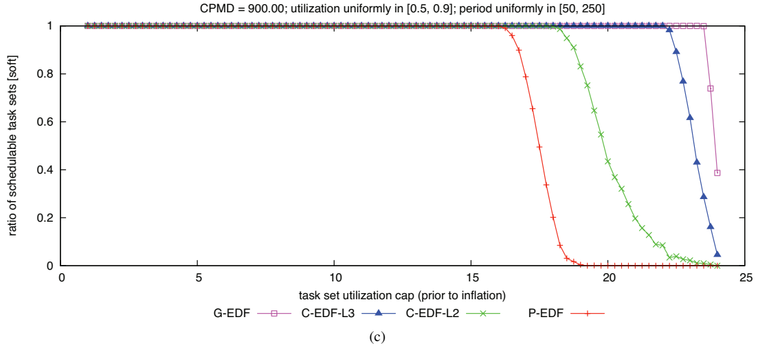
Figure 335: CPMD = 900.00. Soft schedulability of task sets with uniform heavy per-task utilizations and (a) short, (b) moderate, and (c) long periods.
