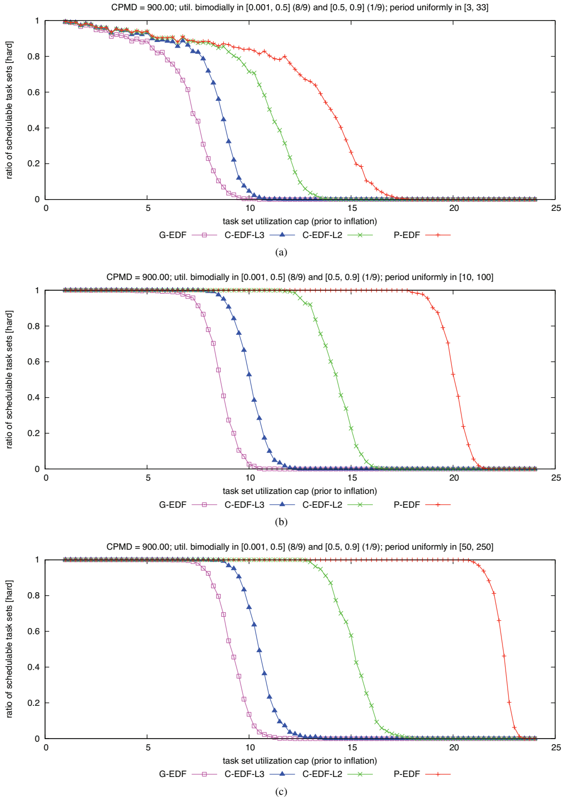
Figure 135: CPMD = 900.00. Hard W(D) schedulability of task sets with bimodal light per-task utilizations and (a) short, (b) moderate, and (c) long periods.
