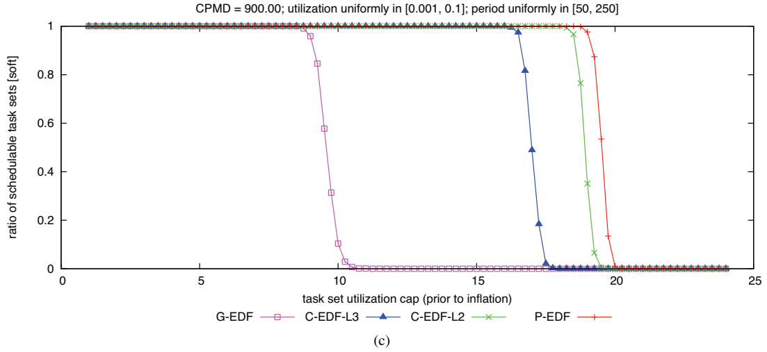
Figure 331: CPMD = 900.00. Soft schedulability of task sets with uniform light per-task utilizations and (a) short, (b) moderate, and (c) long periods.
