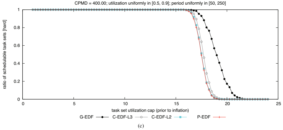
Figure 82: CPMD = 400.00. Hard BF schedulability of task sets with uniform heavy per-task utilizations and (a) short, (b) moderate, and (c) long periods.
