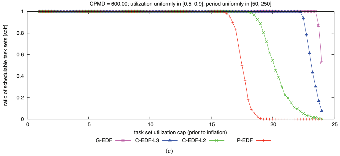
Figure 317: CPMD = 600.00. Soft schedulability of task sets with uniform heavy per-task utilizations and (a) short, (b) moderate, and (c) long periods.
