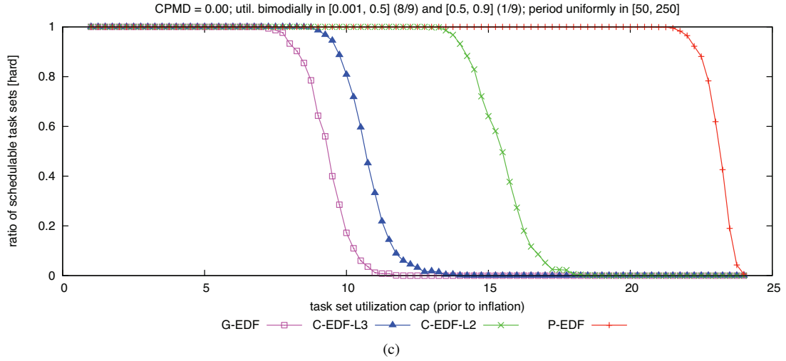
Figure 27: CPMD = 0.00. Hard W(D) schedulability of task sets with bimodal light per-task utilizations and (a) short, (b) moderate, and (c) long periods.
