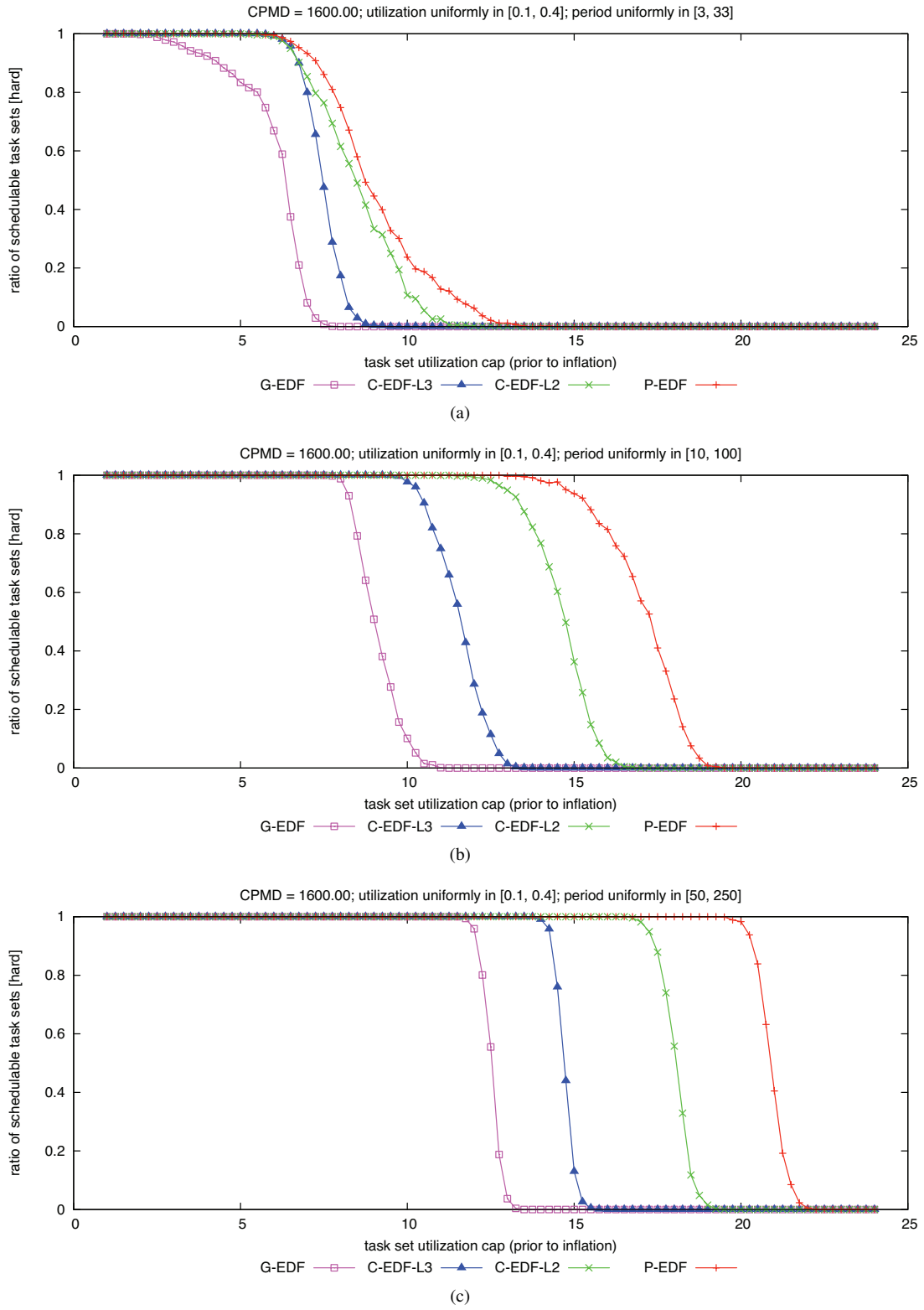
Figure 221: CPMD = 1600.00. Hard W(D) schedulability of task sets with uniform medium per-task utilizations and (a) short, (b) moderate, and (c) long periods.
