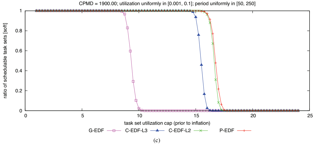
Figure 391: CPMD = 1900.00. Soft schedulability of task sets with uniform light per-task utilizations and (a) short, (b) moderate, and (c) long periods.
