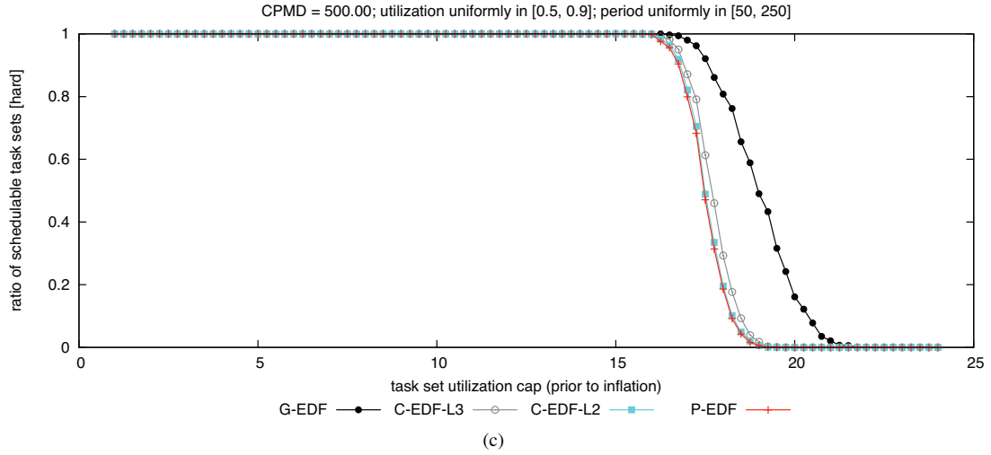
Figure 94: CPMD = 500.00. Hard BF schedulability of task sets with uniform heavy per-task utilizations and (a) short, (b) moderate, and (c) long periods.
