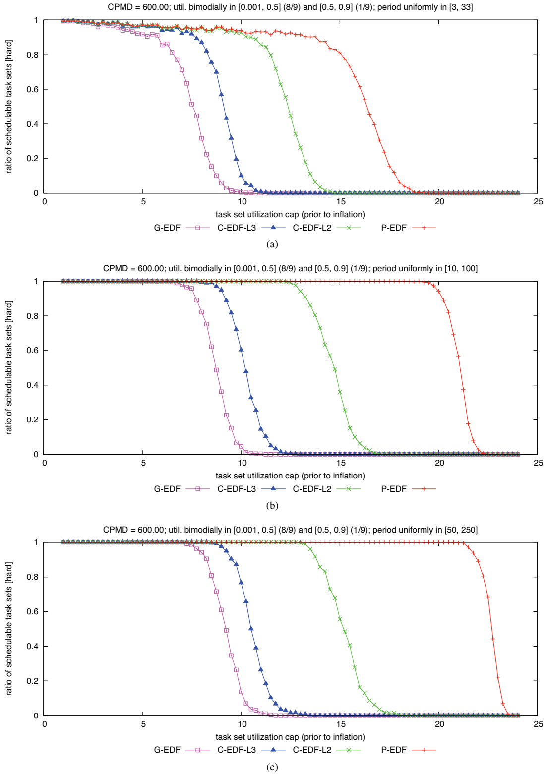
Figure 99: CPMD = 600.00. Hard W(D) schedulability of task sets with bimodal light per-task utilizations and (a) short, (b) moderate, and (c) long periods.
