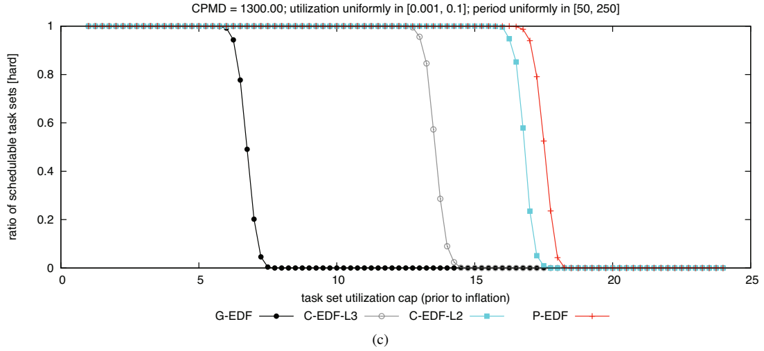
Figure 182: CPMD = 1300.00. Hard BF schedulability of task sets with uniform light per-task utilizations and (a) short, (b) moderate, and (c) long periods.
