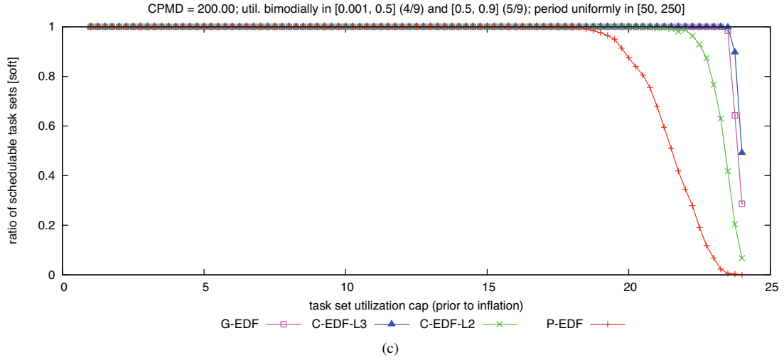
Figure 294: CPMD = 200.00. Soft schedulability of task sets with bimodal heavy per-task utilizations and (a) short, (b) moderate, and (c) long periods.
