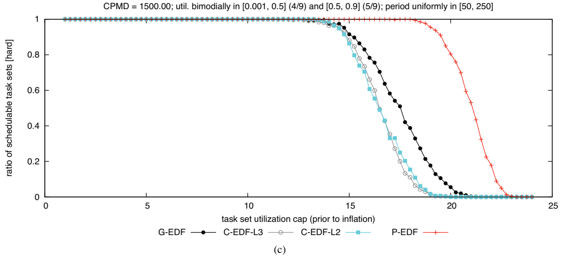
Figure 216: CPMD = 1500.00. Hard BF schedulability of task sets with bimodal heavy per-task utilizations and (a) short, (b) moderate, and (c) long periods.
