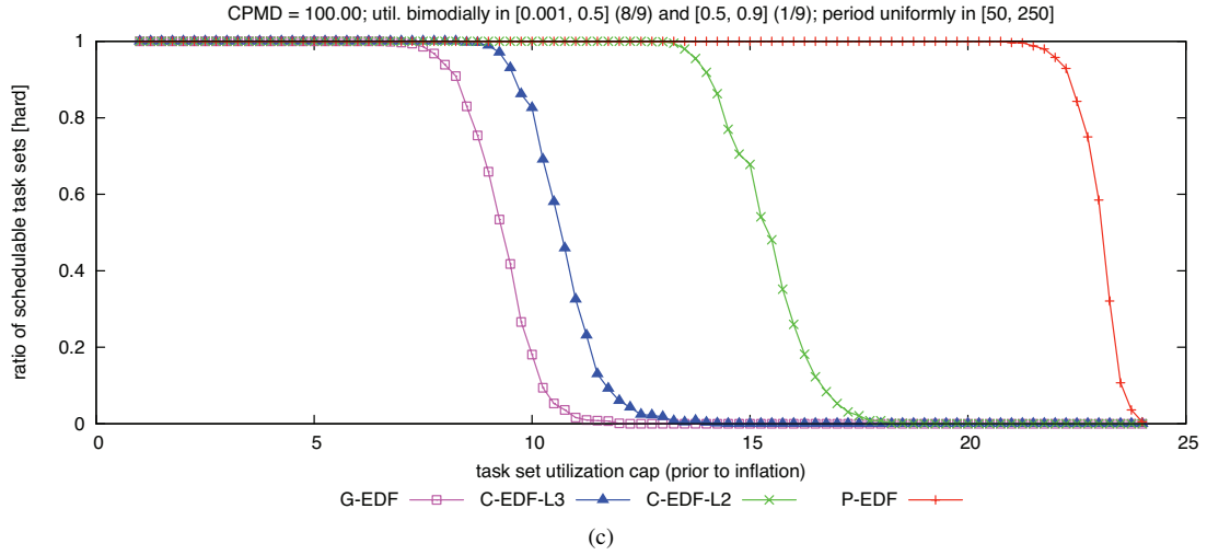
Figure 39: CPMD = 100.00. Hard W(D) schedulability of task sets with bimodal light per-task utilizations and (a) short, (b) moderate, and (c) long periods.
