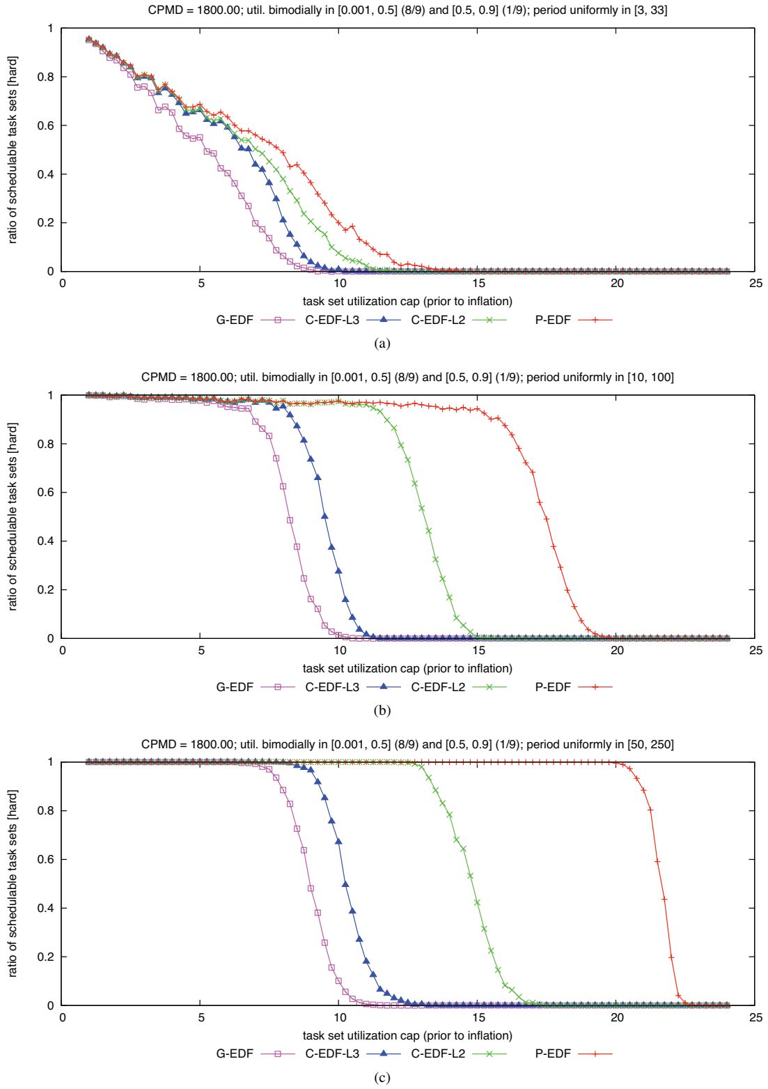
Figure 243: CPMD = 1800.00. Hard W(D) schedulability of task sets with bimodal light per-task utilizations and (a) short, (b) moderate, and (c) long periods.
