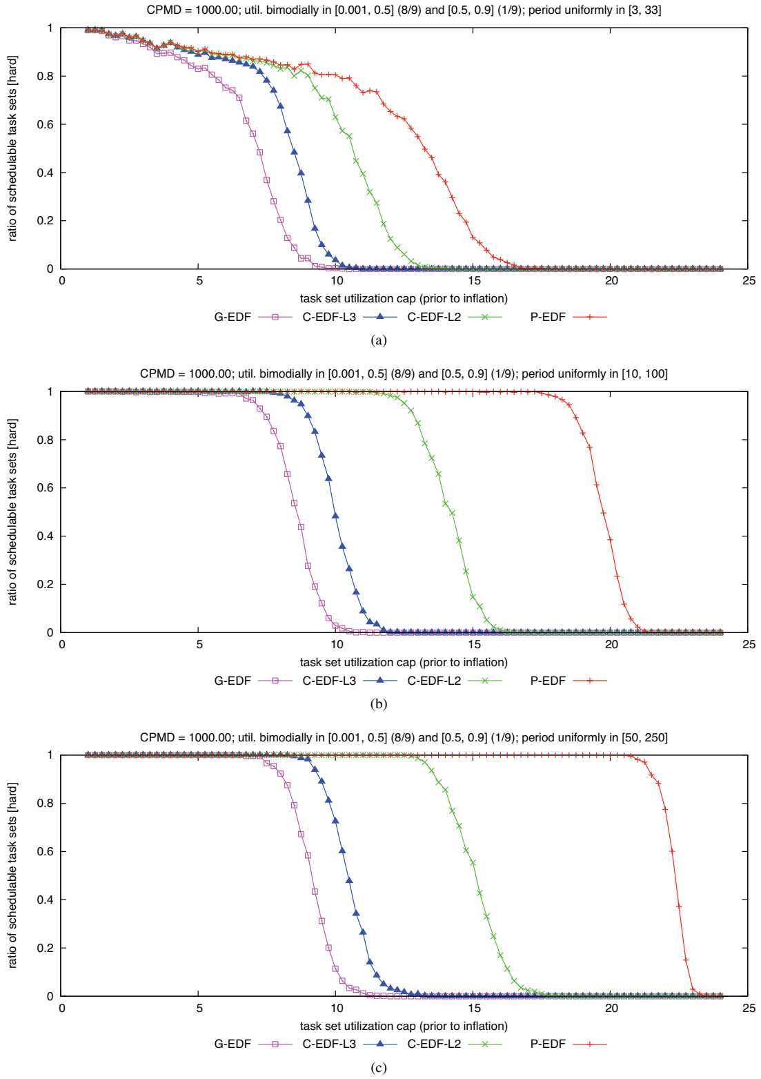
Figure 147: CPMD = 1000.00. Hard W(D) schedulability of task sets with bimodal light per-task utilizations and (a) short, (b) moderate, and (c) long periods.
