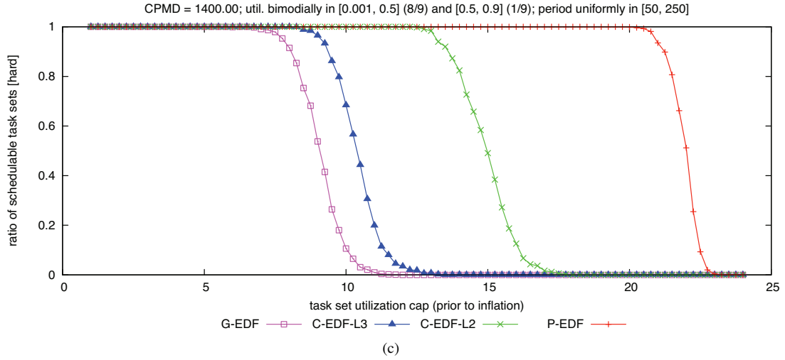
Figure 195: CPMD = 1400.00. Hard W(D) schedulability of task sets with bimodal light per-task utilizations and (a) short, (b) moderate, and (c) long periods.
