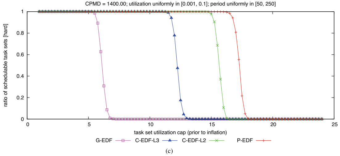
Figure 193: CPMD = 1400.00. Hard W(D) schedulability of task sets with uniform light per-task utilizations and (a) short, (b) moderate, and (c) long periods.
