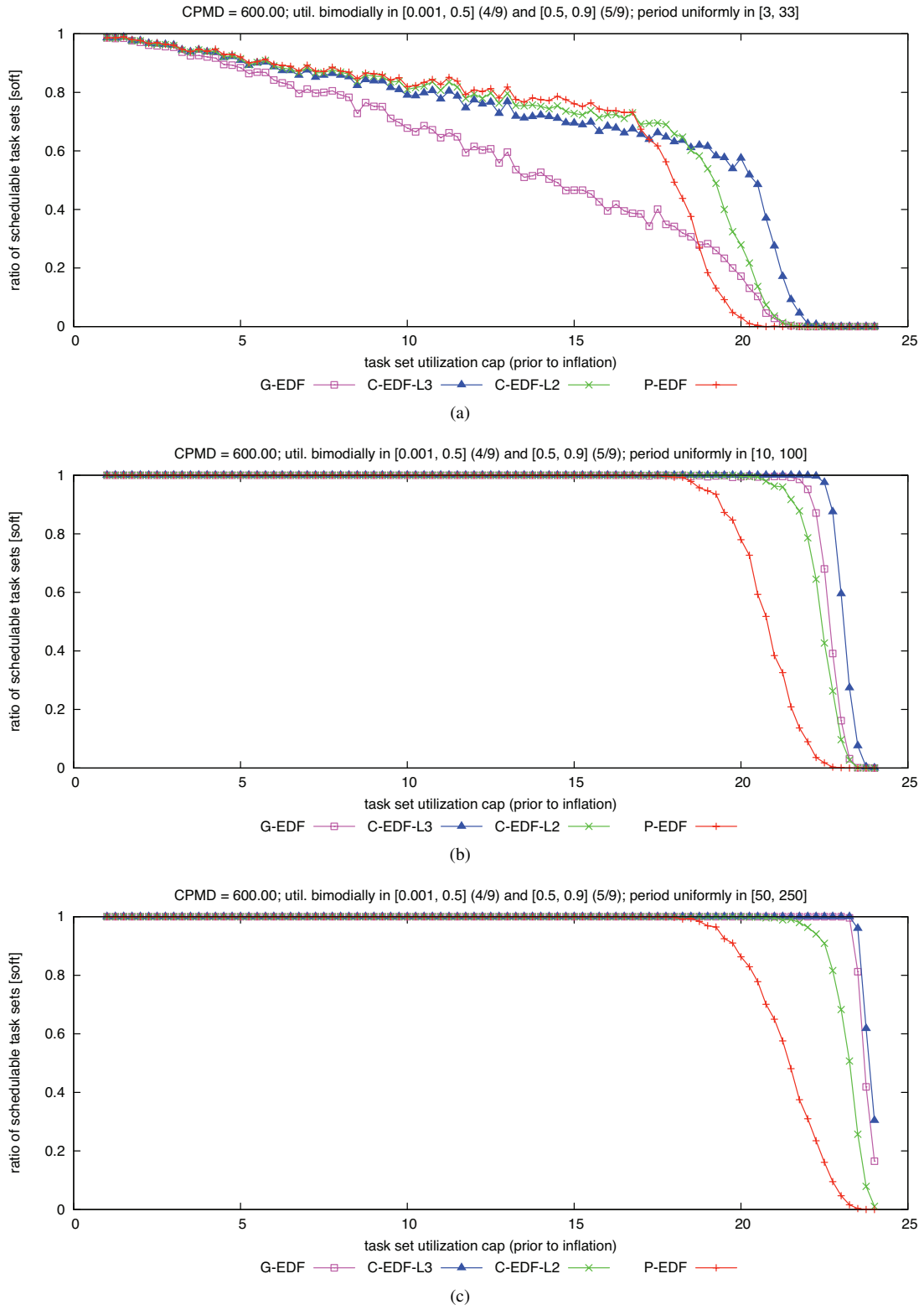
Figure 318: CPMD = 600.00. Soft schedulability of task sets with bimodal heavy per-task utilizations and (a) short, (b) moderate, and (c) long periods.
