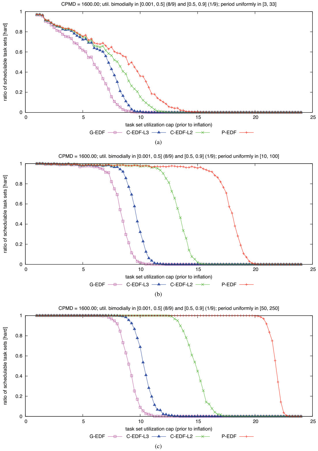
Figure 219: CPMD = 1600.00. Hard W(D) schedulability of task sets with bimodal light per-task utilizations and (a) short, (b) moderate, and (c) long periods.
