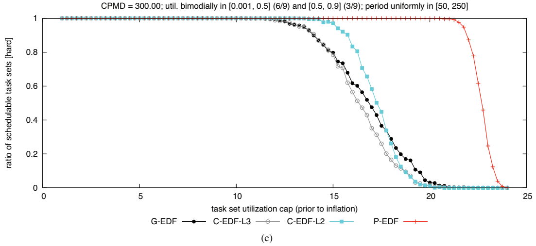
Figure 68: CPMD = 300.00. Hard BF schedulability of task sets with bimodal medium per-task utilizations and (a) short, (b) moderate, and (c) long periods.
