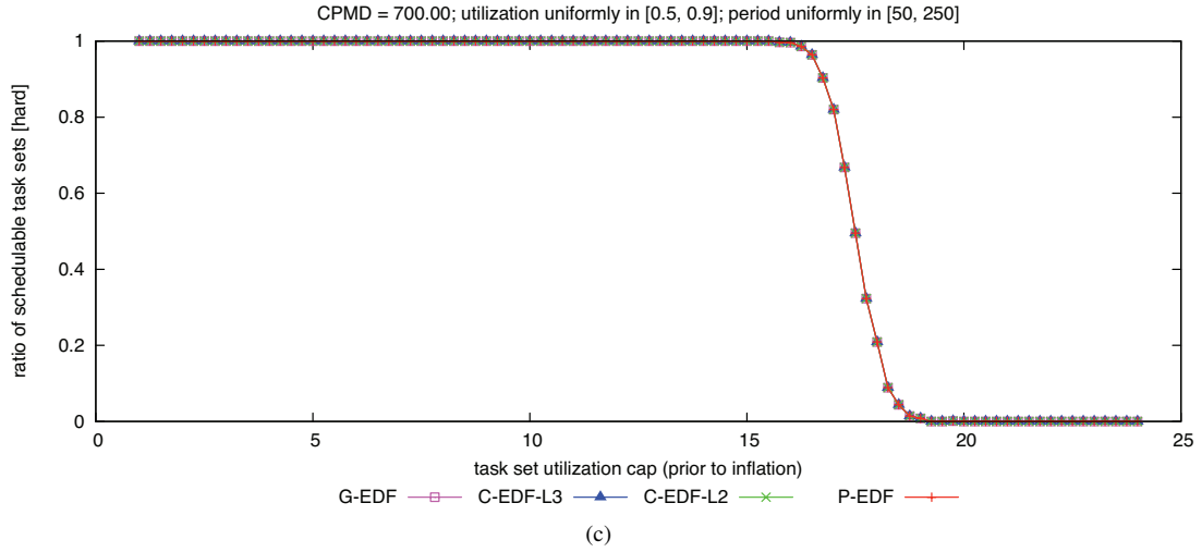
Figure 117: CPMD = 700.00. Hard W(D) schedulability of task sets with uniform heavy per-task utilizations and (a) short, (b) moderate, and (c) long periods.
