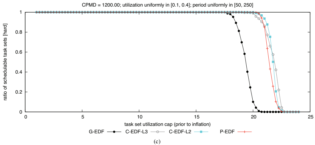
Figure 174: CPMD = 1200.00. Hard BF schedulability of task sets with uniform medium per-task utilizations and (a) short, (b) moderate, and (c) long periods.
