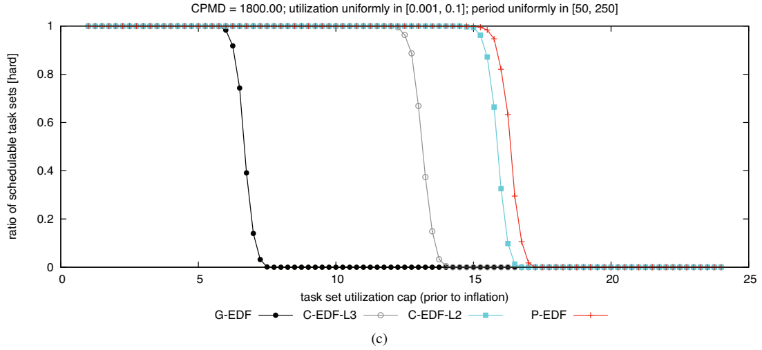
Figure 242: CPMD = 1800.00. Hard BF schedulability of task sets with uniform light per-task utilizations and (a) short, (b) moderate, and (c) long periods.
