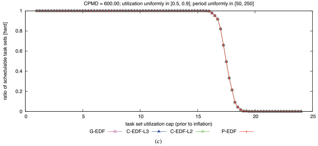
Figure 105: CPMD = 600.00. Hard W(D) schedulability of task sets with uniform heavy per-task utilizations and (a) short, (b) moderate, and (c) long periods.
