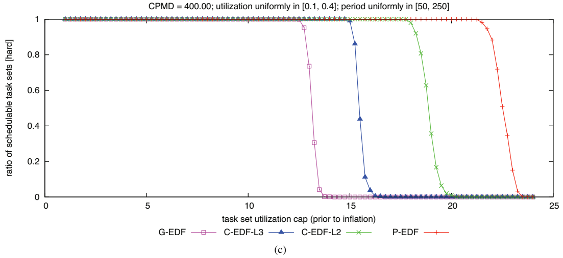
Figure 77: CPMD = 400.00. Hard W(D) schedulability of task sets with uniform medium per-task utilizations and (a) short, (b) moderate, and (c) long periods.
