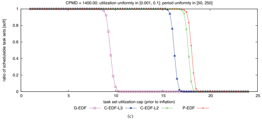
Figure 361: CPMD = 1400.00. Soft schedulability of task sets with uniform light per-task utilizations and (a) short, (b) moderate, and (c) long periods.
