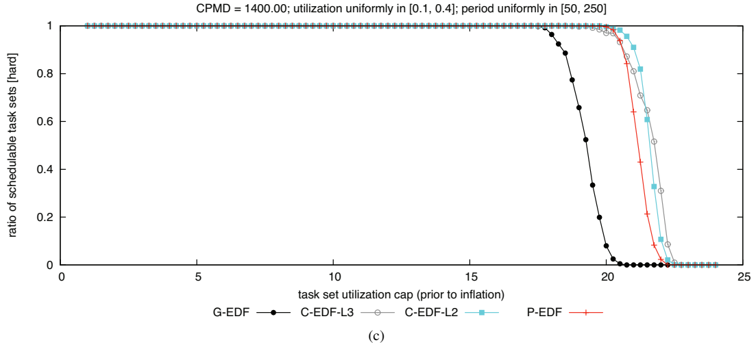
Figure 198: CPMD = 1400.00. Hard BF schedulability of task sets with uniform medium per-task utilizations and (a) short, (b) moderate, and (c) long periods.
