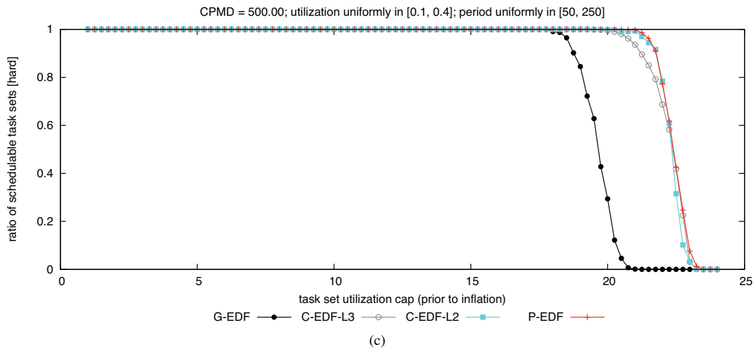
Figure 90: CPMD = 500.00. Hard BF schedulability of task sets with uniform medium per-task utilizations and (a) short, (b) moderate, and (c) long periods.
