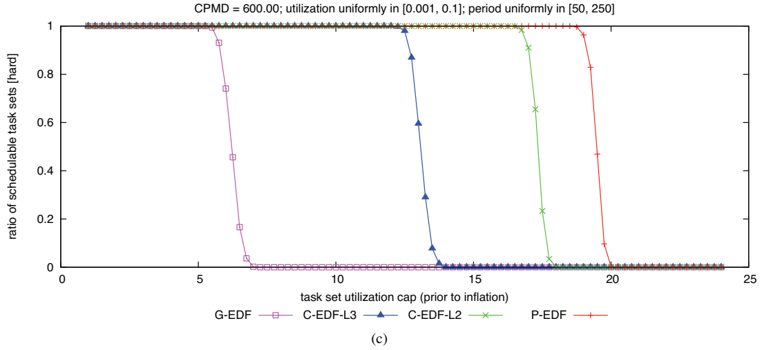
Figure 97: CPMD = 600.00. Hard W(D) schedulability of task sets with uniform light per-task utilizations and (a) short, (b) moderate, and (c) long periods.
