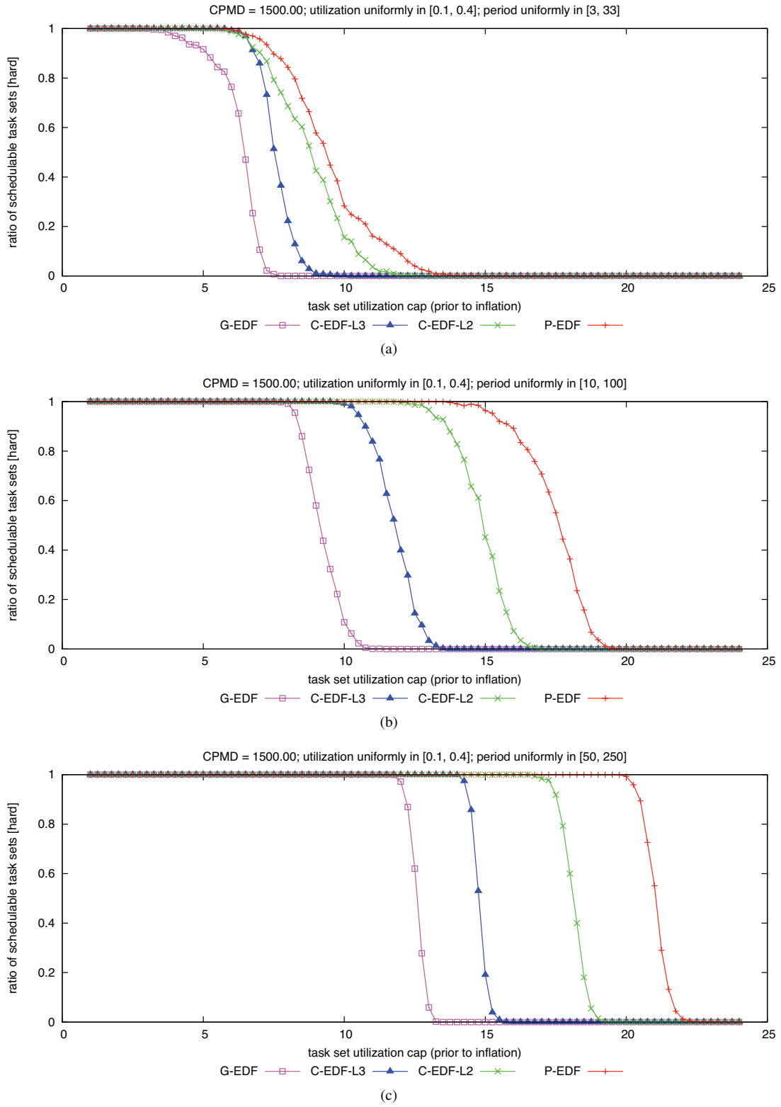
Figure 209: CPMD = 1500.00. Hard W(D) schedulability of task sets with uniform medium per-task utilizations and (a) short, (b) moderate, and (c) long periods.
