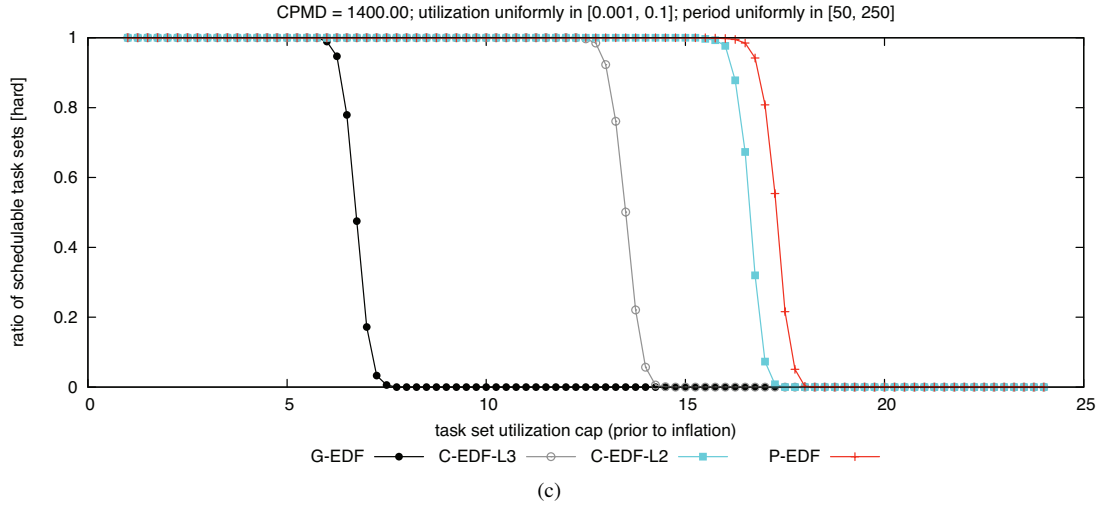
Figure 194: CPMD = 1400.00. Hard BF schedulability of task sets with uniform light per-task utilizations and (a) short, (b) moderate, and (c) long periods.
