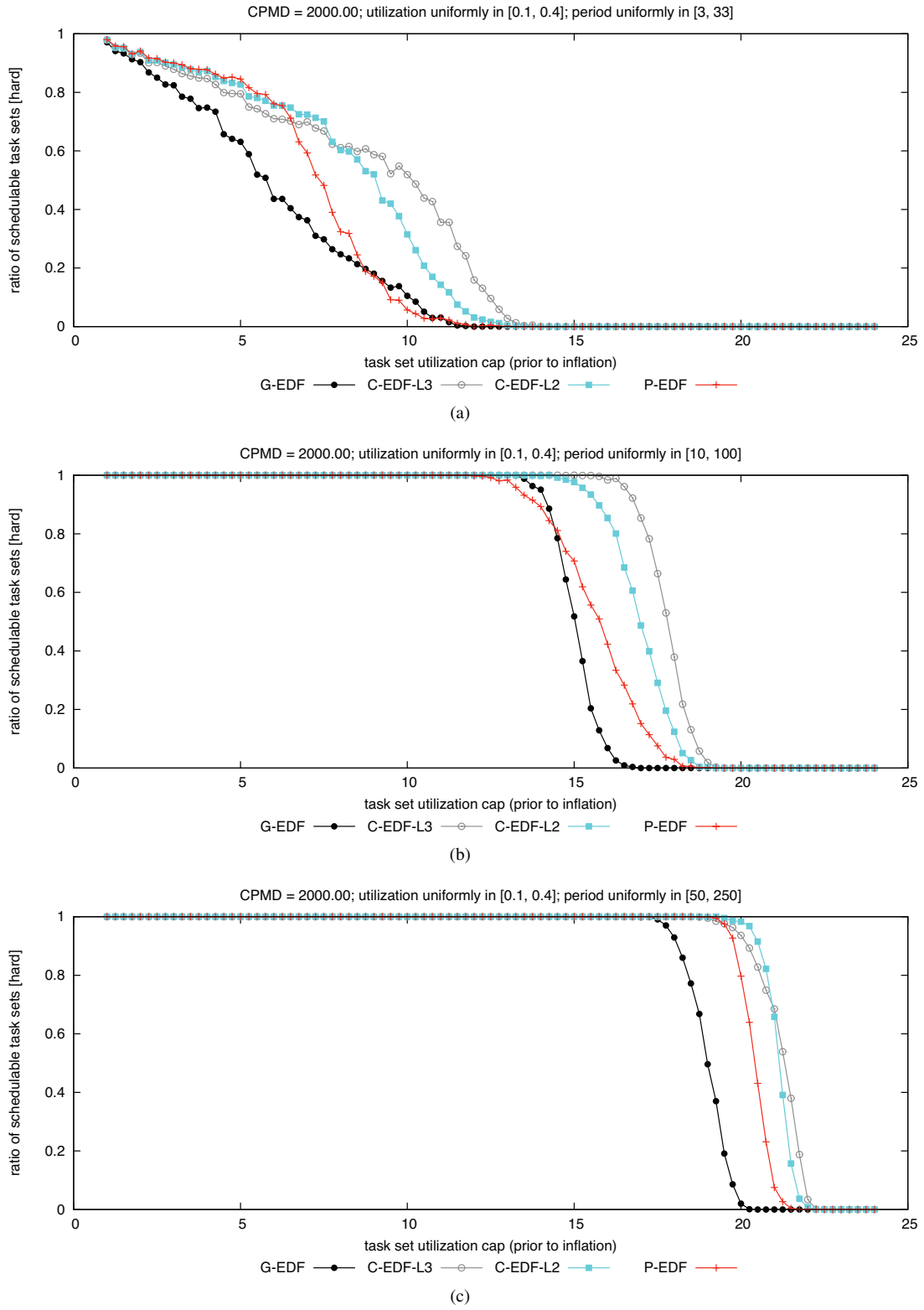
Figure 270: CPMD = 2000.00. Hard BF schedulability of task sets with uniform medium per-task utilizations and (a) short, (b) moderate, and (c) long periods.
