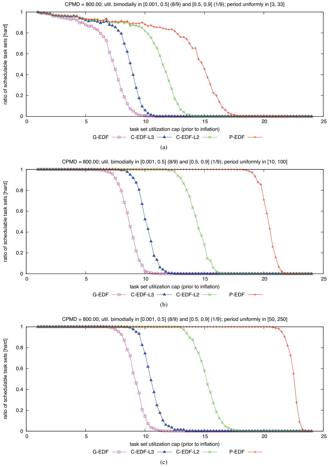
Figure 123: CPMD = 800.00. Hard W(D) schedulability of task sets with bimodal light per-task utilizations and (a) short, (b) moderate, and (c) long periods.
