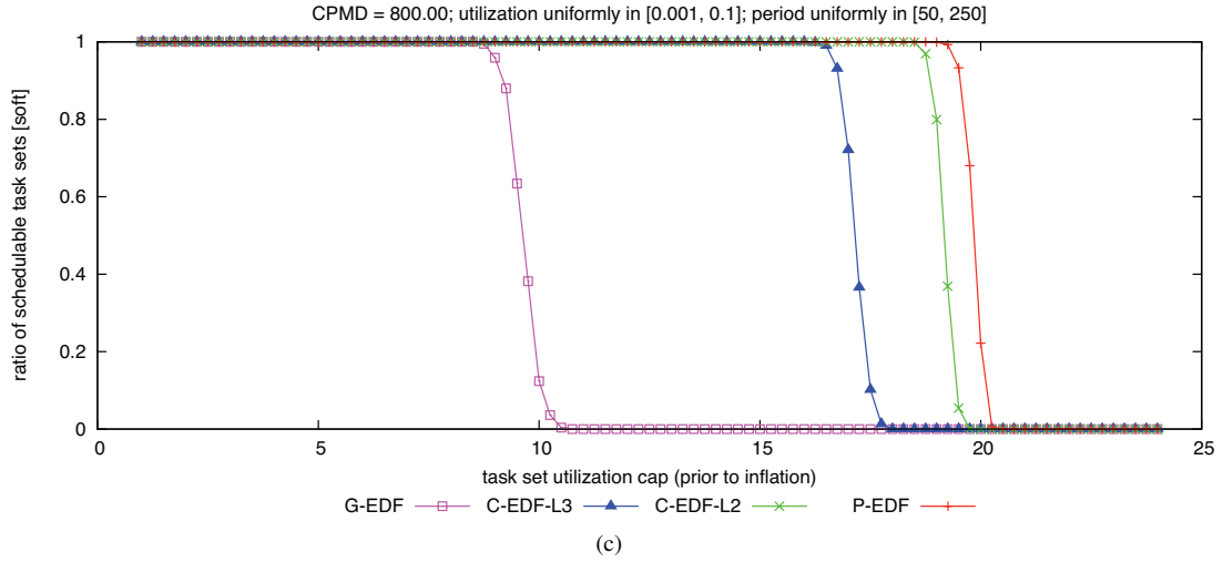
Figure 325: CPMD = 800.00. Soft schedulability of task sets with uniform light per-task utilizations and (a) short, (b) moderate, and (c) long periods.
