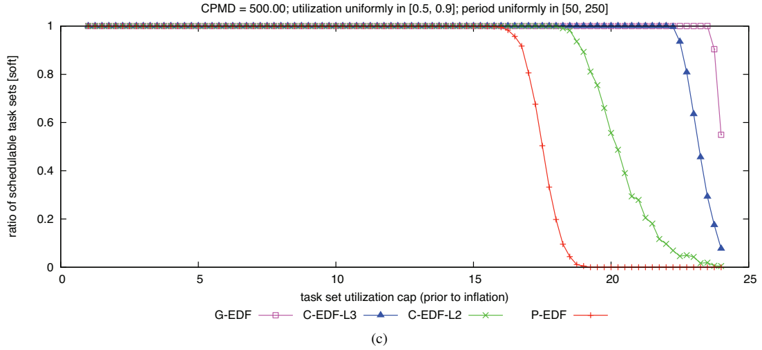
Figure 311: CPMD = 500.00. Soft schedulability of task sets with uniform heavy per-task utilizations and (a) short, (b) moderate, and (c) long periods.
