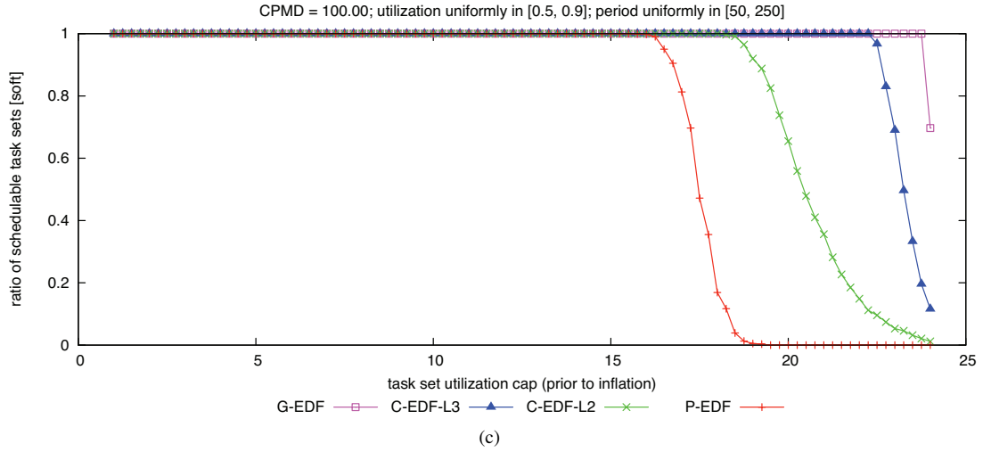
Figure 287: CPMD = 100.00. Soft schedulability of task sets with uniform heavy per-task utilizations and (a) short, (b) moderate, and (c) long periods.
