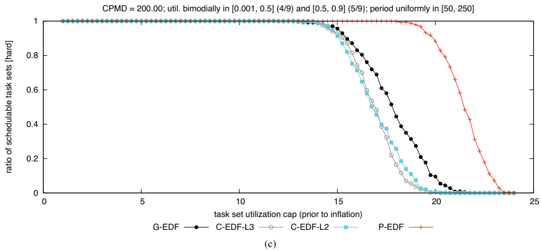
Figure 60: CPMD = 200.00. Hard BF schedulability of task sets with bimodal heavy per-task utilizations and (a) short, (b) moderate, and (c) long periods.
