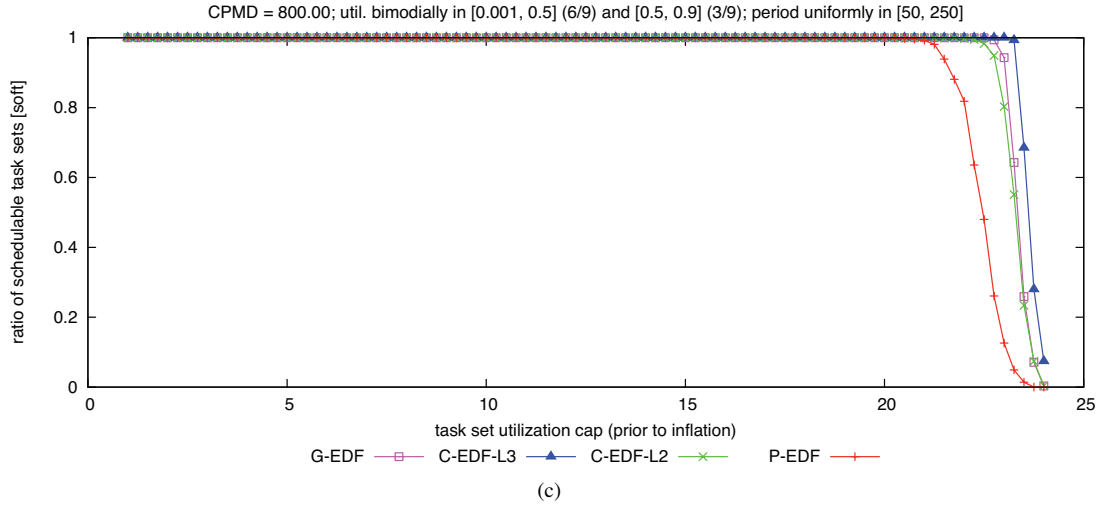
Figure 328: CPMD = 800.00. Soft schedulability of task sets with bimodal medium per-task utilizations and (a) short, (b) moderate, and (c) long periods.
