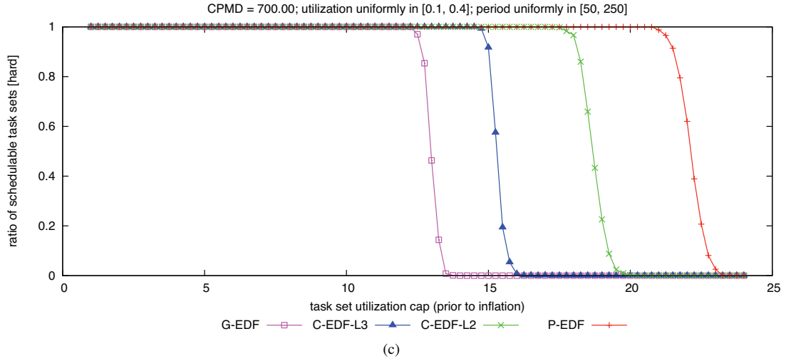
Figure 113: CPMD = 700.00. Hard W(D) schedulability of task sets with uniform medium per-task utilizations and (a) short, (b) moderate, and (c) long periods.
