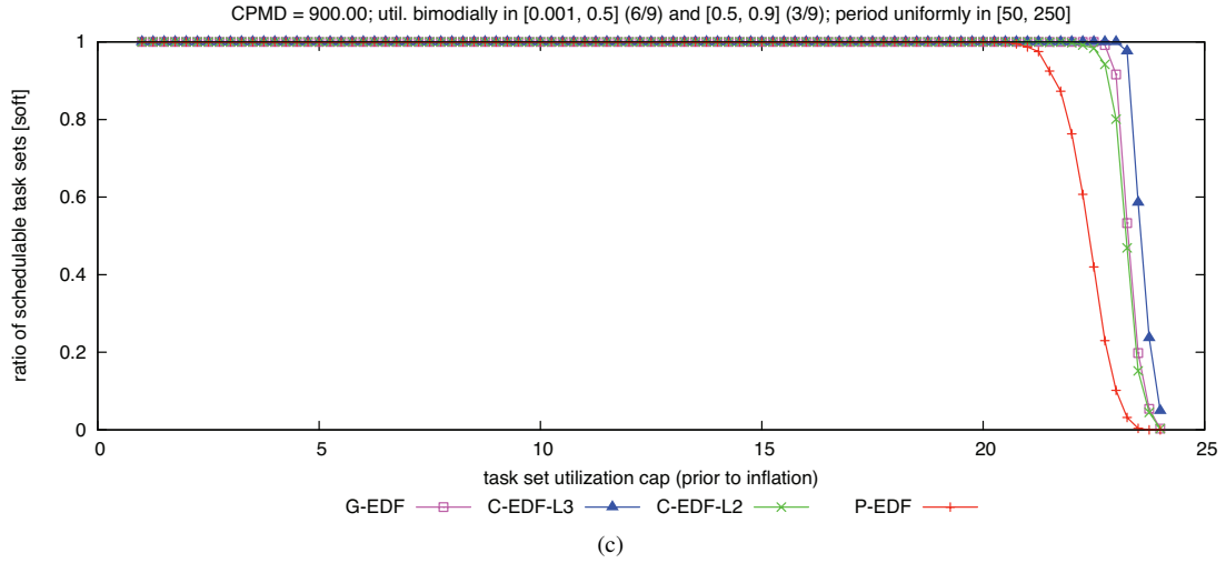
Figure 334: CPMD = 900.00. Soft schedulability of task sets with bimodal medium per-task utilizations and (a) short, (b) moderate, and (c) long periods.
