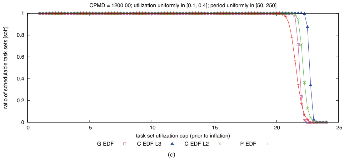
Figure 351: CPMD = 1200.00. Soft schedulability of task sets with uniform medium per-task utilizations and (a) short, (b) moderate, and (c) long periods.
