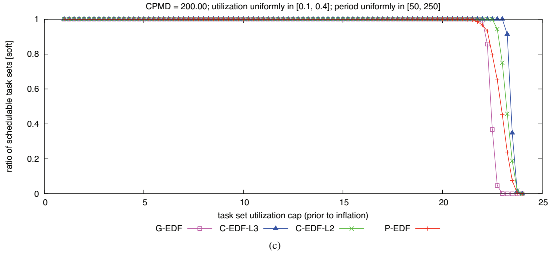
Figure 291: CPMD = 200.00. Soft schedulability of task sets with uniform medium per-task utilizations and (a) short, (b) moderate, and (c) long periods.
