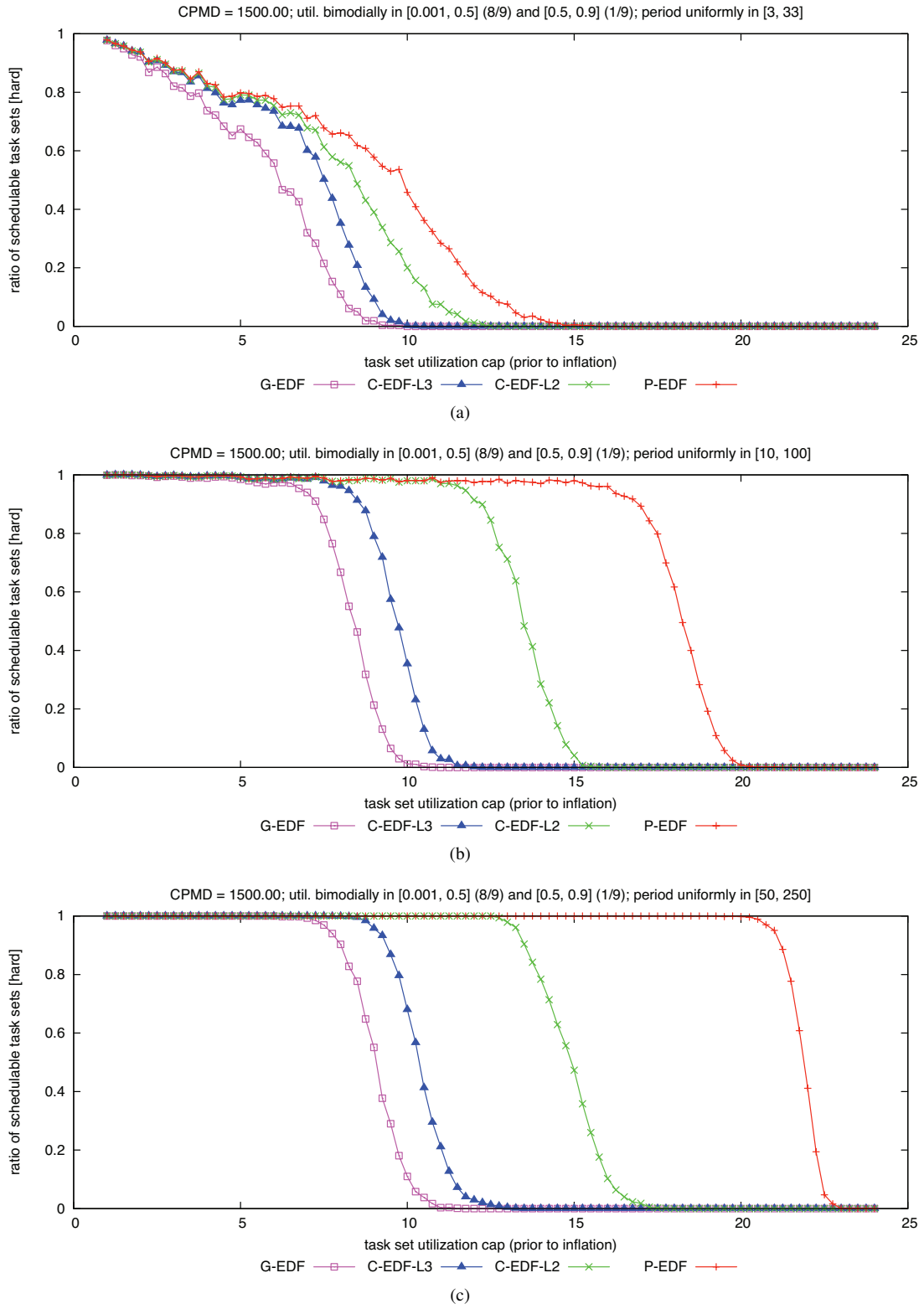
Figure 207: CPMD = 1500.00. Hard W(D) schedulability of task sets with bimodal light per-task utilizations and (a) short, (b) moderate, and (c) long periods.
