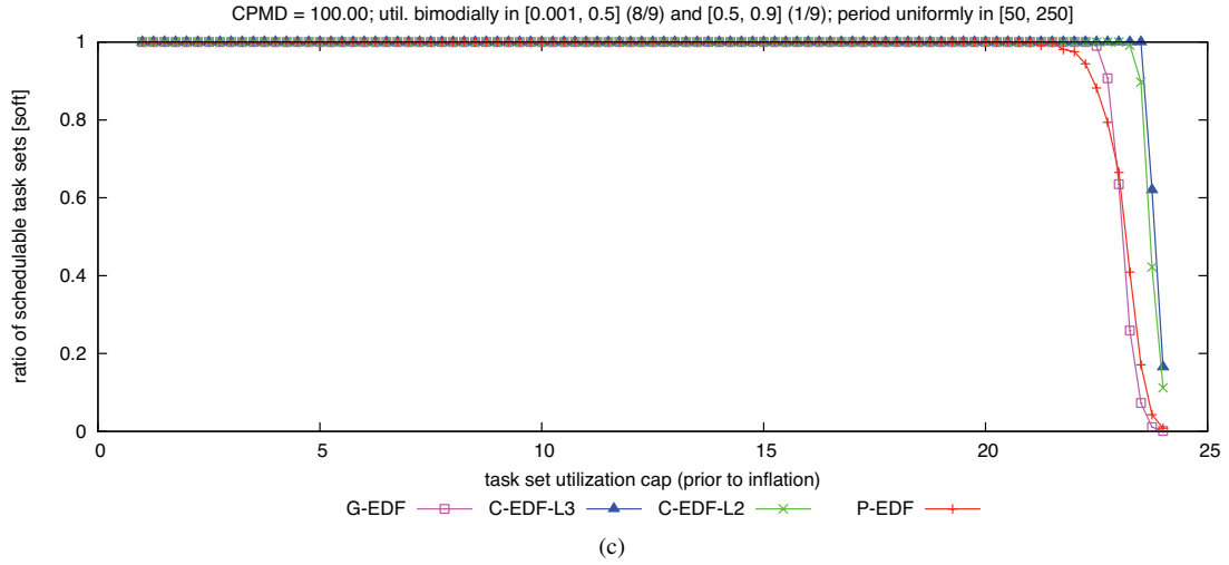
Figure 284: CPMD = 100.00. Soft schedulability of task sets with bimodal light per-task utilizations and (a) short, (b) moderate, and (c) long periods.
