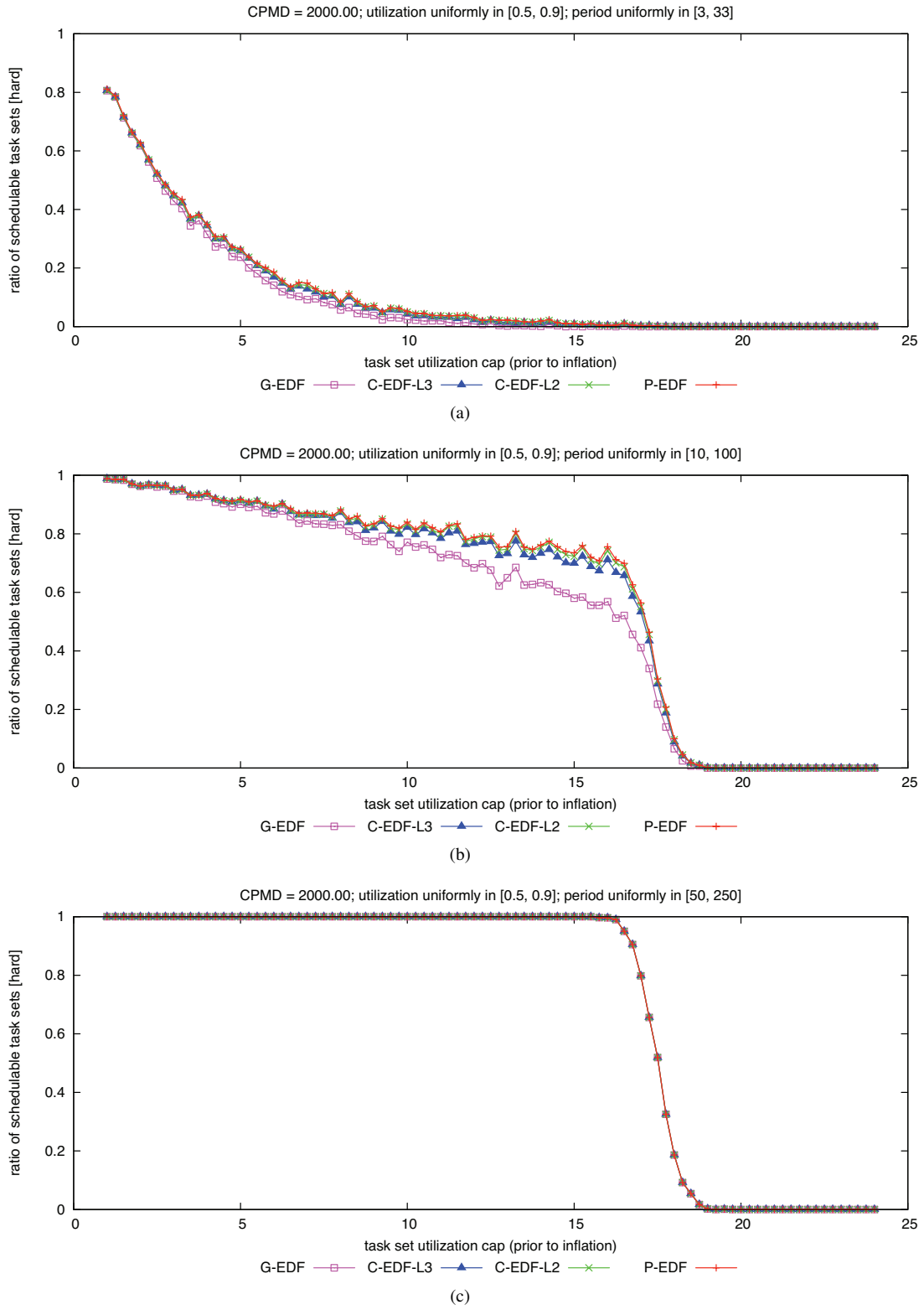
Figure 273: CPMD = 2000.00. Hard W(D) schedulability of task sets with uniform heavy per-task utilizations and (a) short, (b) moderate, and (c) long periods.
