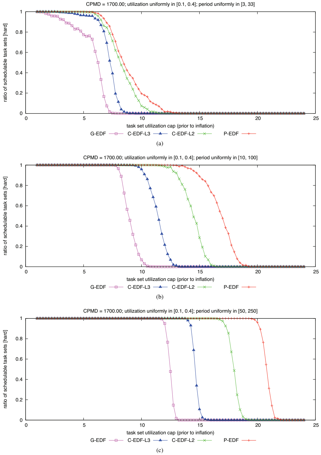
Figure 233: CPMD = 1700.00. Hard W(D) schedulability of task sets with uniform medium per-task utilizations and (a) short, (b) moderate, and (c) long periods.
