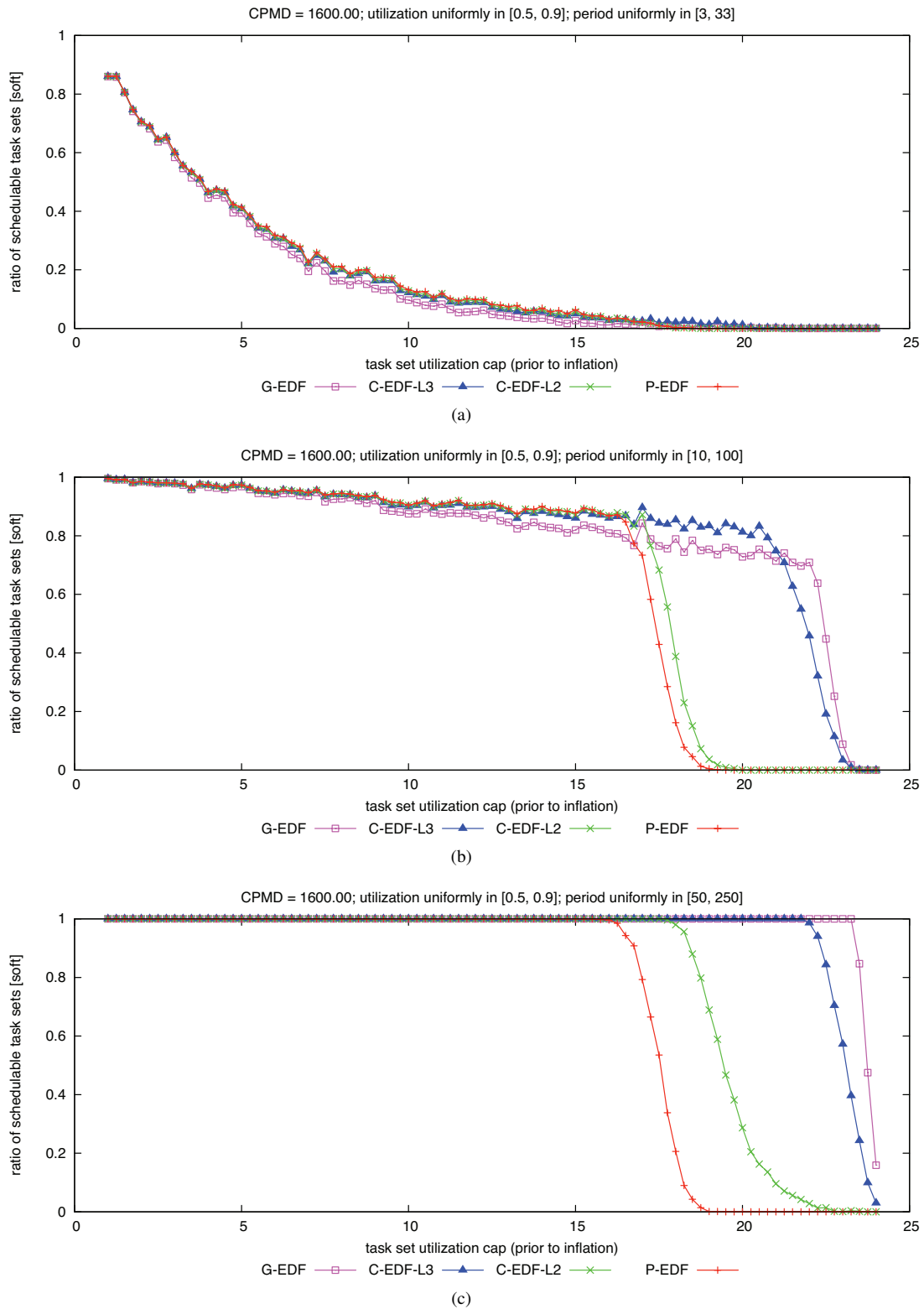
Figure 377: CPMD = 1600.00. Soft schedulability of task sets with uniform heavy per-task utilizations and (a) short, (b) moderate, and (c) long periods.
