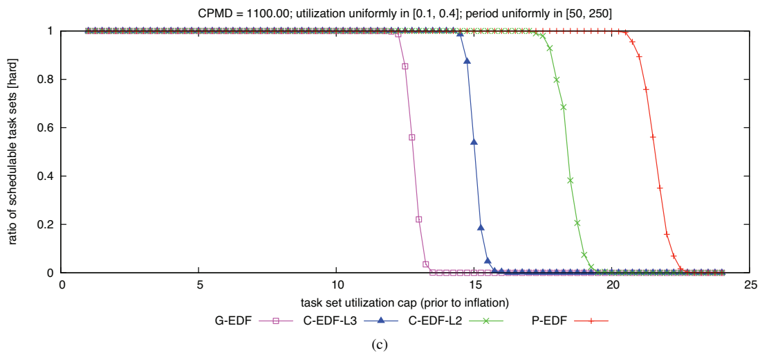
Figure 161: CPMD = 1100.00. Hard W(D) schedulability of task sets with uniform medium per-task utilizations and (a) short, (b) moderate, and (c) long periods.
