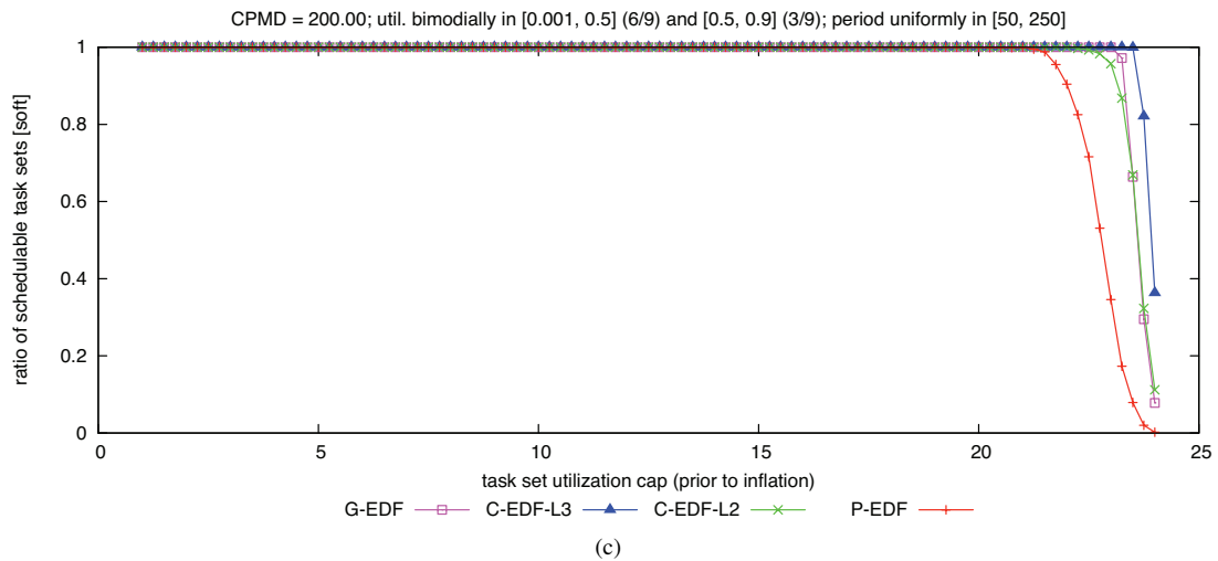
Figure 292: CPMD = 200.00. Soft schedulability of task sets with bimodal medium per-task utilizations and (a) short, (b) moderate, and (c) long periods.
