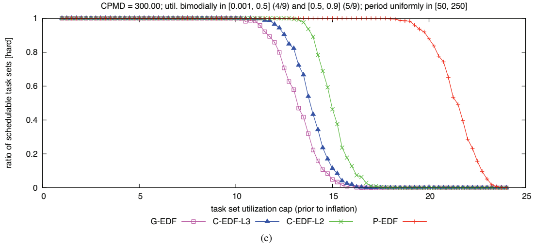
Figure 71: CPMD = 300.00. Hard W(D) schedulability of task sets with bimodal heavy per-task utilizations and (a) short, (b) moderate, and (c) long periods.
