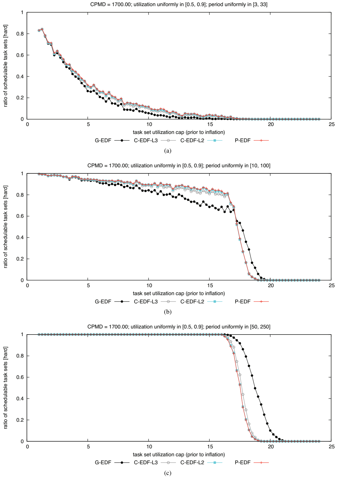
Figure 238: CPMD = 1700.00. Hard BF schedulability of task sets with uniform heavy per-task utilizations and (a) short, (b) moderate, and (c) long periods.
