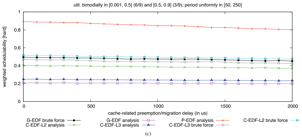
Figure 16: Hard weighted schedulability of task sets with bimodal medium per-task utilizations and (a) short, (b) moderate, and (c) long periods.
