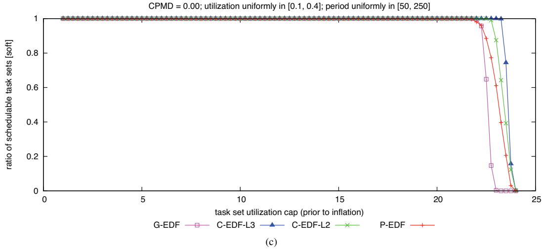
Figure 279: CPMD = 0.00. Soft schedulability of task sets with uniform medium per-task utilizations and (a) short, (b) moderate, and (c) long periods.
