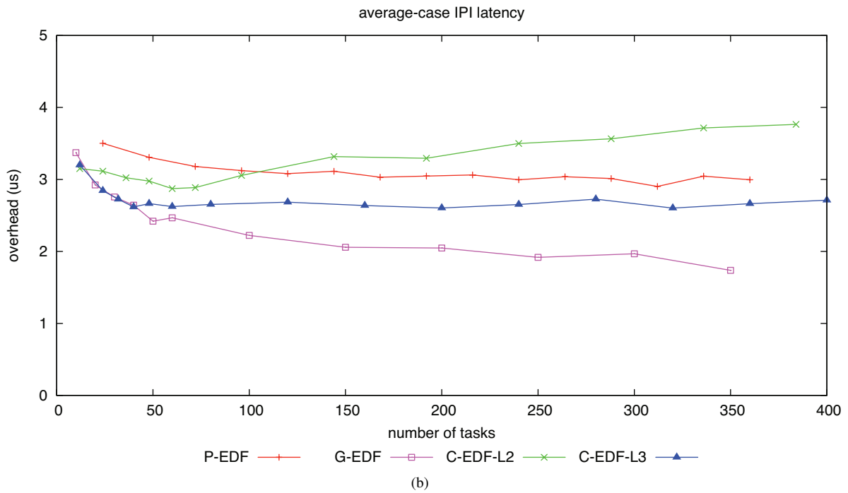
Figure 12: Measured IPI latency. (a) Measured worst case. (b) Measured average case.
