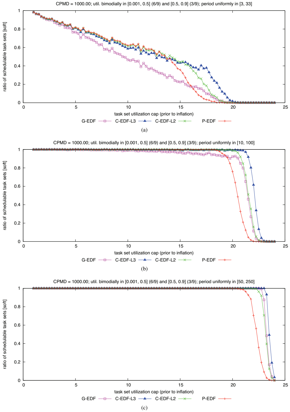
Figure 340: CPMD = 1000.00. Soft schedulability of task sets with bimodal medium per-task utilizations and (a) short, (b) moderate, and (c) long periods.
