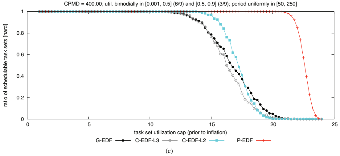
Figure 80: CPMD = 400.00. Hard BF schedulability of task sets with bimodal medium per-task utilizations and (a) short, (b) moderate, and (c) long periods.
