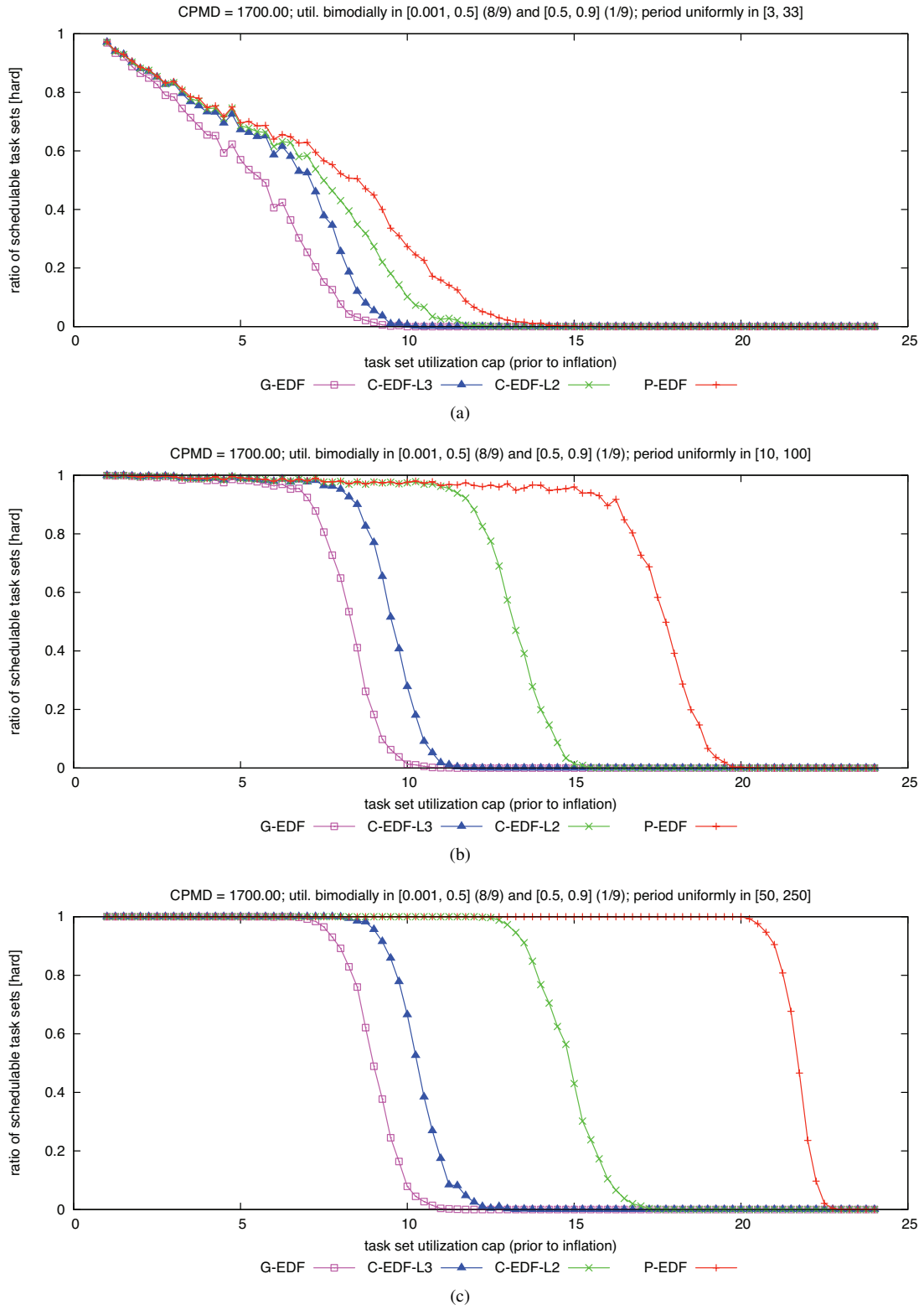
Figure 231: CPMD = 1700.00. Hard W(D) schedulability of task sets with bimodal light per-task utilizations and (a) short, (b) moderate, and (c) long periods.
