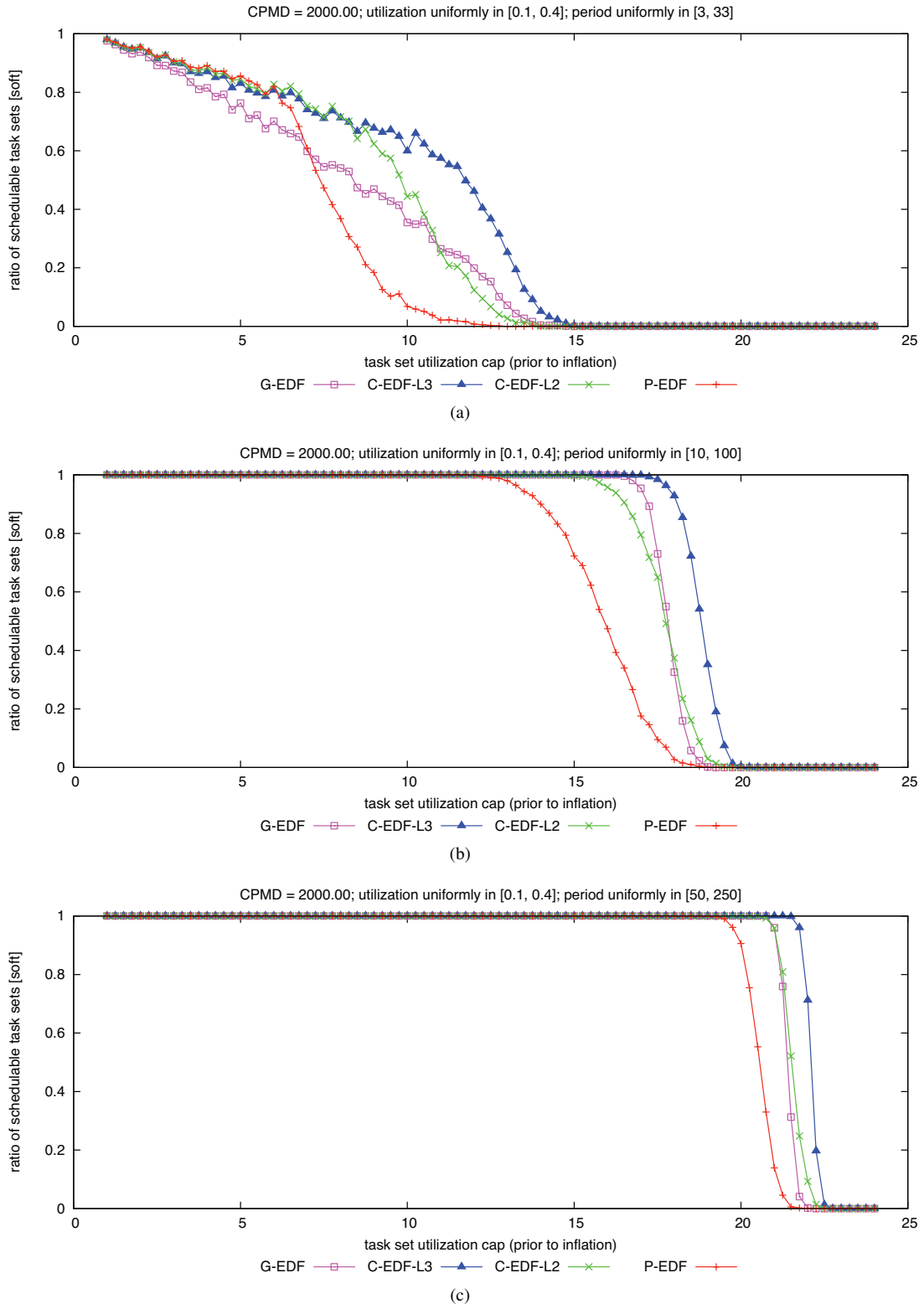
Figure 399: CPMD = 2000.00. Soft schedulability of task sets with uniform medium per-task utilizations and (a) short, (b) moderate, and (c) long periods.
