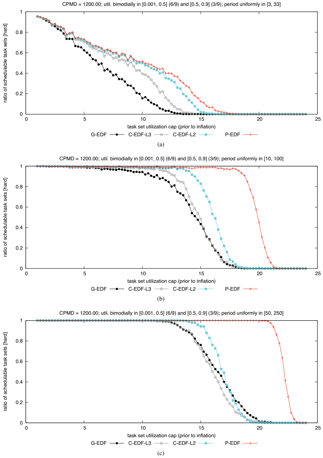
Figure 176: CPMD = 1200.00. Hard BF schedulability of task sets with bimodal medium per-task utilizations and (a) short, (b) moderate, and (c) long periods.
