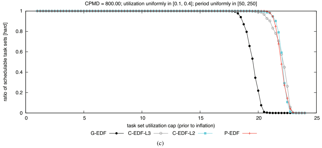
Figure 126: CPMD = 800.00. Hard BF schedulability of task sets with uniform medium per-task utilizations and (a) short, (b) moderate, and (c) long periods.
