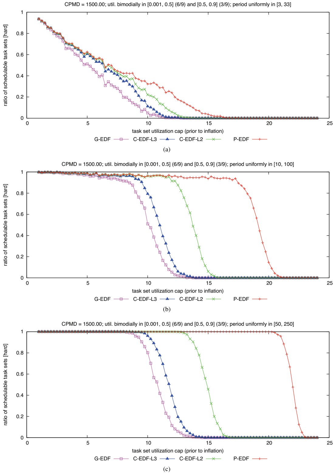
Figure 211: CPMD = 1500.00. Hard W(D) schedulability of task sets with bimodal medium per-task utilizations and (a) short, (b) moderate, and (c) long periods.
