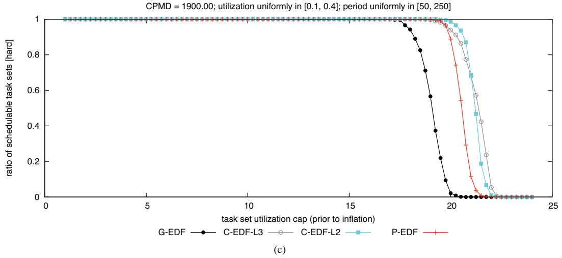
Figure 258: CPMD = 1900.00. Hard BF schedulability of task sets with uniform medium per-task utilizations and (a) short, (b) moderate, and (c) long periods.
