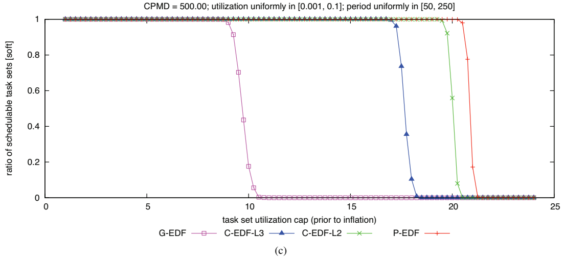
Figure 307: CPMD = 500.00. Soft schedulability of task sets with uniform light per-task utilizations and (a) short, (b) moderate, and (c) long periods.
