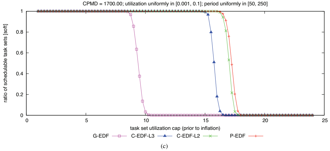
Figure 379: CPMD = 1700.00. Soft schedulability of task sets with uniform light per-task utilizations and (a) short, (b) moderate, and (c) long periods.
