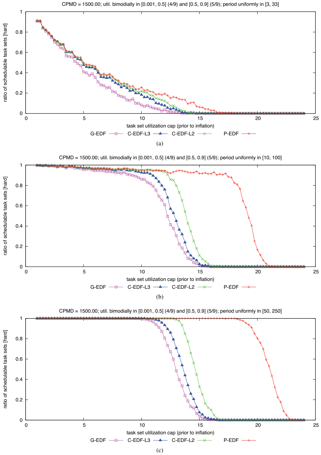
Figure 215: CPMD = 1500.00. Hard W(D) schedulability of task sets with bimodal heavy per-task utilizations and (a) short, (b) moderate, and (c) long periods.
