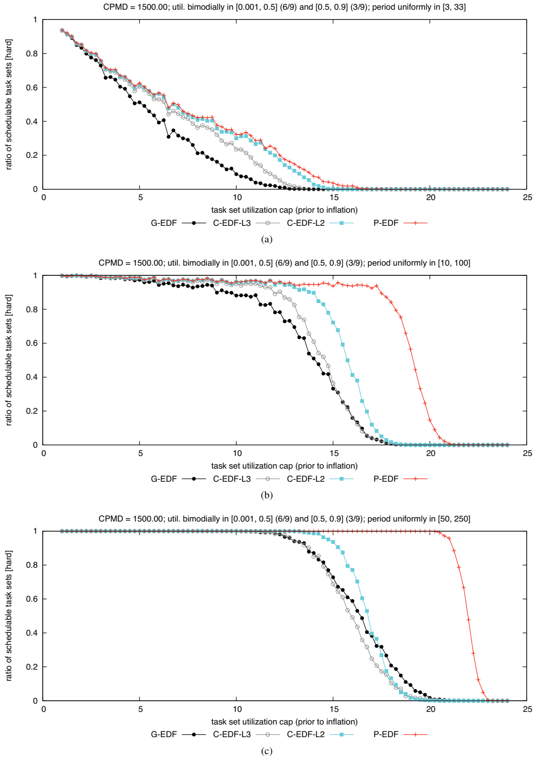
Figure 212: CPMD = 1500.00. Hard BF schedulability of task sets with bimodal medium per-task utilizations and (a) short, (b) moderate, and (c) long periods.
