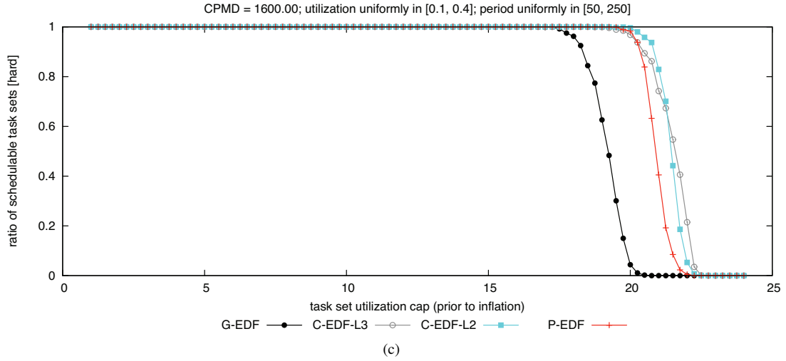
Figure 222: CPMD = 1600.00. Hard BF schedulability of task sets with uniform medium per-task utilizations and (a) short, (b) moderate, and (c) long periods.
