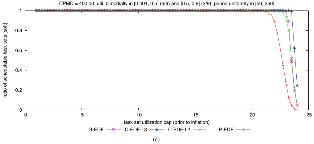
Figure 304: CPMD = 400.00. Soft schedulability of task sets with bimodal medium per-task utilizations and (a) short, (b) moderate, and (c) long periods.
