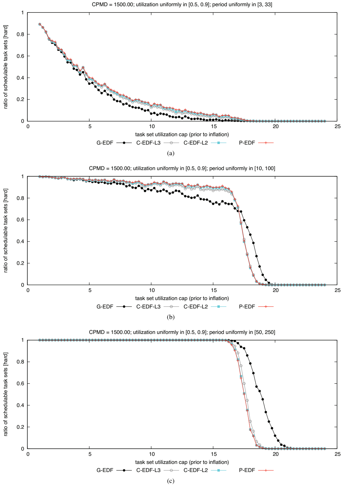
Figure 214: CPMD = 1500.00. Hard BF schedulability of task sets with uniform heavy per-task utilizations and (a) short, (b) moderate, and (c) long periods.
