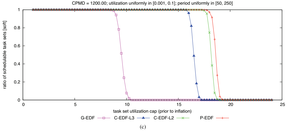
Figure 349: CPMD = 1200.00. Soft schedulability of task sets with uniform light per-task utilizations and (a) short, (b) moderate, and (c) long periods.
