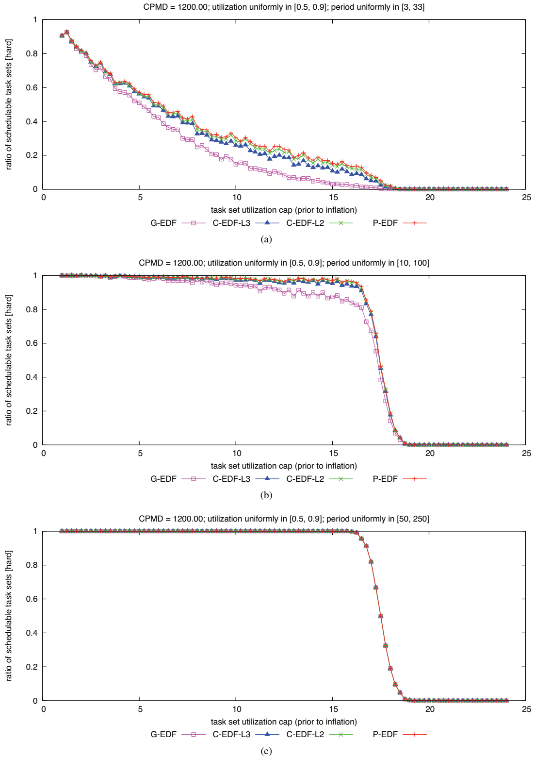
Figure 177: CPMD = 1200.00. Hard W(D) schedulability of task sets with uniform heavy per-task utilizations and (a) short, (b) moderate, and (c) long periods.
