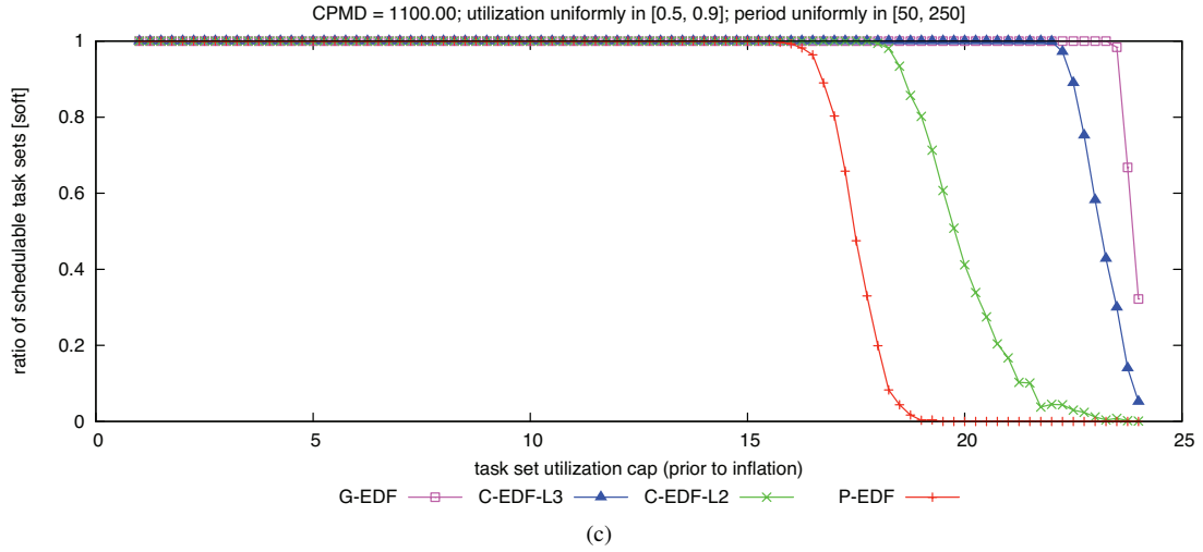
Figure 347: CPMD = 1100.00. Soft schedulability of task sets with uniform heavy per-task utilizations and (a) short, (b) moderate, and (c) long periods.
