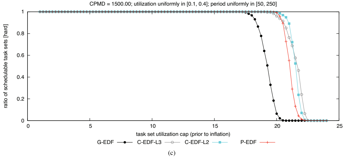
Figure 210: CPMD = 1500.00. Hard BF schedulability of task sets with uniform medium per-task utilizations and (a) short, (b) moderate, and (c) long periods.
