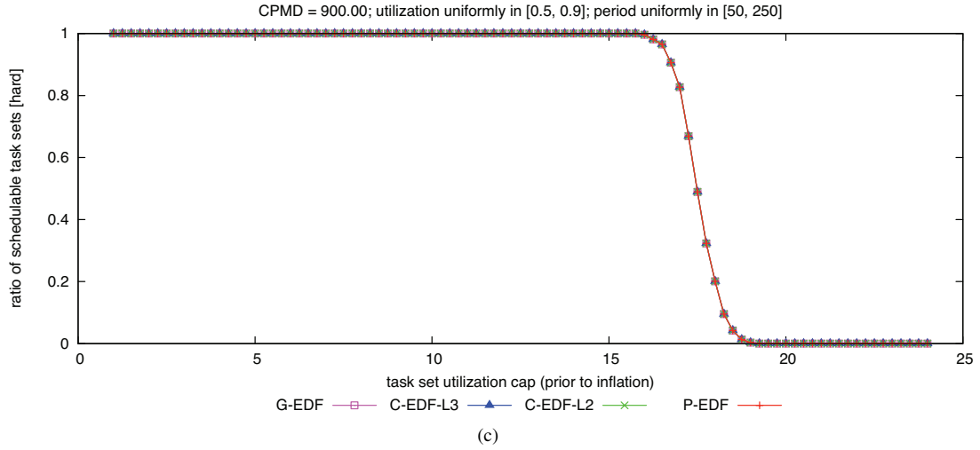
Figure 141: CPMD = 900.00. Hard W(D) schedulability of task sets with uniform heavy per-task utilizations and (a) short, (b) moderate, and (c) long periods.
