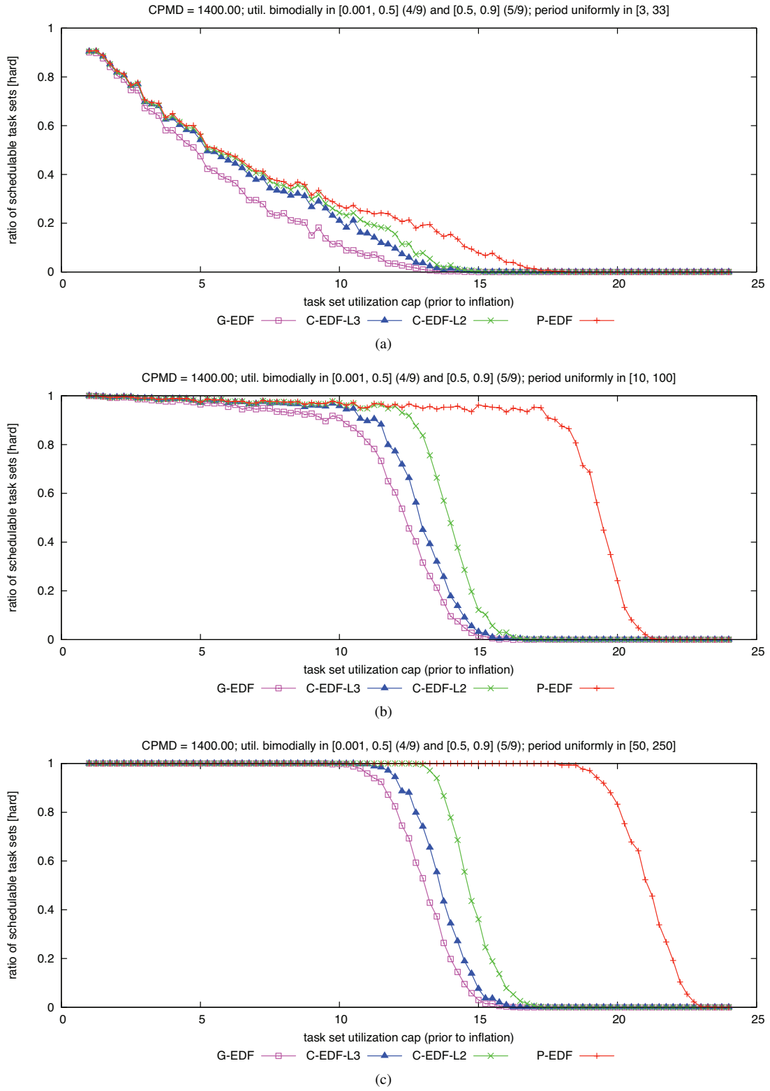
Figure 203: CPMD = 1400.00. Hard W(D) schedulability of task sets with bimodal heavy per-task utilizations and (a) short, (b) moderate, and (c) long periods.
