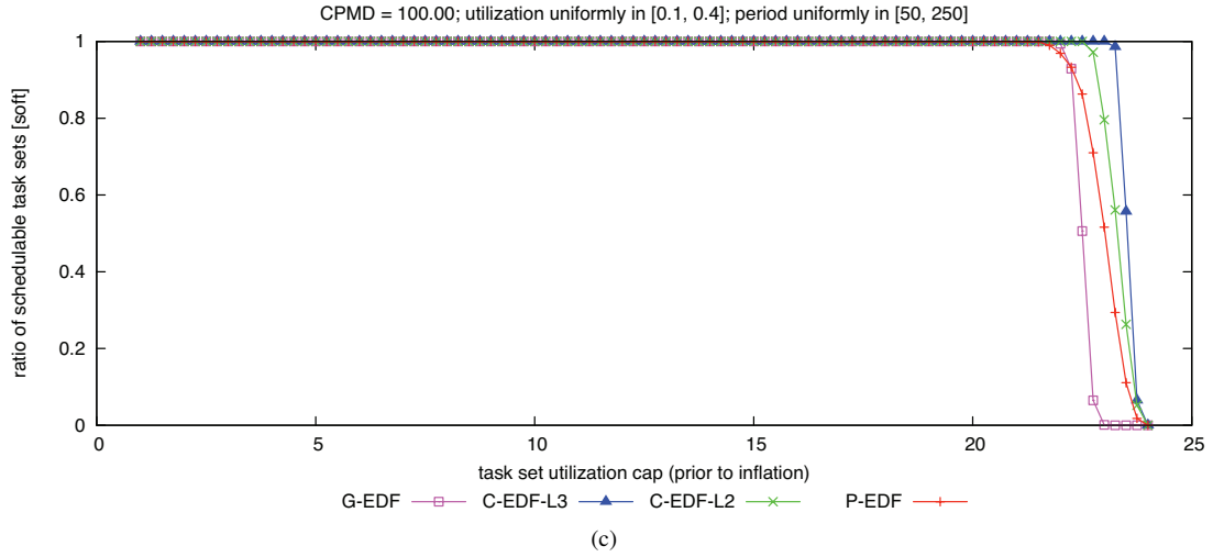
Figure 285: CPMD = 100.00. Soft schedulability of task sets with uniform medium per-task utilizations and (a) short, (b) moderate, and (c) long periods.
