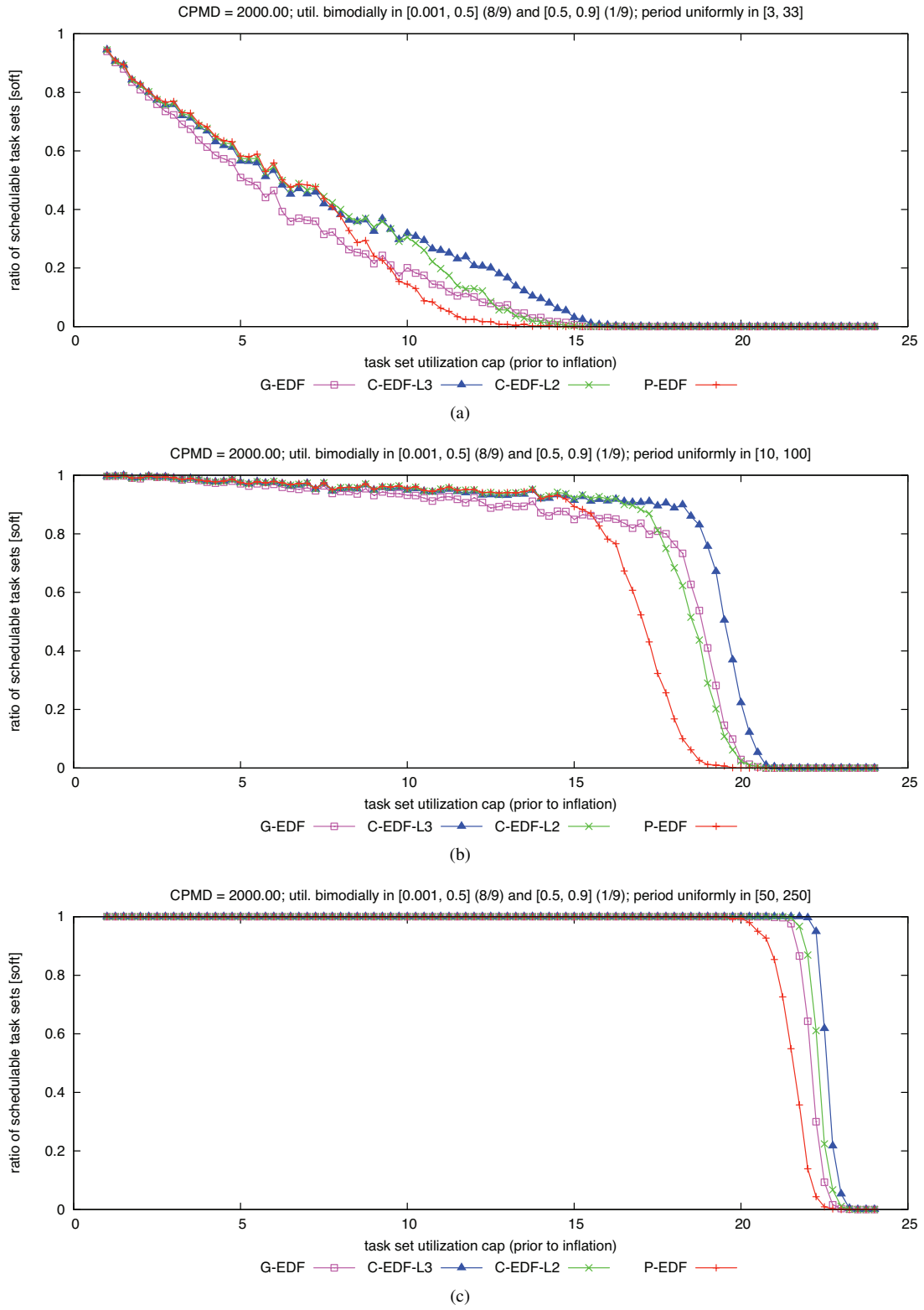
Figure 398: CPMD = 2000.00. Soft schedulability of task sets with bimodal light per-task utilizations and (a) short, (b) moderate, and (c) long periods.
