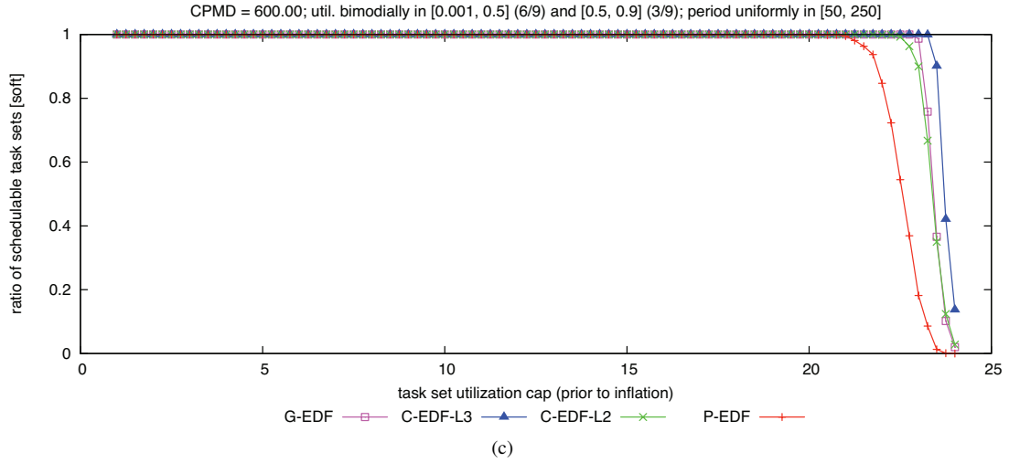
Figure 316: CPMD = 600.00. Soft schedulability of task sets with bimodal medium per-task utilizations and (a) short, (b) moderate, and (c) long periods.
