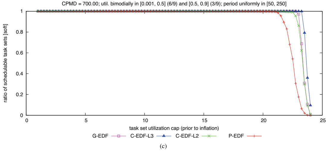
Figure 322: CPMD = 700.00. Soft schedulability of task sets with bimodal medium per-task utilizations and (a) short, (b) moderate, and (c) long periods.
