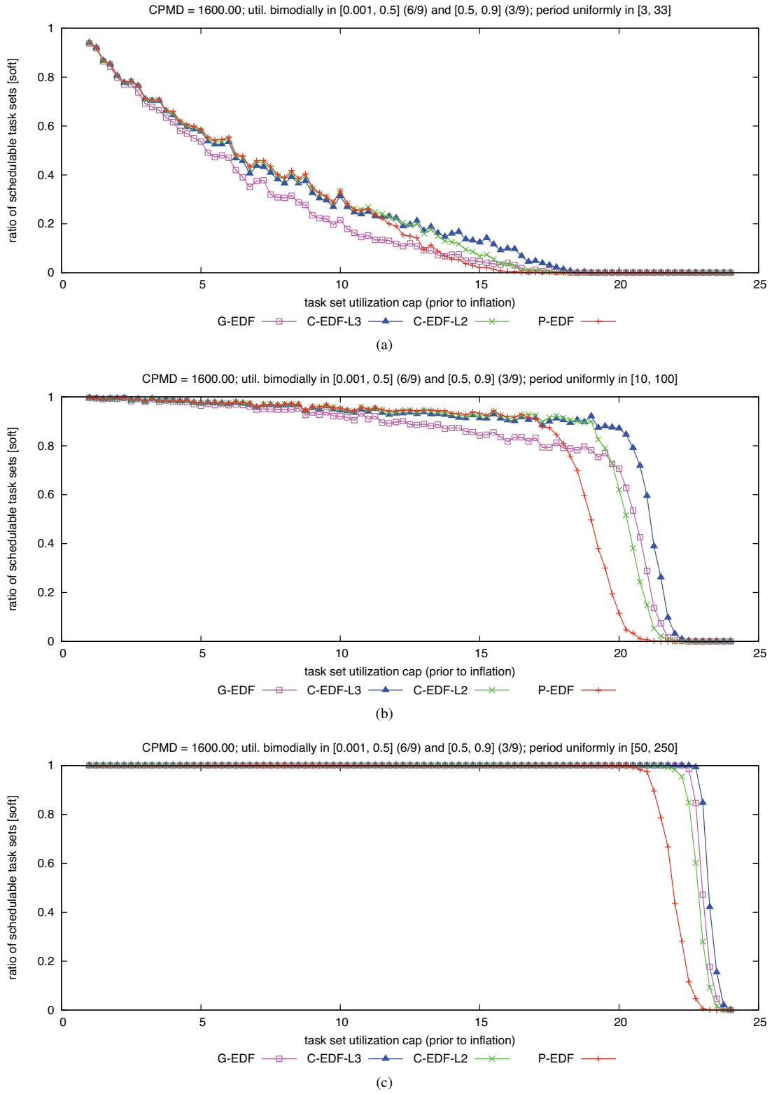
Figure 376: CPMD = 1600.00. Soft schedulability of task sets with bimodal medium per-task utilizations and (a) short, (b) moderate, and (c) long periods.
