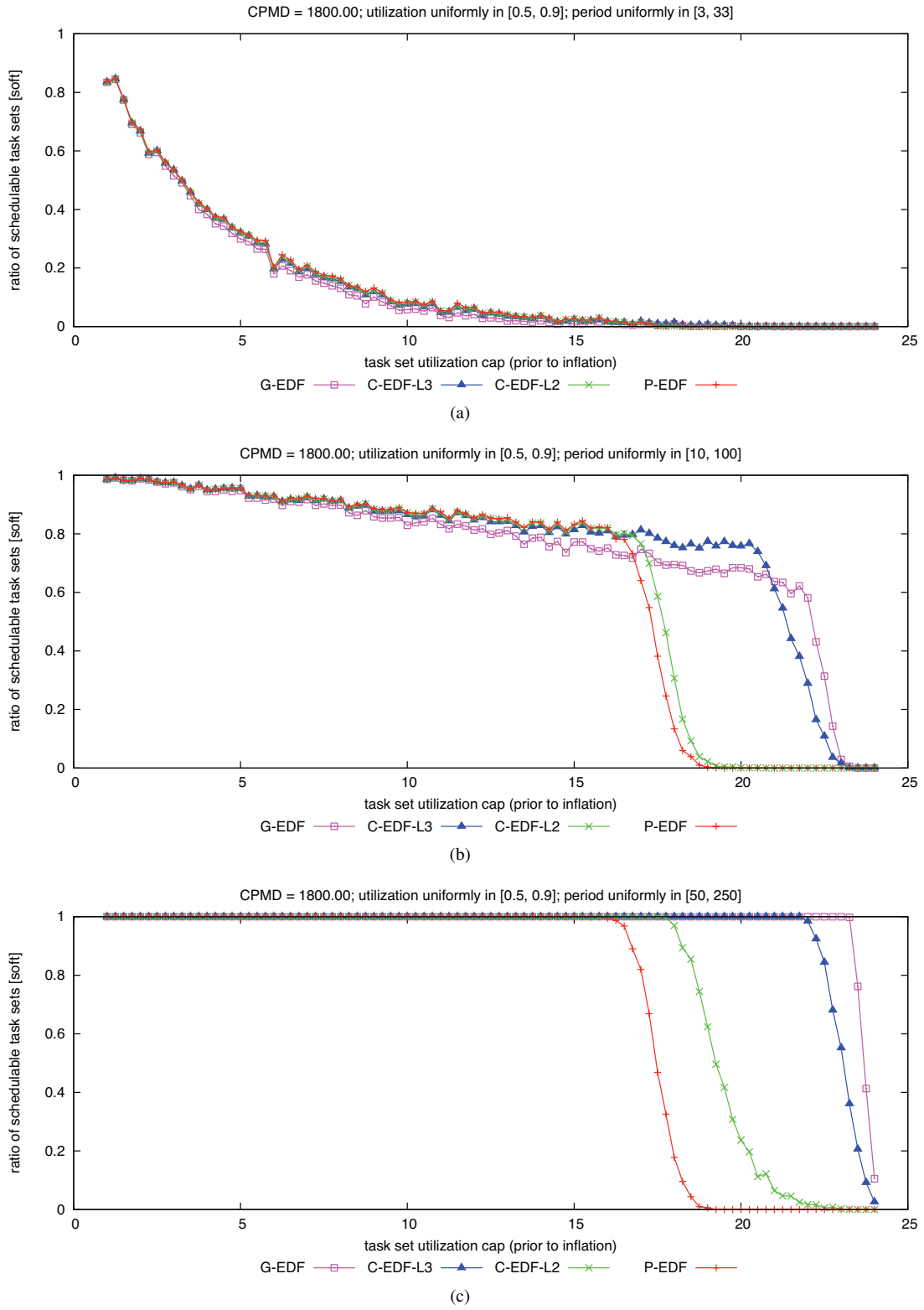
Figure 389: CPMD = 1800.00. Soft schedulability of task sets with uniform heavy per-task utilizations and (a) short, (b) moderate, and (c) long periods.
