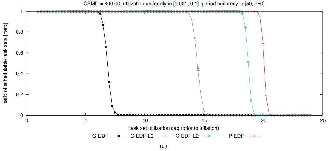
Figure 74: CPMD = 400.00. Hard BF schedulability of task sets with uniform light per-task utilizations and (a) short, (b) moderate, and (c) long periods.
