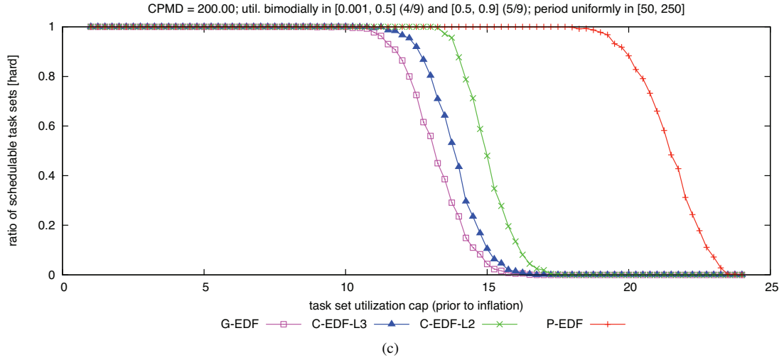
Figure 59: CPMD = 200.00. Hard W(D) schedulability of task sets with bimodal heavy per-task utilizations and (a) short, (b) moderate, and (c) long periods.
