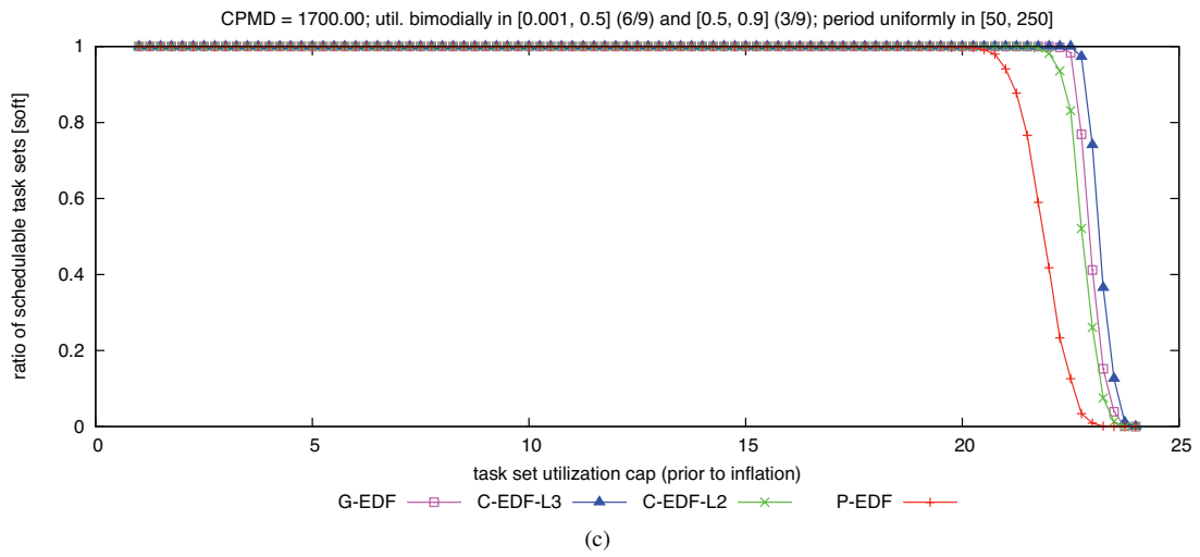
Figure 382: CPMD = 1700.00. Soft schedulability of task sets with bimodal medium per-task utilizations and (a) short, (b) moderate, and (c) long periods.
