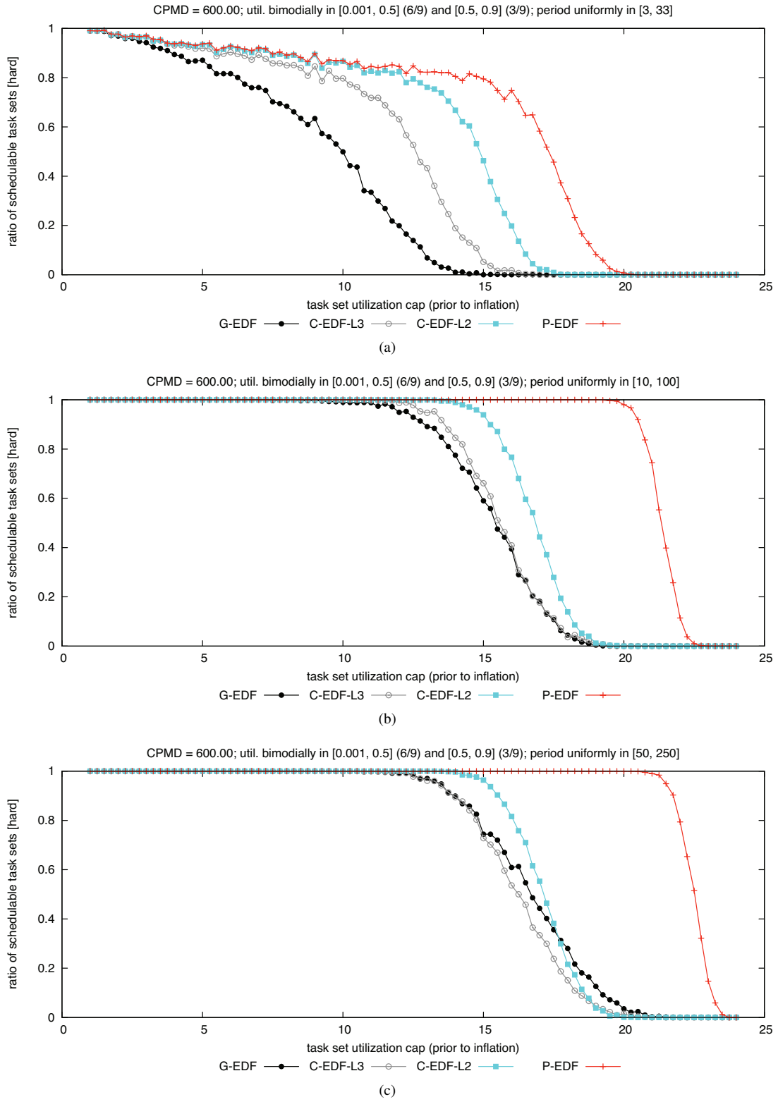
Figure 104: CPMD = 600.00. Hard BF schedulability of task sets with bimodal medium per-task utilizations and (a) short, (b) moderate, and (c) long periods.
