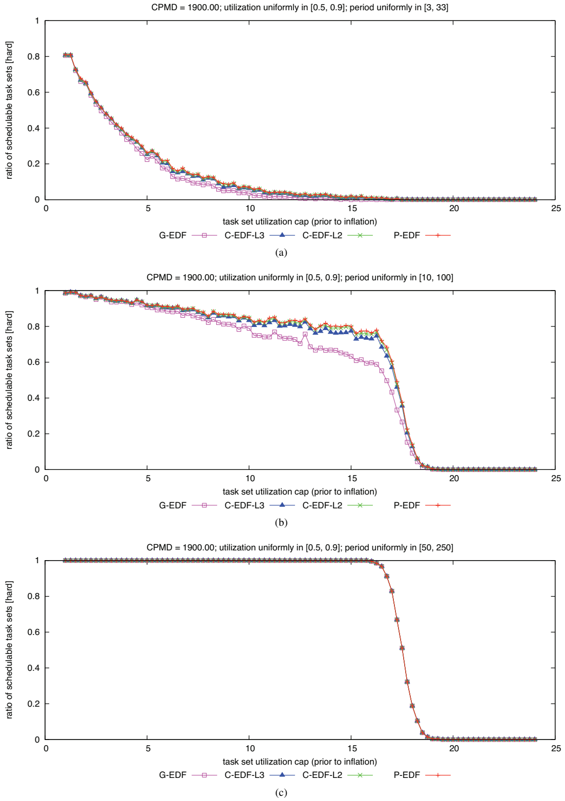
Figure 261: CPMD = 1900.00. Hard W(D) schedulability of task sets with uniform heavy per-task utilizations and (a) short, (b) moderate, and (c) long periods.
