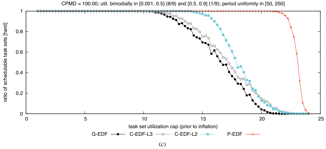
Figure 40: CPMD = 100.00. Hard BF schedulability of task sets with bimodal light per-task utilizations and (a) short, (b) moderate, and (c) long periods.
