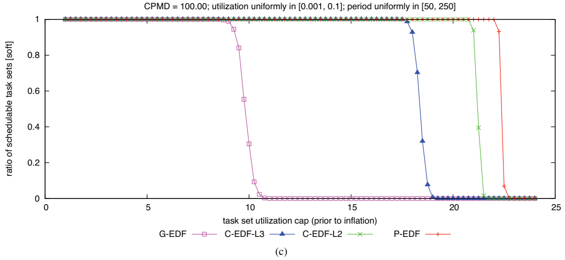
Figure 283: CPMD = 100.00. Soft schedulability of task sets with uniform light per-task utilizations and (a) short, (b) moderate, and (c) long periods.
