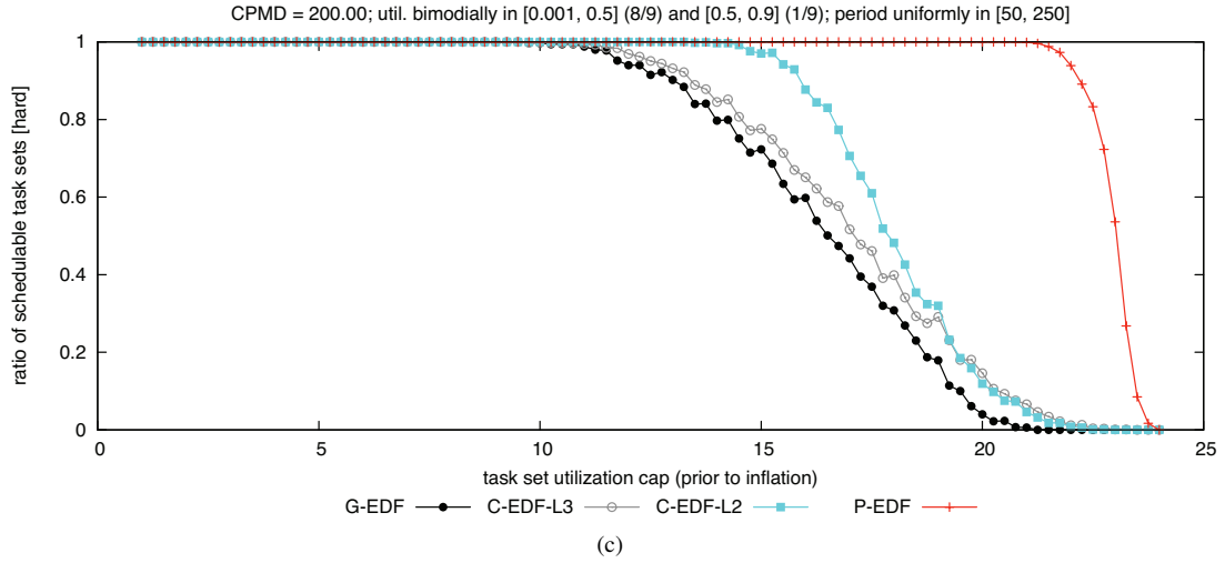
Figure 52: CPMD = 200.00. Hard BF schedulability of task sets with bimodal light per-task utilizations and (a) short, (b) moderate, and (c) long periods.
