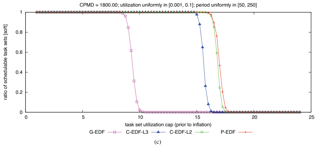
Figure 385: CPMD = 1800.00. Soft schedulability of task sets with uniform light per-task utilizations and (a) short, (b) moderate, and (c) long periods.
