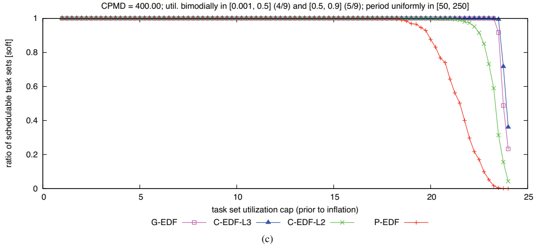
Figure 306: CPMD = 400.00. Soft schedulability of task sets with bimodal heavy per-task utilizations and (a) short, (b) moderate, and (c) long periods.
