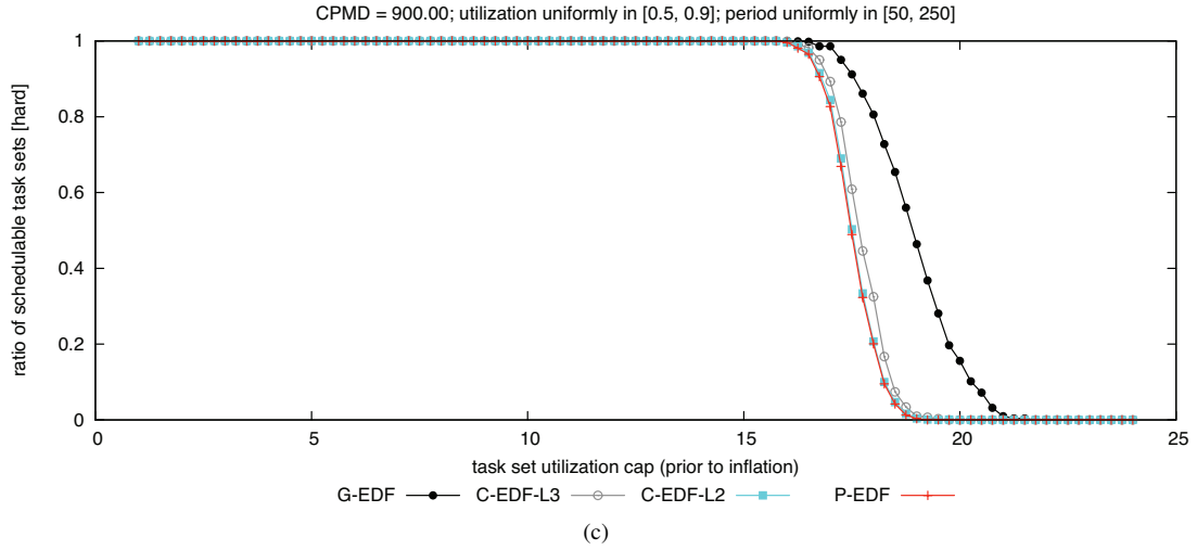
Figure 142: CPMD = 900.00. Hard BF schedulability of task sets with uniform heavy per-task utilizations and (a) short, (b) moderate, and (c) long periods.
