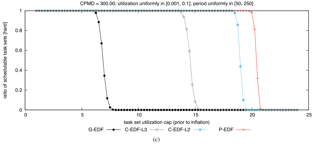
Figure 62: CPMD = 300.00. Hard BF schedulability of task sets with uniform light per-task utilizations and (a) short, (b) moderate, and (c) long periods.
