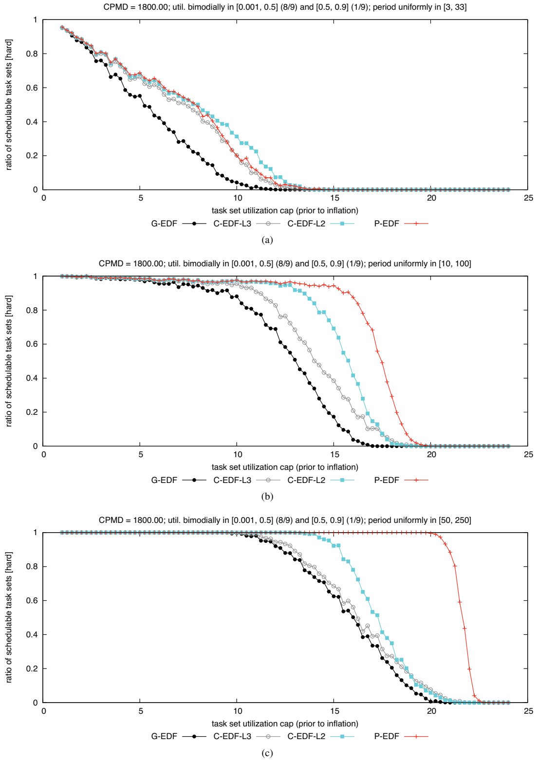
Figure 244: CPMD = 1800.00. Hard BF schedulability of task sets with bimodal light per-task utilizations and (a) short, (b) moderate, and (c) long periods.
