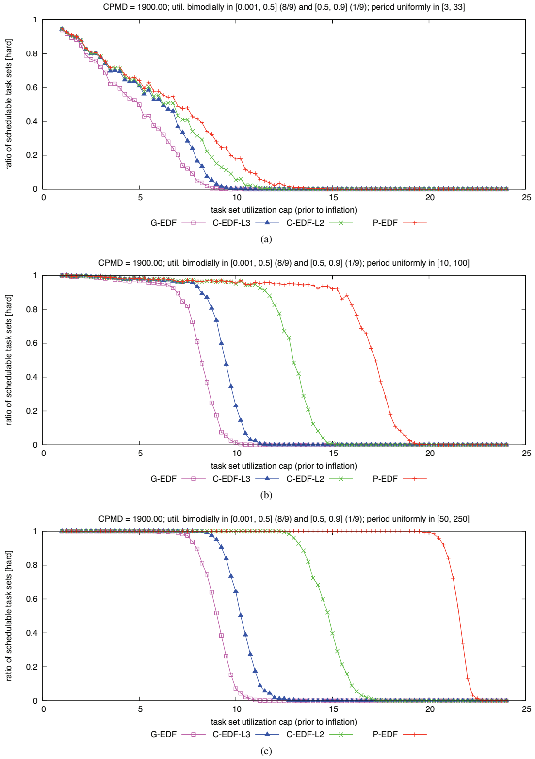
Figure 255: CPMD = 1900.00. Hard W(D) schedulability of task sets with bimodal light per-task utilizations and (a) short, (b) moderate, and (c) long periods.
