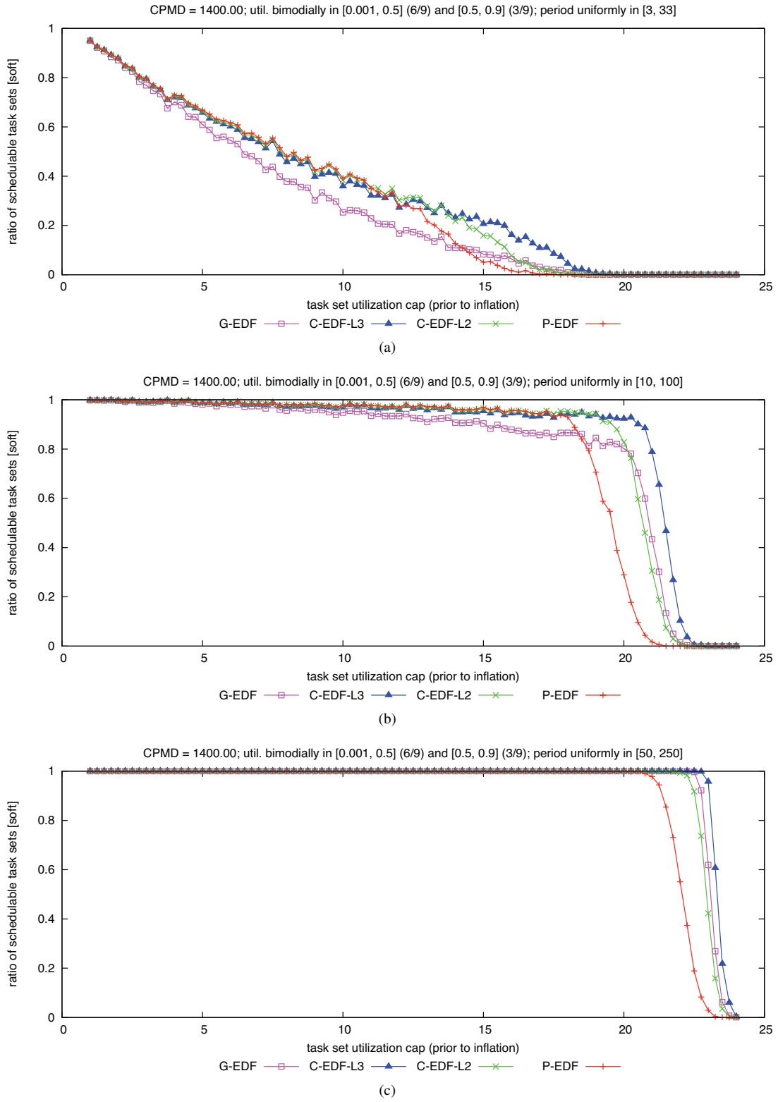
Figure 364: CPMD = 1400.00. Soft schedulability of task sets with bimodal medium per-task utilizations and (a) short, (b) moderate, and (c) long periods.
