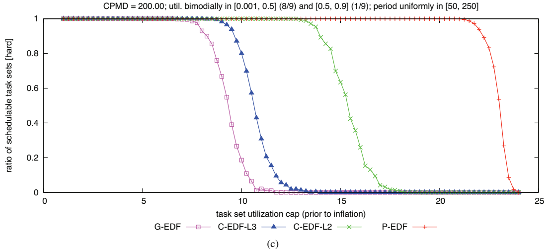
Figure 51: CPMD = 200.00. Hard W(D) schedulability of task sets with bimodal light per-task utilizations and (a) short, (b) moderate, and (c) long periods.
