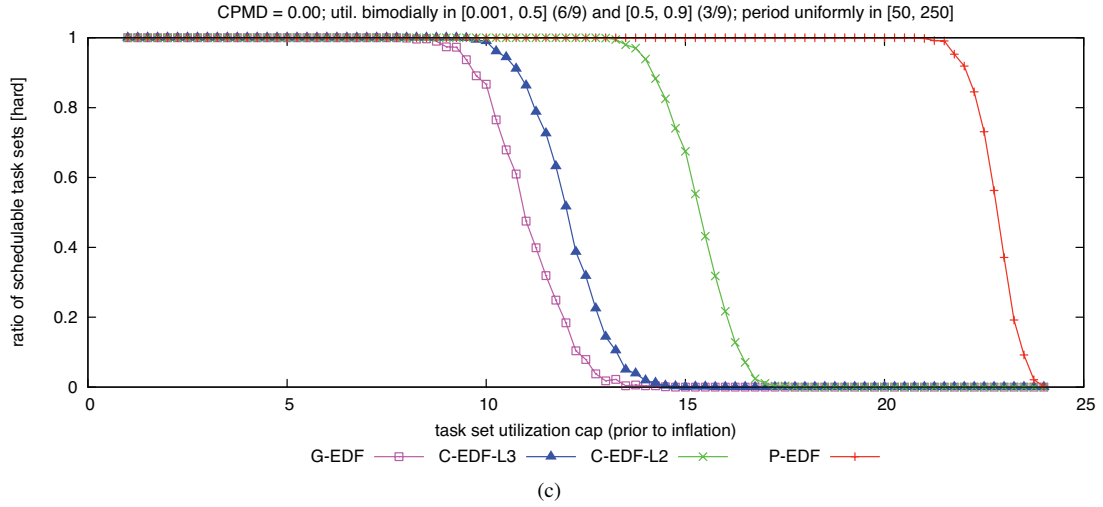
Figure 31: CPMD = 0.00. Hard W(D) schedulability of task sets with bimodal medium per-task utilizations and (a) short, (b) moderate, and (c) long periods.
