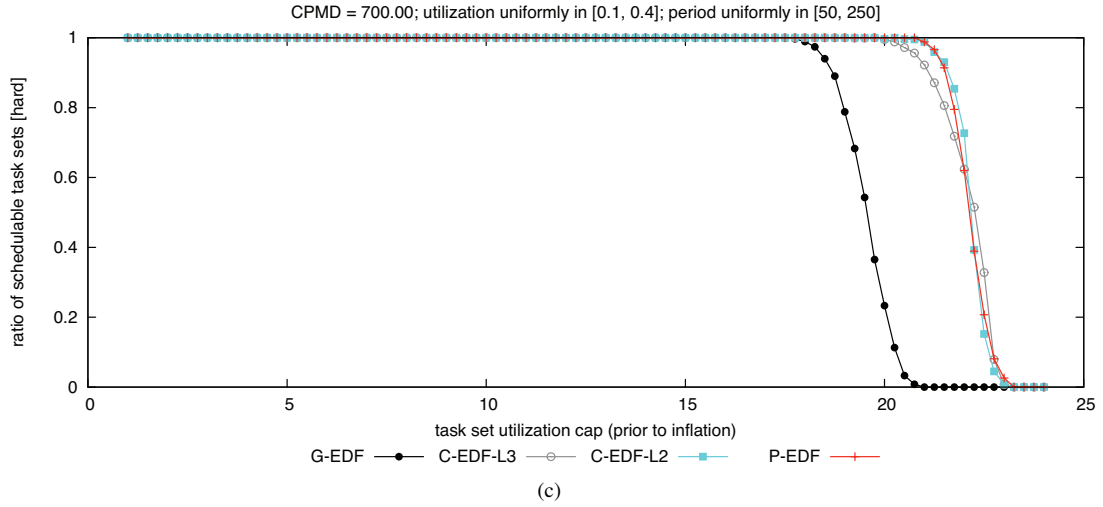
Figure 114: CPMD = 700.00. Hard BF schedulability of task sets with uniform medium per-task utilizations and (a) short, (b) moderate, and (c) long periods.
