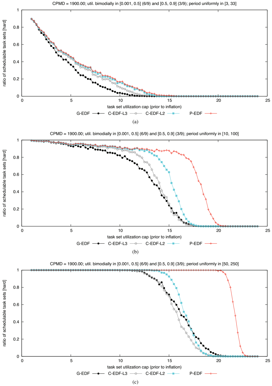
Figure 260: CPMD = 1900.00. Hard BF schedulability of task sets with bimodal medium per-task utilizations and (a) short, (b) moderate, and (c) long periods.
