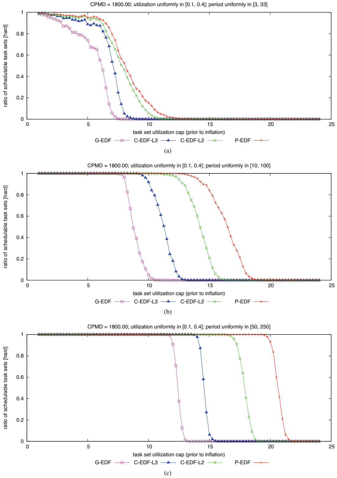
Figure 245: CPMD = 1800.00. Hard W(D) schedulability of task sets with uniform medium per-task utilizations and (a) short, (b) moderate, and (c) long periods.
