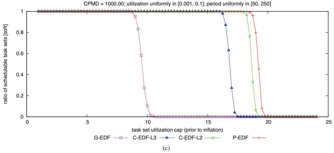
Figure 337: CPMD = 1000.00. Soft schedulability of task sets with uniform light per-task utilizations and (a) short, (b) moderate, and (c) long periods.
