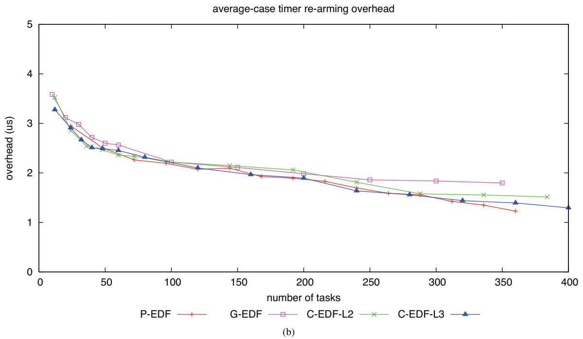
Figure 8: Measured timer re-arming overhead. (a) Measured worst case. (b) Measured average case.
