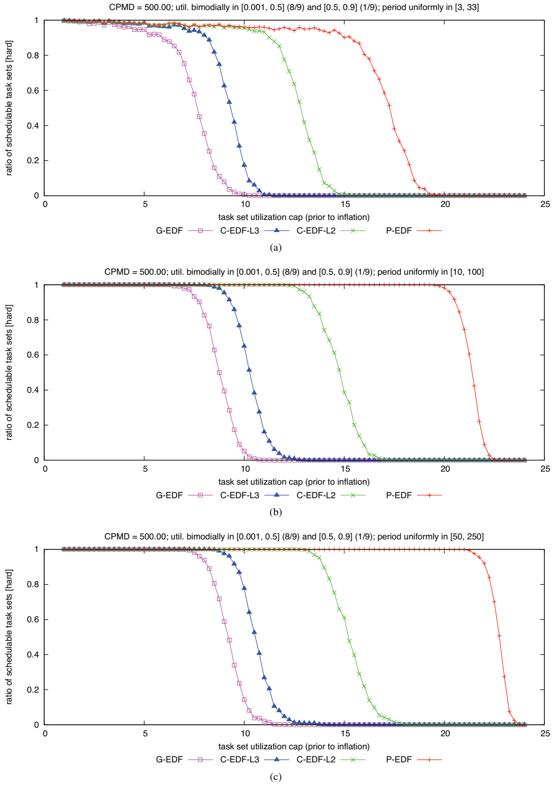
Figure 87: CPMD = 500.00. Hard W(D) schedulability of task sets with bimodal light per-task utilizations and (a) short, (b) moderate, and (c) long periods.
