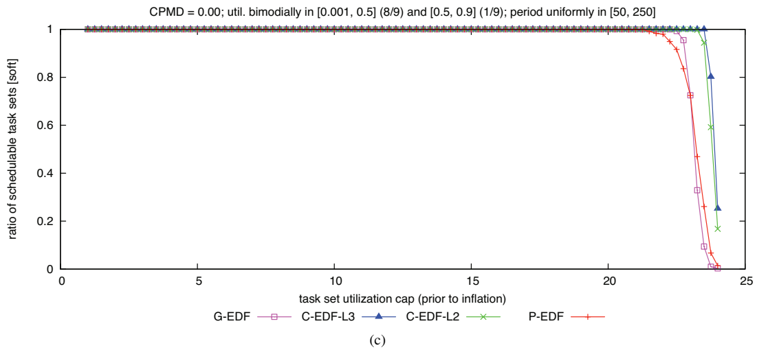
Figure 278: CPMD = 0.00. Soft schedulability of task sets with bimodal light per-task utilizations and (a) short, (b) moderate, and (c) long periods.
