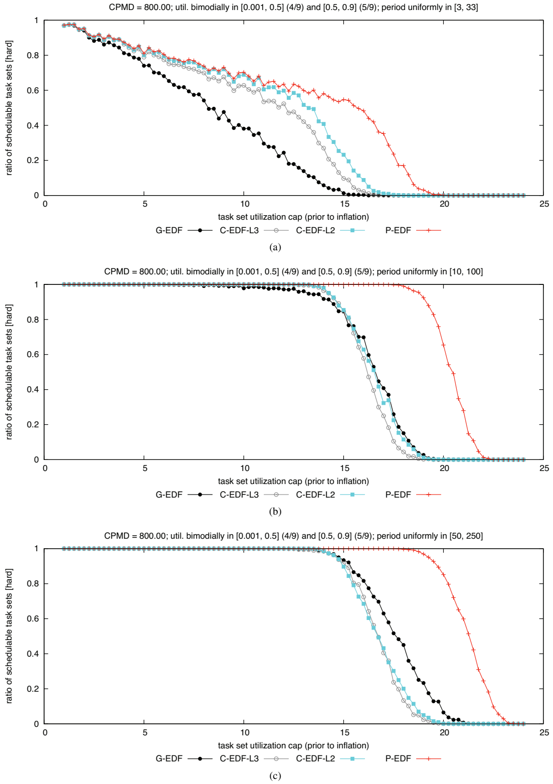
Figure 132: CPMD = 800.00. Hard BF schedulability of task sets with bimodal heavy per-task utilizations and (a) short, (b) moderate, and (c) long periods.
