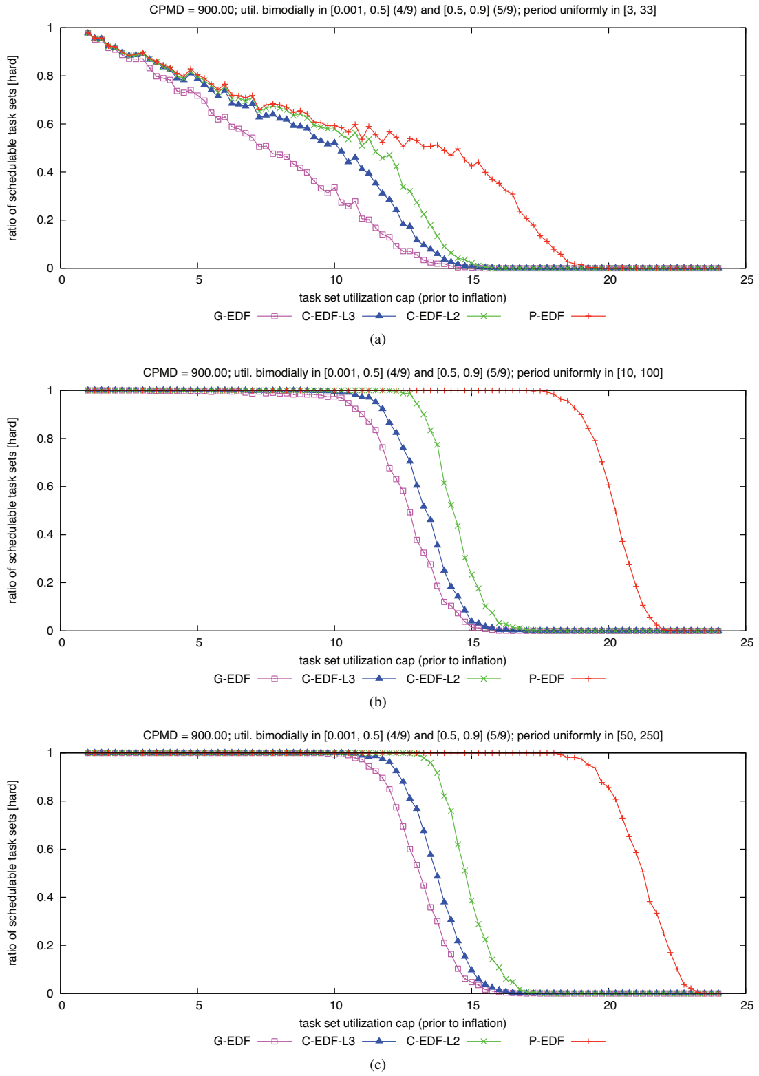
Figure 143: CPMD = 900.00. Hard W(D) schedulability of task sets with bimodal heavy per-task utilizations and (a) short, (b) moderate, and (c) long periods.
