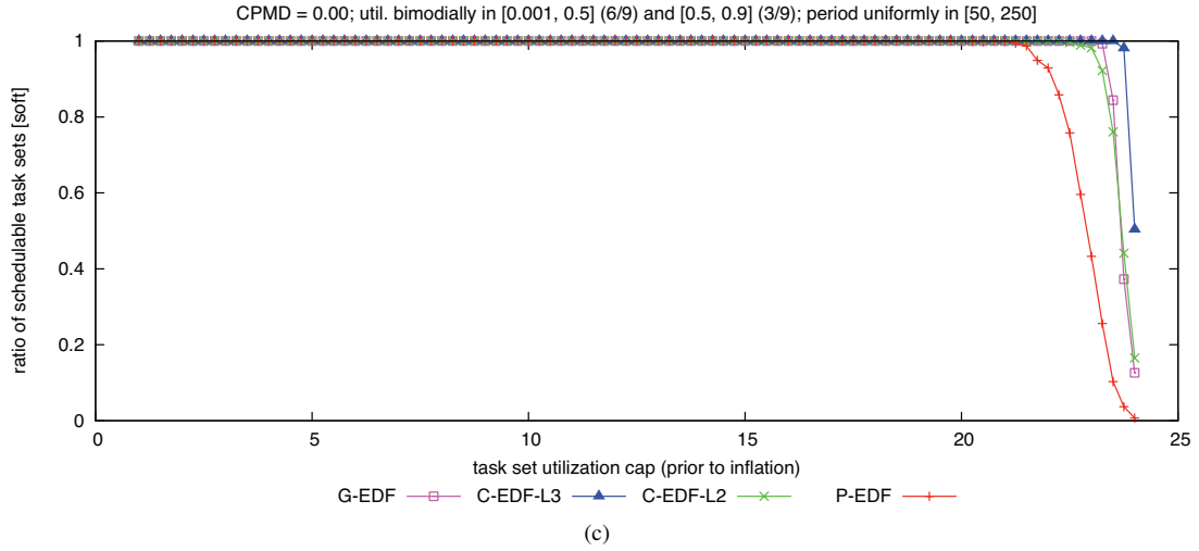
Figure 280: CPMD = 0.00. Soft schedulability of task sets with bimodal medium per-task utilizations and (a) short, (b) moderate, and (c) long periods.
