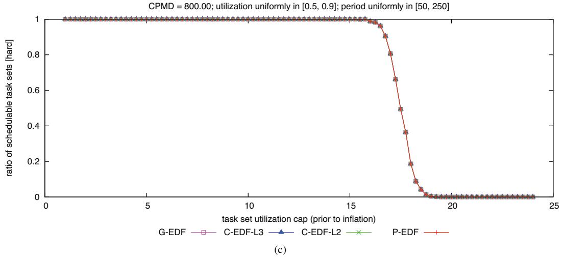
Figure 129: CPMD = 800.00. Hard W(D) schedulability of task sets with uniform heavy per-task utilizations and (a) short, (b) moderate, and (c) long periods.
