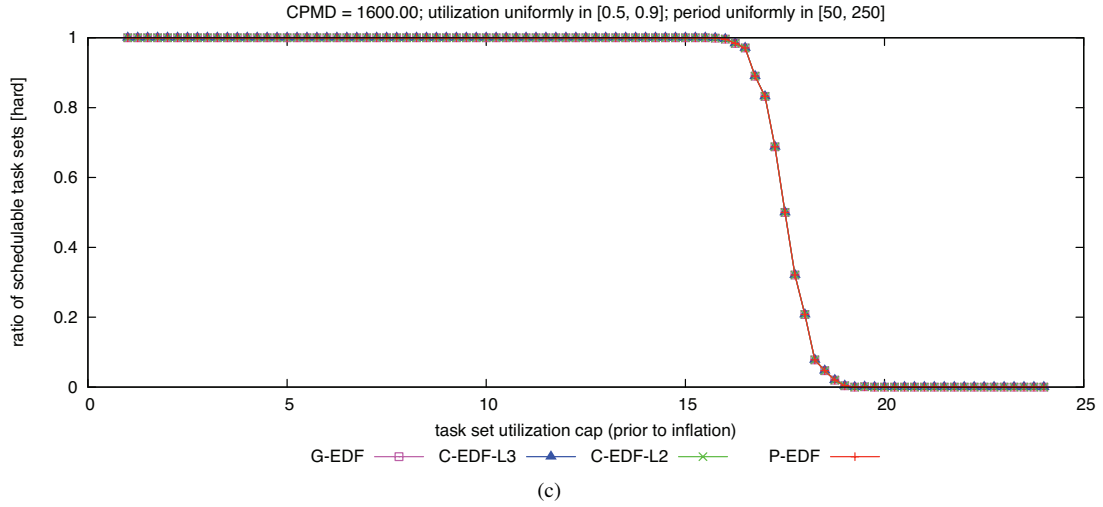
Figure 225: CPMD = 1600.00. Hard W(D) schedulability of task sets with uniform heavy per-task utilizations and (a) short, (b) moderate, and (c) long periods.
