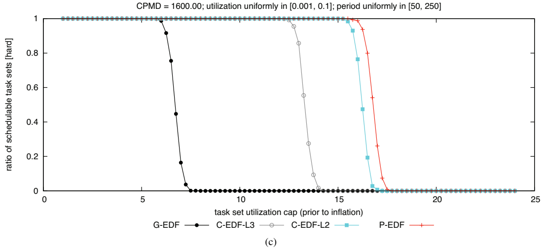
Figure 218: CPMD = 1600.00. Hard BF schedulability of task sets with uniform light per-task utilizations and (a) short, (b) moderate, and (c) long periods.
