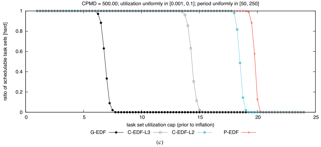
Figure 86: CPMD = 500.00. Hard BF schedulability of task sets with uniform light per-task utilizations and (a) short, (b) moderate, and (c) long periods.
