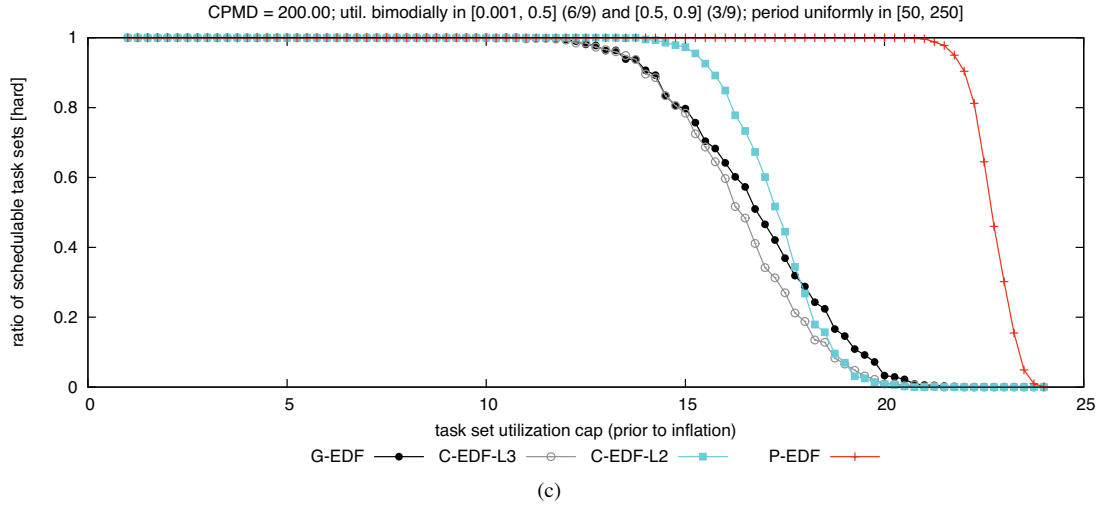
Figure 56: CPMD = 200.00. Hard BF schedulability of task sets with bimodal medium per-task utilizations and (a) short, (b) moderate, and (c) long periods.
