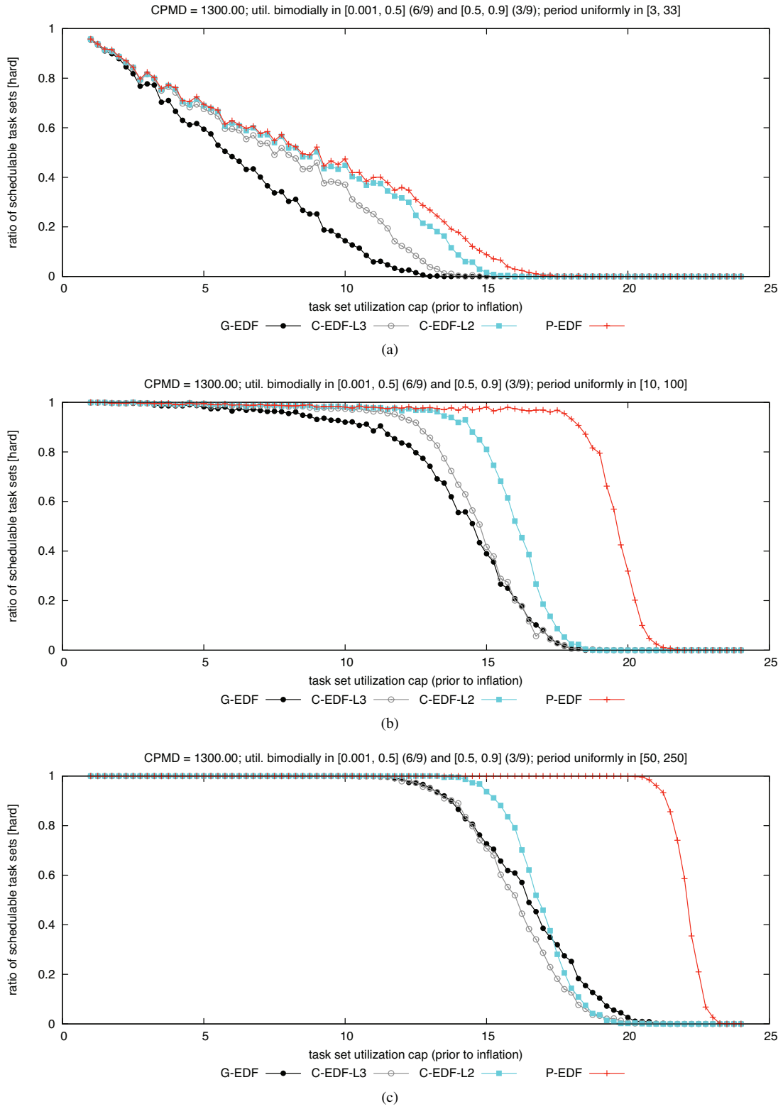
Figure 188: CPMD = 1300.00. Hard BF schedulability of task sets with bimodal medium per-task utilizations and (a) short, (b) moderate, and (c) long periods.
