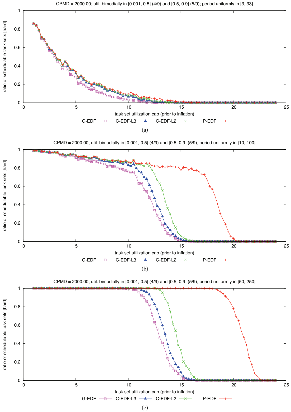
Figure 275: CPMD = 2000.00. Hard W(D) schedulability of task sets with bimodal heavy per-task utilizations and (a) short, (b) moderate, and (c) long periods.
