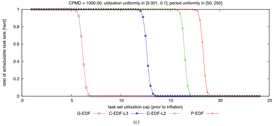
Figure 145: CPMD = 1000.00. Hard W(D) schedulability of task sets with uniform light per-task utilizations and (a) short, (b) moderate, and (c) long periods.
