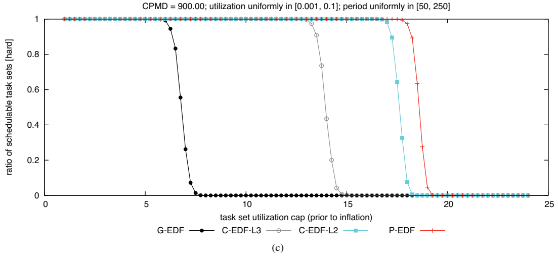
Figure 134: CPMD = 900.00. Hard BF schedulability of task sets with uniform light per-task utilizations and (a) short, (b) moderate, and (c) long periods.
