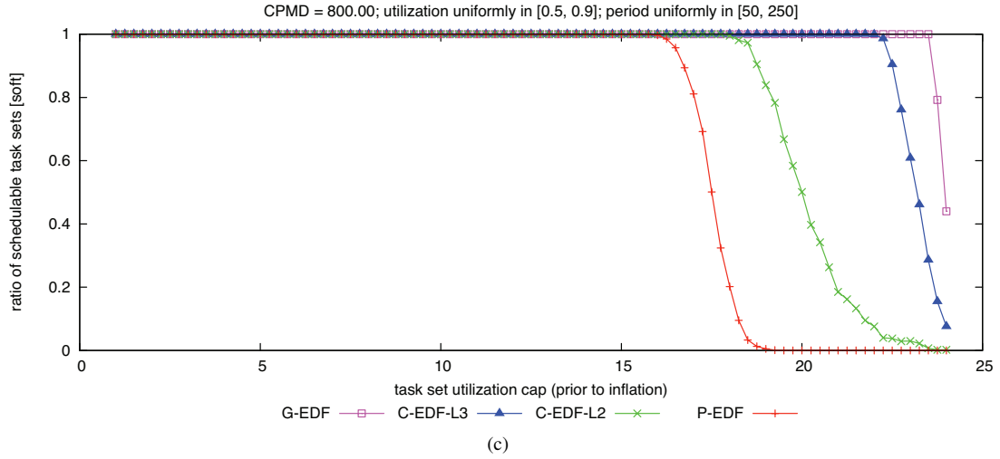
Figure 329: CPMD = 800.00. Soft schedulability of task sets with uniform heavy per-task utilizations and (a) short, (b) moderate, and (c) long periods.
