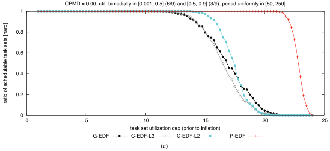
Figure 32: CPMD = 0.00. Hard BF schedulability of task sets with bimodal medium per-task utilizations and (a) short, (b) moderate, and (c) long periods.
