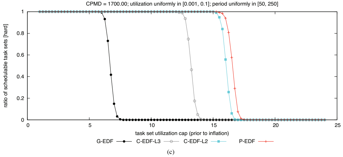
Figure 230: CPMD = 1700.00. Hard BF schedulability of task sets with uniform light per-task utilizations and (a) short, (b) moderate, and (c) long periods.
