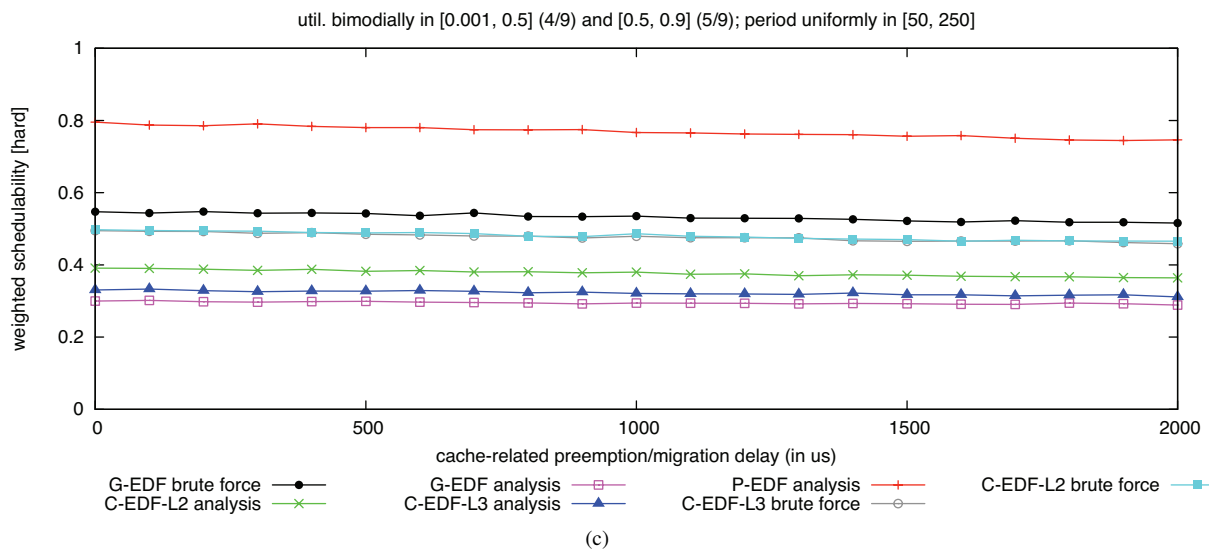
Figure 18: Hard weighted schedulability of task sets with bimodal heavy per-task utilizations and (a) short, (b) moderate, and (c) long periods.
