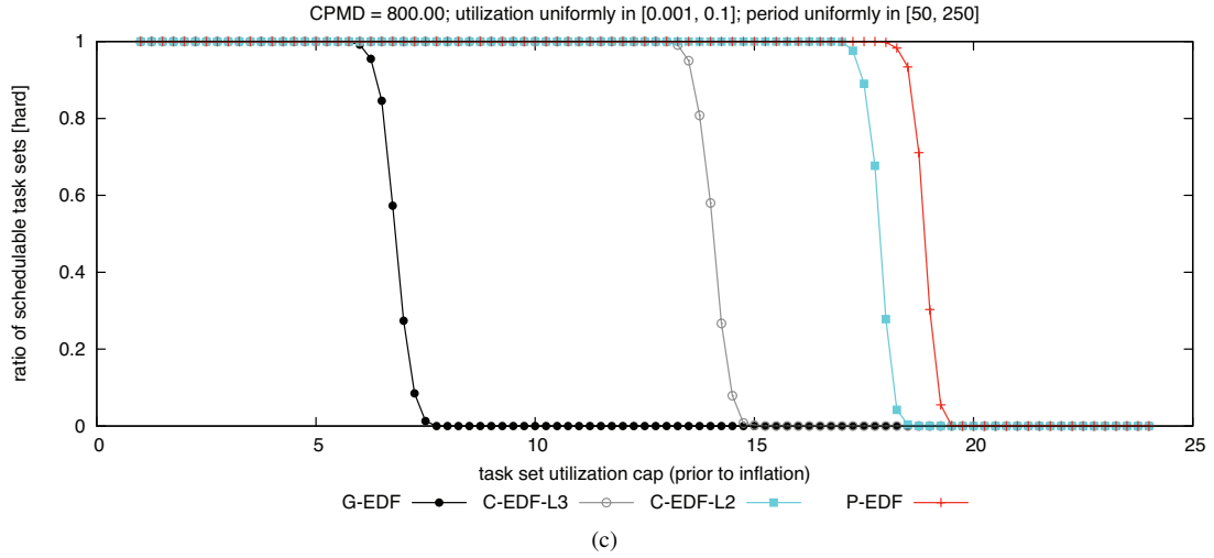
Figure 122: CPMD = 800.00. Hard BF schedulability of task sets with uniform light per-task utilizations and (a) short, (b) moderate, and (c) long periods.
