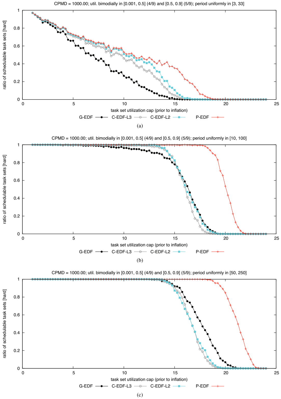
Figure 156: CPMD = 1000.00. Hard BF schedulability of task sets with bimodal heavy per-task utilizations and (a) short, (b) moderate, and (c) long periods.
