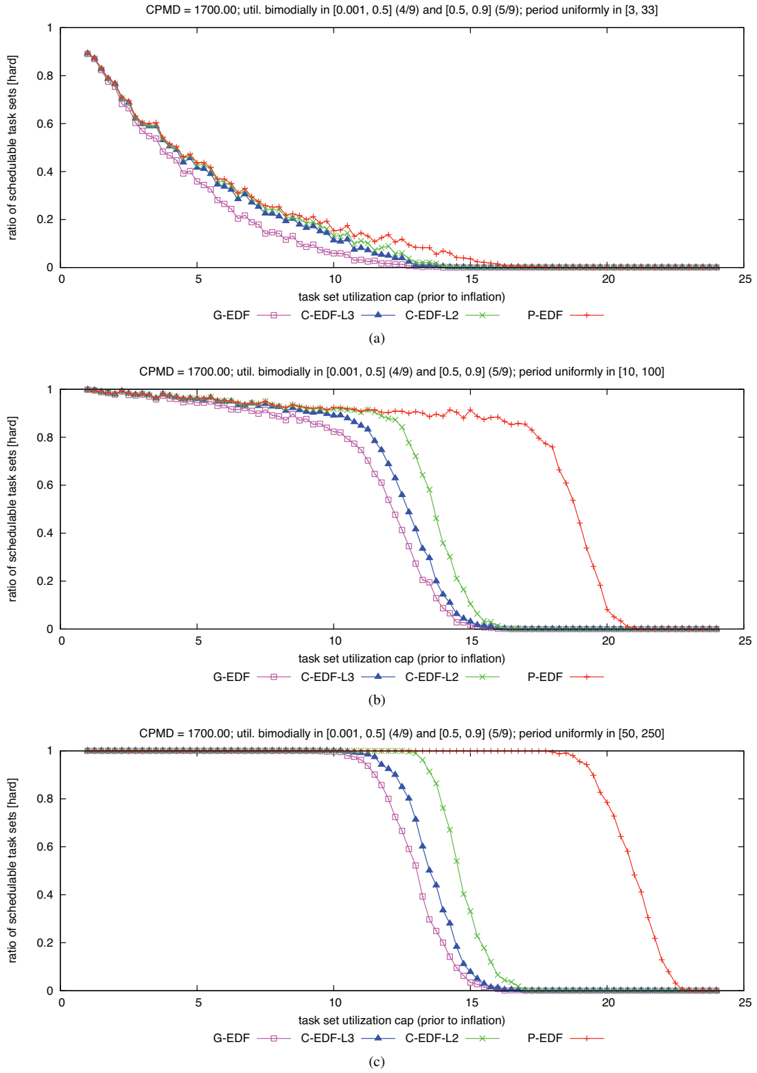
Figure 239: CPMD = 1700.00. Hard W(D) schedulability of task sets with bimodal heavy per-task utilizations and (a) short, (b) moderate, and (c) long periods.
