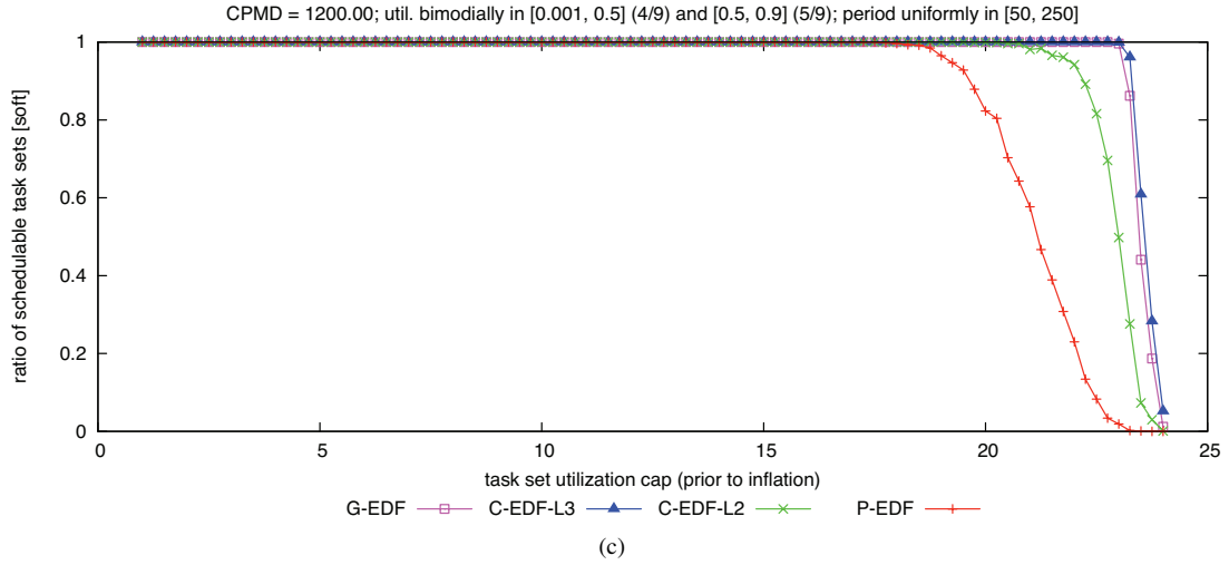
Figure 354: CPMD = 1200.00. Soft schedulability of task sets with bimodal heavy per-task utilizations and (a) short, (b) moderate, and (c) long periods.
