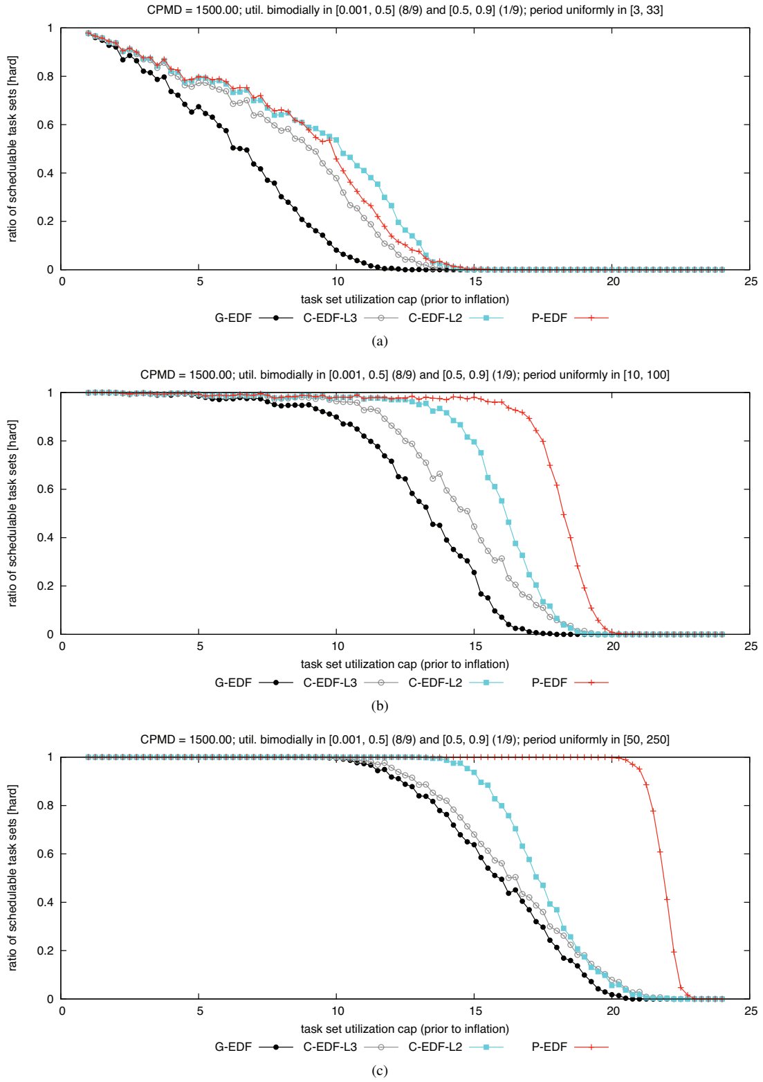
Figure 208: CPMD = 1500.00. Hard BF schedulability of task sets with bimodal light per-task utilizations and (a) short, (b) moderate, and (c) long periods.
