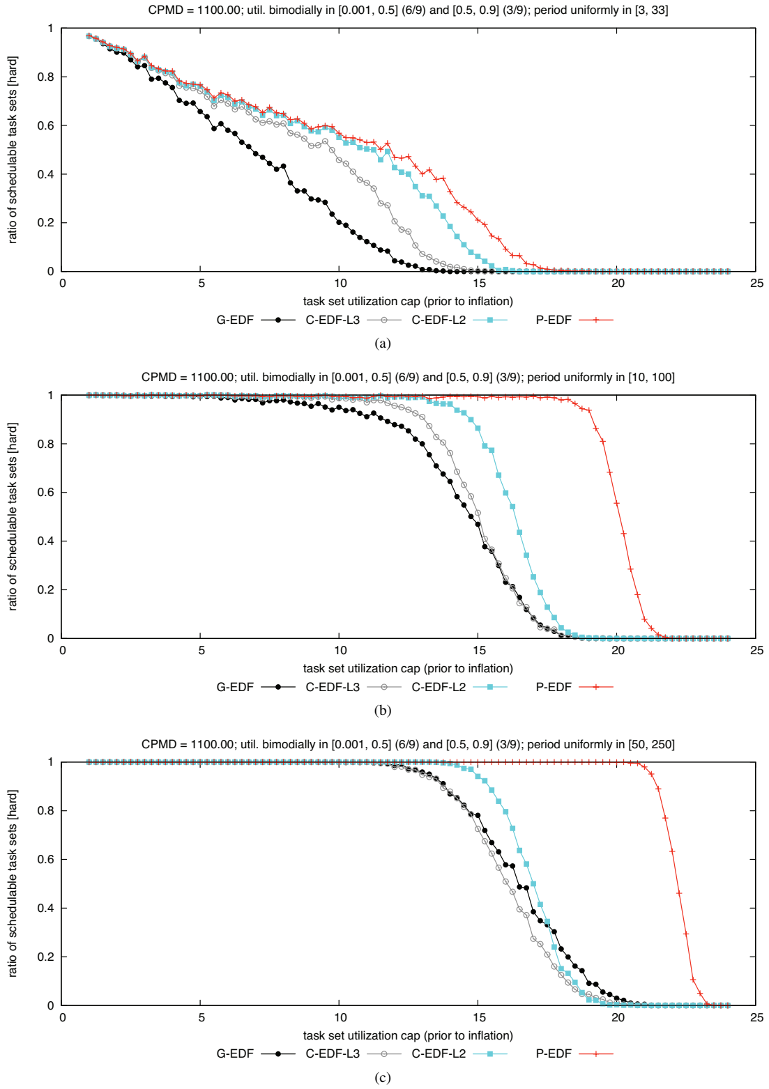
Figure 164: CPMD = 1100.00. Hard BF schedulability of task sets with bimodal medium per-task utilizations and (a) short, (b) moderate, and (c) long periods.
