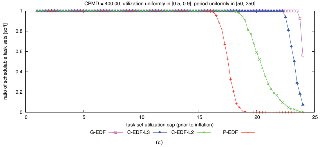
Figure 305: CPMD = 400.00. Soft schedulability of task sets with uniform heavy per-task utilizations and (a) short, (b) moderate, and (c) long periods.
