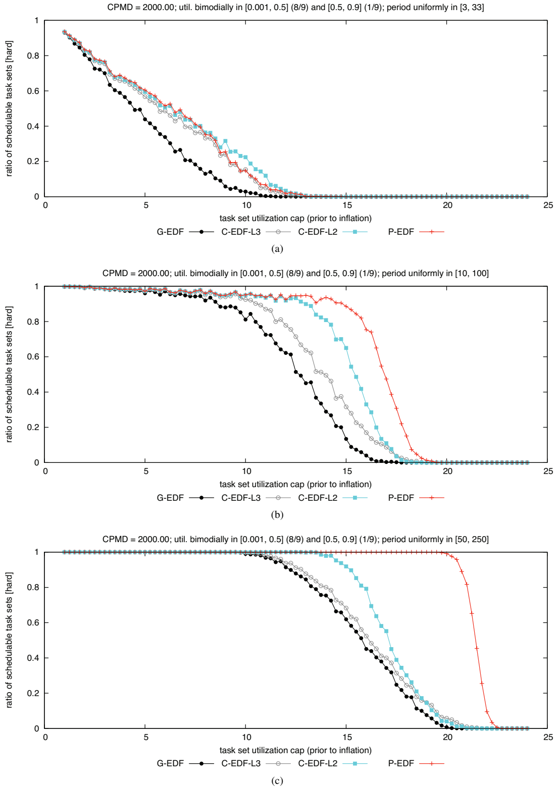
Figure 268: CPMD = 2000.00. Hard BF schedulability of task sets with bimodal light per-task utilizations and (a) short, (b) moderate, and (c) long periods.
