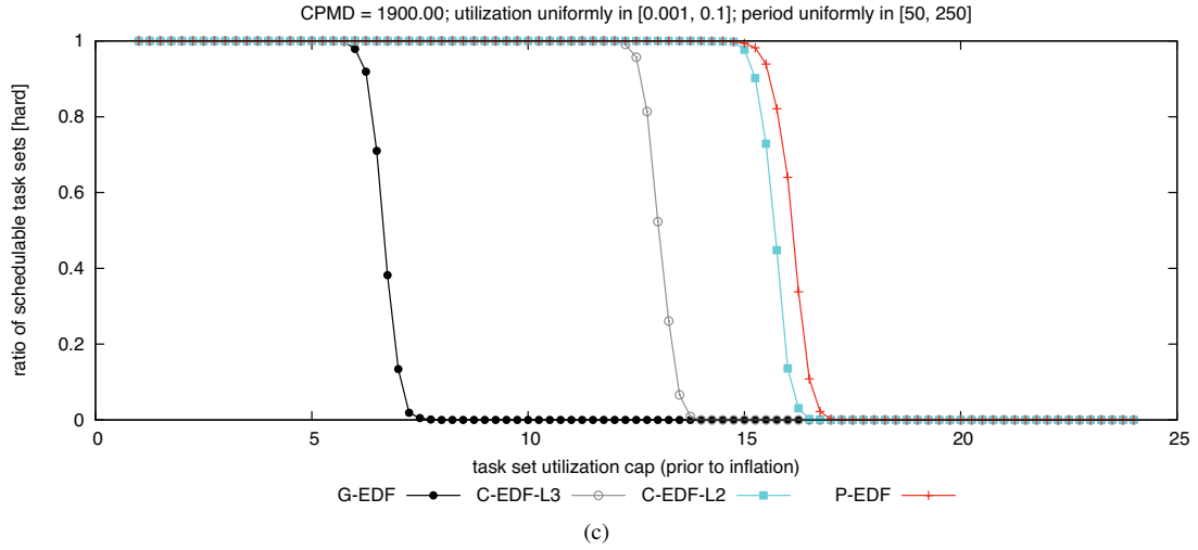
Figure 254: CPMD = 1900.00. Hard BF schedulability of task sets with uniform light per-task utilizations and (a) short, (b) moderate, and (c) long periods.
