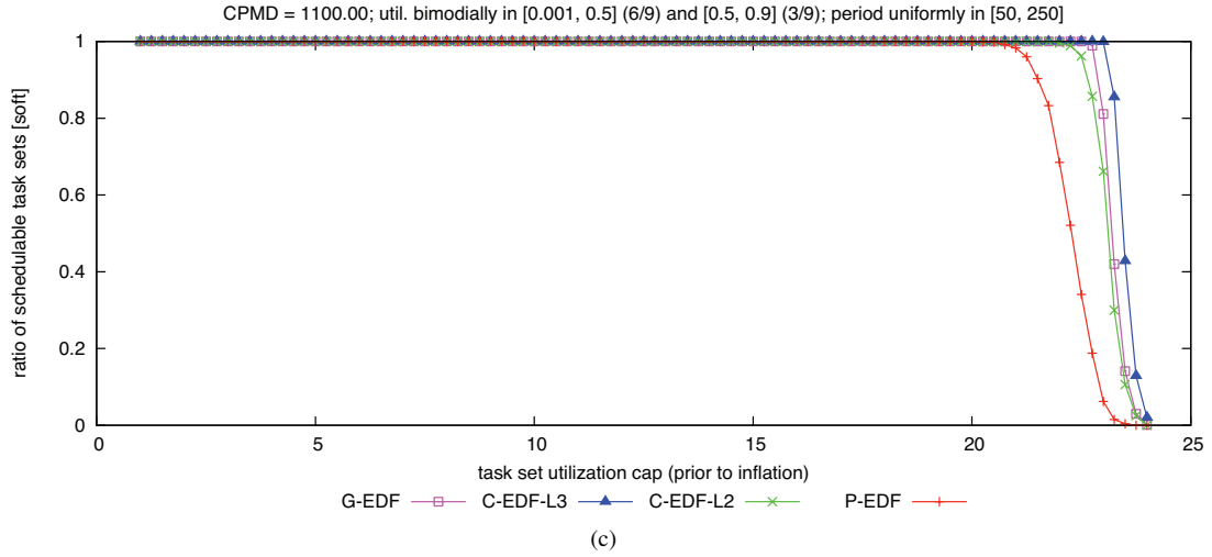
Figure 346: CPMD = 1100.00. Soft schedulability of task sets with bimodal medium per-task utilizations and (a) short, (b) moderate, and (c) long periods.
