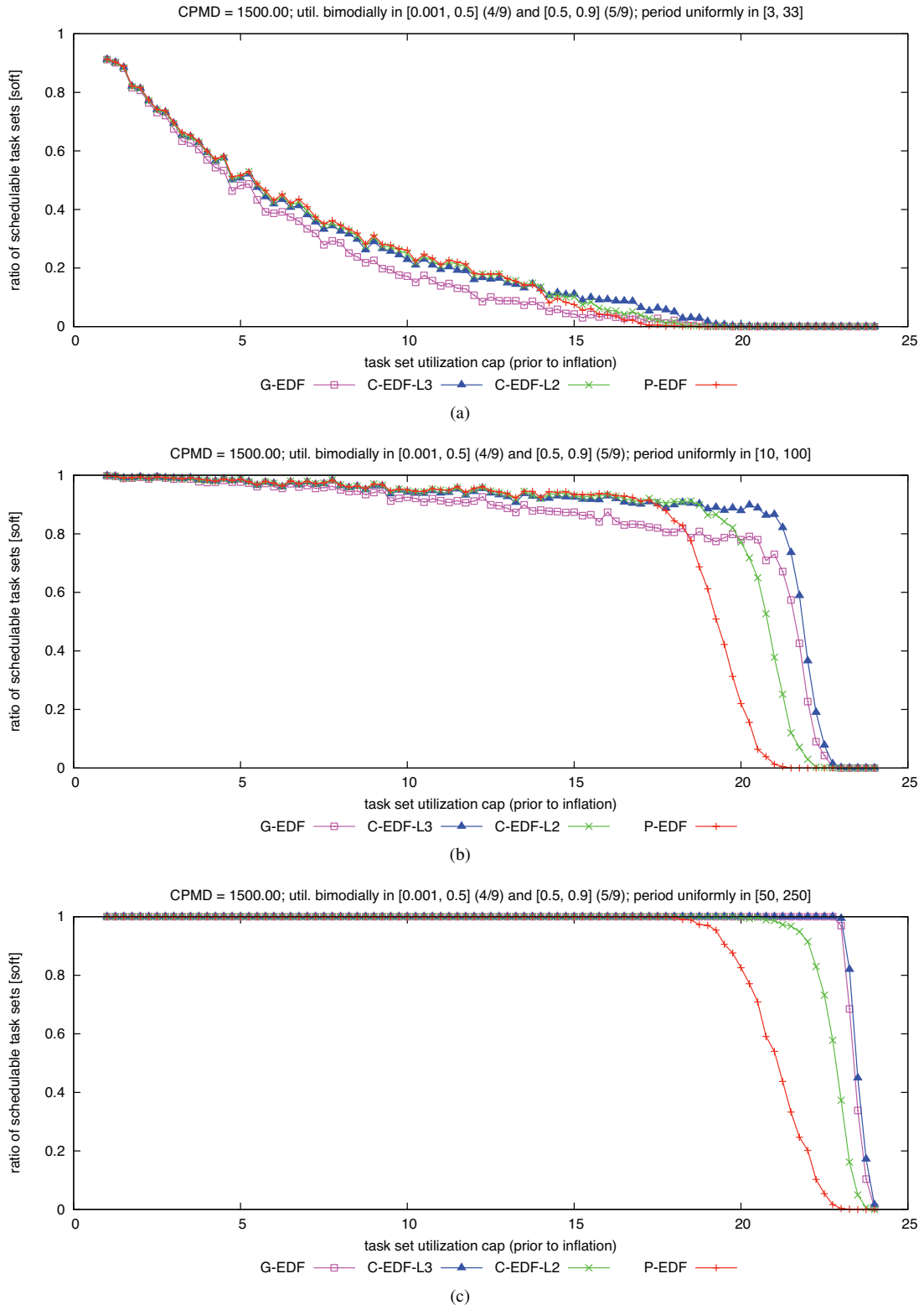
Figure 372: CPMD = 1500.00. Soft schedulability of task sets with bimodal heavy per-task utilizations and (a) short, (b) moderate, and (c) long periods.
