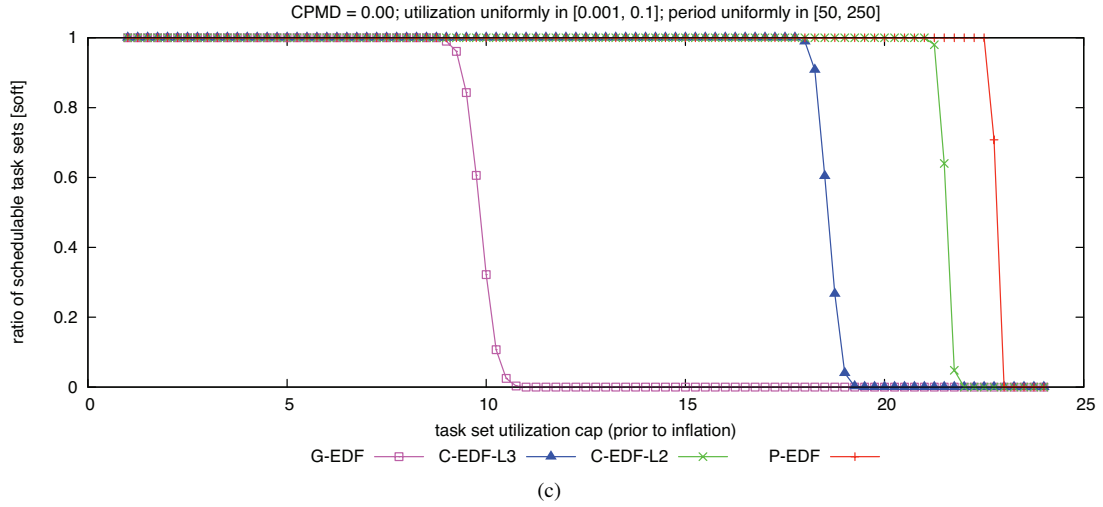
Figure 277: CPMD = 0.00. Soft schedulability of task sets with uniform light per-task utilizations and (a) short, (b) moderate, and (c) long periods.
