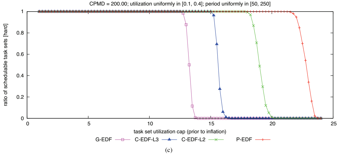
Figure 53: CPMD = 200.00. Hard W(D) schedulability of task sets with uniform medium per-task utilizations and (a) short, (b) moderate, and (c) long periods.
