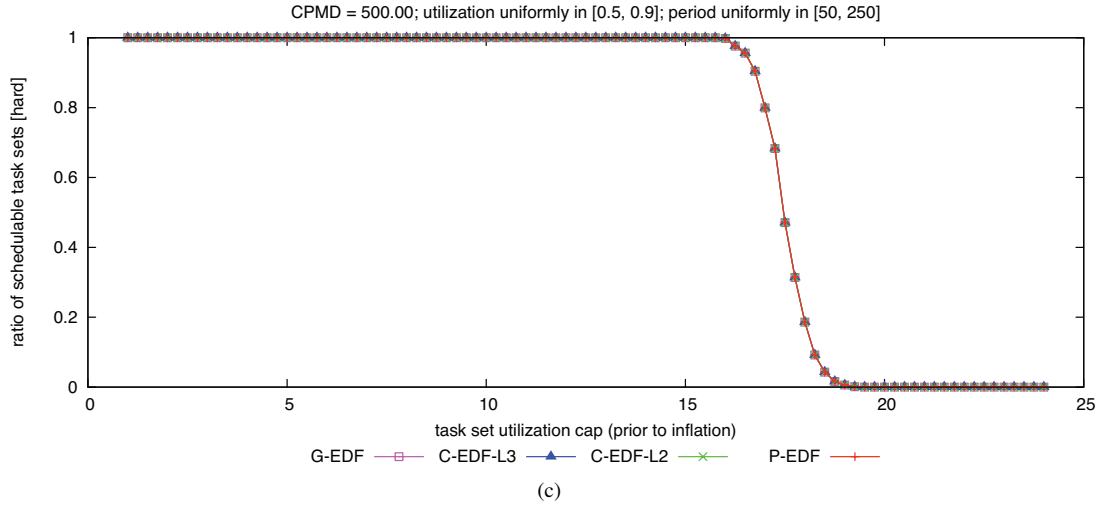
Figure 93: CPMD = 500.00. Hard W(D) schedulability of task sets with uniform heavy per-task utilizations and (a) short, (b) moderate, and (c) long periods.
