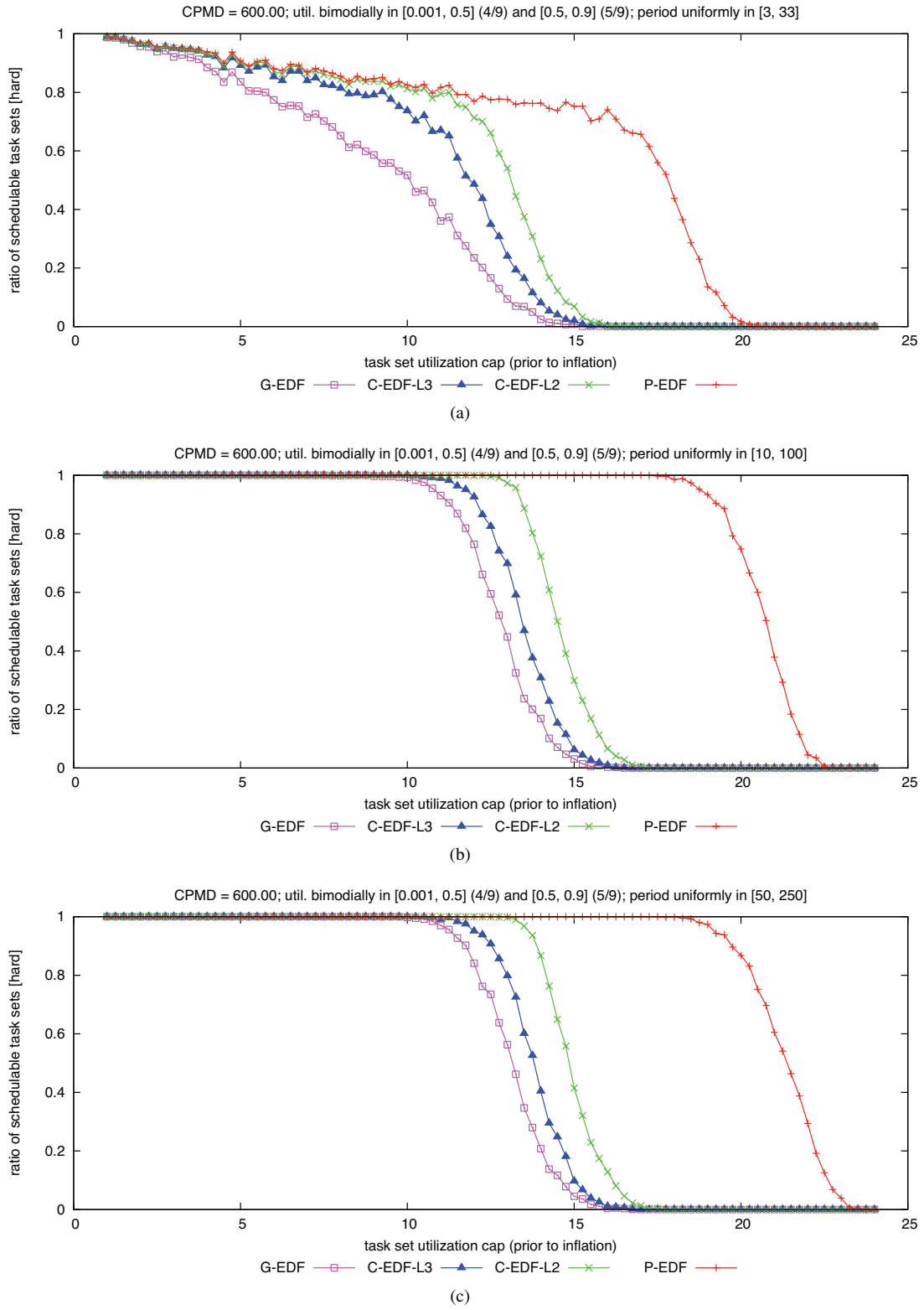
Figure 107: CPMD = 600.00. Hard W(D) schedulability of task sets with bimodal heavy per-task utilizations and (a) short, (b) moderate, and (c) long periods.
