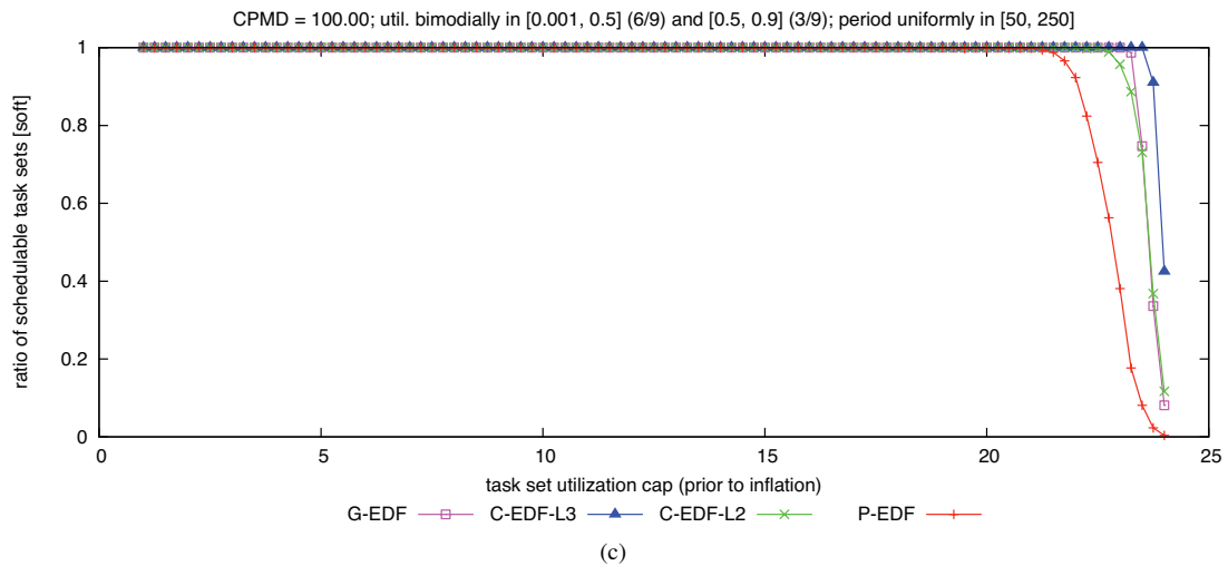
Figure 286: CPMD = 100.00. Soft schedulability of task sets with bimodal medium per-task utilizations and (a) short, (b) moderate, and (c) long periods.
