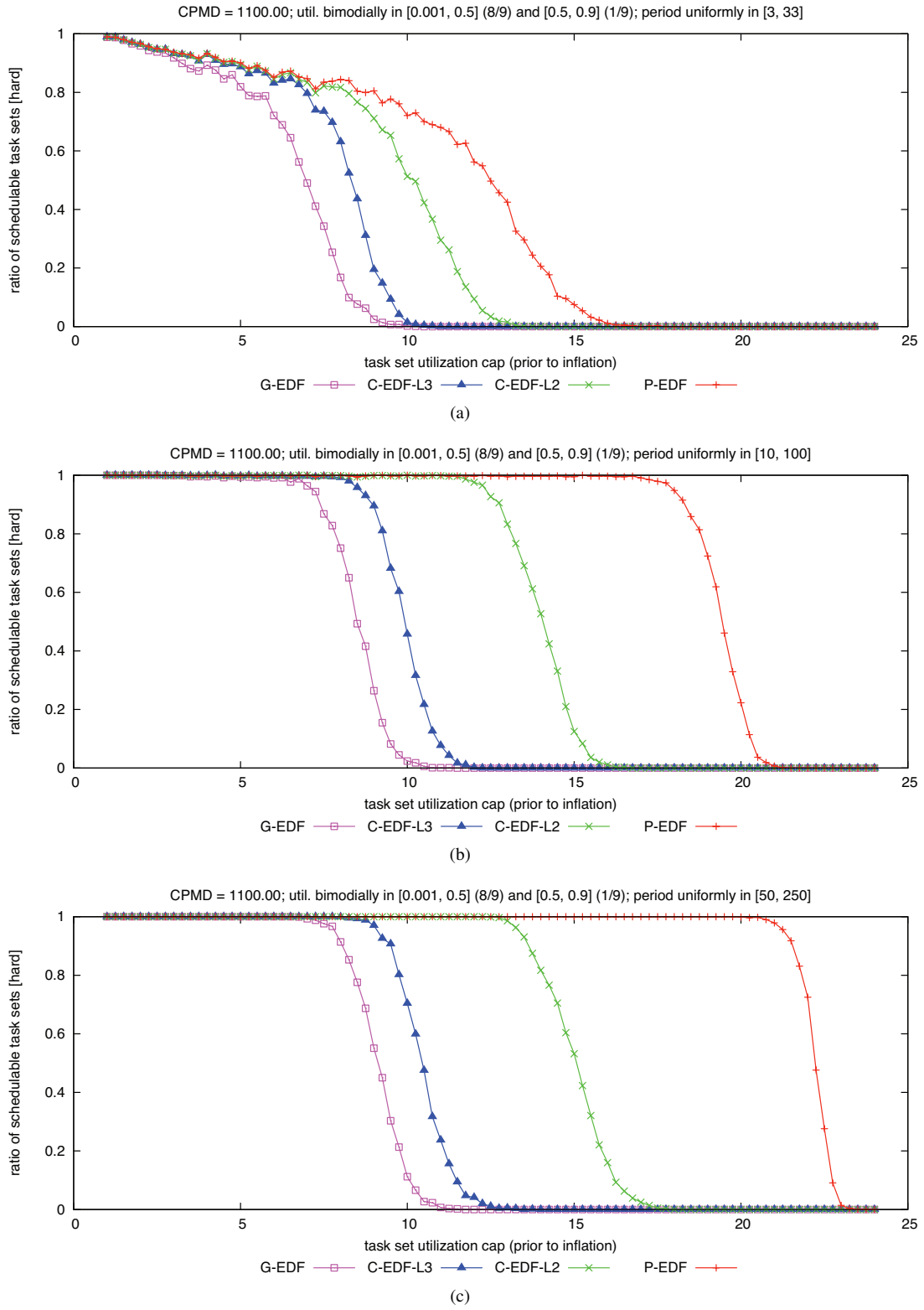
Figure 159: CPMD = 1100.00. Hard W(D) schedulability of task sets with bimodal light per-task utilizations and (a) short, (b) moderate, and (c) long periods.
