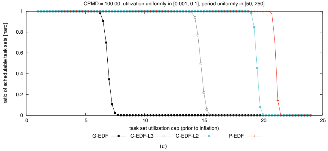
Figure 38: CPMD = 100.00. Hard BF schedulability of task sets with uniform light per-task utilizations and (a) short, (b) moderate, and (c) long periods.
