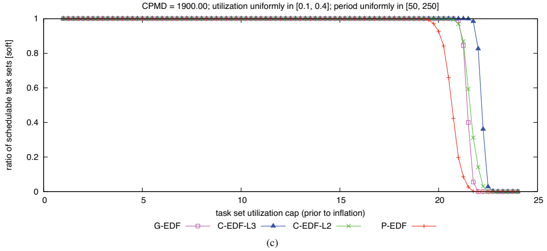
Figure 393: CPMD = 1900.00. Soft schedulability of task sets with uniform medium per-task utilizations and (a) short, (b) moderate, and (c) long periods.
