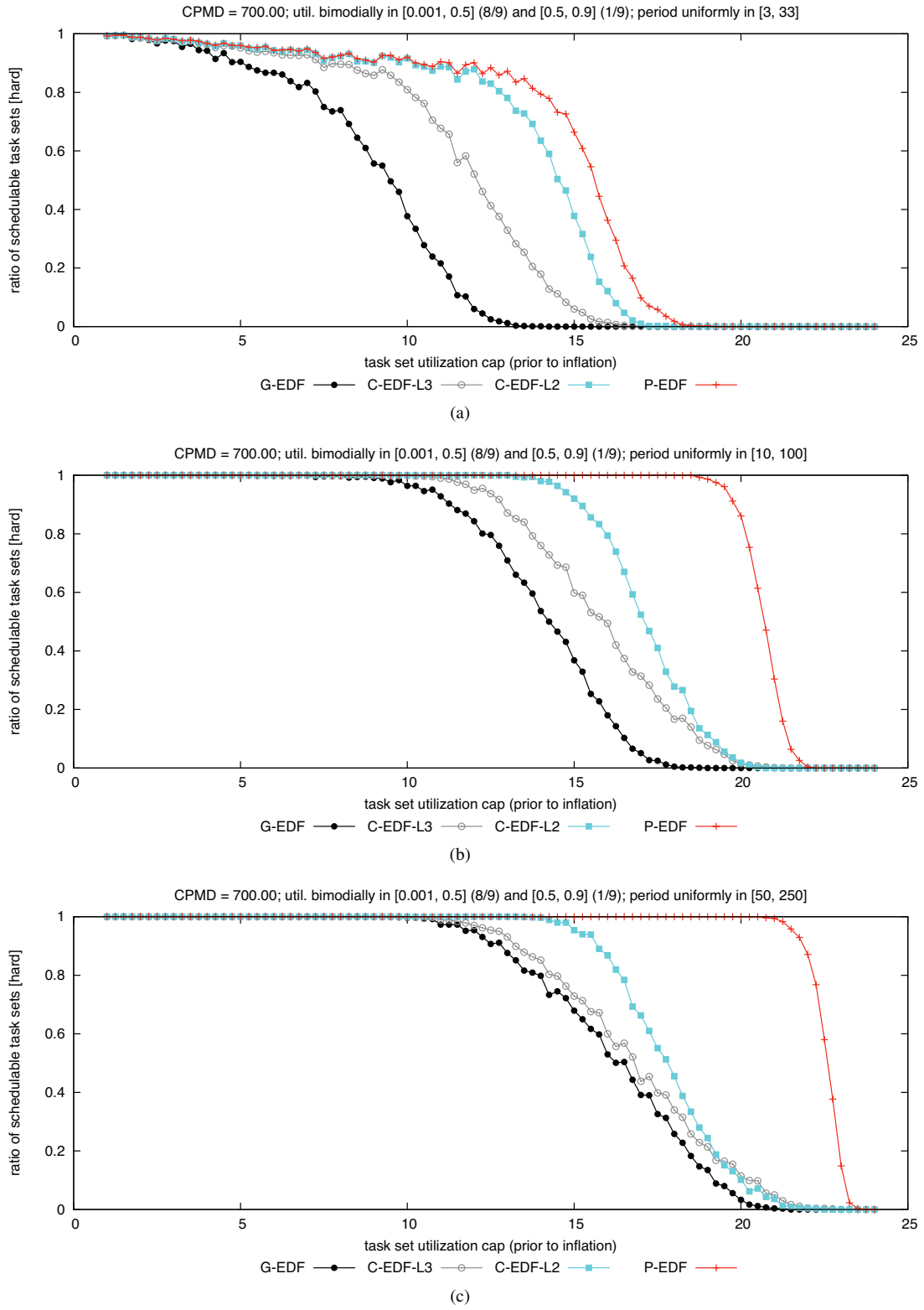
Figure 112: CPMD = 700.00. Hard BF schedulability of task sets with bimodal light per-task utilizations and (a) short, (b) moderate, and (c) long periods.
