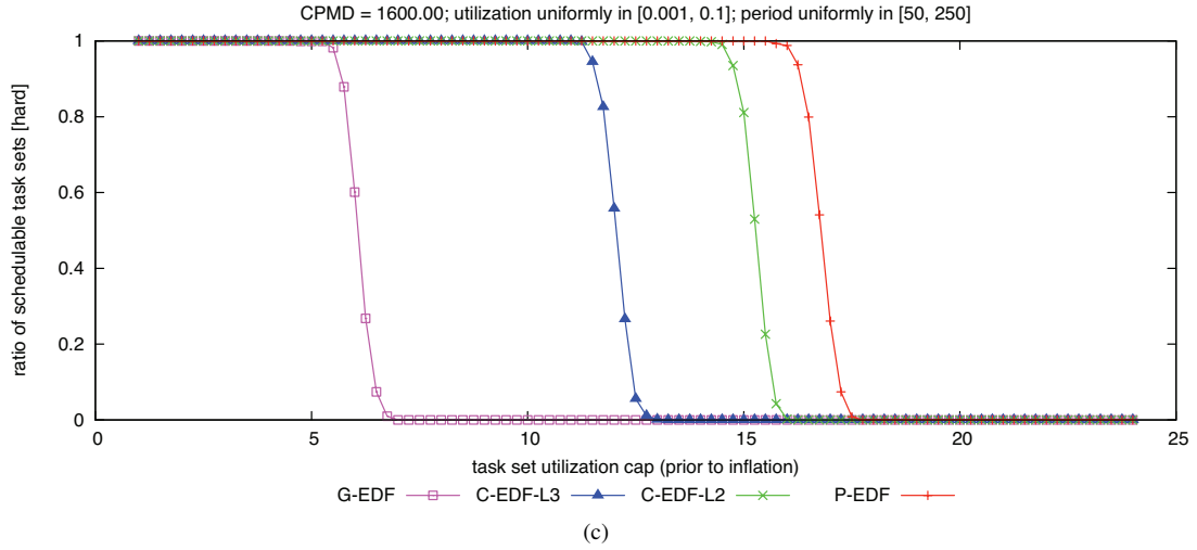
Figure 217: CPMD = 1600.00. Hard W(D) schedulability of task sets with uniform light per-task utilizations and (a) short, (b) moderate, and (c) long periods.
