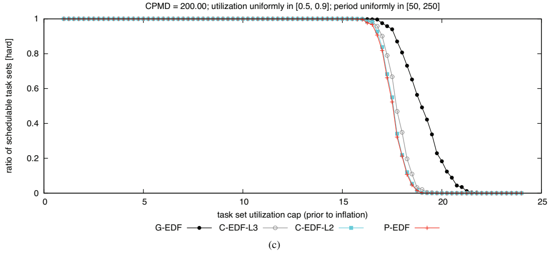
Figure 58: CPMD = 200.00. Hard BF schedulability of task sets with uniform heavy per-task utilizations and (a) short, (b) moderate, and (c) long periods.
