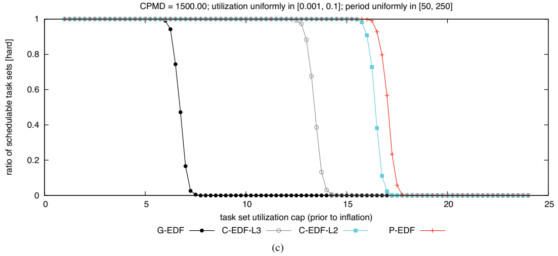
Figure 206: CPMD = 1500.00. Hard BF schedulability of task sets with uniform light per-task utilizations and (a) short, (b) moderate, and (c) long periods.
