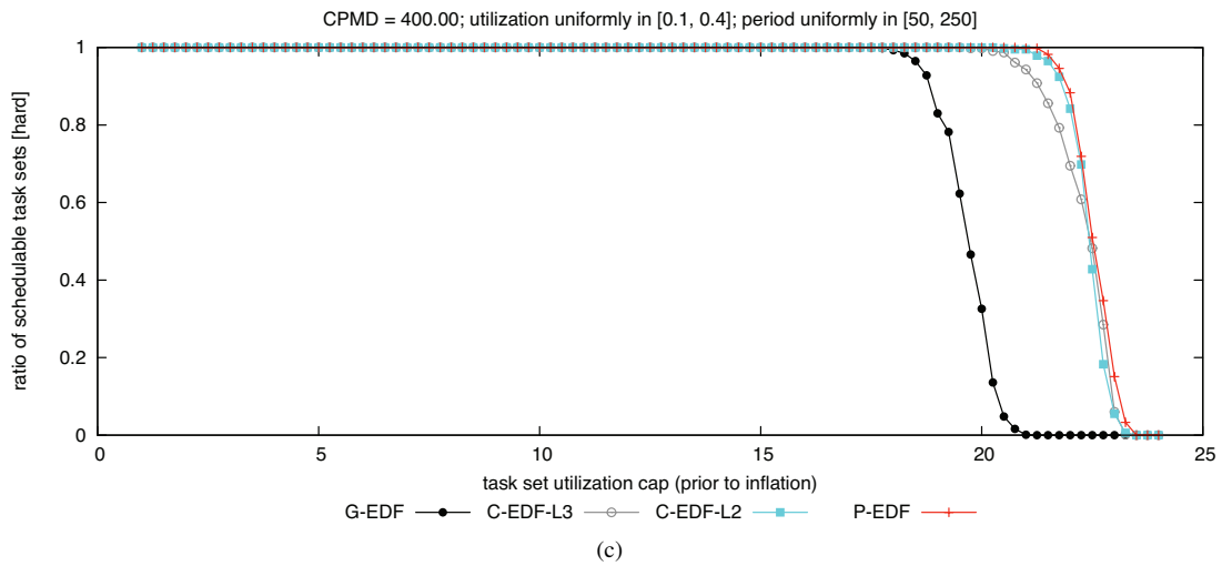
Figure 78: CPMD = 400.00. Hard BF schedulability of task sets with uniform medium per-task utilizations and (a) short, (b) moderate, and (c) long periods.
