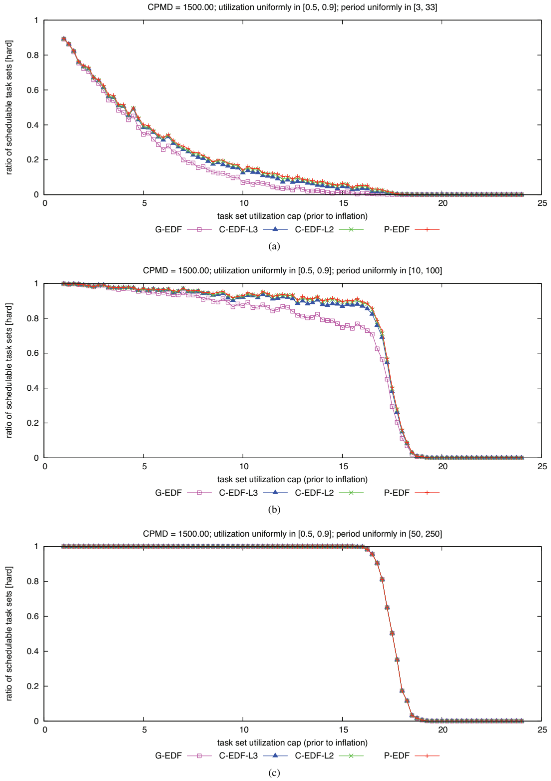
Figure 213: CPMD = 1500.00. Hard W(D) schedulability of task sets with uniform heavy per-task utilizations and (a) short, (b) moderate, and (c) long periods.
