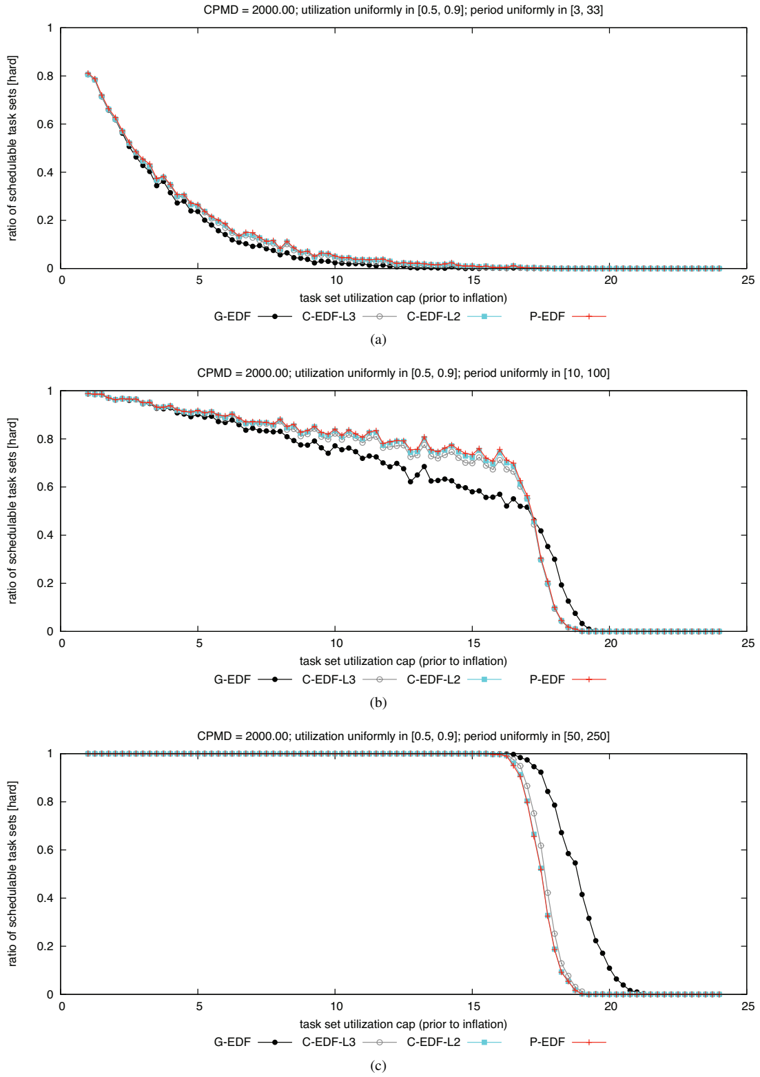
Figure 274: CPMD = 2000.00. Hard BF schedulability of task sets with uniform heavy per-task utilizations and (a) short, (b) moderate, and (c) long periods.
