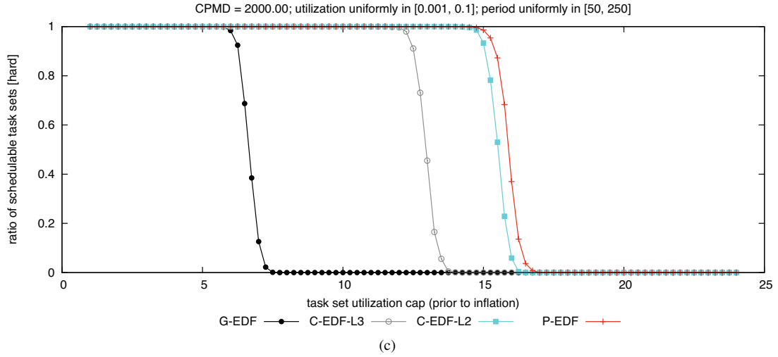
Figure 266: CPMD = 2000.00. Hard BF schedulability of task sets with uniform light per-task utilizations and (a) short, (b) moderate, and (c) long periods.
