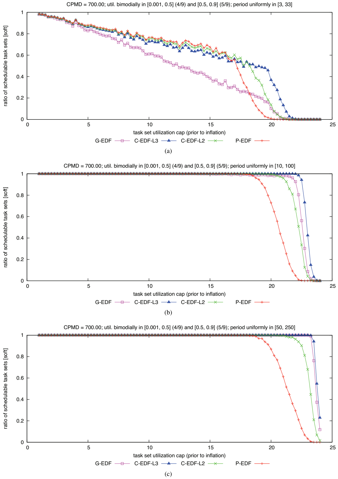
Figure 324: CPMD = 700.00. Soft schedulability of task sets with bimodal heavy per-task utilizations and (a) short, (b) moderate, and (c) long periods.
