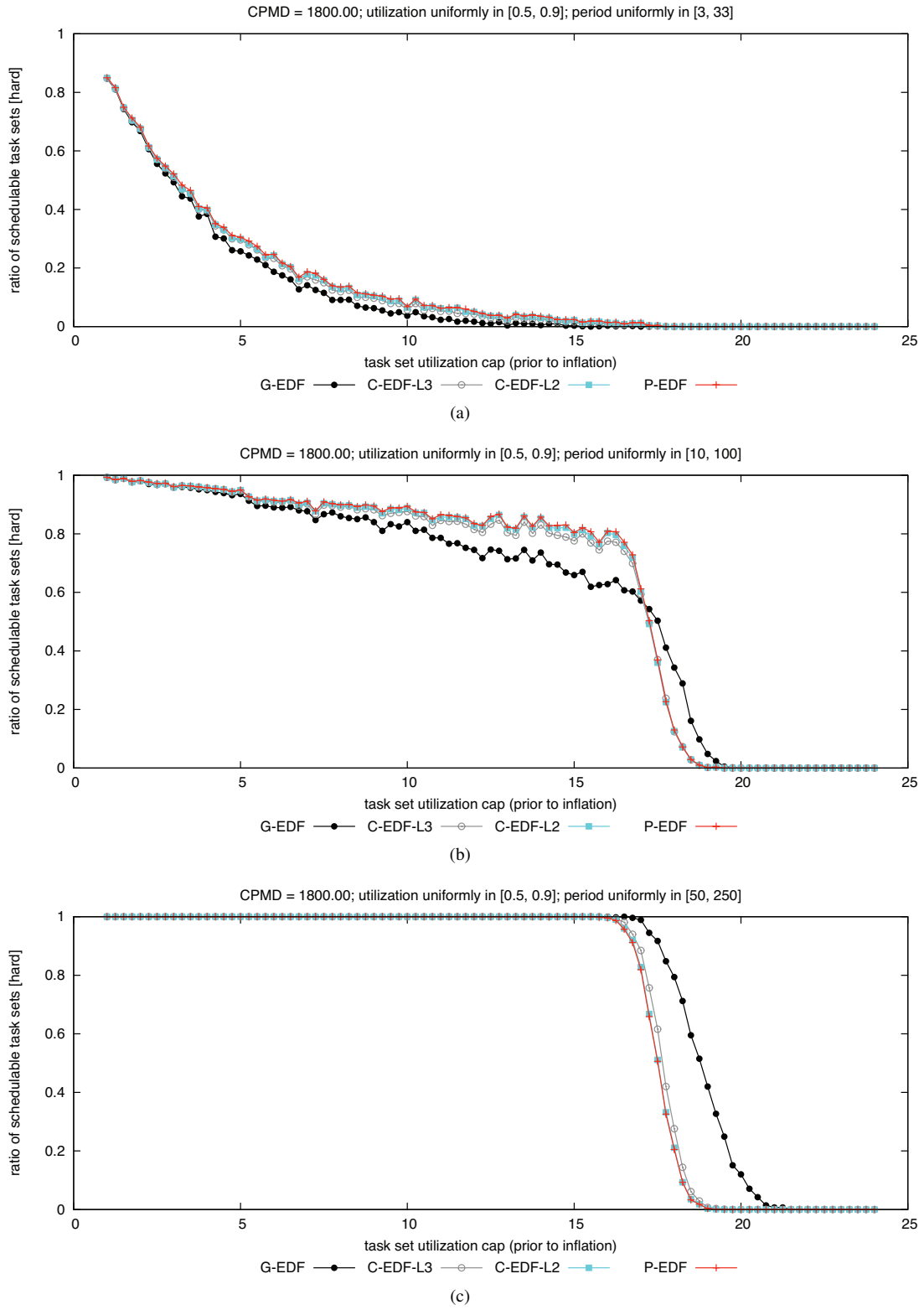
Figure 250: CPMD = 1800.00. Hard BF schedulability of task sets with uniform heavy per-task utilizations and (a) short, (b) moderate, and (c) long periods.
