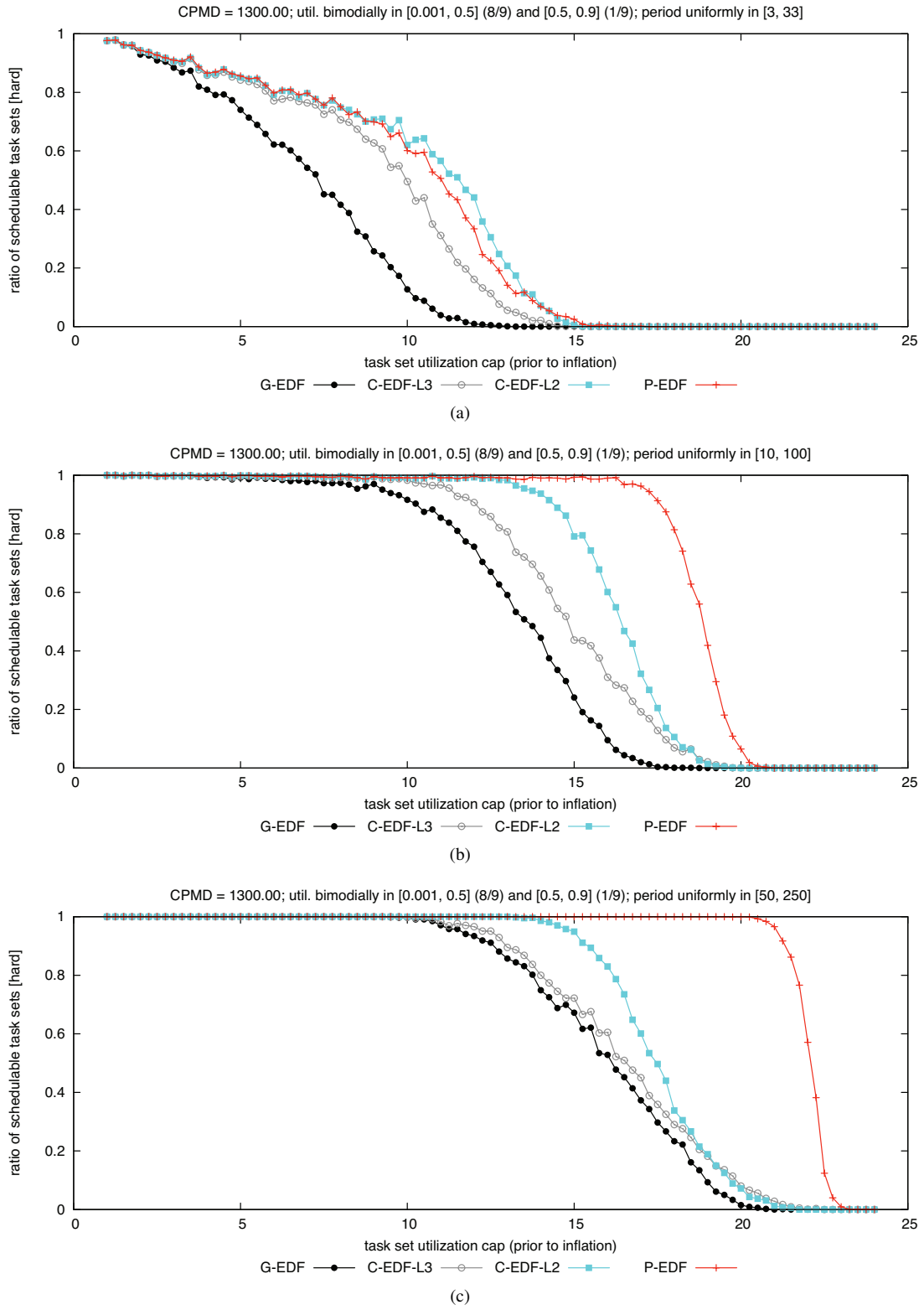
Figure 184: CPMD = 1300.00. Hard BF schedulability of task sets with bimodal light per-task utilizations and (a) short, (b) moderate, and (c) long periods.
