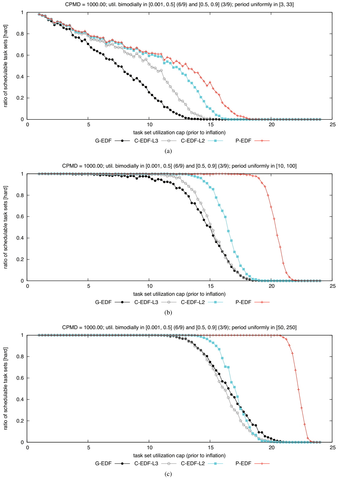
Figure 152: CPMD = 1000.00. Hard BF schedulability of task sets with bimodal medium per-task utilizations and (a) short, (b) moderate, and (c) long periods.
