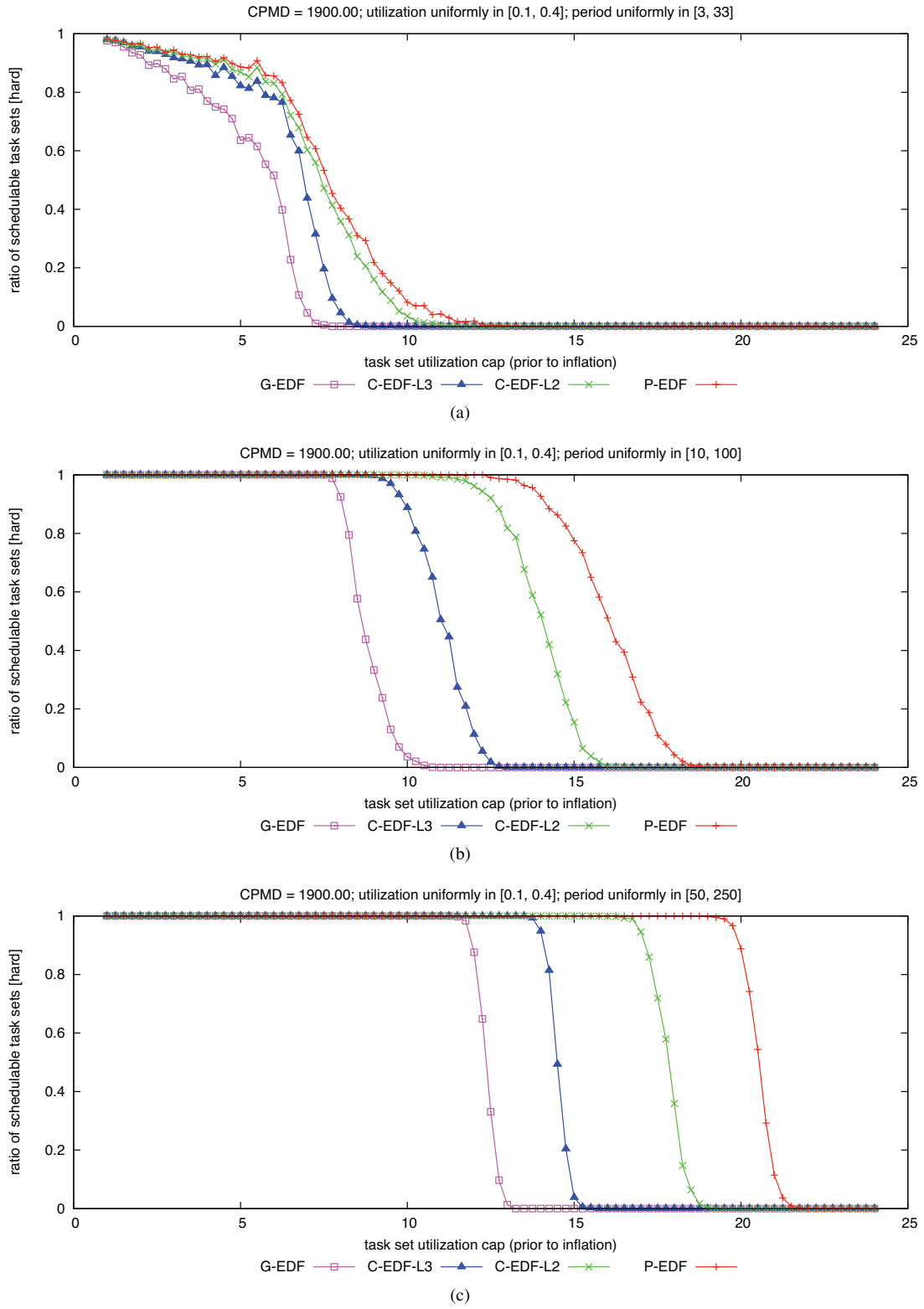
Figure 257: CPMD = 1900.00. Hard W(D) schedulability of task sets with uniform medium per-task utilizations and (a) short, (b) moderate, and (c) long periods.
