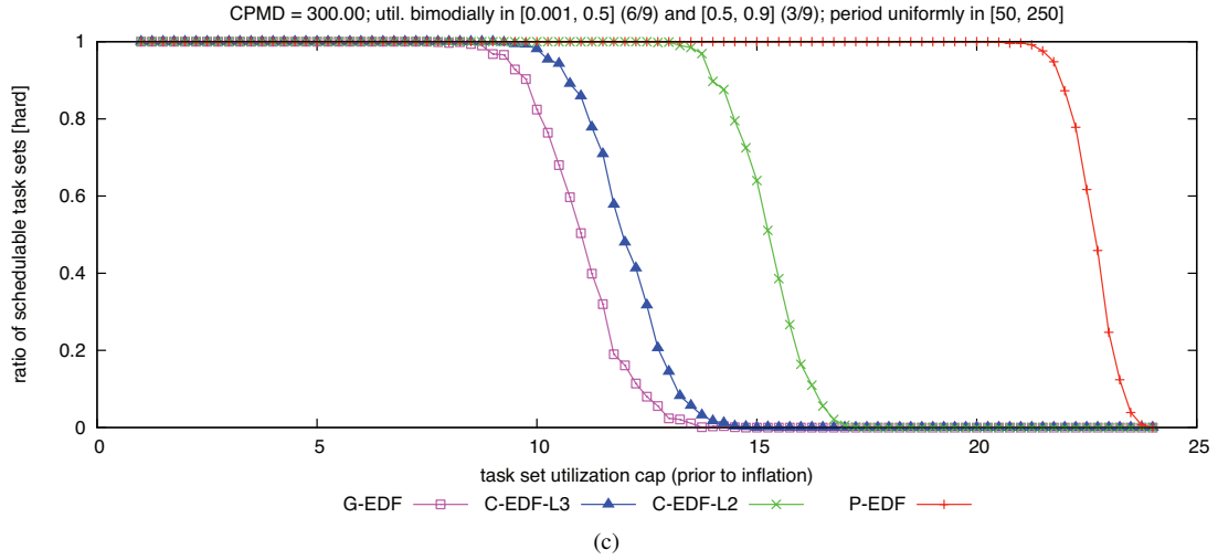
Figure 67: CPMD = 300.00. Hard W(D) schedulability of task sets with bimodal medium per-task utilizations and (a) short, (b) moderate, and (c) long periods.
