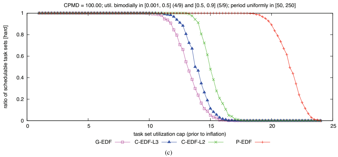
Figure 47: CPMD = 100.00. Hard W(D) schedulability of task sets with bimodal heavy per-task utilizations and (a) short, (b) moderate, and (c) long periods.
