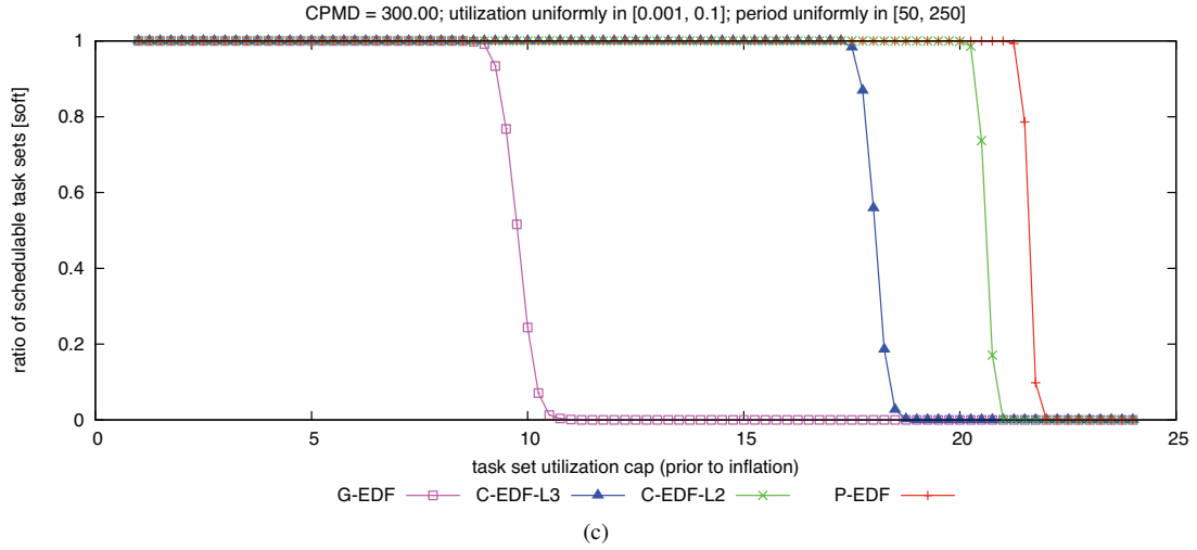
Figure 295: CPMD = 300.00. Soft schedulability of task sets with uniform light per-task utilizations and (a) short, (b) moderate, and (c) long periods.
