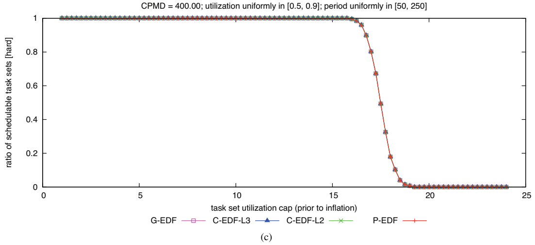
Figure 81: CPMD = 400.00. Hard W(D) schedulability of task sets with uniform heavy per-task utilizations and (a) short, (b) moderate, and (c) long periods.
