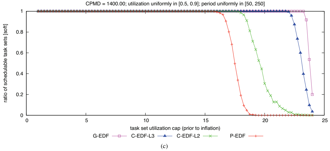
Figure 365: CPMD = 1400.00. Soft schedulability of task sets with uniform heavy per-task utilizations and (a) short, (b) moderate, and (c) long periods.
