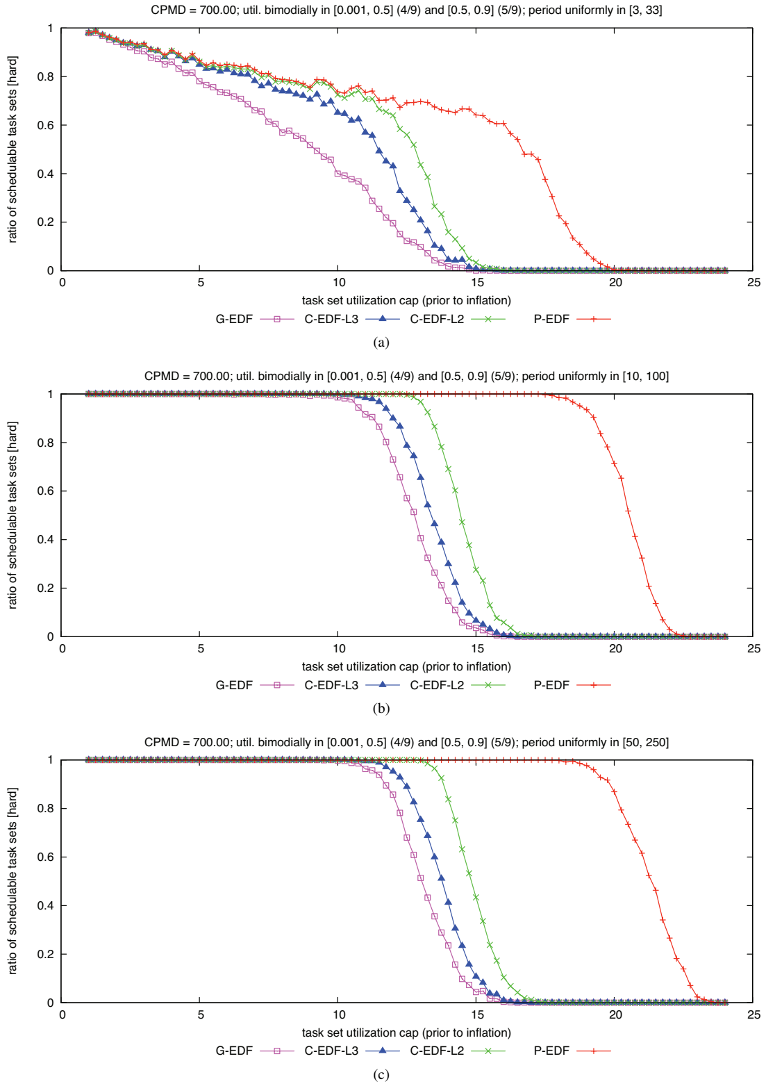
Figure 119: CPMD = 700.00. Hard W(D) schedulability of task sets with bimodal heavy per-task utilizations and (a) short, (b) moderate, and (c) long periods.
