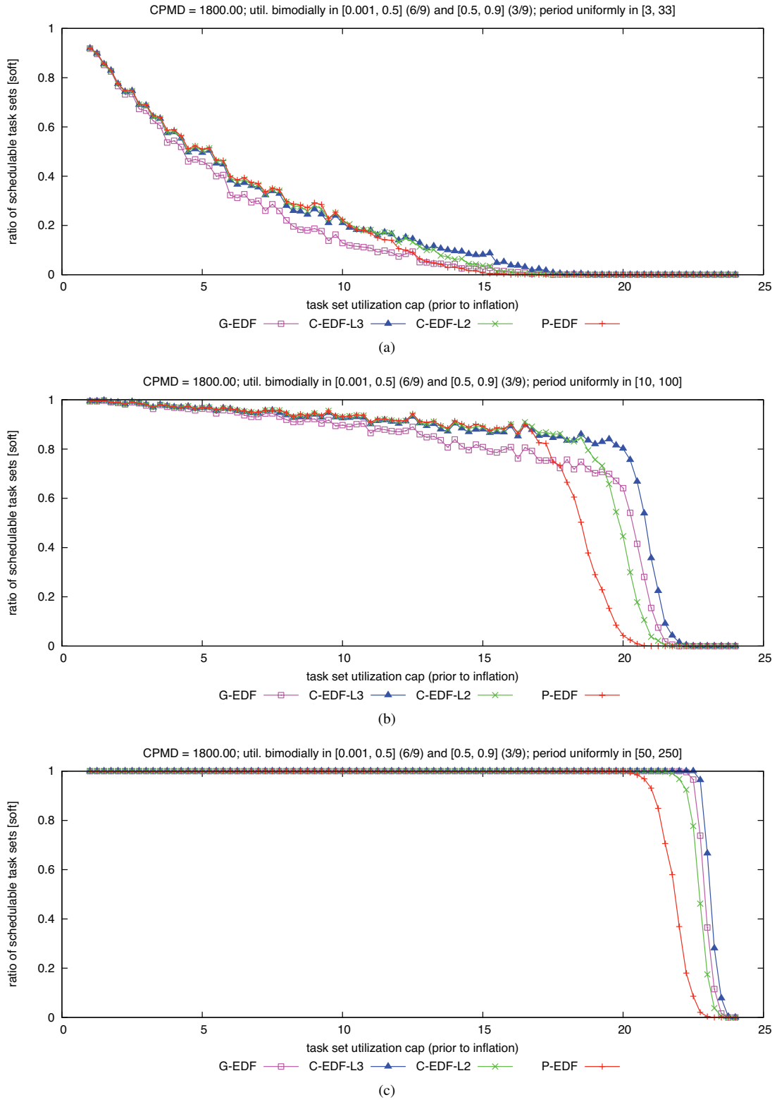
Figure 388: CPMD = 1800.00. Soft schedulability of task sets with bimodal medium per-task utilizations and (a) short, (b) moderate, and (c) long periods.
