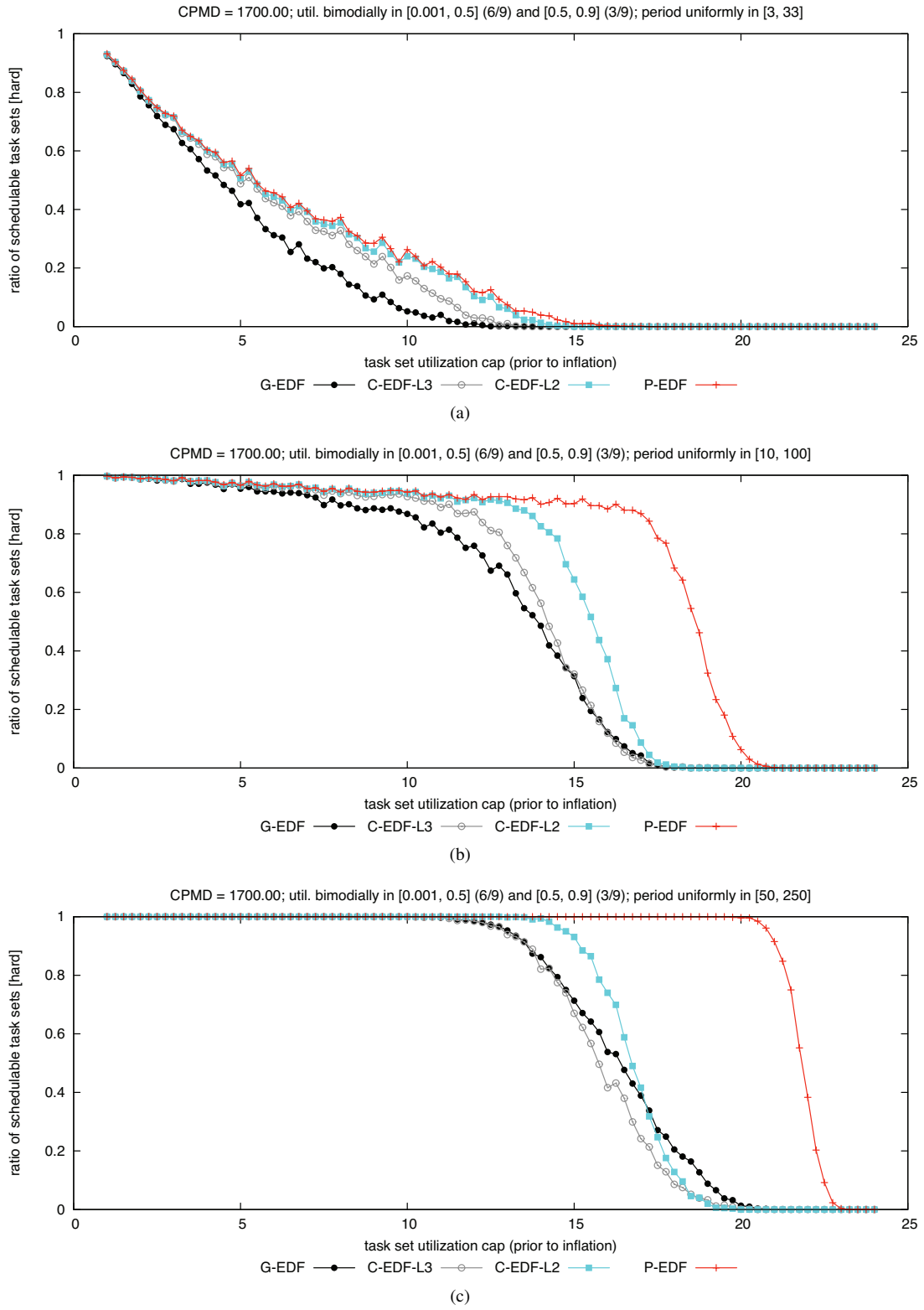
Figure 236: CPMD = 1700.00. Hard BF schedulability of task sets with bimodal medium per-task utilizations and (a) short, (b) moderate, and (c) long periods.
