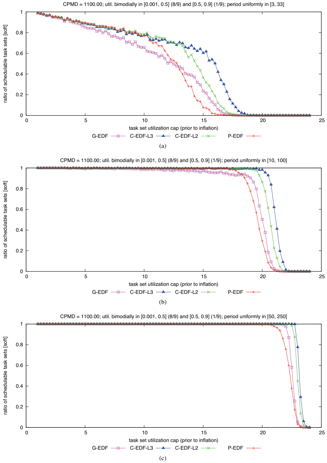
Figure 344: CPMD = 1100.00. Soft schedulability of task sets with bimodal light per-task utilizations and (a) short, (b) moderate, and (c) long periods.
