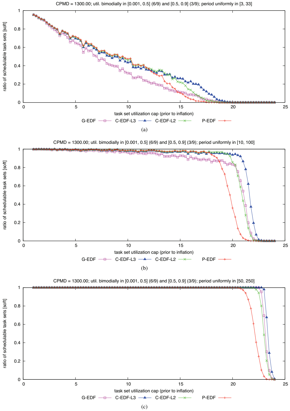
Figure 358: CPMD = 1300.00. Soft schedulability of task sets with bimodal medium per-task utilizations and (a) short, (b) moderate, and (c) long periods.
