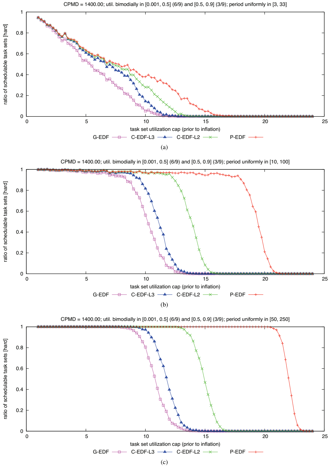
Figure 199: CPMD = 1400.00. Hard W(D) schedulability of task sets with bimodal medium per-task utilizations and (a) short, (b) moderate, and (c) long periods.
