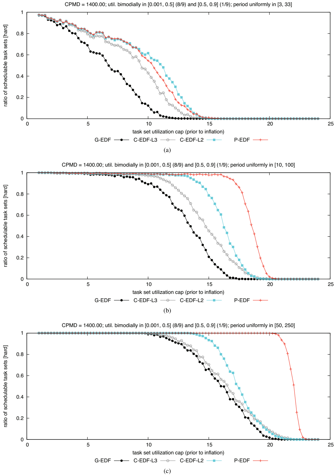
Figure 196: CPMD = 1400.00. Hard BF schedulability of task sets with bimodal light per-task utilizations and (a) short, (b) moderate, and (c) long periods.
