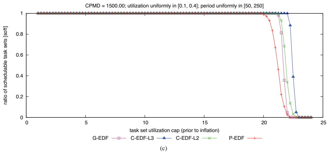
Figure 369: CPMD = 1500.00. Soft schedulability of task sets with uniform medium per-task utilizations and (a) short, (b) moderate, and (c) long periods.
