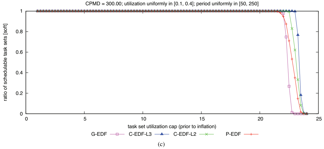
Figure 297: CPMD = 300.00. Soft schedulability of task sets with uniform medium per-task utilizations and (a) short, (b) moderate, and (c) long periods.
