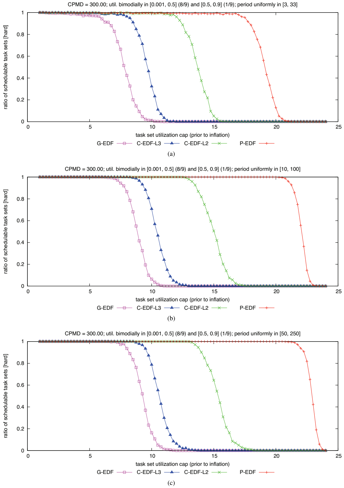
Figure 63: CPMD = 300.00. Hard W(D) schedulability of task sets with bimodal light per-task utilizations and (a) short, (b) moderate, and (c) long periods.
