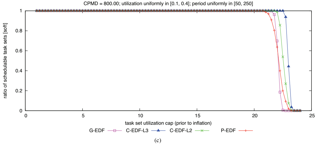
Figure 327: CPMD = 800.00. Soft schedulability of task sets with uniform medium per-task utilizations and (a) short, (b) moderate, and (c) long periods.
