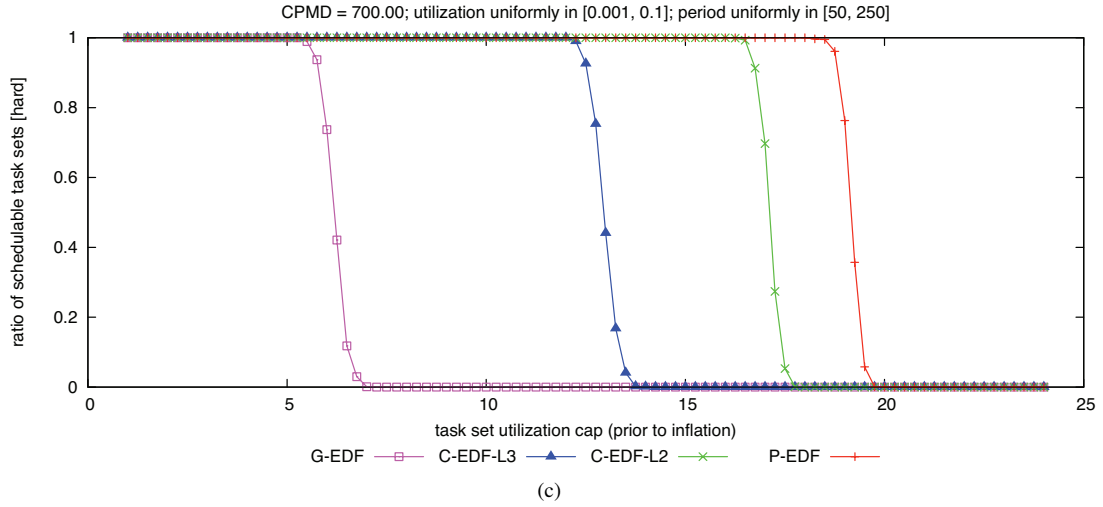
Figure 109: CPMD = 700.00. Hard W(D) schedulability of task sets with uniform light per-task utilizations and (a) short, (b) moderate, and (c) long periods.
