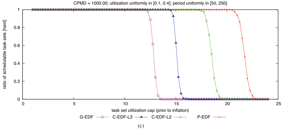
Figure 149: CPMD = 1000.00. Hard W(D) schedulability of task sets with uniform medium per-task utilizations and (a) short, (b) moderate, and (c) long periods.
