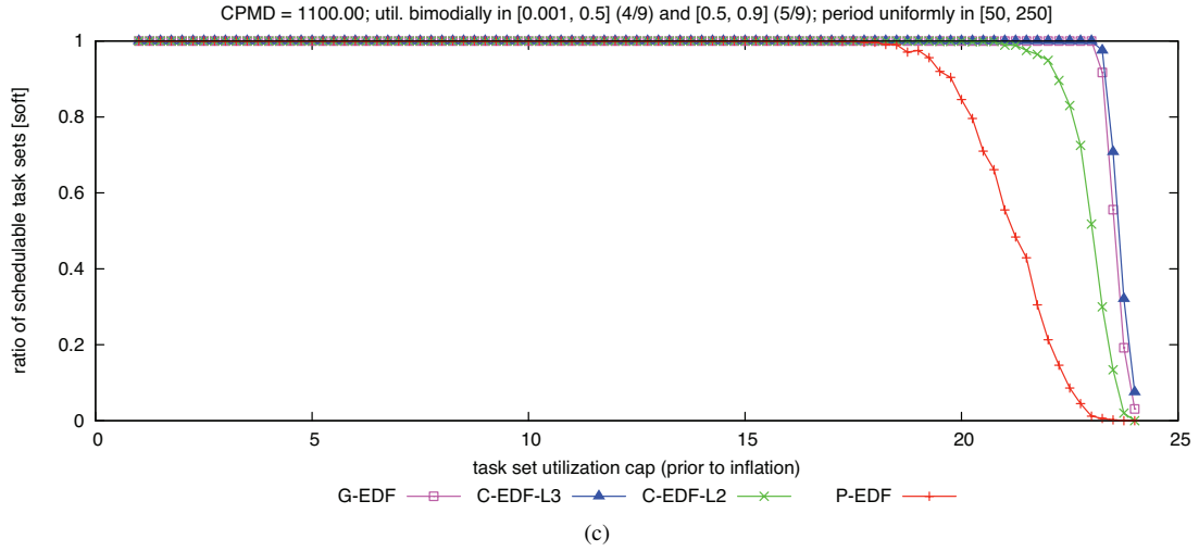
Figure 348: CPMD = 1100.00. Soft schedulability of task sets with bimodal heavy per-task utilizations and (a) short, (b) moderate, and (c) long periods.
