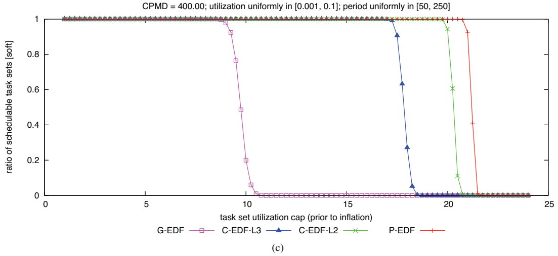
Figure 301: CPMD = 400.00. Soft schedulability of task sets with uniform light per-task utilizations and (a) short, (b) moderate, and (c) long periods.
