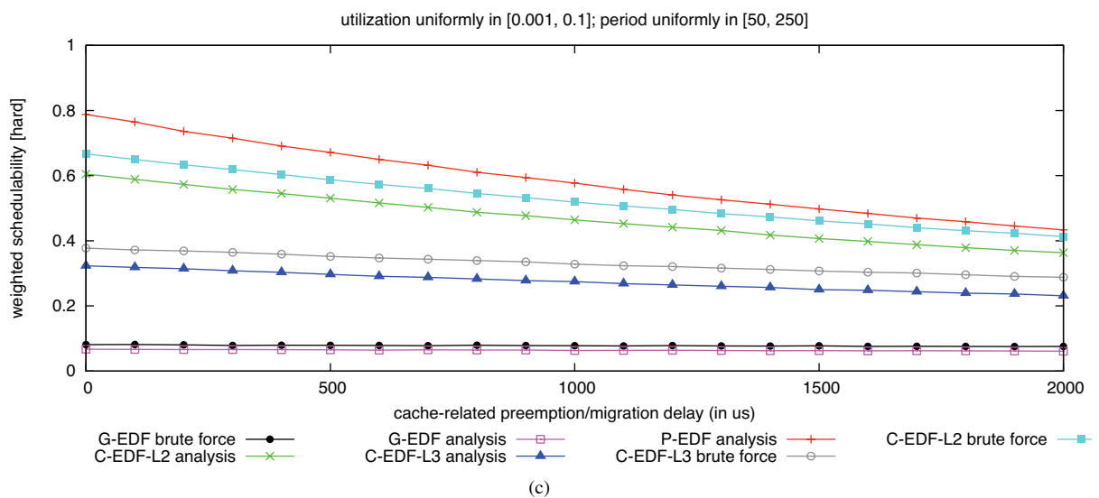
Figure 13: Hard weighted schedulability of task sets with uniform light per-task utilizations and (a) short, (b) moderate, and (c) long periods.
