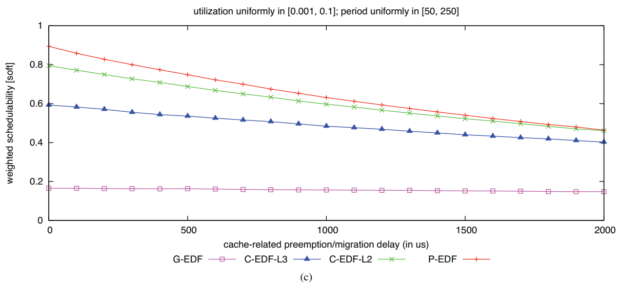
Figure 19: Soft weighted schedulability of task sets with uniform light per-task utilizations and (a) short, (b) moderate, and (c) long periods.
