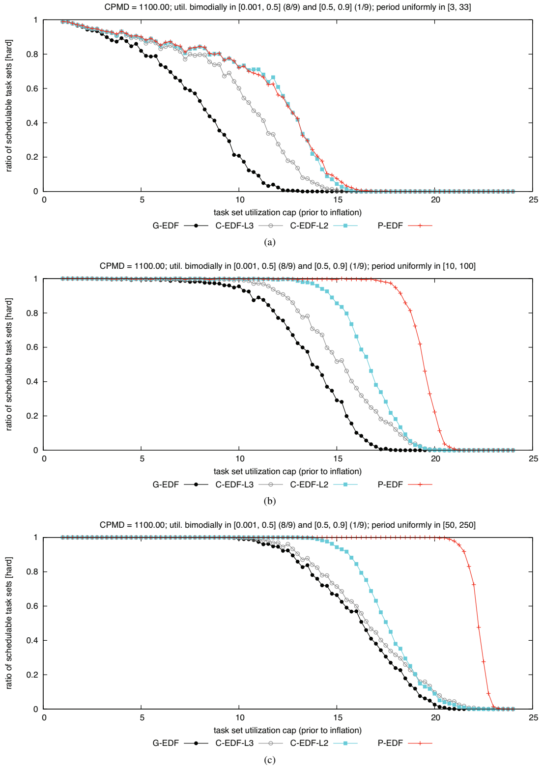
Figure 160: CPMD = 1100.00. Hard BF schedulability of task sets with bimodal light per-task utilizations and (a) short, (b) moderate, and (c) long periods.
