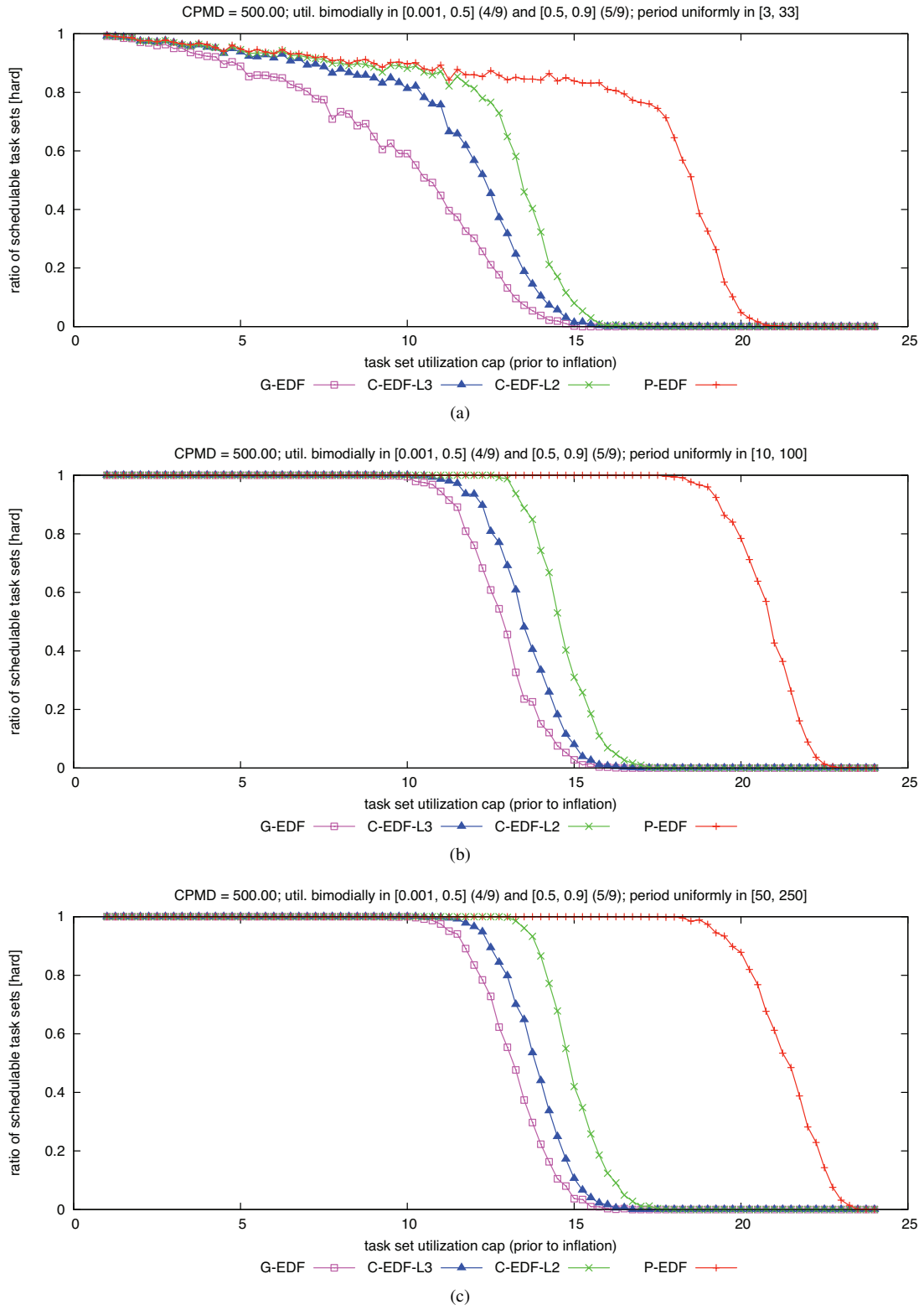
Figure 95: CPMD = 500.00. Hard W(D) schedulability of task sets with bimodal heavy per-task utilizations and (a) short, (b) moderate, and (c) long periods.
