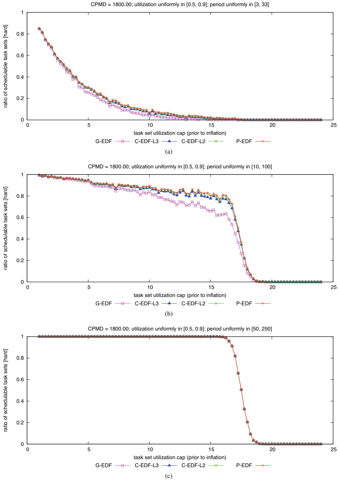
Figure 249: CPMD = 1800.00. Hard W(D) schedulability of task sets with uniform heavy per-task utilizations and (a) short, (b) moderate, and (c) long periods.
