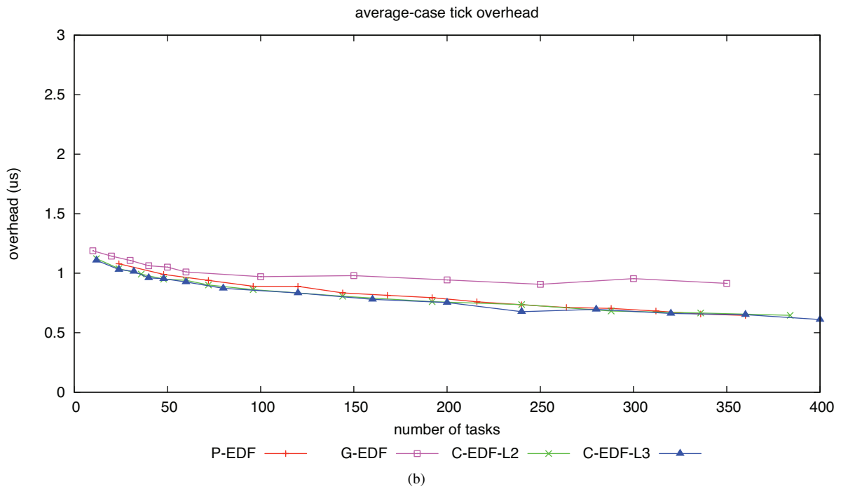
Figure 9: Measured tick overhead. (a) Measured worst case. (b) Measured average case.
