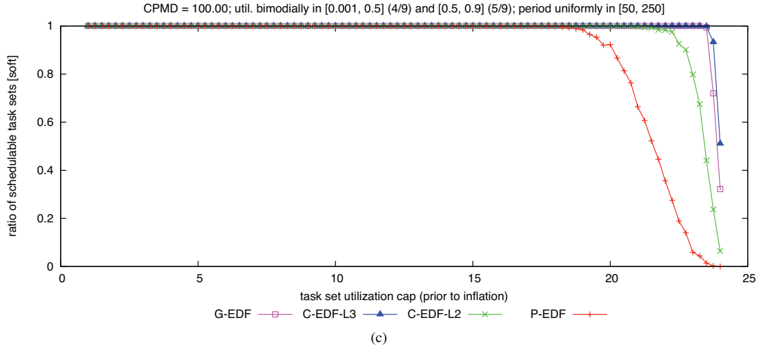
Figure 288: CPMD = 100.00. Soft schedulability of task sets with bimodal heavy per-task utilizations and (a) short, (b) moderate, and (c) long periods.
