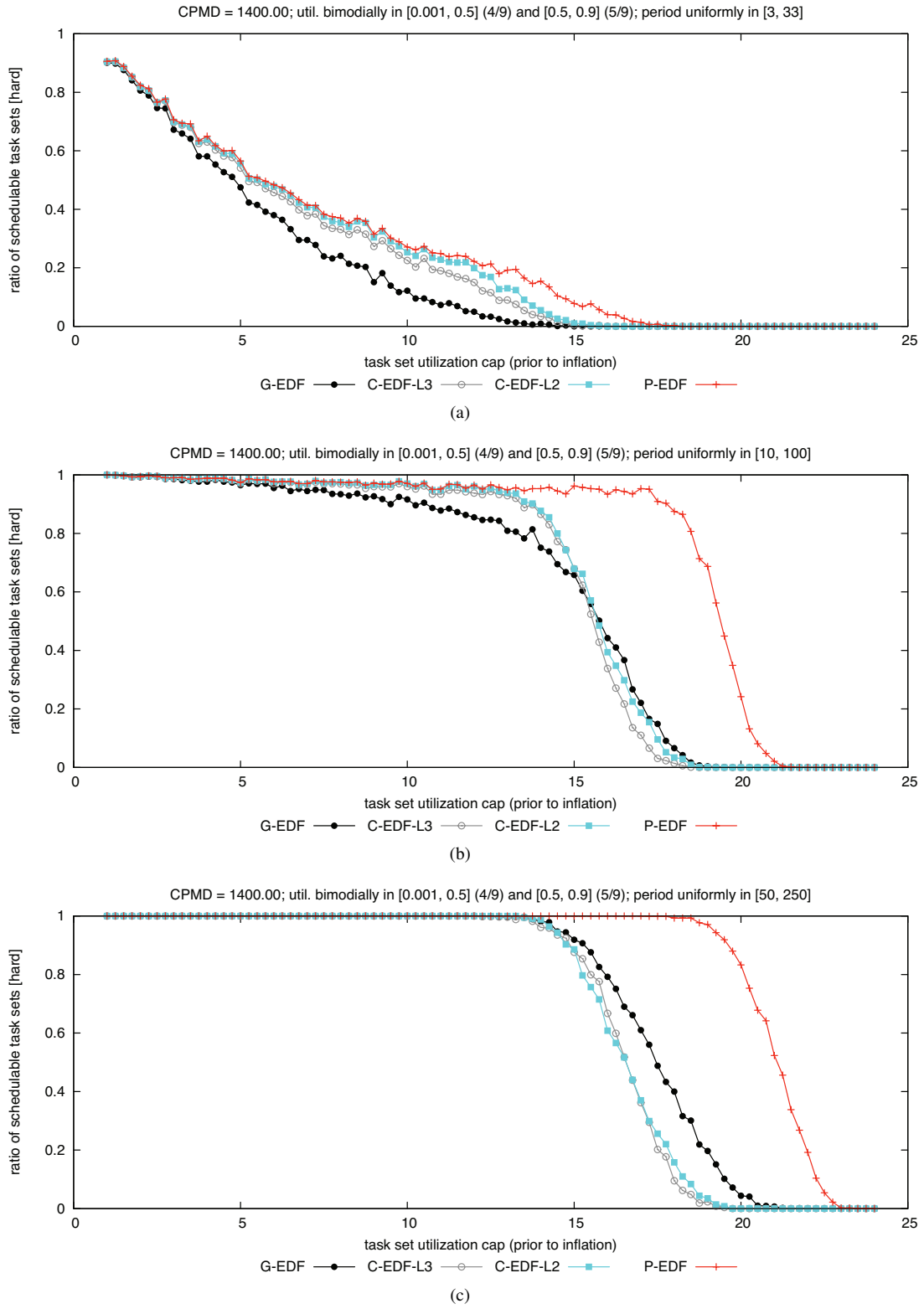
Figure 204: CPMD = 1400.00. Hard BF schedulability of task sets with bimodal heavy per-task utilizations and (a) short, (b) moderate, and (c) long periods.
