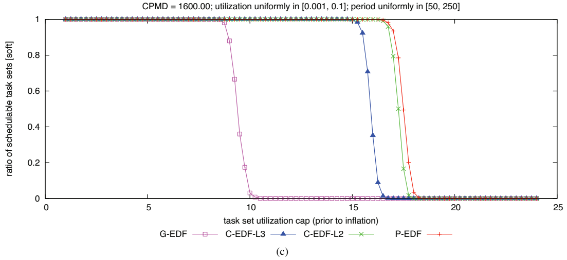
Figure 373: CPMD = 1600.00. Soft schedulability of task sets with uniform light per-task utilizations and (a) short, (b) moderate, and (c) long periods.
