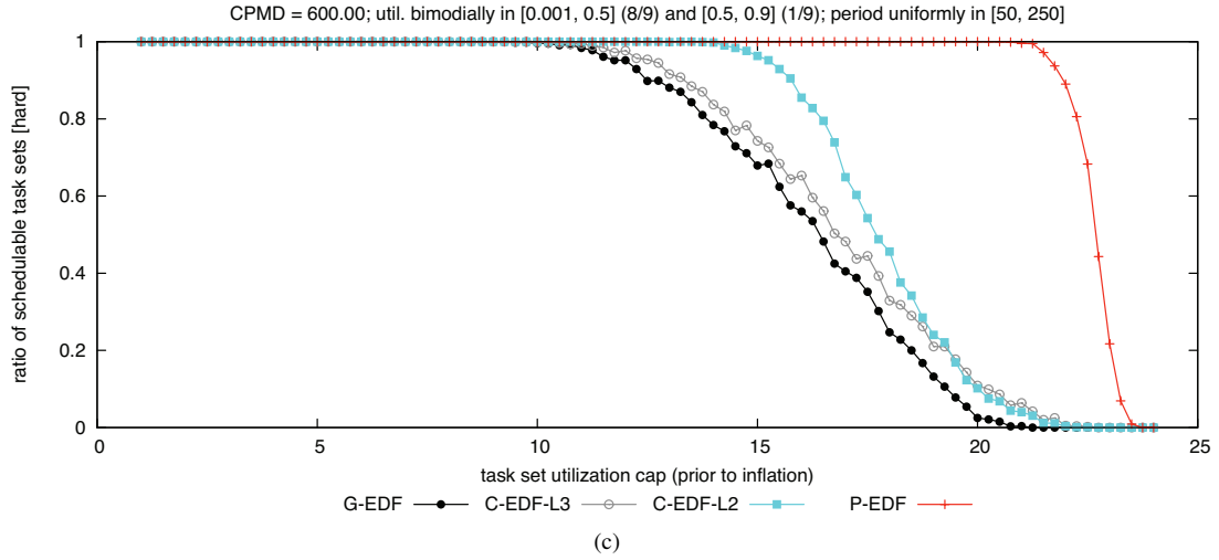
Figure 100: CPMD = 600.00. Hard BF schedulability of task sets with bimodal light per-task utilizations and (a) short, (b) moderate, and (c) long periods.
