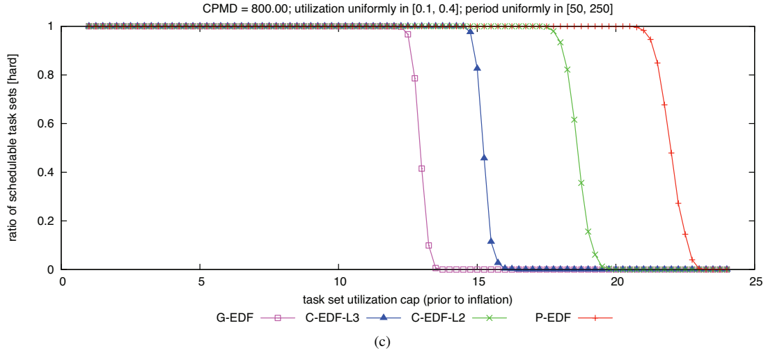
Figure 125: CPMD = 800.00. Hard W(D) schedulability of task sets with uniform medium per-task utilizations and (a) short, (b) moderate, and (c) long periods.
