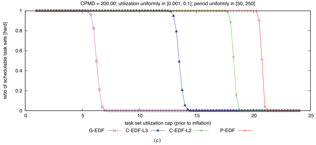
Figure 49: CPMD = 200.00. Hard W(D) schedulability of task sets with uniform light per-task utilizations and (a) short, (b) moderate, and (c) long periods.
