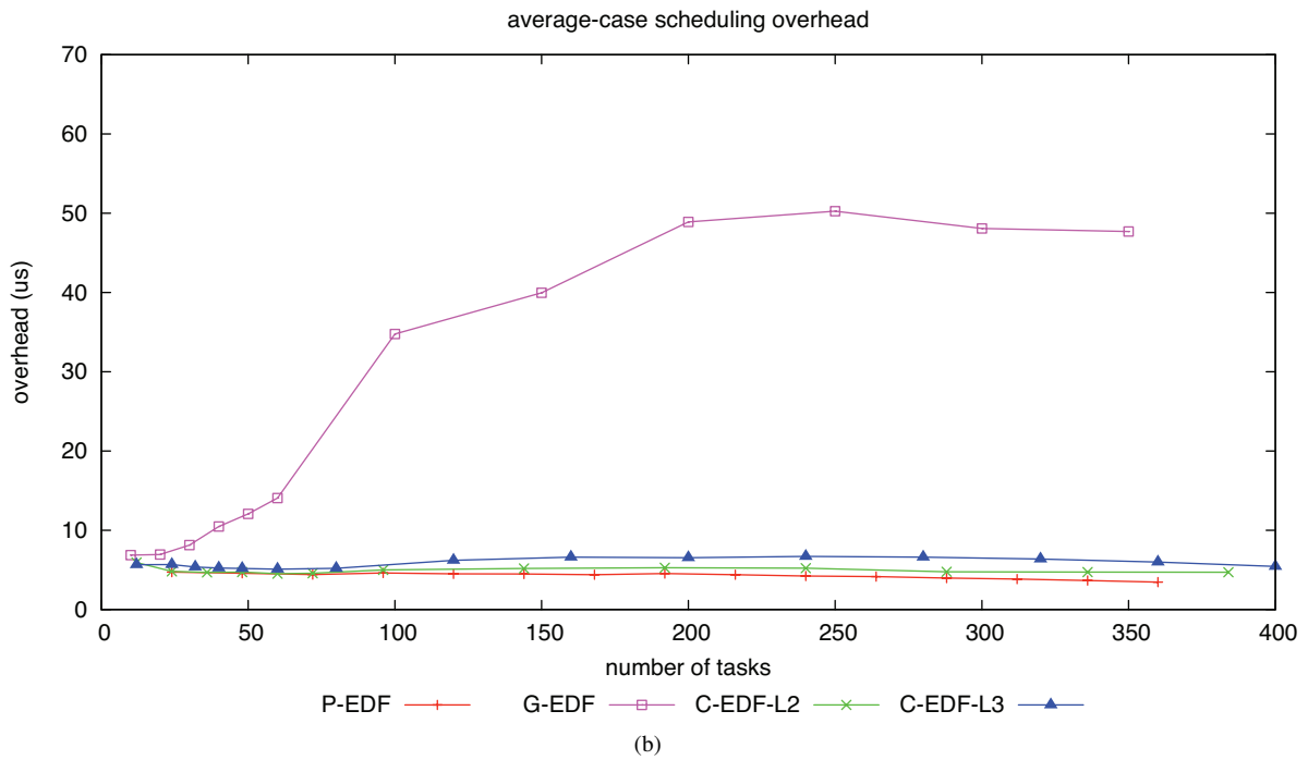
Figure 7: Measured scheduling overhead. (a) Measured worst case. (b) Measured average case.
