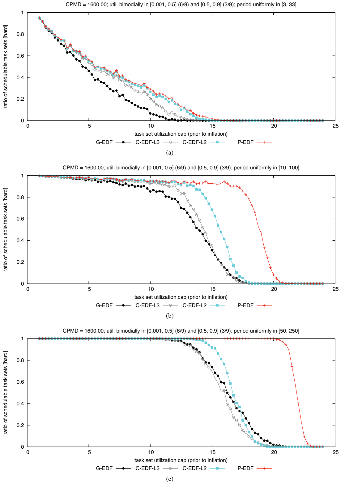
Figure 224: CPMD = 1600.00. Hard BF schedulability of task sets with bimodal medium per-task utilizations and (a) short, (b) moderate, and (c) long periods.
