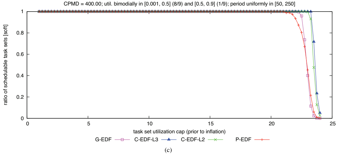
Figure 302: CPMD = 400.00. Soft schedulability of task sets with bimodal light per-task utilizations and (a) short, (b) moderate, and (c) long periods.
