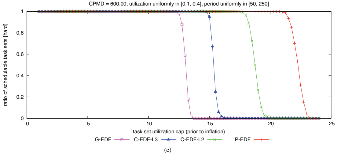
Figure 101: CPMD = 600.00. Hard W(D) schedulability of task sets with uniform medium per-task utilizations and (a) short, (b) moderate, and (c) long periods.
