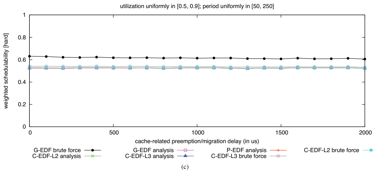
Figure 17: Hard weighted schedulability of task sets with uniform heavy per-task utilizations and (a) short, (b) moderate, and (c) long periods.
