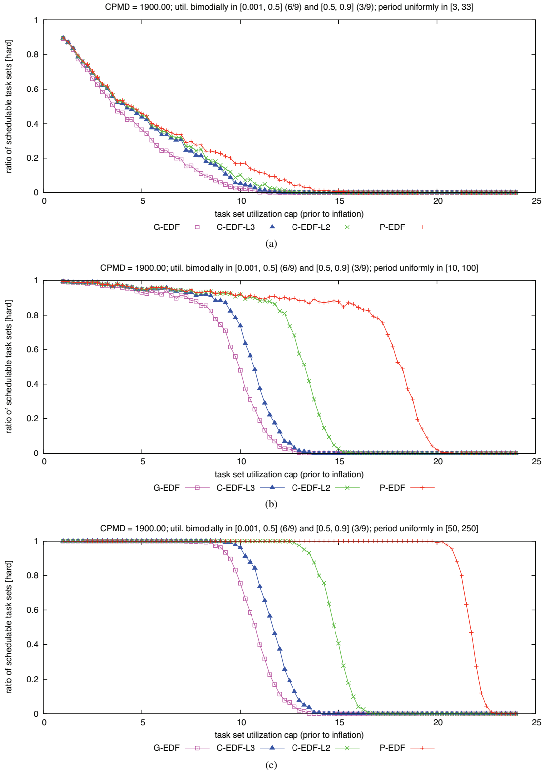
Figure 259: CPMD = 1900.00. Hard W(D) schedulability of task sets with bimodal medium per-task utilizations and (a) short, (b) moderate, and (c) long periods.
