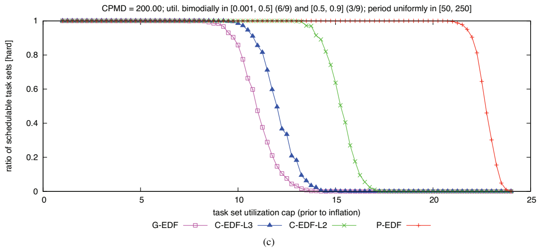
Figure 55: CPMD = 200.00. Hard W(D) schedulability of task sets with bimodal medium per-task utilizations and (a) short, (b) moderate, and (c) long periods.
