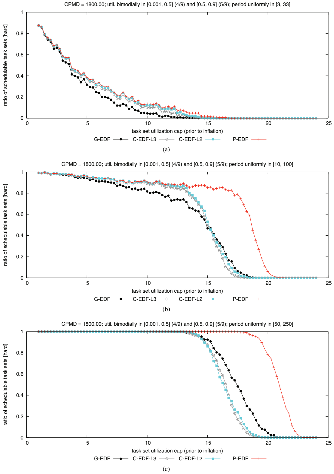
Figure 252: CPMD = 1800.00. Hard BF schedulability of task sets with bimodal heavy per-task utilizations and (a) short, (b) moderate, and (c) long periods.
