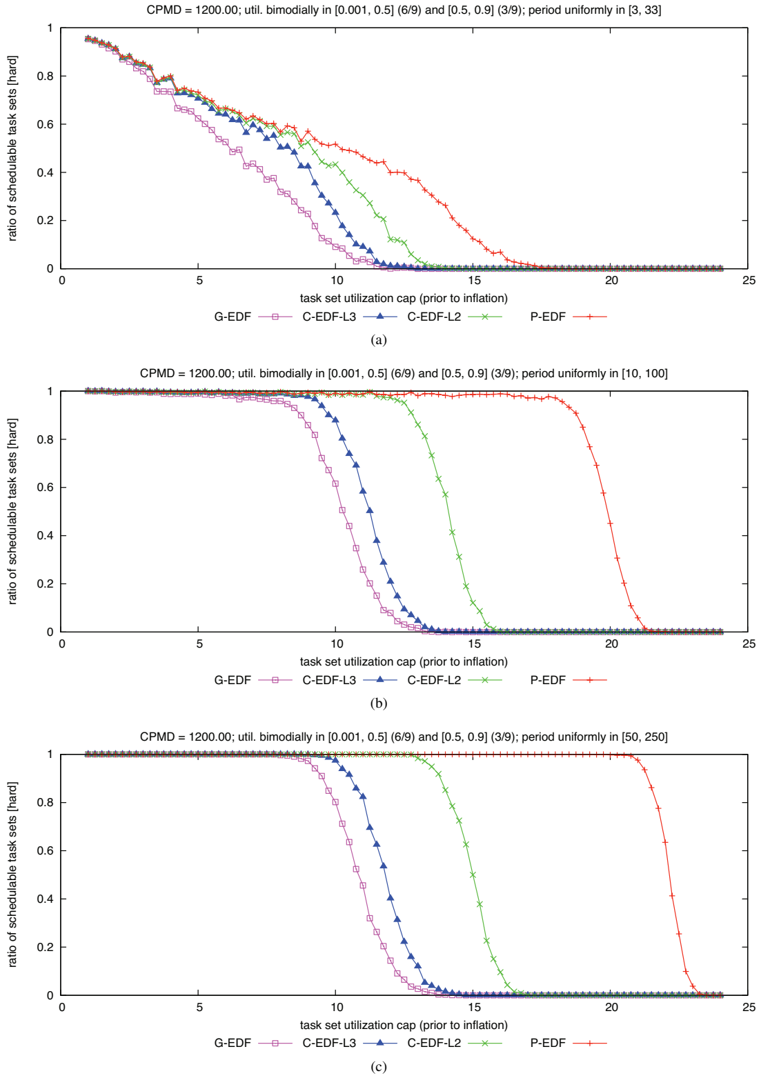
Figure 175: CPMD = 1200.00. Hard W(D) schedulability of task sets with bimodal medium per-task utilizations and (a) short, (b) moderate, and (c) long periods.
