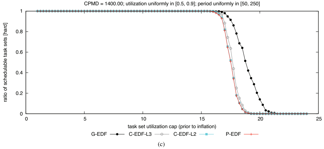
Figure 202: CPMD = 1400.00. Hard BF schedulability of task sets with uniform heavy per-task utilizations and (a) short, (b) moderate, and (c) long periods.
