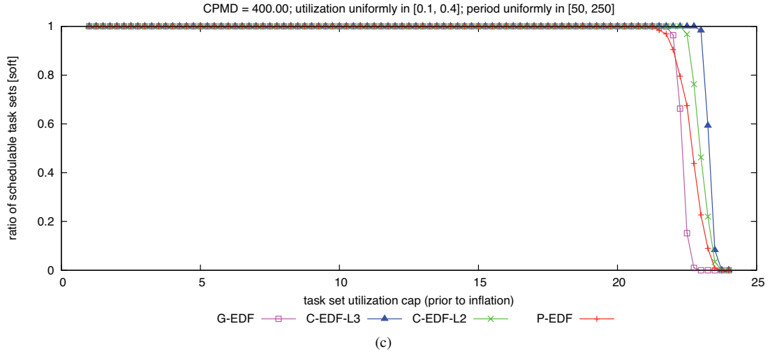
Figure 303: CPMD = 400.00. Soft schedulability of task sets with uniform medium per-task utilizations and (a) short, (b) moderate, and (c) long periods.
