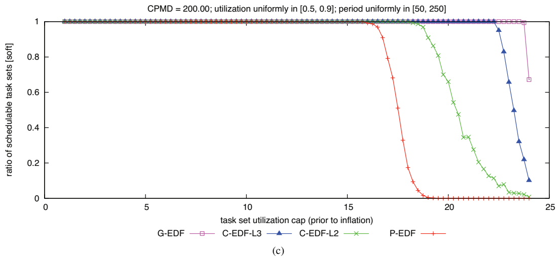
Figure 293: CPMD = 200.00. Soft schedulability of task sets with uniform heavy per-task utilizations and (a) short, (b) moderate, and (c) long periods.
