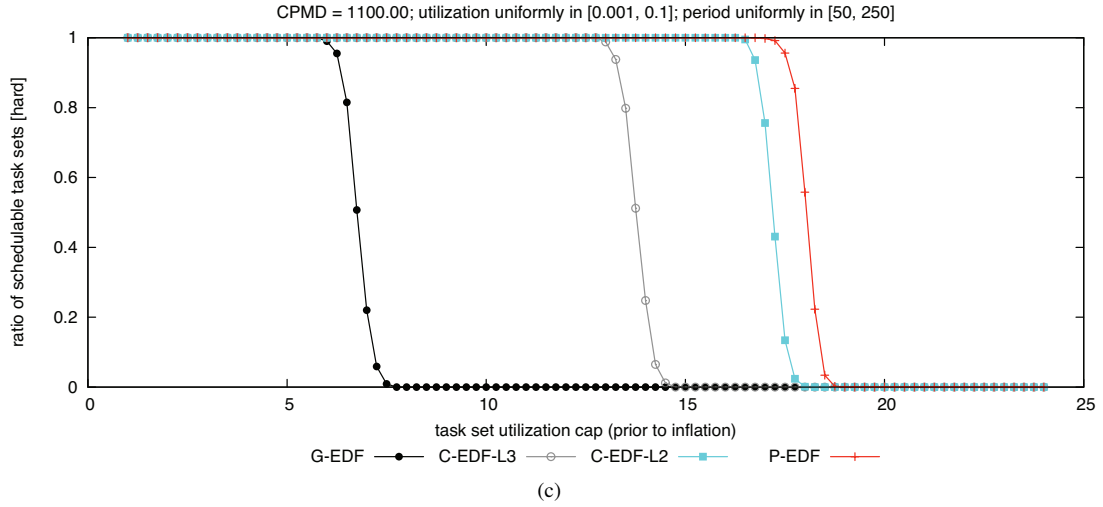
Figure 158: CPMD = 1100.00. Hard BF schedulability of task sets with uniform light per-task utilizations and (a) short, (b) moderate, and (c) long periods.
