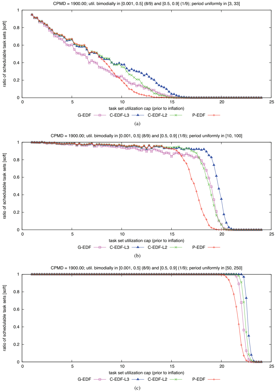
Figure 392: CPMD = 1900.00. Soft schedulability of task sets with bimodal light per-task utilizations and (a) short, (b) moderate, and (c) long periods.
