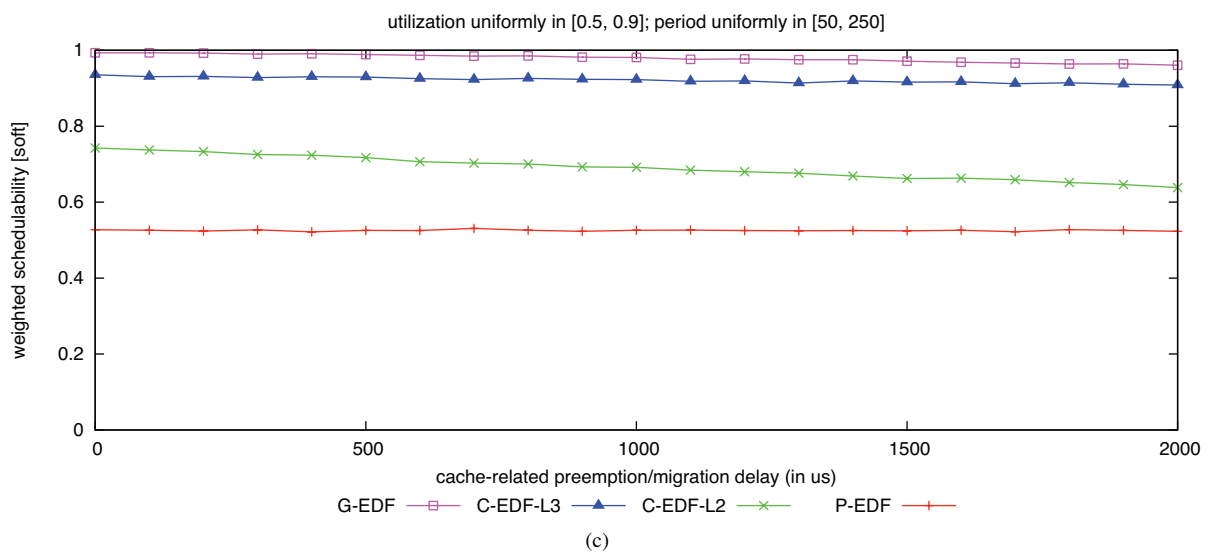
Figure 23: Soft weighted schedulability of task sets with uniform heavy per-task utilizations and (a) short, (b) moderate, and (c) long periods.
