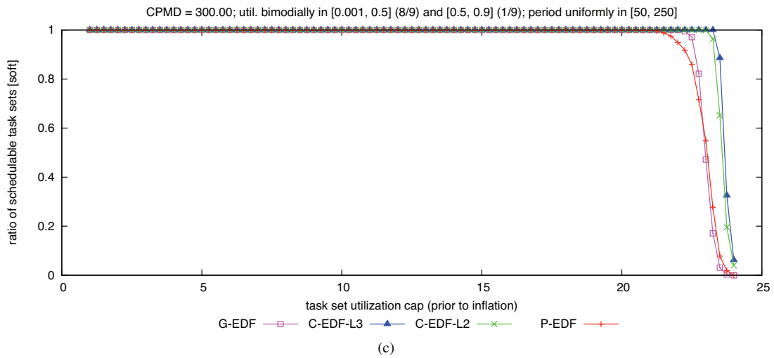
Figure 296: CPMD = 300.00. Soft schedulability of task sets with bimodal light per-task utilizations and (a) short, (b) moderate, and (c) long periods.
