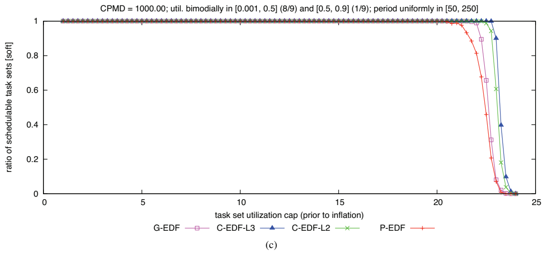
Figure 338: CPMD = 1000.00. Soft schedulability of task sets with bimodal light per-task utilizations and (a) short, (b) moderate, and (c) long periods.
