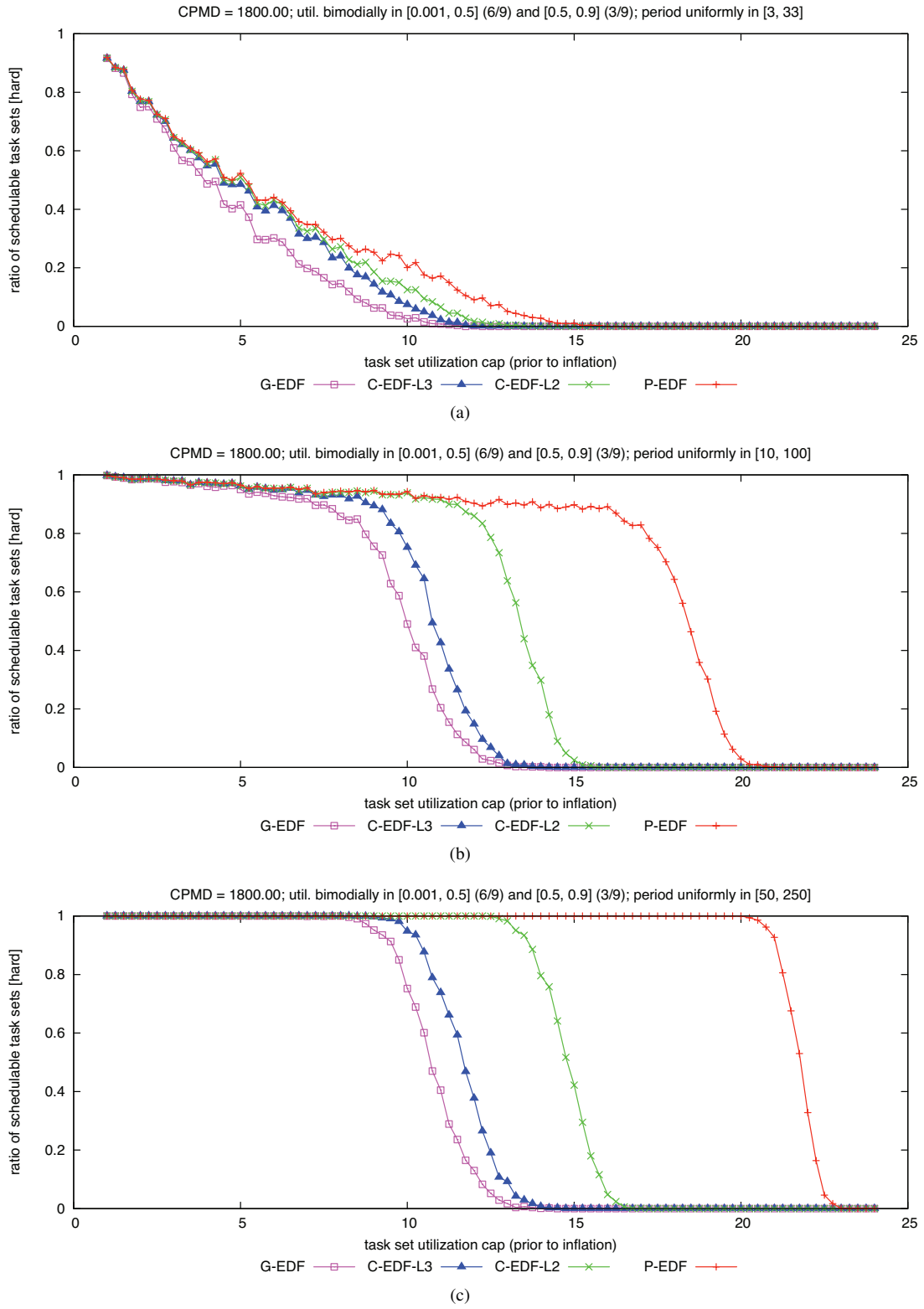
Figure 247: CPMD = 1800.00. Hard W(D) schedulability of task sets with bimodal medium per-task utilizations and (a) short, (b) moderate, and (c) long periods.
