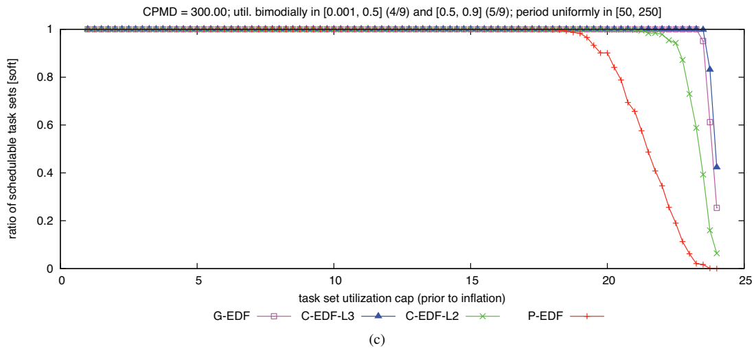
Figure 300: CPMD = 300.00. Soft schedulability of task sets with bimodal heavy per-task utilizations and (a) short, (b) moderate, and (c) long periods.
