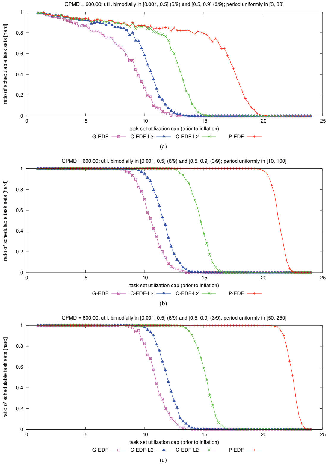
Figure 103: CPMD = 600.00. Hard W(D) schedulability of task sets with bimodal medium per-task utilizations and (a) short, (b) moderate, and (c) long periods.
