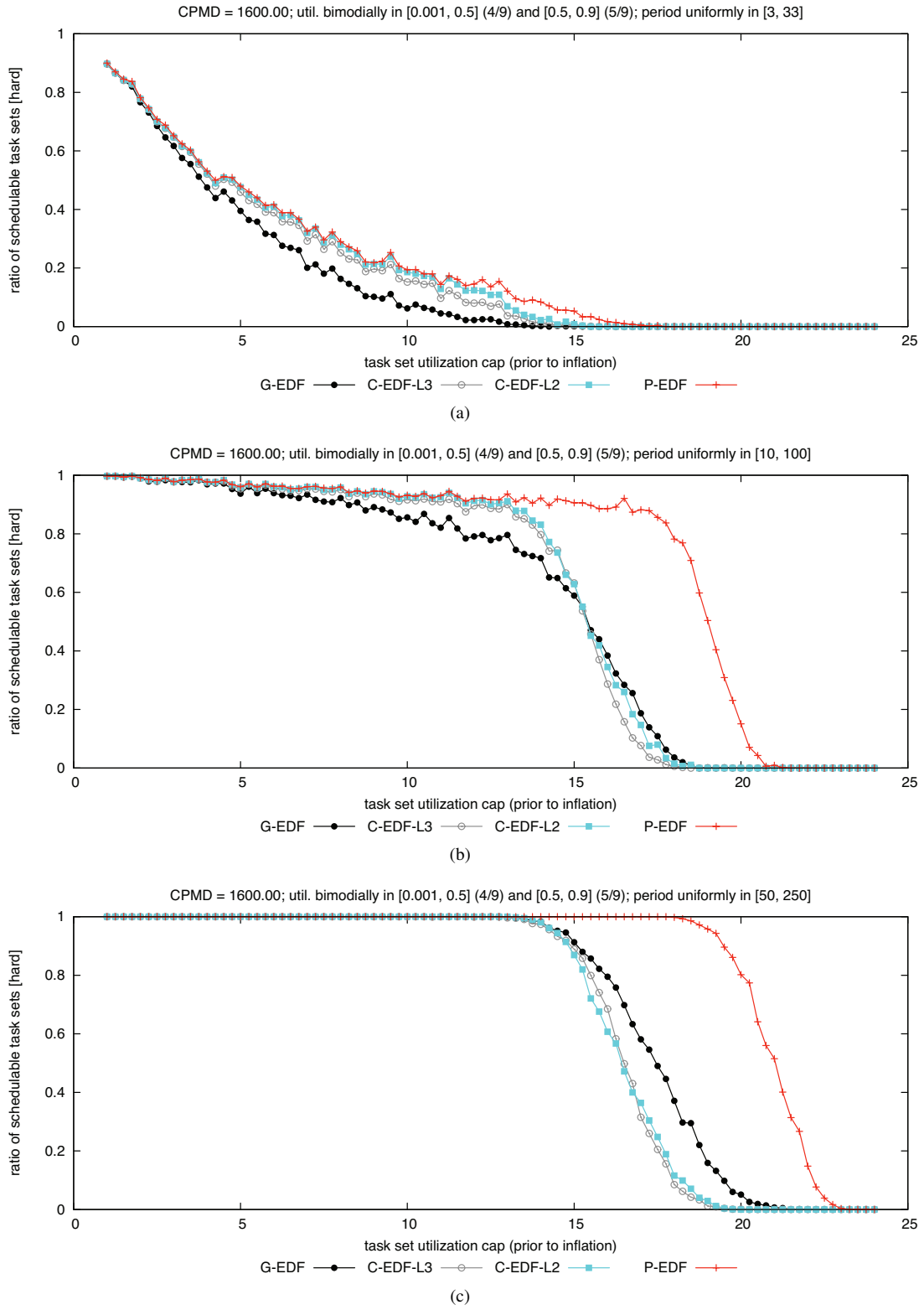
Figure 228: CPMD = 1600.00. Hard BF schedulability of task sets with bimodal heavy per-task utilizations and (a) short, (b) moderate, and (c) long periods.
