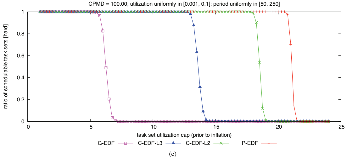
Figure 37: CPMD = 100.00. Hard W(D) schedulability of task sets with uniform light per-task utilizations and (a) short, (b) moderate, and (c) long periods.
