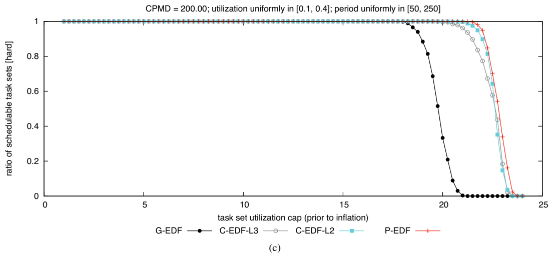
Figure 54: CPMD = 200.00. Hard BF schedulability of task sets with uniform medium per-task utilizations and (a) short, (b) moderate, and (c) long periods.
