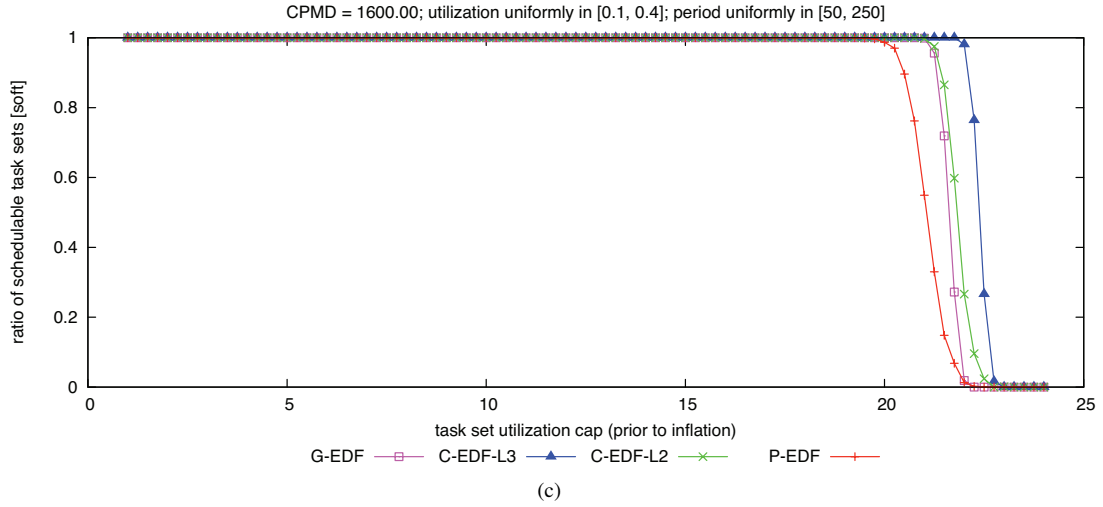
Figure 375: CPMD = 1600.00. Soft schedulability of task sets with uniform medium per-task utilizations and (a) short, (b) moderate, and (c) long periods.
