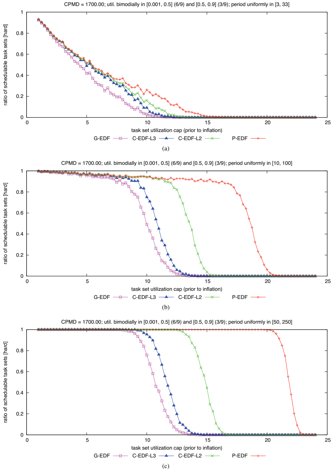
Figure 235: CPMD = 1700.00. Hard W(D) schedulability of task sets with bimodal medium per-task utilizations and (a) short, (b) moderate, and (c) long periods.
