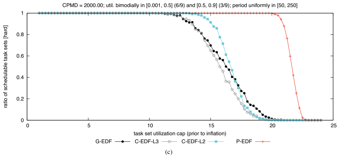
Figure 272: CPMD = 2000.00. Hard BF schedulability of task sets with bimodal medium per-task utilizations and (a) short, (b) moderate, and (c) long periods.
