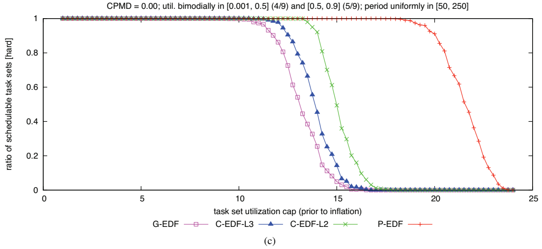
Figure 35: CPMD = 0.00. Hard W(D) schedulability of task sets with bimodal heavy per-task utilizations and (a) short, (b) moderate, and (c) long periods.
