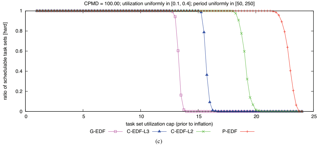
Figure 41: CPMD = 100.00. Hard W(D) schedulability of task sets with uniform medium per-task utilizations and (a) short, (b) moderate, and (c) long periods.
