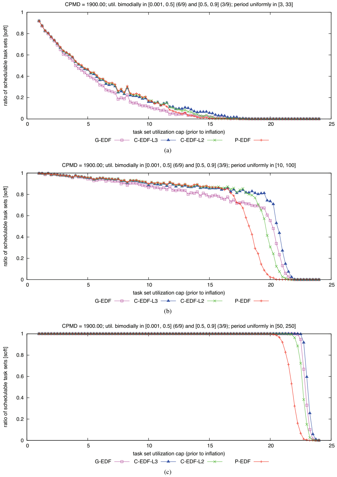
Figure 394: CPMD = 1900.00. Soft schedulability of task sets with bimodal medium per-task utilizations and (a) short, (b) moderate, and (c) long periods.
