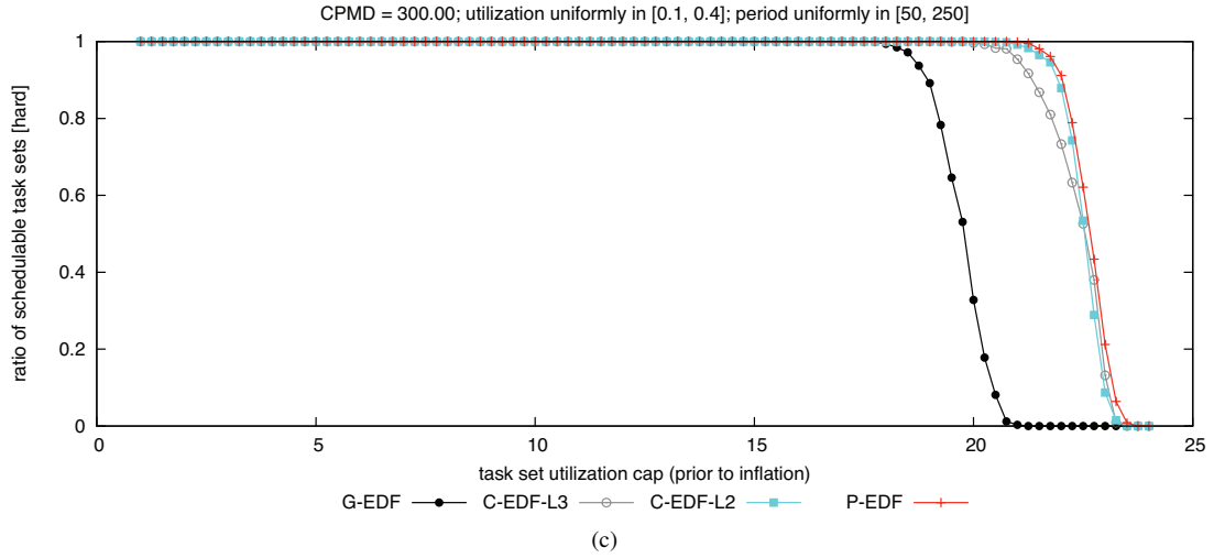
Figure 66: CPMD = 300.00. Hard BF schedulability of task sets with uniform medium per-task utilizations and (a) short, (b) moderate, and (c) long periods.
