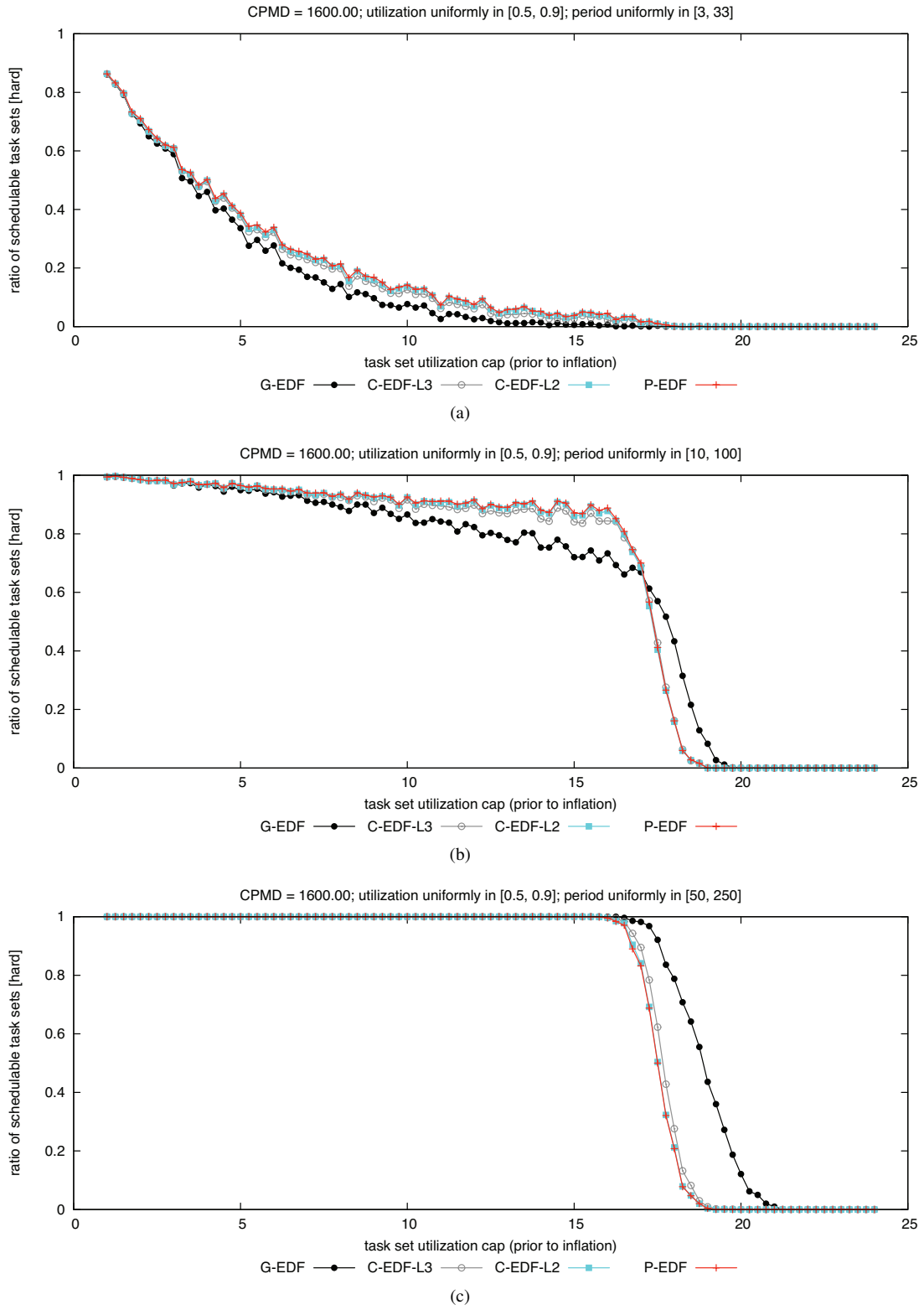
Figure 226: CPMD = 1600.00. Hard BF schedulability of task sets with uniform heavy per-task utilizations and (a) short, (b) moderate, and (c) long periods.
