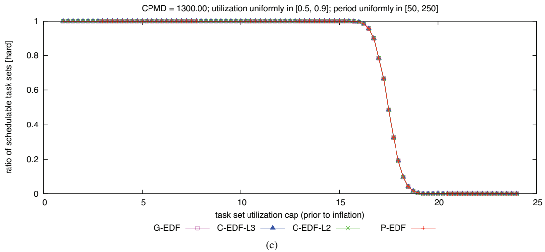
Figure 189: CPMD = 1300.00. Hard W(D) schedulability of task sets with uniform heavy per-task utilizations and (a) short, (b) moderate, and (c) long periods.
