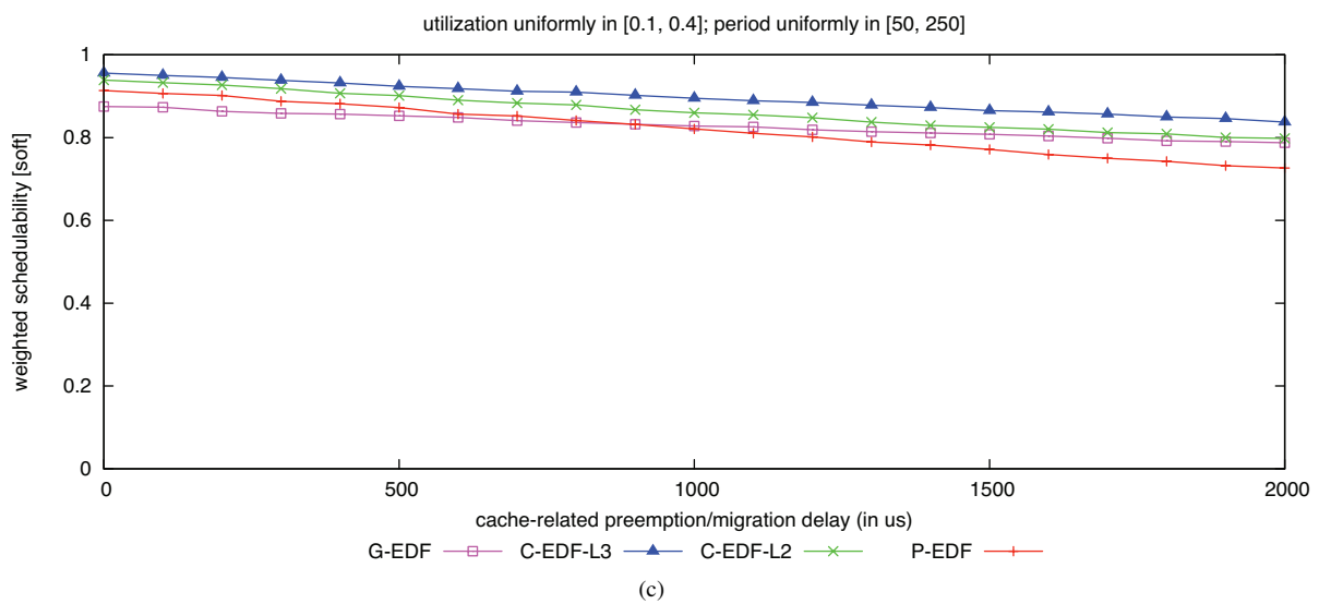
Figure 21: Soft weighted schedulability of task sets with uniform medium per-task utilizations and (a) short, (b) moderate, and (c) long periods.
