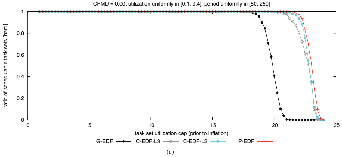
Figure 30: CPMD = 0.00. Hard BF schedulability of task sets with uniform medium per-task utilizations and (a) short, (b) moderate, and (c) long periods.
