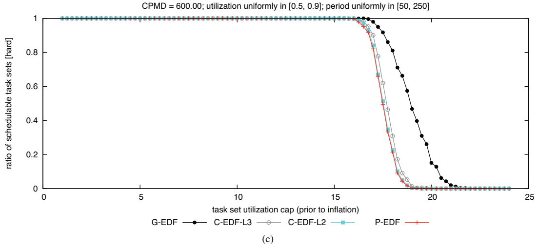
Figure 106: CPMD = 600.00. Hard BF schedulability of task sets with uniform heavy per-task utilizations and (a) short, (b) moderate, and (c) long periods.
