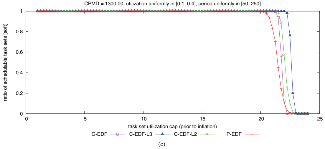
Figure 357: CPMD = 1300.00. Soft schedulability of task sets with uniform medium per-task utilizations and (a) short, (b) moderate, and (c) long periods.
