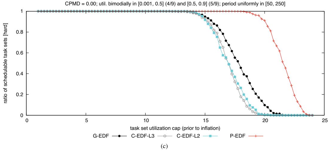
Figure 36: CPMD = 0.00. Hard BF schedulability of task sets with bimodal heavy per-task utilizations and (a) short, (b) moderate, and (c) long periods.
