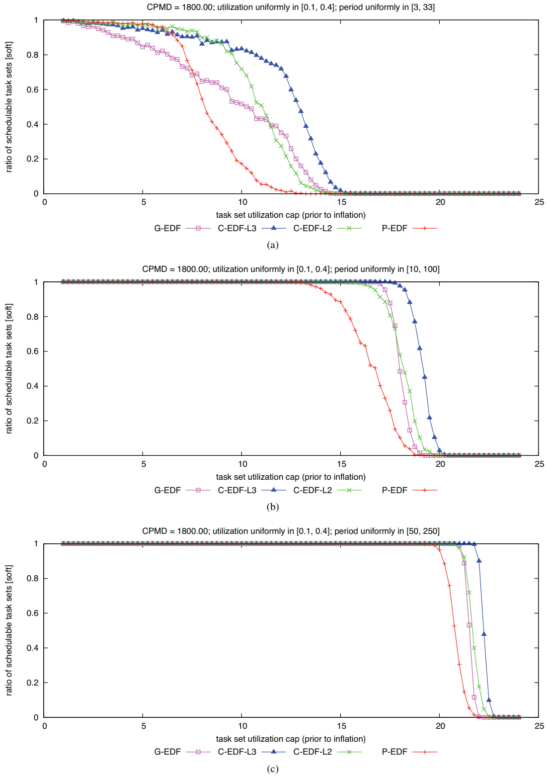
Figure 387: CPMD = 1800.00. Soft schedulability of task sets with uniform medium per-task utilizations and (a) short, (b) moderate, and (c) long periods.
