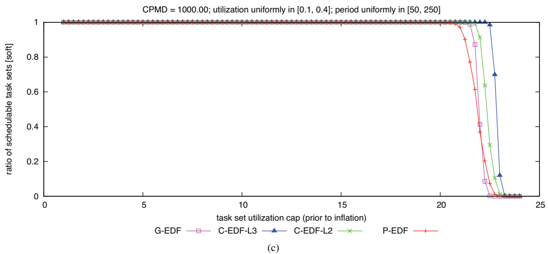
Figure 339: CPMD = 1000.00. Soft schedulability of task sets with uniform medium per-task utilizations and (a) short, (b) moderate, and (c) long periods.
