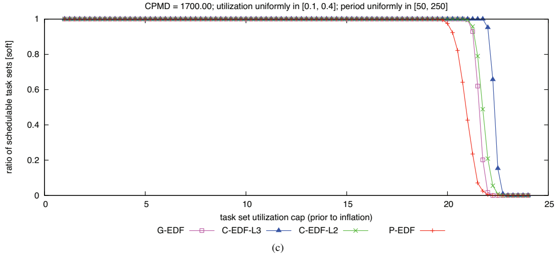
Figure 381: CPMD = 1700.00. Soft schedulability of task sets with uniform medium per-task utilizations and (a) short, (b) moderate, and (c) long periods.
