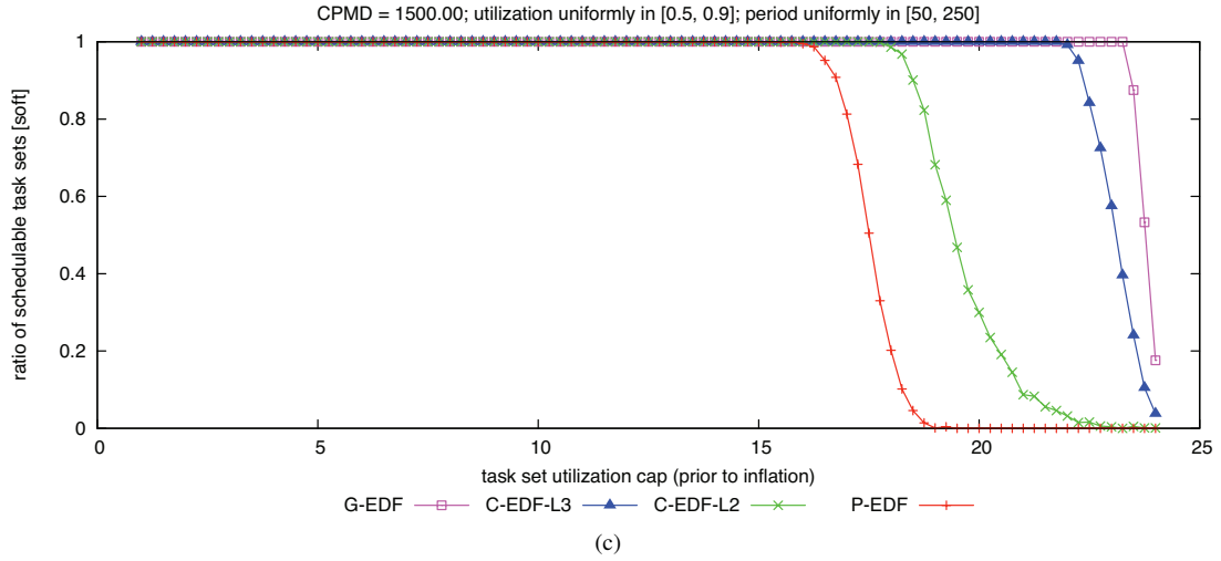
Figure 371: CPMD = 1500.00. Soft schedulability of task sets with uniform heavy per-task utilizations and (a) short, (b) moderate, and (c) long periods.
