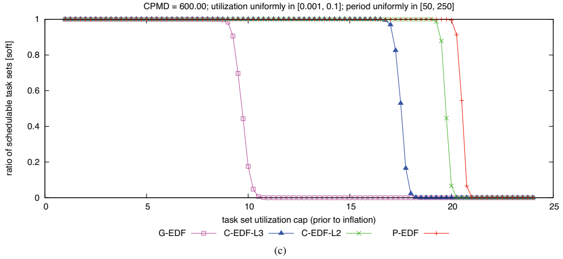
Figure 313: CPMD = 600.00. Soft schedulability of task sets with uniform light per-task utilizations and (a) short, (b) moderate, and (c) long periods.
