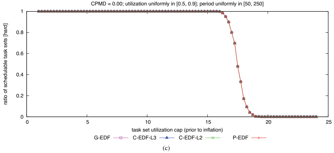
Figure 33: CPMD = 0.00. Hard W(D) schedulability of task sets with uniform heavy per-task utilizations and (a) short, (b) moderate, and (c) long periods.
