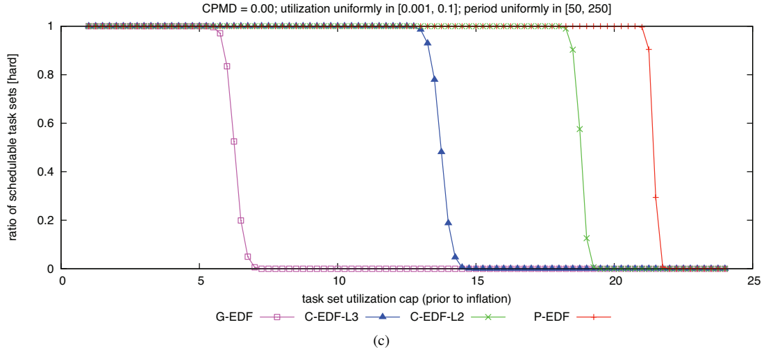
Figure 25: CPMD = 0.00. Hard W(D) schedulability of task sets with uniform light per-task utilizations and (a) short, (b) moderate, and (c) long periods.
