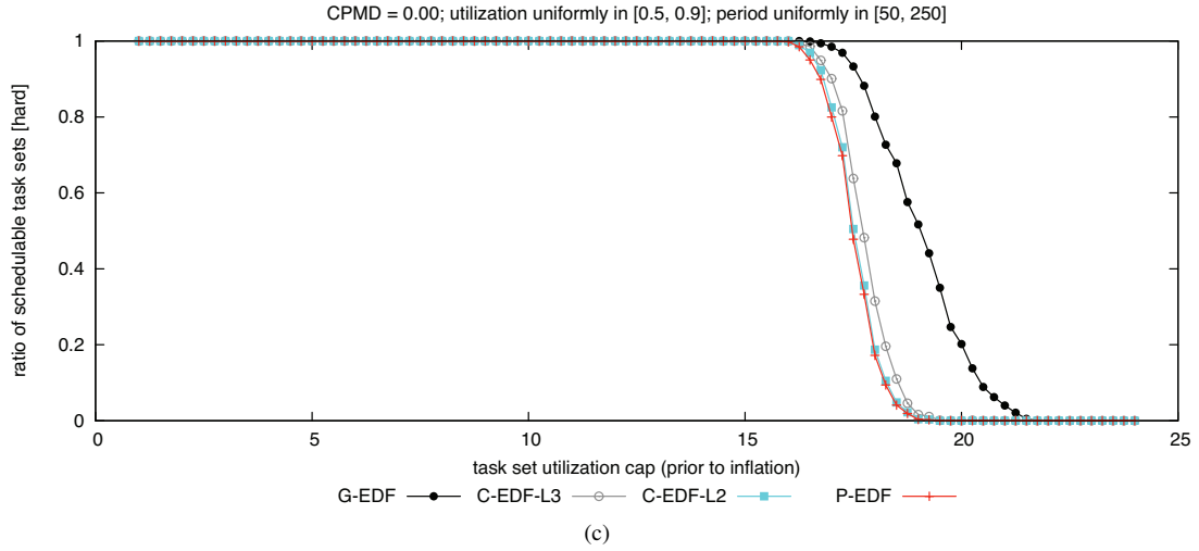
Figure 34: CPMD = 0.00. Hard BF schedulability of task sets with uniform heavy per-task utilizations and (a) short, (b) moderate, and (c) long periods.
