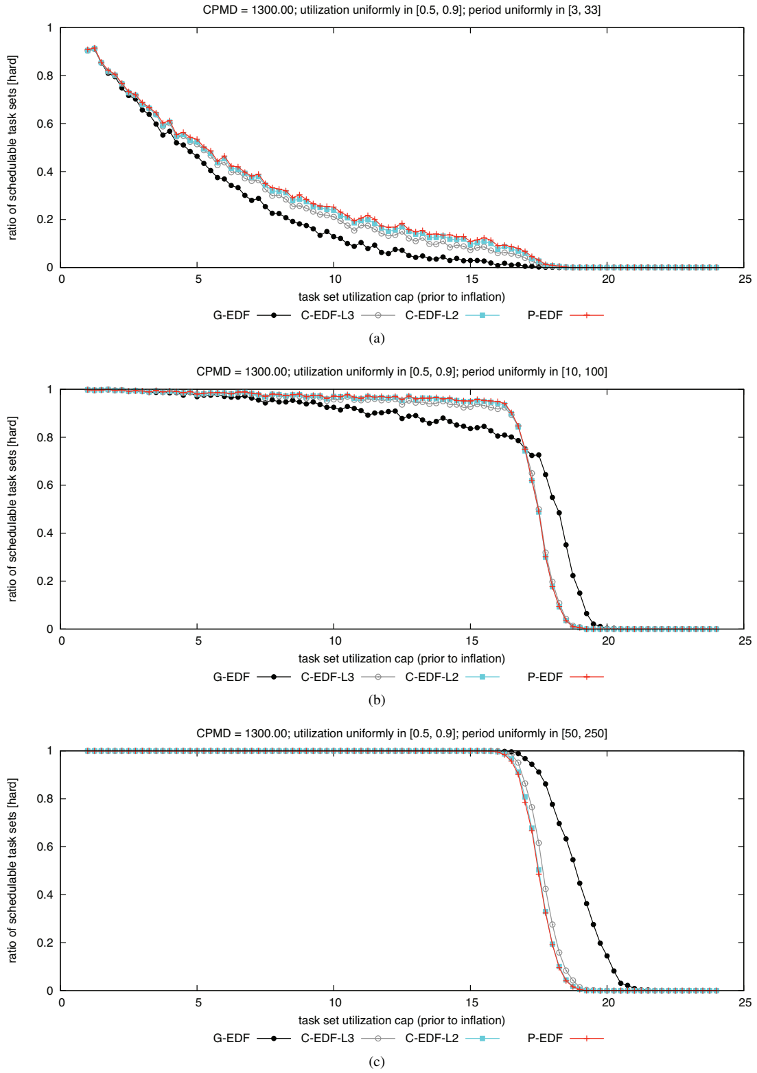
Figure 190: CPMD = 1300.00. Hard BF schedulability of task sets with uniform heavy per-task utilizations and (a) short, (b) moderate, and (c) long periods.
