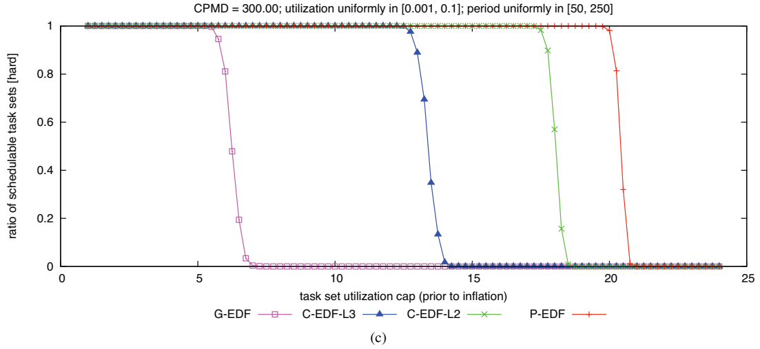
Figure 61: CPMD = 300.00. Hard W(D) schedulability of task sets with uniform light per-task utilizations and (a) short, (b) moderate, and (c) long periods.
