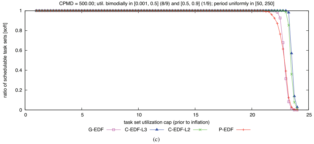
Figure 308: CPMD = 500.00. Soft schedulability of task sets with bimodal light per-task utilizations and (a) short, (b) moderate, and (c) long periods.
