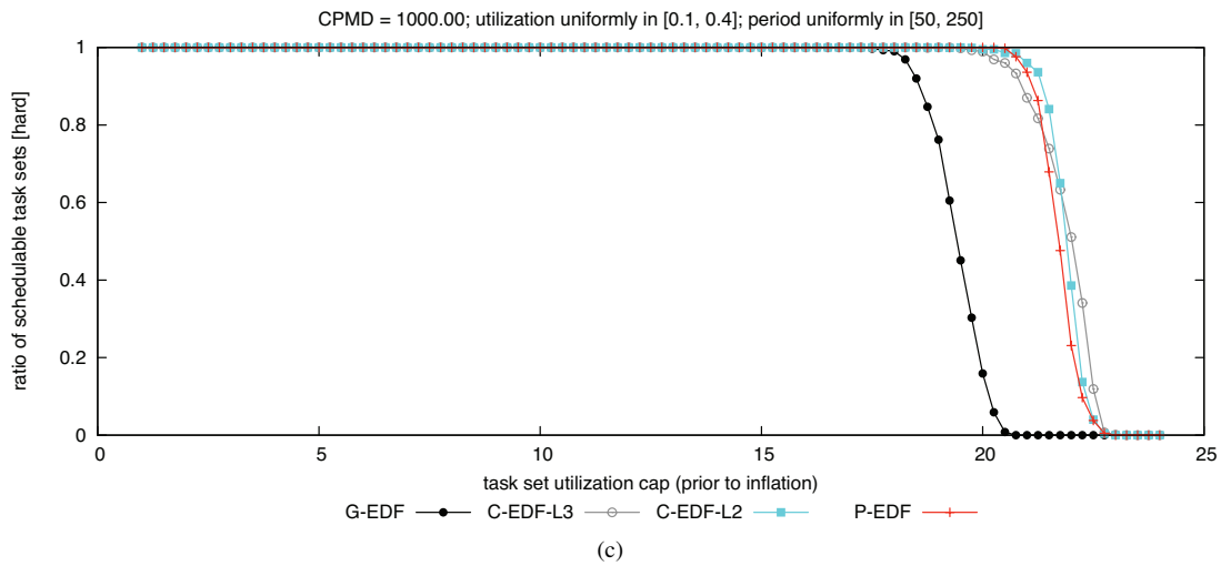
Figure 150: CPMD = 1000.00. Hard BF schedulability of task sets with uniform medium per-task utilizations and (a) short, (b) moderate, and (c) long periods.
