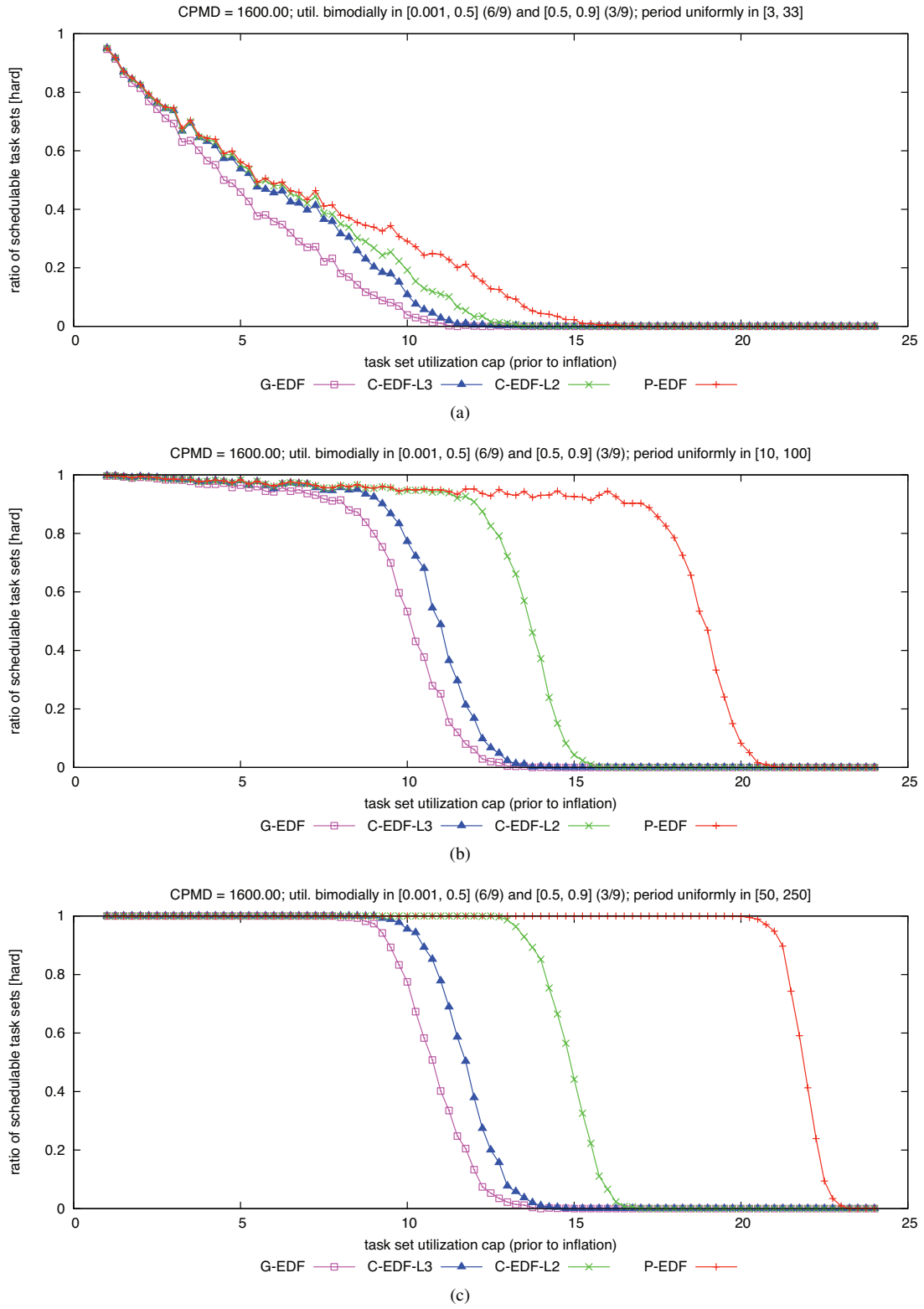
Figure 223: CPMD = 1600.00. Hard W(D) schedulability of task sets with bimodal medium per-task utilizations and (a) short, (b) moderate, and (c) long periods.
