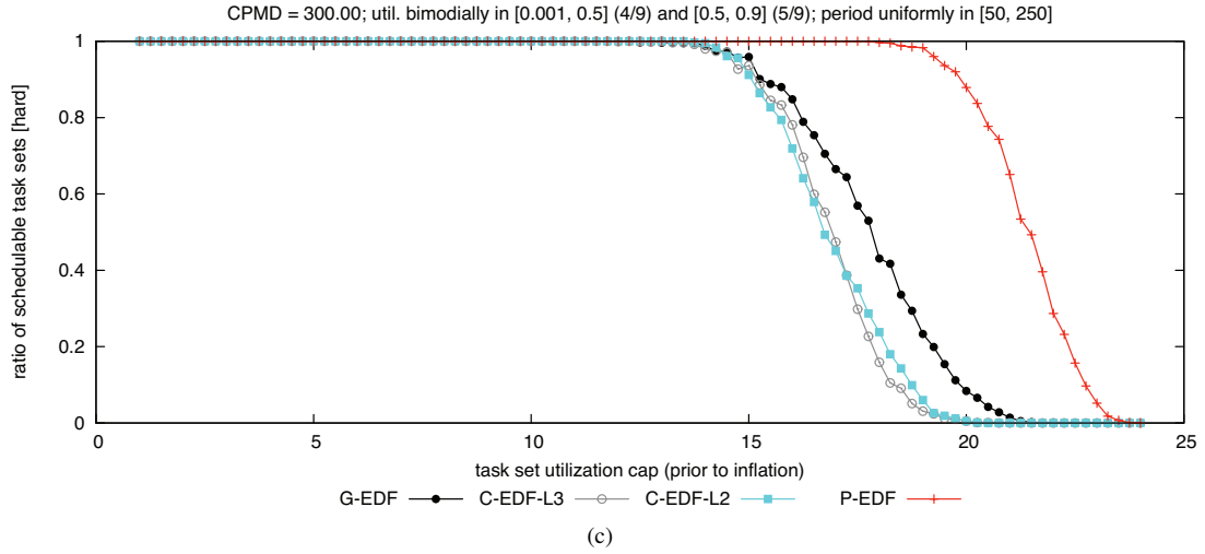
Figure 72: CPMD = 300.00. Hard BF schedulability of task sets with bimodal heavy per-task utilizations and (a) short, (b) moderate, and (c) long periods.
