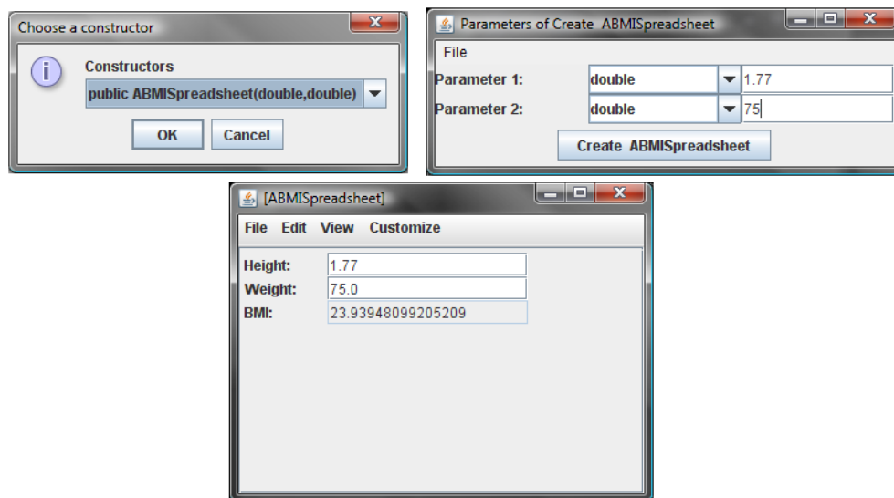
Figure 26. Creating an instance of ABMISpreadsheet using a constructor with parameters
