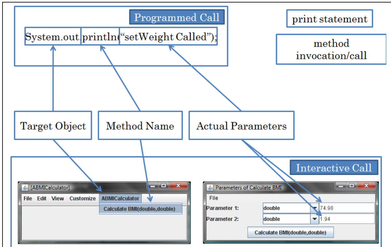
Figure 11. Programmed vs. interactive call
