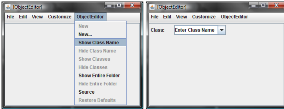
Figure 18. State-full ObjectEditor
