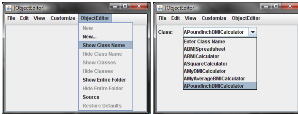
Figure 21. ObjectEditor Show Class Names command reads names of classes from folder form which ObjectEditor is executed
