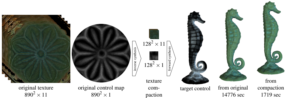
Figure 31: Inverse texture synthesis [WHZ*08]. Given a large globally-varying texture with an auxiliary control map (patina sequence from [LGG*07] in this case), the algorithm automatically computes a small texture compaction that best summarizes the original, including both texture and control. This small texture compaction can be used to reconstruct the original texture from its original control map, or to re-synthesize a new texture under a user-supplied control map. Due to the reduced data size, re-synthesis from our compaction is much faster than from the original without compromising image quality (right two images). In this example we use [KEBK05] for forward synthesis, but other algorithms can also be used since our compactions are just ordinary images.
