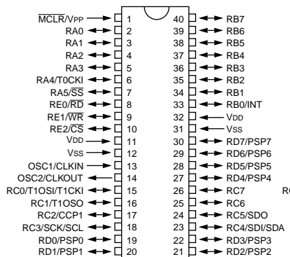
PIC16C64
