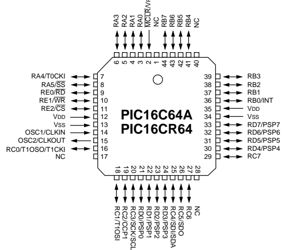
PLCC
