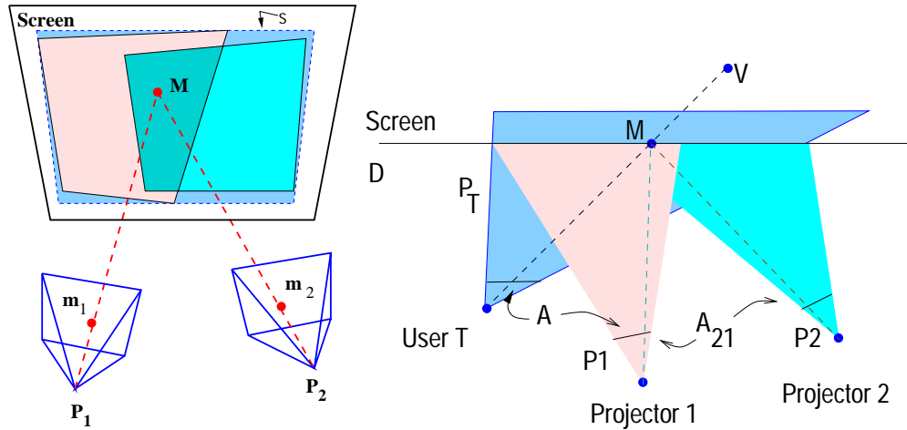
Figure 4.14: Collineation between overlapping projectors on planar display surface.
