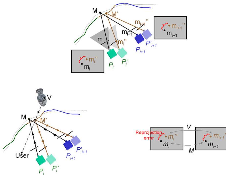
Figure 4.7: (a) Reprojection error, shown in red, for two overlapping projectors. (b) A virtual point for which the image is computed to be projected at M . (c) The physical correspondence due to M and computational correspondence due to virtual point V . The goal of post-rendering warp is to exploit the two known correspondences to achieve geometric registration.
