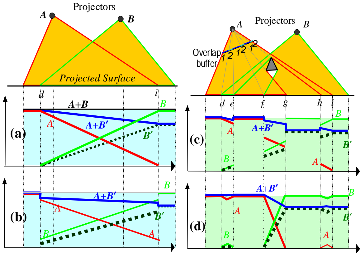
Figure 5.9: Intensity weights using feathering methods. The plots show the contribution of projectors A , B and B' and the resultant accumulation A+B and A+B' along the lit planar surface. Our technique, shown in (d), creates smooth weight transitions. (a) Simple intensity ramps on planar overlap create smooth transitions. (b) Weights computed using surface normals are not sufficient. (c) Occluders create sharp transitions (d) Our solution, which considers depth continuity, maintains the local smoothness of intensity weights.
