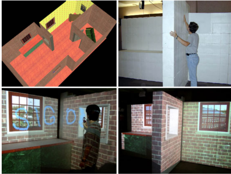
Figure 5.2: Spatially augmenting large environment (Kok-lim Low et al, 2001). (Top left) Virtual model; (Top right) Physical display environment constructed using Styrofoam blocks; (Bottom row) Augmented display. Note the view dependent nature of the display, the perspective correct view through the hole in the wall and the windows.
