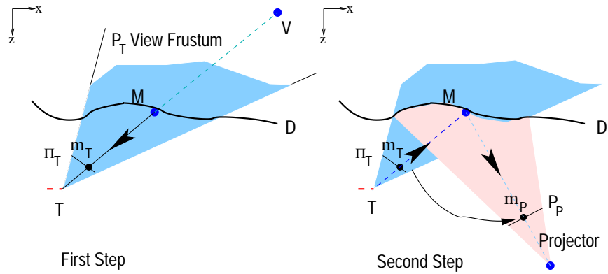
Figure 3.5: The Rendering Framework. The two rendering steps corresponding to the display configuration shown in 3.2 (left).
