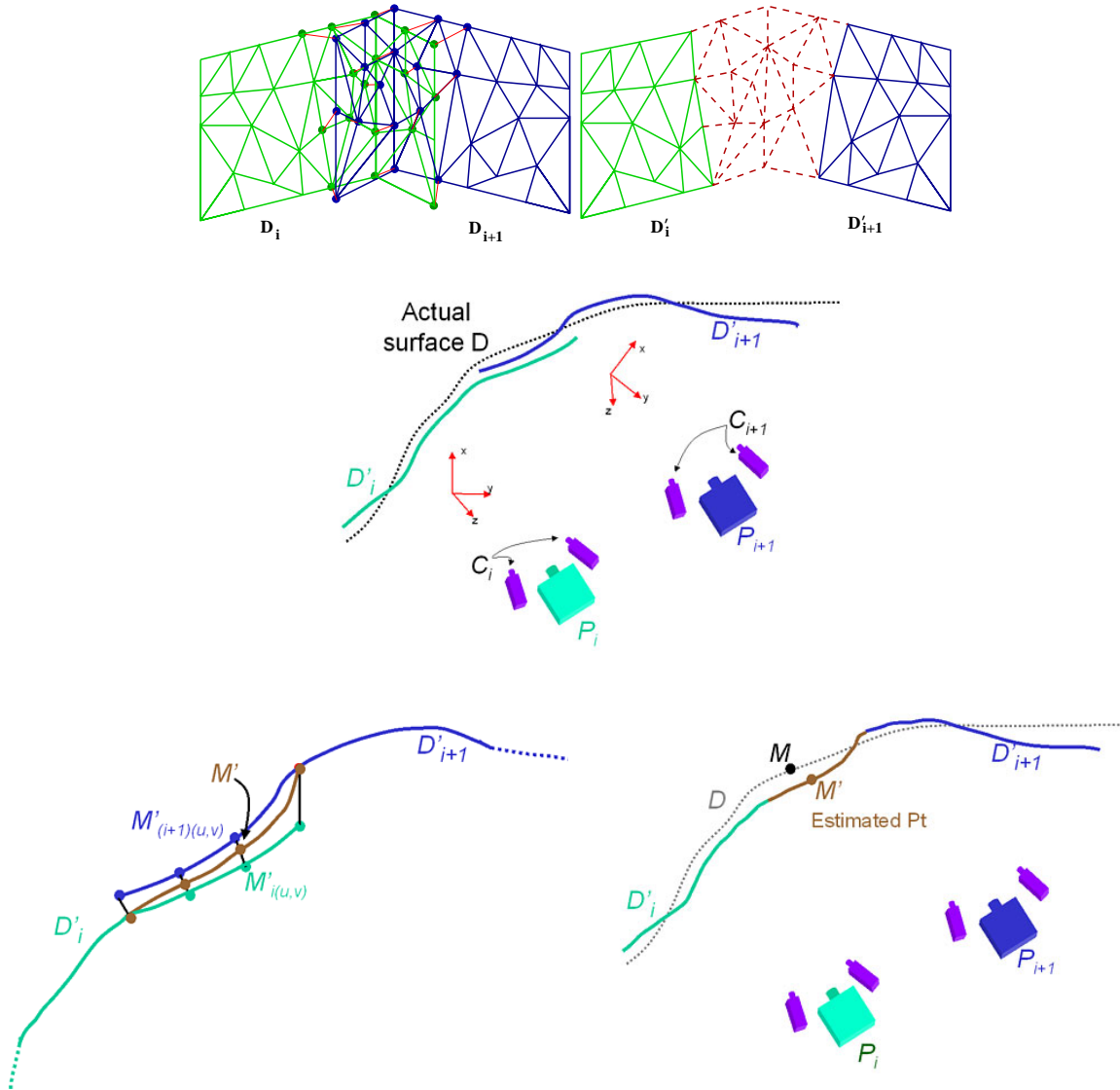
Figure 4.5: 3D points of the two display surfaces do not agree after registration with a rigid transformation so we use weighted averaging to obtain geometric continuity across the surfaces. Top row: Before and after mesh unification. Middle row: In flat land, before unification. Bottom left: Select corresponding points on the meshes and find a weighted average for smooth transition. Bottom right: Unified mesh. Note that the unified mesh is a convex combination of the component meshes but does not necessarily eliminate the deviation from the original mesh.
