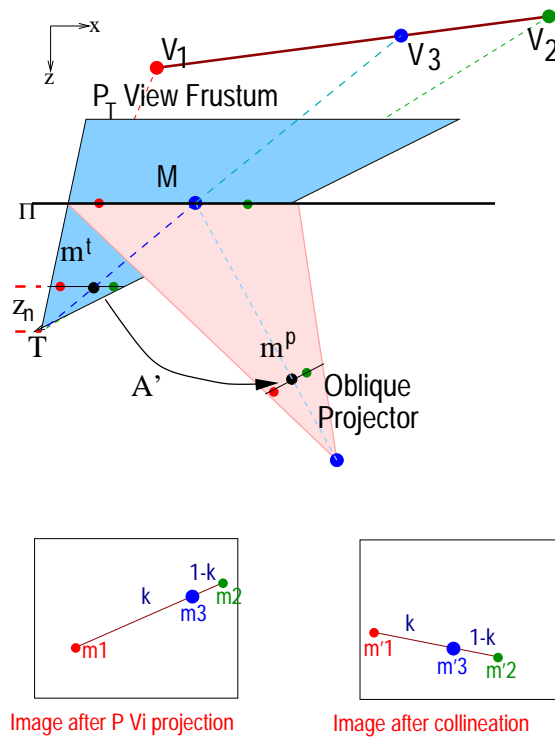
Figure B.1: Projection using off-axis projection matrix P_T followed by a warp using collineation A' .
