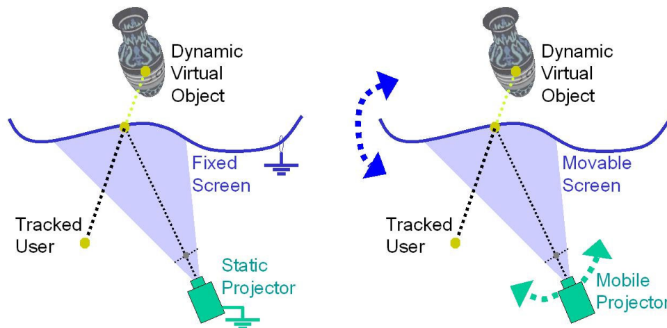
Figure 6.1: In the geometric framework for applications discussed so far, the projector and display surface is assumed static (left). However, the same geometric relationship can be expressed for dynamic projector and movable display surfaces (right).
