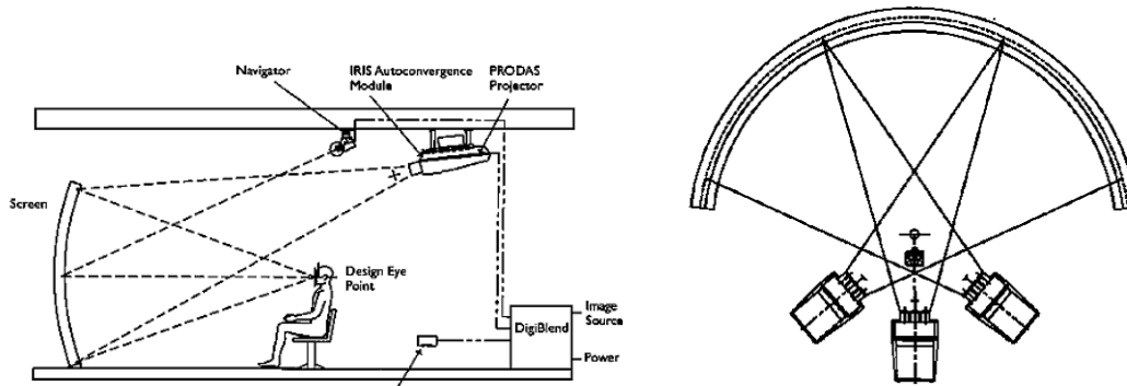
Figure 2.2: Layout for three projector Reality Room by Trimensions Inc.
