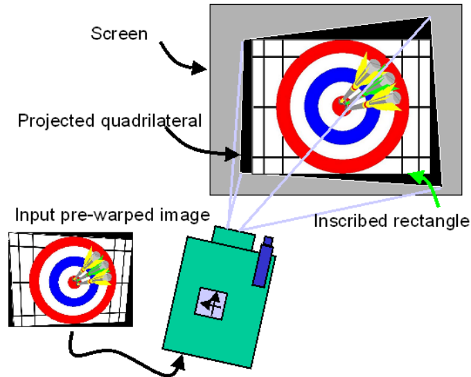
Figure 3.8: Given three angles of relative orientation, how should the input image be pre-warped to display axis aligned rectangular image?
