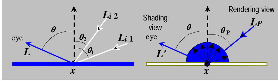
Figure 5.7: The radiance at a point in the direction (right) The radiance as a result of illumination from a projector lamp. By rearranging the parameters in the optical path, the two can be made equal.
