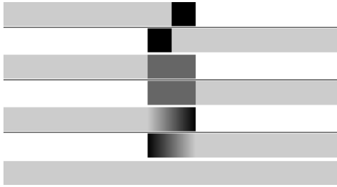
Figure 3.9: Ideal case, accurate registration. Top two rows, choice (a): contribution from a single projector for each point. Rows 3 and 4, choice (b): equal contribution from each projector in the overlap. Rows 5 and 6, choice (c): linear ramps in the overlap. Bottom row: Per pixel addition of contributing weights, all methods result in same solution.
