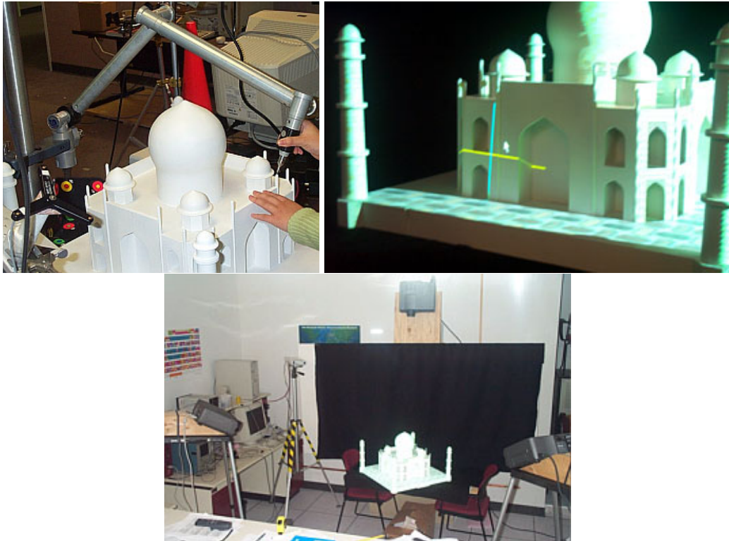
Figure 5.11: Top left: We used a 3D touch probe scanner to create a 3D model of the real object. Top right: The projectors are calibrated with respect to the model finding which pixels (the center of the cross) illuminate known 3D features. Bottom: The setup with projectors and the illuminated TajMahal model.
