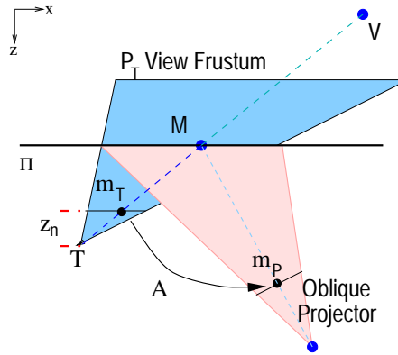
Figure 3.7: Rendering for planar surface. The pixels m_T and m_P are related by a homography.
