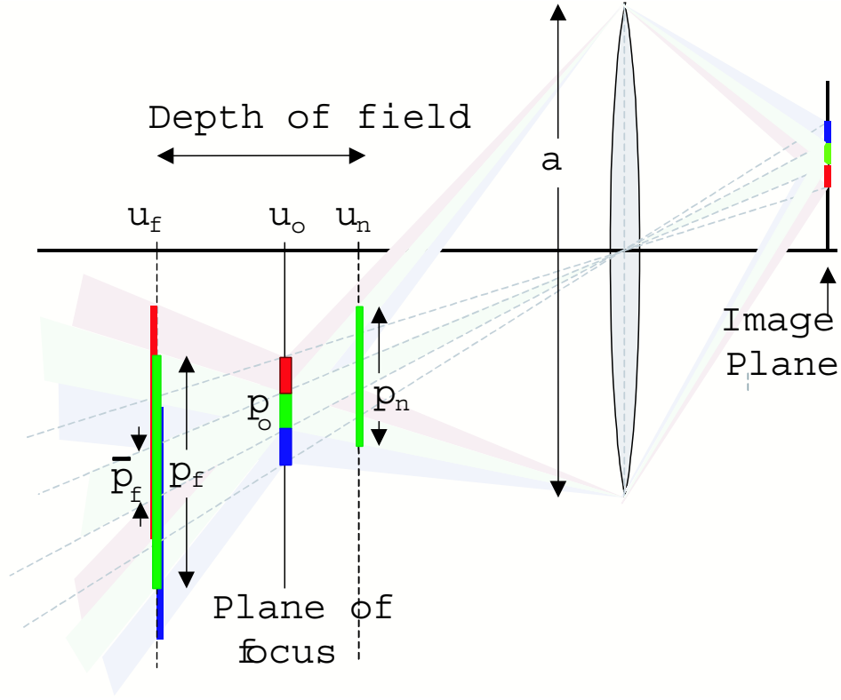
Figure A.1: Relationship between plane of focus and depth of field for a projector assuming thin lens model
