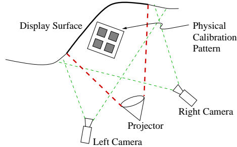
Figure 4.2: Configuration for single projector.
