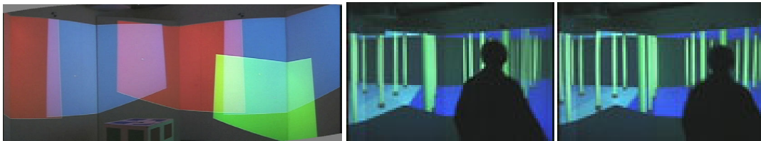
Figure 4.8: Left, Display environment with five projectors. Middle and Right, The images appear seamless and are updated as the user moves.
