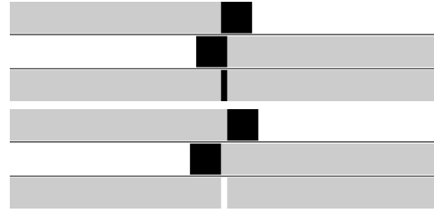
Figure 3.10: Choice (a): Contribution from a single projector at every point in overlap. Top three rows show result of mis-registration in case of projectors moving away from each other. Top row, projector moves to left. Second row, projector moves to right. Third row, resulting addition shows a dark gap. Bottom three rows show extra overlap results in a spiked region that is twice as bright.
