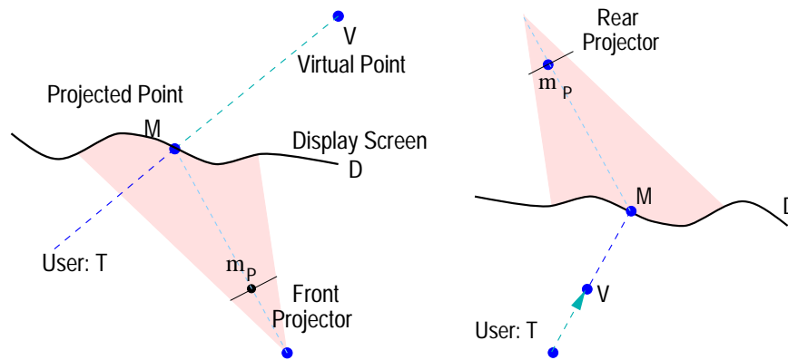
Figure 3.2: Rendering the image of virtual object under different projector display configurations. Left: A front projection display with a point on the virtual object behind the screen. Right: A rear-projection system with the virtual point in front of the screen. The display surface in both cases is non-planar.
