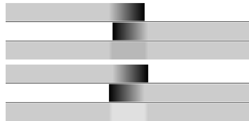
Figure 3.12: Choice (c): Linear ramps in overlap. Top three rows show projector moving away from each other, resulting in a overlap region with overall slightly lower intensity. Bottom three rows show extra overlap results in slightly brighter overlap regions.
