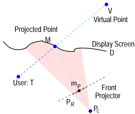
Figure 3.3: Relationship between geometric components.
