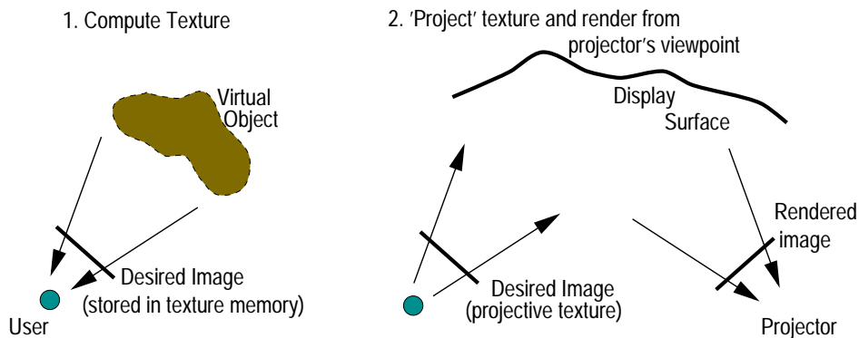
Figure 3.6: Two-pass rendering for non-planar display surface involves forward and backward mapping.
