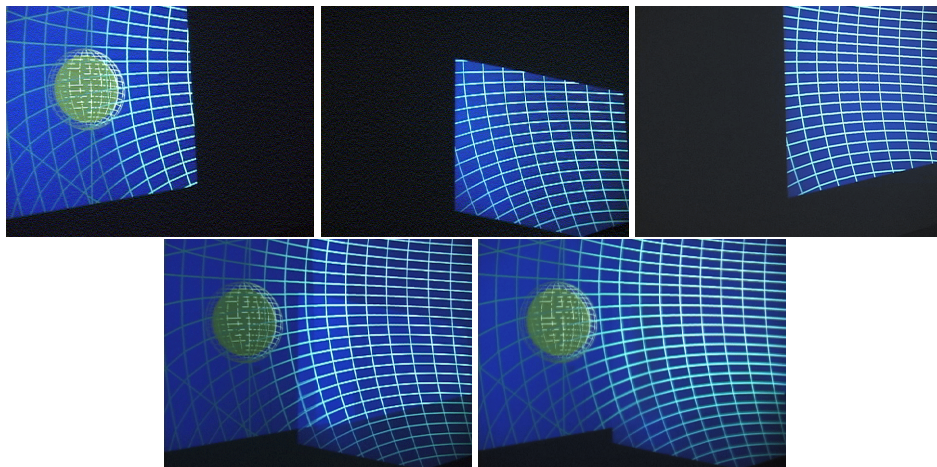
Figure 4.16: Top row: Images displayed by oblique projector which created keystoned imagery and but corrected using collineation. Bottom row: Displayed image without and with intensity blending.
