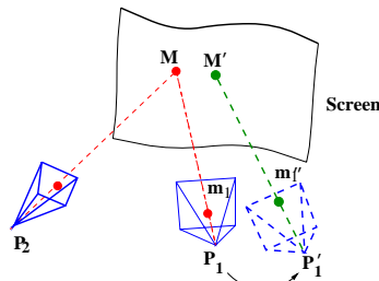
Figure 4.6: (a) Error in estimation of a physical point M on the display surface and error in estimated projection matrix P'_1 creates mis-registration. The reprojection error is m'' - m .
