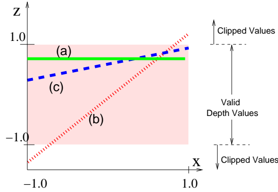
Figure 4.13: The plot shows depth buffer values along a scan line for points along constant depth. (a) Using P_T (b) After collineation, A_{4 \times 4}P_T , the depth values range beyond [-1, 1] (c) With an approximation of depth-buffer, A'_{4 \times 4}P_T , traditional graphics pipeline can be used to render perspectively correct images for a tracked moving user.
