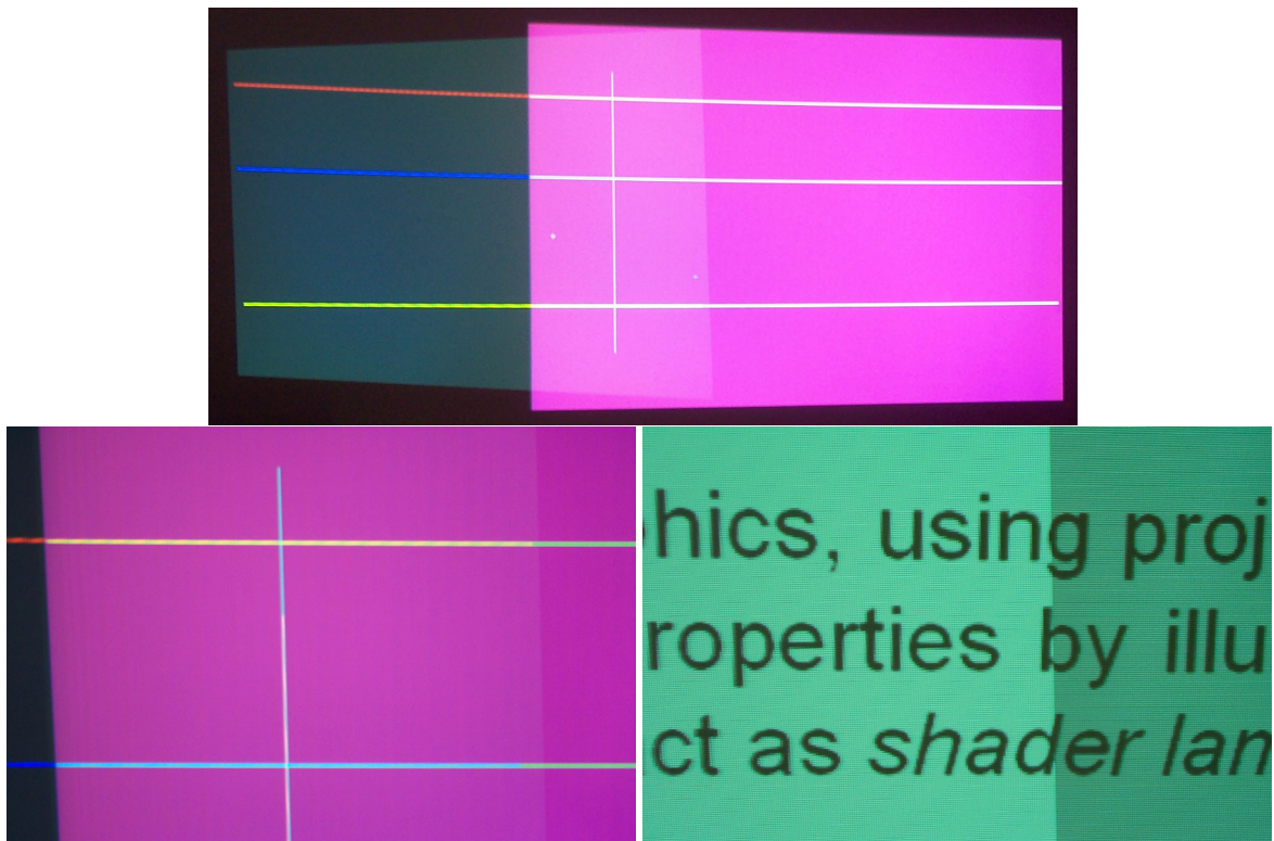
Figure 4.15: For a given plane of focus, projector can be treated as a pin-hole device. The pictures here show experimental verification of linear perspective projection. Straight line segments in image plane appear straight on a planar display surface (top). Further, line segments projected by overlapping projectors can be aligned to sub-pixel accuracy using homography (bottom left). Example of overlapping text in a warped image (bottom right).
