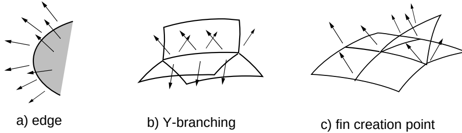
FIGURE 6. Local generic structure for Blum Medial axes in \mathbb{R}^3 and the associated Radial Vector Fields
