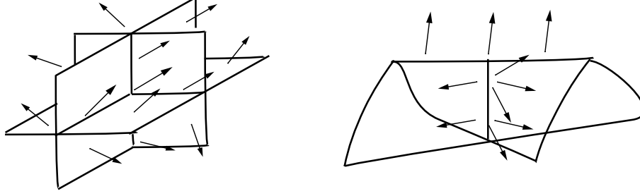
FIGURE 7. Possible nongeneric skeletal structures in \mathbb{R}^3 and associated Radial Vector Fields
