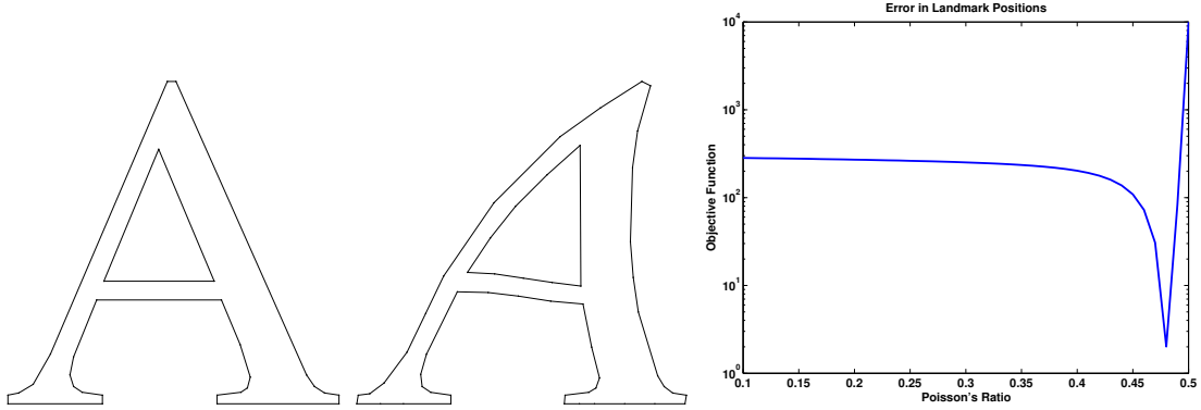
Figure 1.8: The initial shape (left), target shape (middle), and the plot of error versus Poisson’s ratio (right), where the error is based on the distance between corresponding vertices; the recovered value is 0.48 (ground truth is 0.49).
