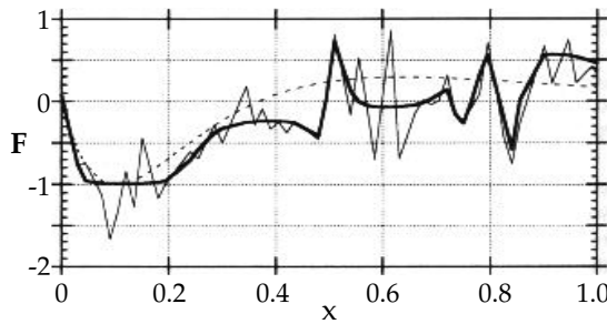
Underlying function (dotted), noisy sampling (thin line), and MLP generated model (thick line). Overtraining fits noise Figure 2.57
