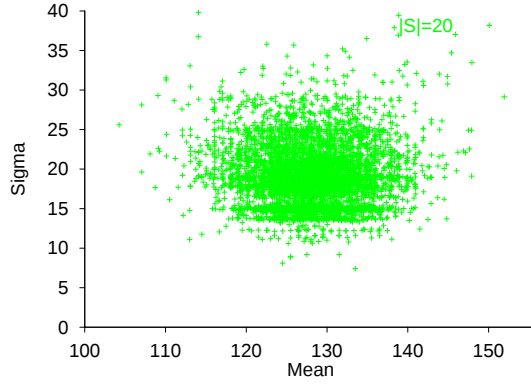
Scattergram of \mu, \sigma of local max in GGoF using X^2_{R\&C} given 20 samples Figure 4.46
