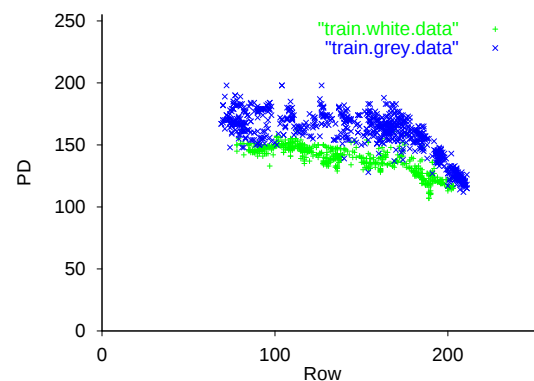
Scatterplot of samples from Figure 2.1 Figure 2.2
