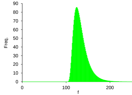
Skewed Gaussian Figure 5.2
