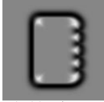
Central-oriented medialness of Figure 3.4 at small scale Figure 3.8
