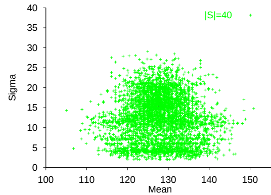
Scattergram of \mu, \sigma of local max in GGoF using \chi^2_{R\&C} given 40 samples Figure 4.38
