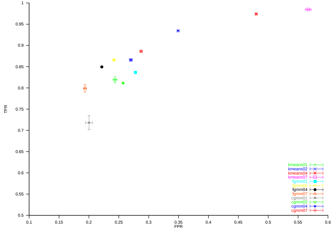
Plot of average TPR/FPR values and their Monte Carlo one-sigma ranges Figure 6.34
