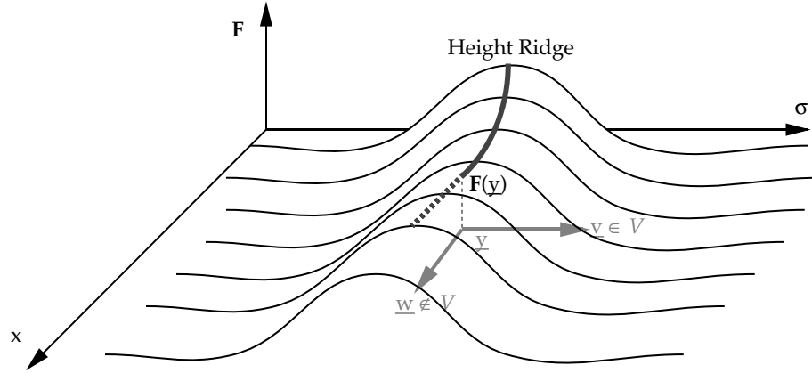
An M=1 dimensional height ridge V=\{\underline{v}\} in \leftarrow^{N+1=2} Figure 3.11
