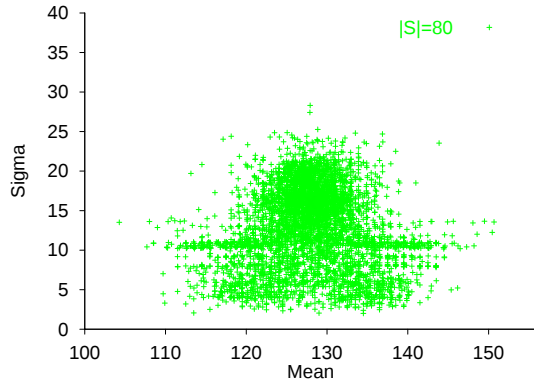
Scattergram of \mu, \sigma of local max in GGoF using X^2_{R\&C} given 80 samples Figure 4.57
