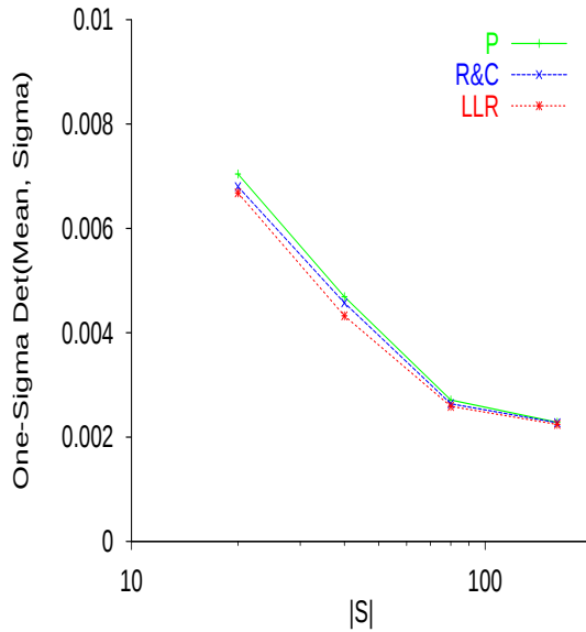
One-sigma of determinant of Monte Carlo \mu , \sigma covar. Figure 4.30
