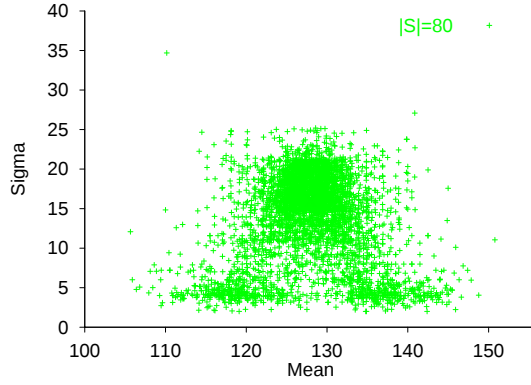
Scattergram of \mu, \sigma of local max in GGoF using X^2_{R\&C} given 80 samples Figure 4.24
