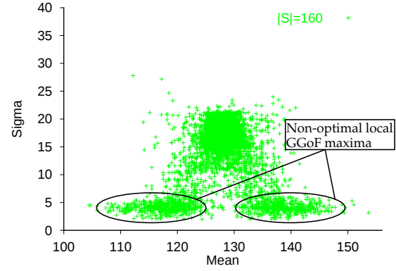
Scattergram of \mu, \sigma of local max in GGoF using X^2_{R\&C} given 160 samples Figure 4.25
