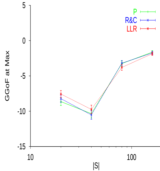
Average GGoF of local max in GGoF and one-sigma range Figure 4.31
