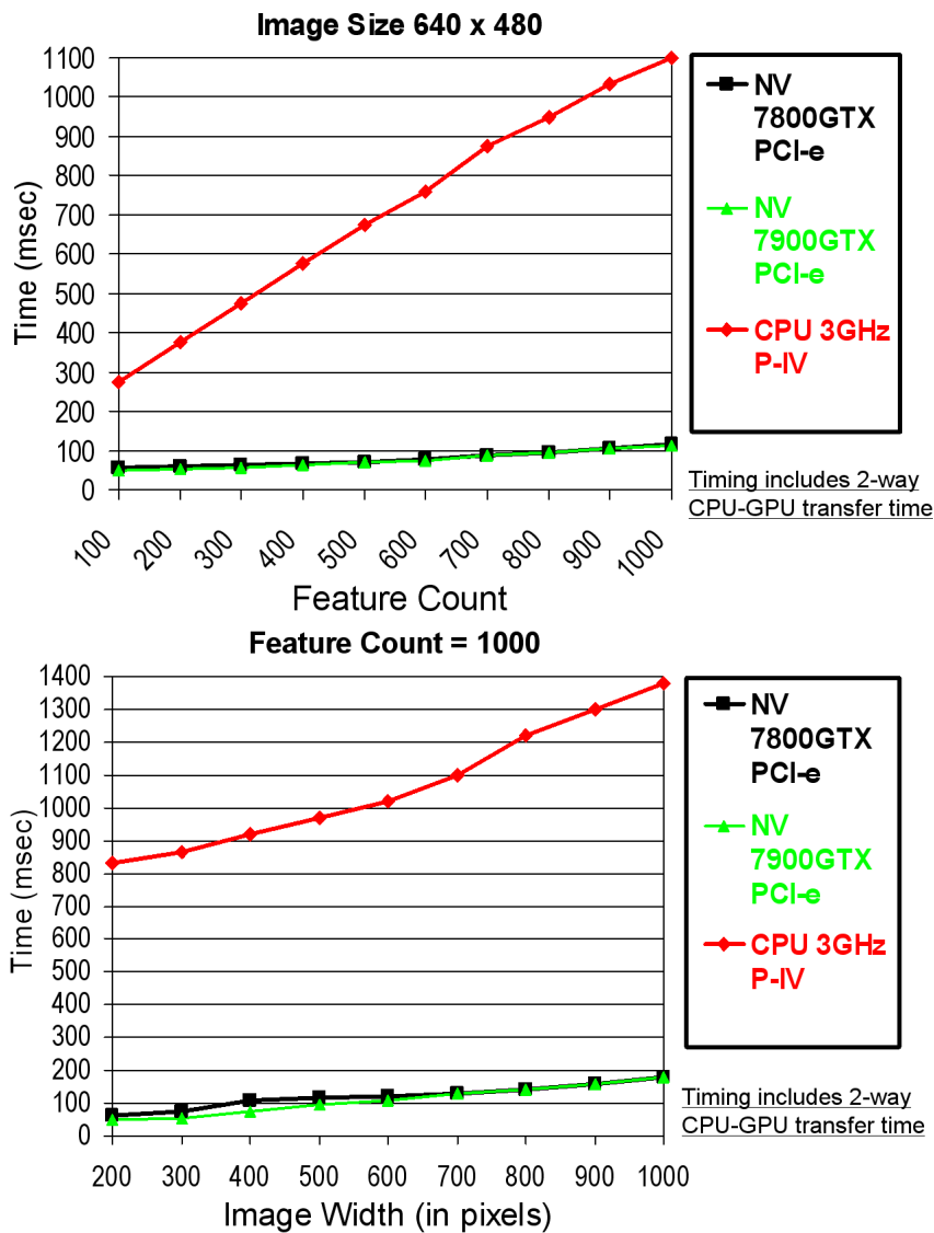
Fig. 9 GPU-SIFT timings compared with an optimized CPU implementation for a range of image-sizes and feature-counts. GPU-SIFT has a 10-12X speed-up.
