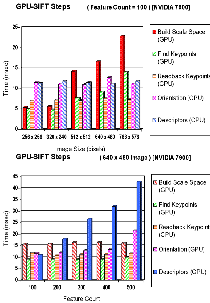
Fig. 10 (Top and Middle Row) Timings of various steps in GPU-SIFT are shown. For large feature-counts, computing descriptors on CPU dominates the running time while for large images, GPU computations dominates.
