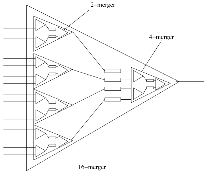
FIG. 6. Expansion of a 16-merger into 2-mergers.
