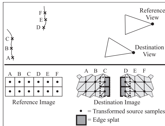
Figure 4.9: My general reconstruction and resampling technique. The top half of the figure is a top view of a scene. The bottom half shows the corresponding reference and destination images. The destination image depicts the transformed samples, the triangle mesh used for reconstructing the interiors of surfaces, and the edge splats used for reconstructing the edges of surfaces.
