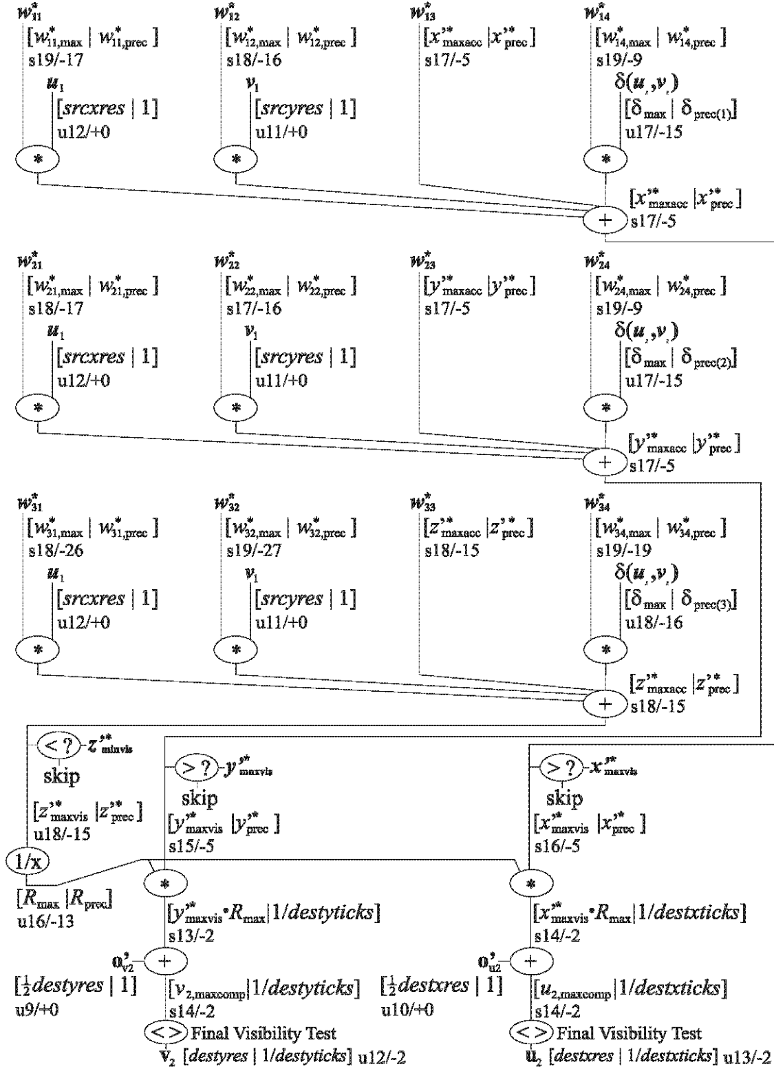
Figure 5.4: Computation tree for fixed-point 3D warp transformation. Sizes and precisions are given symbolically as [maxval | precision] , and numerically (for the parameters in the text) as s|uN / \pm M . s =signed, u =unsigned. N =total bits, not including sign. M =power-of-two for least significant bit.
