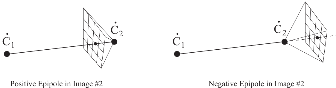
Figure 1.7: The type of epipole (positive or negative) is determined by the location of the epipole's image plane with respect to the two centers of projection.
