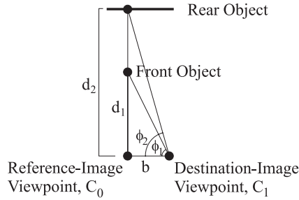
Figure 3.3: Dimensions for approximate calculation of visibility-hole size.
