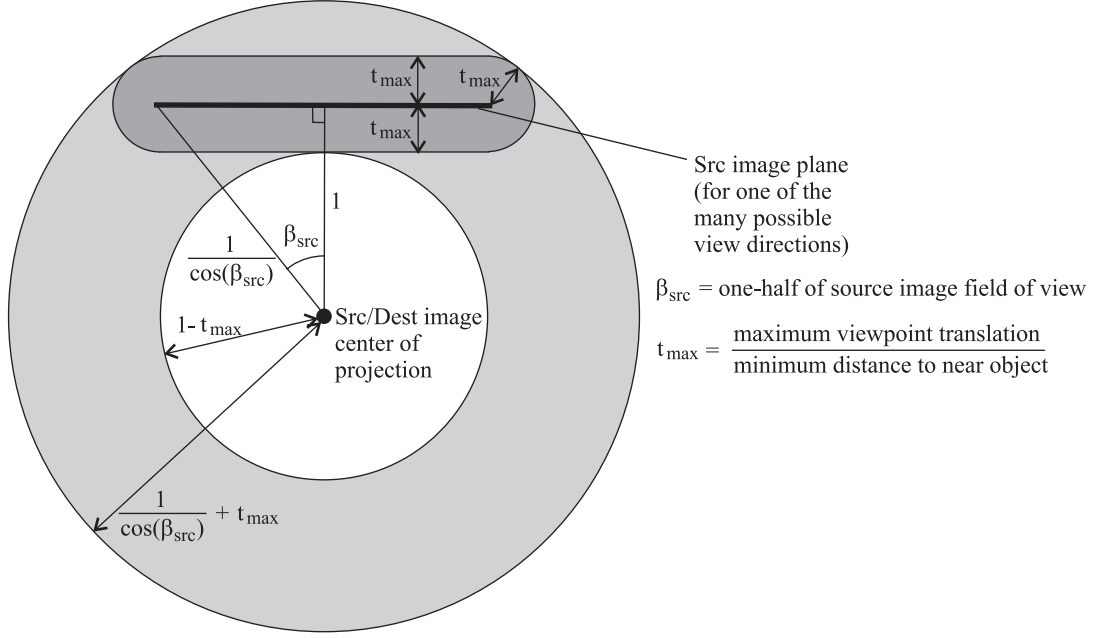
Figure 5.2: A geometric depiction of the behavior of Equations 5.3 for the 3D warp. As in the previous figure, the depiction is in world space, but it is for a 2D world rather than a 3D world. The figure uses McMillan’s disparity-based depiction of the 3D warp. Instead of representing the effects of viewpoint translation by showing separate source and destination viewpoints, the disparity-based depiction uses co-located source and destination viewpoints, and expresses translation by moving the source-image points away from the source-image plane. The magnitude of this movement is proportional to the disparity ( \delta ) of the point. The movement is bounded if we impose restrictions on the distance to the nearest object in the scene and the distance between the (true) source and destination image viewpoints. The grey region of the figure indicates the region of world space which can be touched by points on the source-image plane, after they have been translated. In this disparity-based depiction, the destination image shares its center of projection with the source image, but the destination-image view direction (not shown) is arbitrary.
