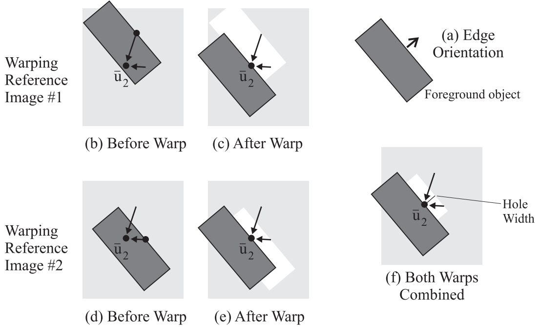
Figure 3.25: Hole size for a particular foreground-object edge and pair of warps. (a) shows the orientation of the edge, in the destination image. The edge orientation can be represented by a normal vector. (b) shows reference image #1 before the warp, with the translation vectors for both warps shown. (c) shows the result of warping reference image #1. (d) shows reference image #2 before the warp. (e) shows the result of warping reference image #2. (f) shows the hole left behind after completing both warps. The thin line from \bar{u}_2 to the foreground-object edge represents the width of the hole. This line is perpendicular to the edge.
