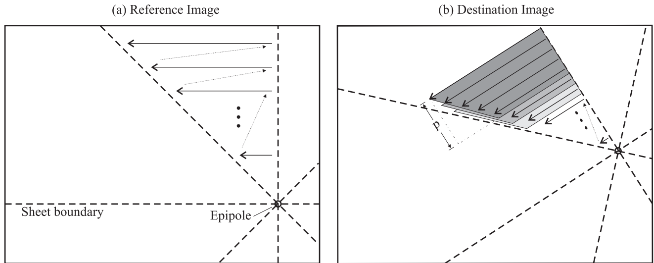
Figure 5.11: Non-simultaneous eight-sheet occlusion-compatible traversal for the 3D warp. The potentially-written areas in the destination image that are produced by different reference-image scan lines overlap almost completely. I show these areas using their worst-case rectangular approximations, with the edges cut off slightly to allow the overlap to be more easily seen.
