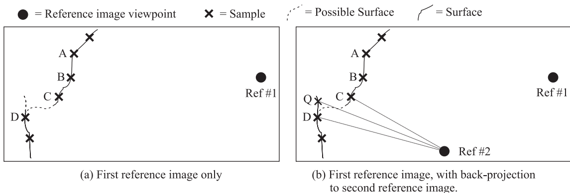
Figure 4.20: Using back-projection for surface segmentation (in flatland). In (a), it is unclear whether or not samples C and D lie on the same surface. In (b), back-projection to a second reference image is used to resolve the ambiguity. Samples C and D are projected into reference image #2, and a new sample Q is detected that lies in between them in the image plane. Because this sample is farther away, there can not be a valid surface connecting samples C and D.
