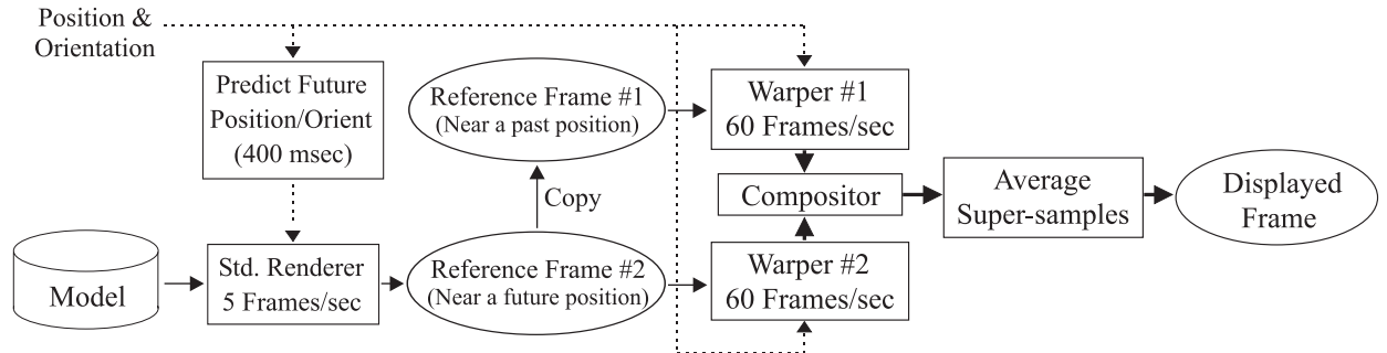
Figure 1.3: Conceptual diagram of a post-rendering 3D warping system.
