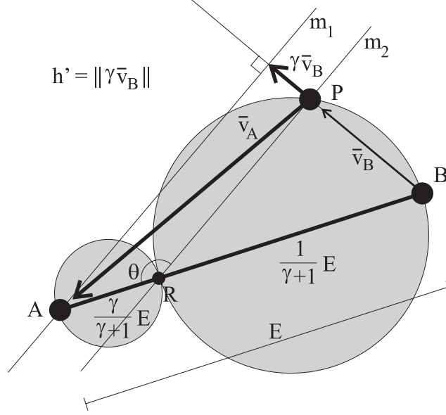
Figure 3.29: Transition between hole-size case #1 and case #2. The transition occurs when point P lies at the edge of the grey circles. The interior of the circles represents the region in which case #2 is applicable.
