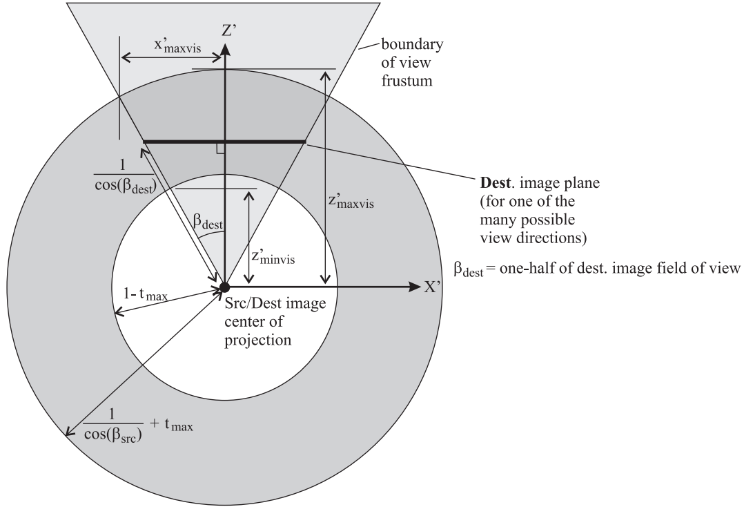
Figure 5.3: Valid locations of transformed points within the destination-image view frustum. The destination-image view frustum is shown in light grey. The destination-image's 3D coordinate system (actually 2D in this reduced-dimension figure) is indicated by the X' and Z' axes. The points to be projected onto the destination image plane all fall within the dark grey region, as calculated earlier. Thus, these points have a minimum and maximum possible z' value: z'_{min} and z'_{max} .
