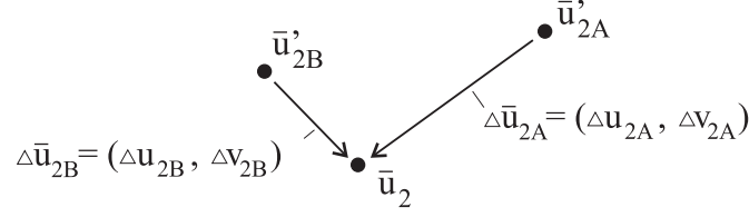
Figure 3.23: Destination-image movement of a single object, due to translation. The same object is represented in two reference images. The pre-translation (post-rotation) destination-image location for the object's representation coming from reference image A is \bar{u}'_{2A} . The corresponding location for reference image B is \bar{u}'_{2B} . The final, post-translation, location of the object is \bar{u}_2 . The arrows indicate the destination-image movement caused by translation, which is described by equation 3.34.
