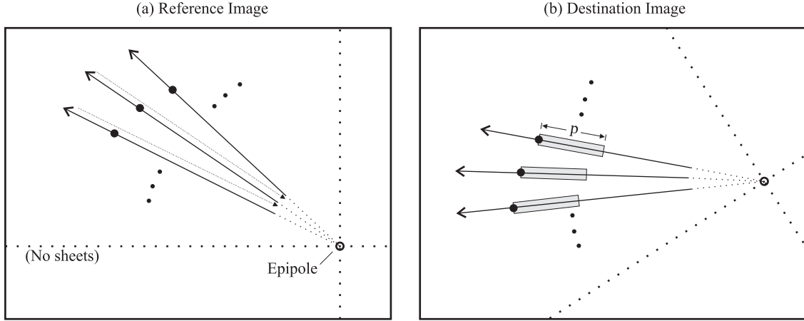
Figure 5.9: Epipolar-line traversal. The destination image shows the potentially-written areas corresponding to the indicated reference-image points.
