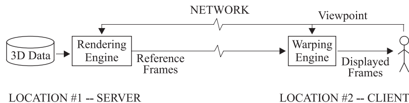
Figure 6.1: Remote display system.
