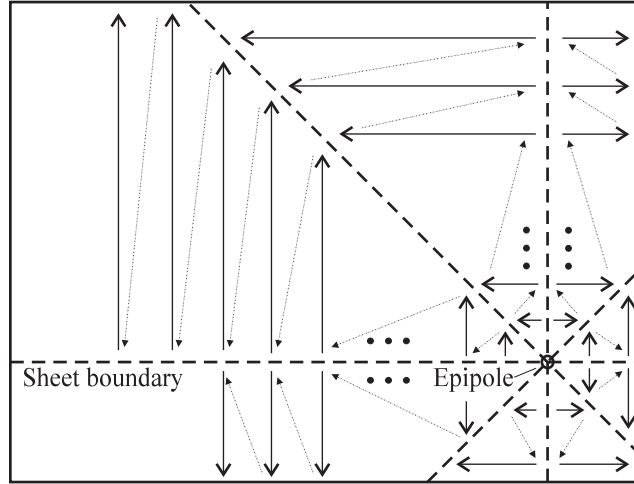
Figure 3.15: Eight-sheet occlusion-compatible image traversal. The image is divided into up to eight sheets. Each sheet is traversed in a raster-like order to perform hole filling. By using eight sheets, we can guarantee that the local traversal direction is always within 45^\circ of the ideal direction specified by the epipolar geometry.
