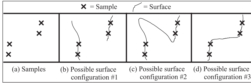
Figure 4.4: Different surface configurations are possible with the same set of samples. In every part of this figure, the reference-image viewpoint is far to the right.
