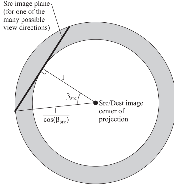
Figure 5.1: A geometric depiction of the behavior of Equations 5.3 for the case of a rotation-only warp (perspective warp). The depiction is in 2D rather than 3D. The grey region indicates the region of world space which can be touched by points on the source-image plane, if we allow an arbitrary view direction for the source image. The destination image (not shown) shares the center of projection with the source image, and also has an arbitrary view direction.
