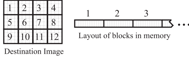
Figure 5.8: Alternative memory layout for the destination image. Pixels belonging to 2D tiles of the destination image are stored contiguously in memory.
