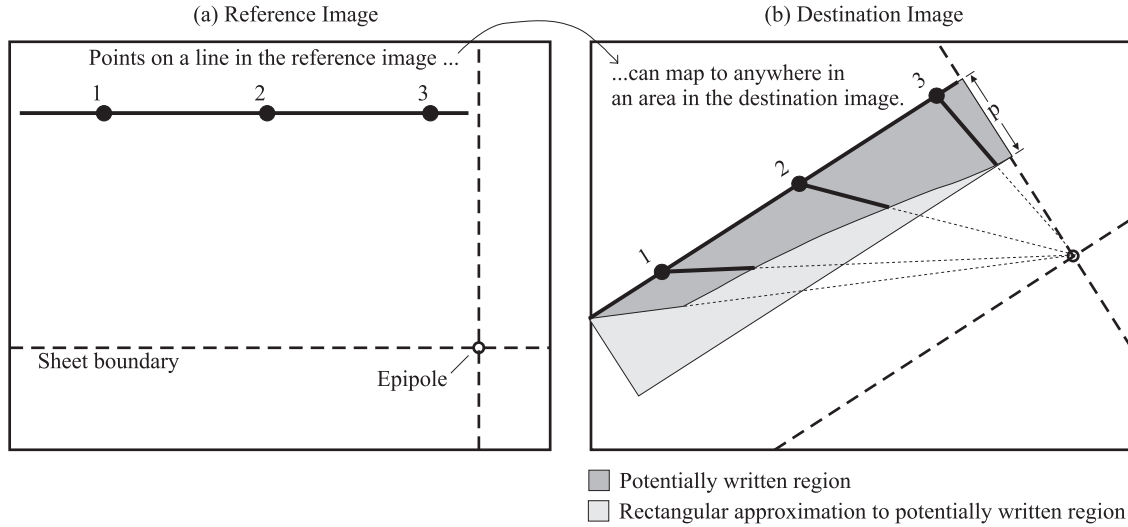
Figure 5.7: 3D warp of a line. The points on a reference-image line can map to anywhere in an area in the destination image. My analysis approximates this area with a worst-case rectangular region.
