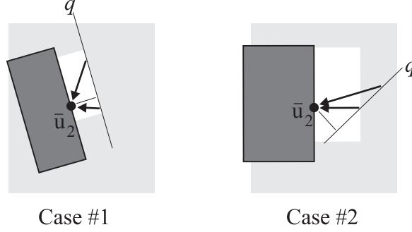
Figure 3.26: There are two possible cases for the worst-possible edge orientation. To determine the correct case, begin by drawing a line, q , between the tails of the two translation vectors. Then, find the perpendicular from line q to point \bar{u}_2 (this perpendicular is the short, thin line in the figure). If the angle at which this perpendicular intersects \bar{u}_2 is in between the angles at which the two translation vectors leave \bar{u}_2 , then case #1 is indicated. For case #1, the worst-possible edge orientation is parallel to line q . If the angle of the perpendicular is not in between the translation-vector angles, then case #2 is indicated. For case #2, the worst-possible edge is perpendicular to the shorter of the two translation vectors.
