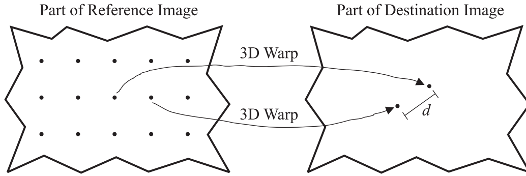
Figure 4.7: The surface segmentation algorithm uses an image-space distance threshold to determine whether or not adjacent source-image samples represent the same surface. If the distance, d , between the transformed locations of the samples exceeds a fixed threshold, then the samples are considered to represent different surfaces.
