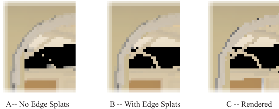
Figure 4.10: Using edge splats improves image quality. Anti-aliasing was disabled for all of the following three images: (a) An image produced without using edge splats. Parts of the window trim disappear completely. (b) An image produced using edge splats. (c) A conventionally rendered image, for comparison purposes.
