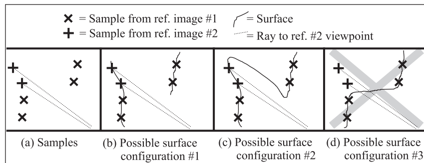
Figure 4.5: Information provided by a second reference image can resolve or partially resolve ambiguities in surface reconstruction. This figure shows that the two additional samples from a second reference image eliminate surface configuration #3 as a possibility.
