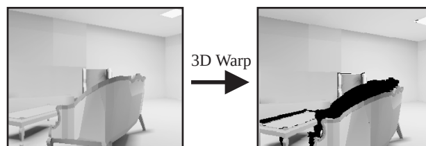
Figure 3.11: Visibility holes left by a 3D warp (shown here in black) are always located at the boundary between a foreground object and the object(s) behind it. In this case, holes form at some of the boundaries of the sofa and table. Note that holes do not appear at all foreground/background boundaries.
