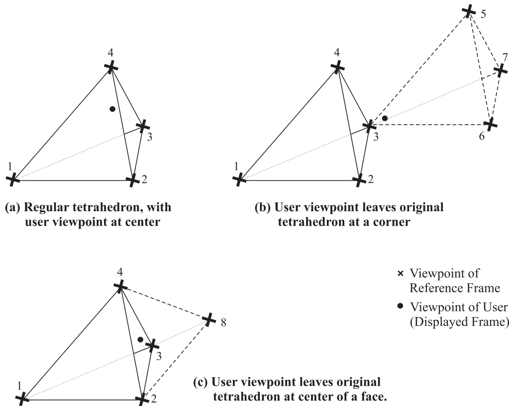
Figure 3.8: Working with four reference-frame viewpoints. (a) Reference viewpoints are arranged in a regular tetrahedron. (b) If the user's viewpoint leaves the tetrahedron near a vertex, three new reference images (#5, #6, and #7) must be generated almost simultaneously. (c) If the user's viewpoint leaves the tetrahedron near the middle of a face, only one new reference image (#8) must be generated.
