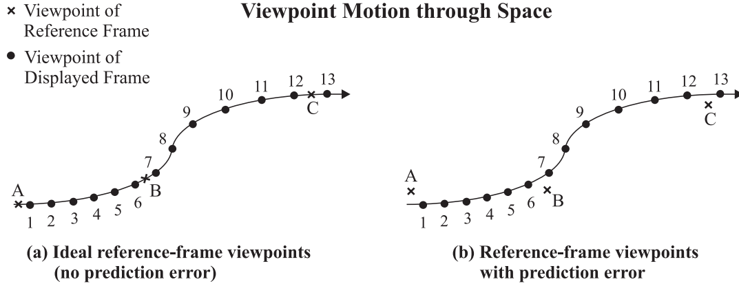
Figure 3.6: Displayed frames are computed by warping two reference frames, one near a past position of the viewer, and one near a future position of the viewer. For example, derived frame #5 is produced by warping reference frames A and B. Ideally the reference frames lie exactly on the viewpoint path, as shown in (a). But if future viewpoint locations are unknown, then viewpoint-motion prediction must be used to estimate them. As a result, the reference frames do not fall exactly on the viewpoint path, as shown in (b).
