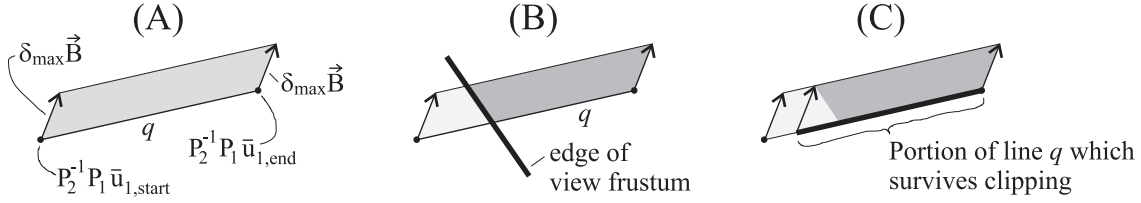
Figure 5.12: Clipping for the 3D warp. (a) Possible locations of warped pixels from a reference-image scan line. These locations form a parallelogram in the displayed image's projective coordinate system. (b) The parallelogram is clipped against the displayed image's view frustum. (c) The clipped vertices are then used to determine the extent of the reference image line which must be warped.
