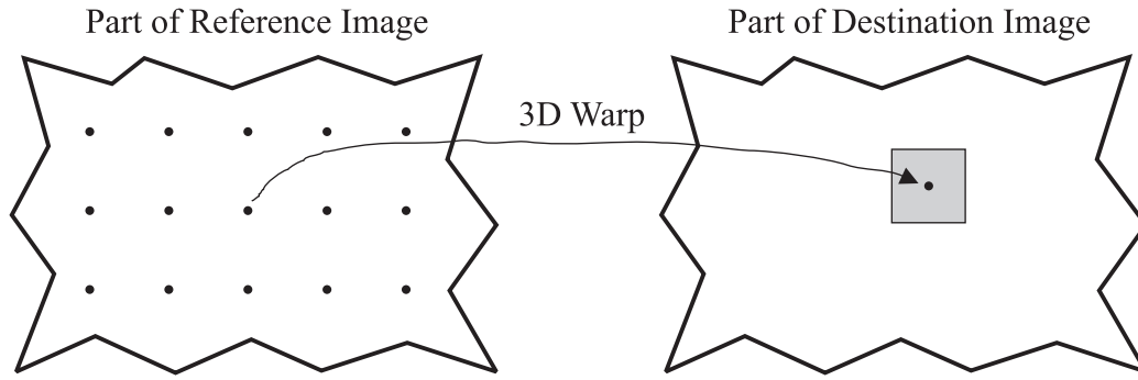
Figure 4.15: Fixed-size splat approach to reconstruction. Each reference-image sample is transformed to the destination image. Then, the warper fills a fixed-size axis-aligned region surrounding the transformed location with the sample’s color.
