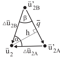
Figure 3.27: Angles and lengths for hole-size computation.
