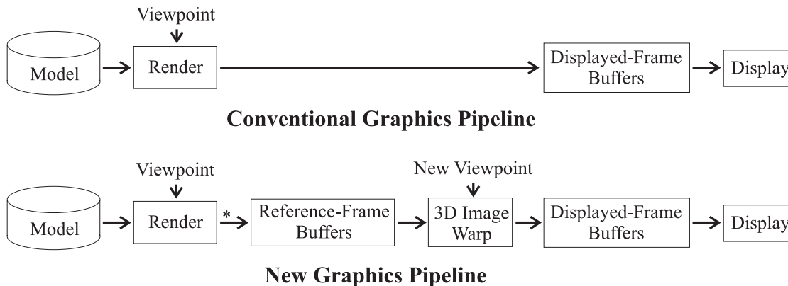
Figure 1.1: Conventional graphics pipeline vs. new proposed pipeline. If desired, the new pipeline can be split into a client half and a server half at the point indicated by * to create a system for low-latency display of rendered images at a remote location. I refer to the images produced by the conventional renderer as reference frames, and the the images that are displayed as displayed frames.
