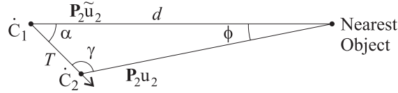
Figure 5.6: Angular object movement across the field-of-view is a function of initial object distance and the distance between reference-image and destination-image viewpoints. The distance to the object is specified by d , and the distance between image viewpoints is specified by T .
