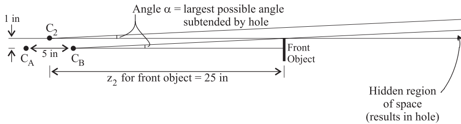
Figure 3.30: The 3D geometry used for my example 3D calculation of hole size. C_A and C_B represent the two source-image centers of projection. The distance between these two centers of projection is \|\vec{b}\| = 5 . The displayed-image center of projection is labeled C_2 . The distance between this center of projection and the line between the two source images is \|\vec{d}\| = 1 . C_2 is equidistant from C_A and C_B . The distance from the displayed-image center of projection to the nearest object in the scene is z_2 = 25 . The hole that opens between the “front object” and a background surface at infinite distance (not shown) subtends an angle \alpha from the displayed-image center of projection ( C_2 ). For calculation purposes, I also show this angle relative to position C_B . Note that the angle \alpha used in this figure is a different angle from the \alpha used in Figure 3.27.
