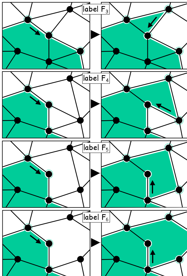
Figure 4: Face Fixer uses labels F_3, F_4, F_5, F_6, \dots to encode polygonal faces in a mesh.
