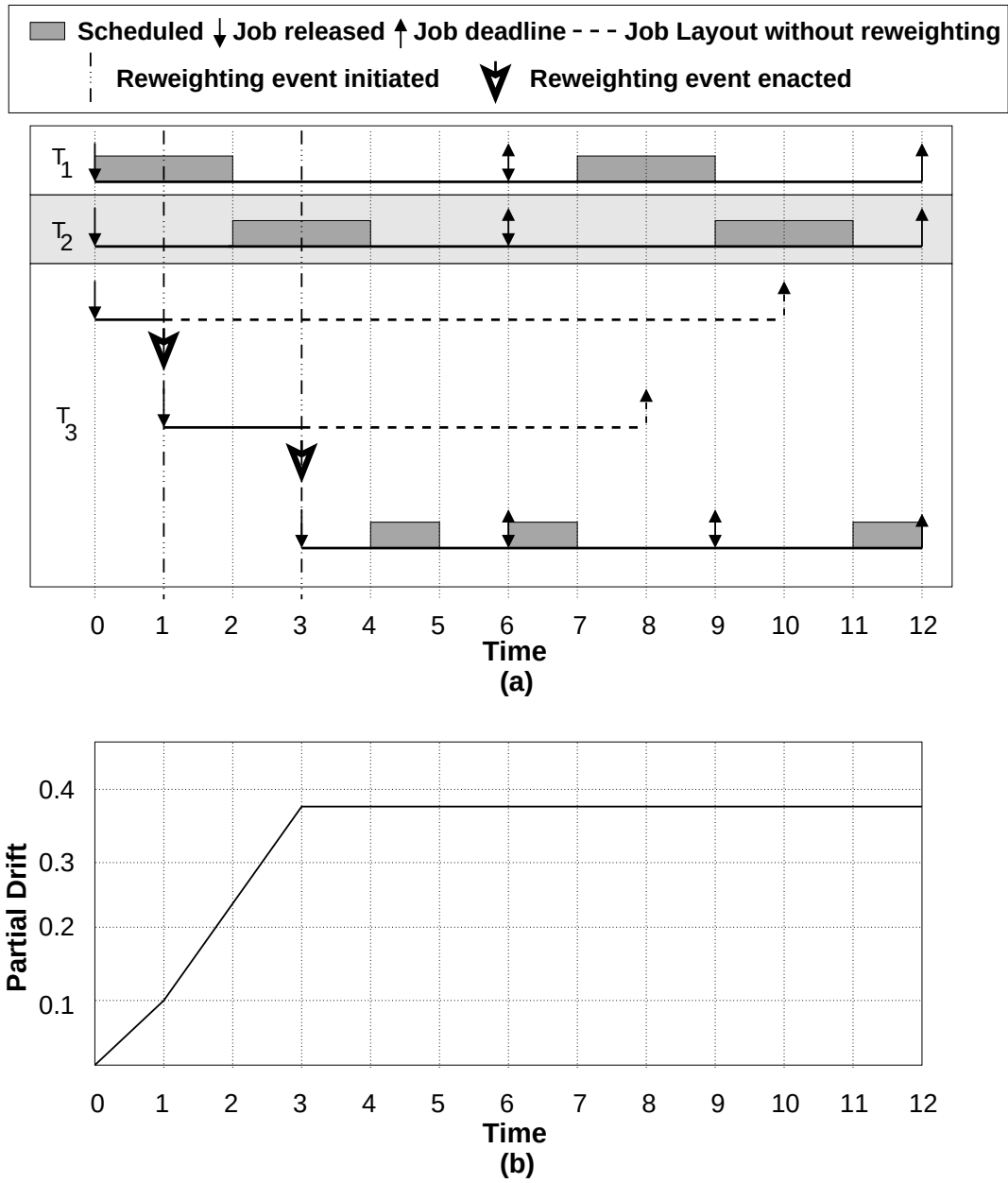
Figure 4.19: A one-processor example of multiple reweighting events. (a) The PEDF schedule. (b) T_3 's partial drift.
