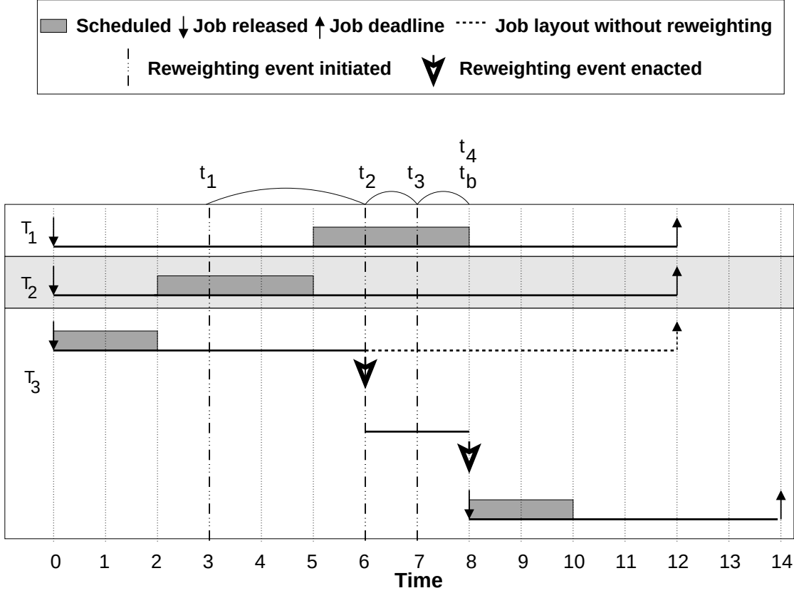
Figure 4.18: A one-processor example of the task decomposition in Lemma 4.4.
