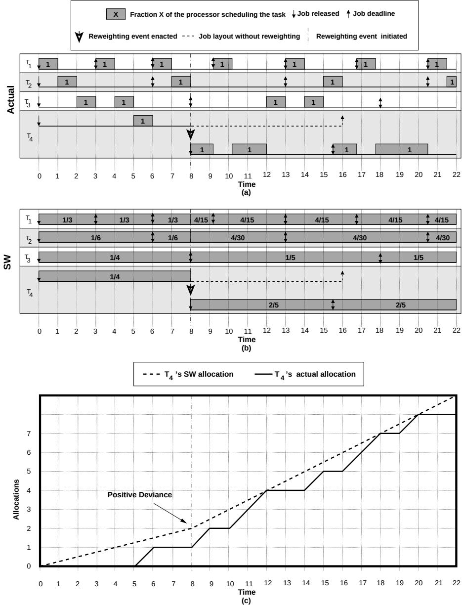
Figure 4.3: A one-processor system with four tasks. (a) The PEDF schedule. (b) The SW schedule. (c) The allocations to T_4 in the PEDF and SW schedules.
