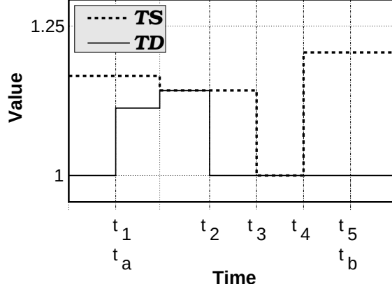
Figure 4.21: Decomposition of a task for Lemma 4.9.
