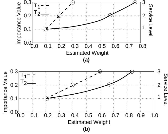
Figure 6.1: Estimated weight vs. importance value/service level for two tasks. (a) e = 0.1 . (b) e = 0.2 .
