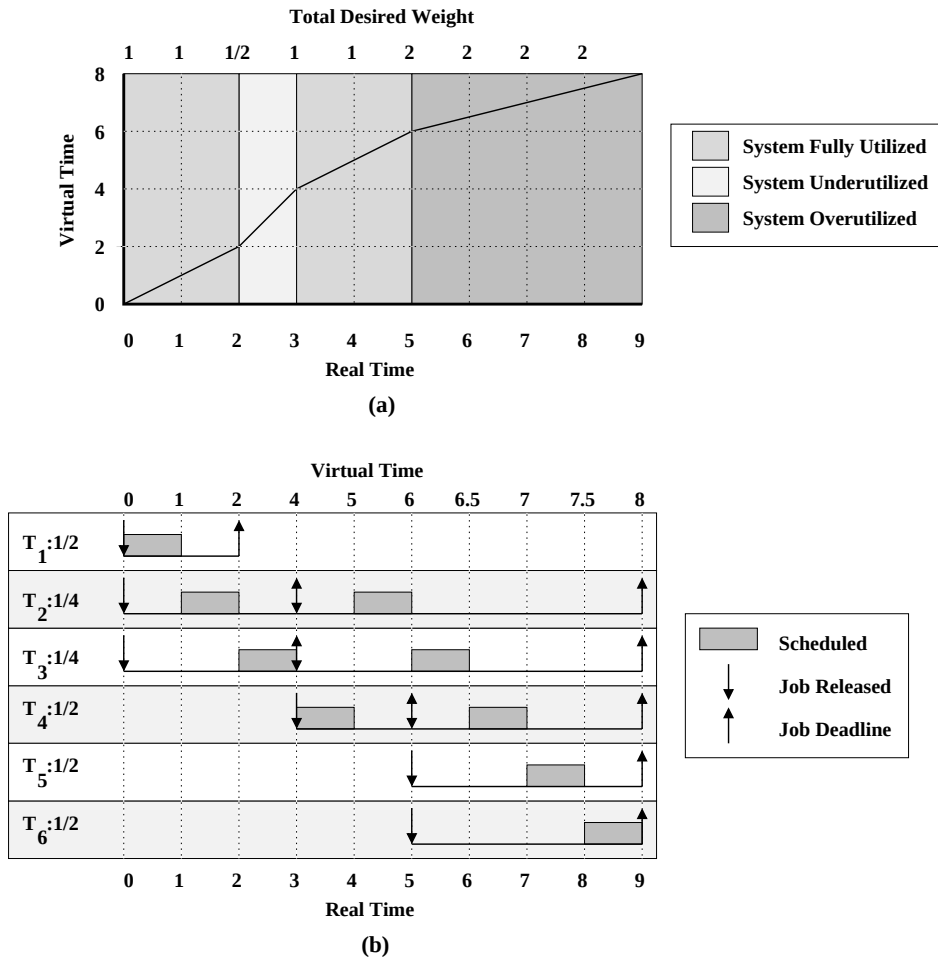
Figure 2.3: A one-processor system scheduled by EEVDF. (a) The mapping of virtual time to real time. The total desired weight of active tasks for each time range [t, t + 1) is labeled across the top axis. (b) The EEVDF schedule.
