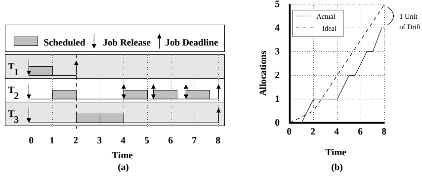
Figure 1.7: The (a) EDF schedule and the (b) ideal and actual allocations to T_2 in a one-processor example of leave/join reweighting.
