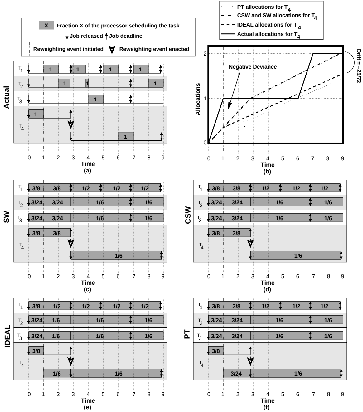
Figure 4.17: A one-processor system with four tasks. (a) The PEDF schedule. (b) The allocations to T_4 in the PEDF, IDEAL, SW, CSW, and PT scheduling algorithms. (c) The SW schedule. (d) The CSW schedule. (e) The IDEAL schedule. (f) The PT schedule.
