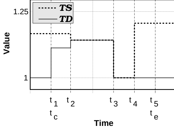
Figure 4.20: Decomposition of a task for Lemma 4.7.
