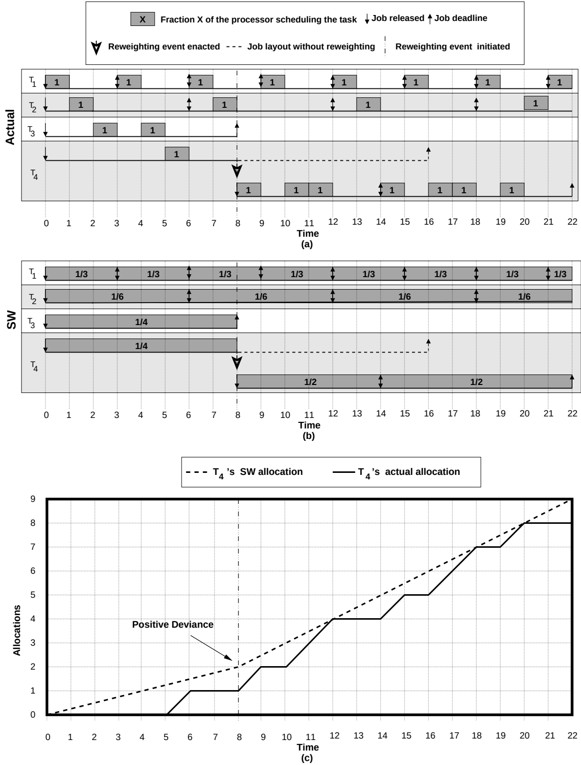
Figure 3.2: A one-processor example of a task that increases its weight. (a) The GEDF schedule. (b) The SW schedule. (c) The allocations to T_4 in the GEDF and schedules.
