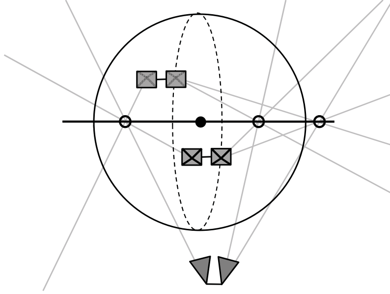
Figure 4.7: The first degenerate case. When all the features (two-view and four-view) lie on a 3D line through the four-view feature the second camera can be anywhere on a circle which is the intersection of the sphere and a plane orthogonal to the line containing the four-view feature.
