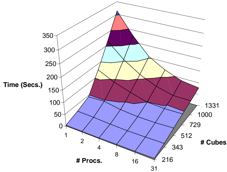
Figure 5.14: This graph shows the time it takes to recalculate HLODs of a scene consisting of a specific number of cubes utilizing a specific number of simplification processes. It shows complex scenes ranging from 216 to 1,331 cubes. Adding processes significantly speeds up the recalculation process as the scenes grow in complexity. For small scenes, adding processes may reduce the performance of the system (see Figure 5.13).
