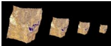
Figure 3.31: Switching distances for LODs of the Sierra object if we allow 1 pixel of error. From left to right these LODs consist of 81,345 faces, 40,671 faces, 20,335 faces, and 10,168 faces. The original object consists of 162,690 faces.
