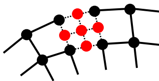
Fig. 4.2. Sub-sampling a slab-like core. Black dots represent previously computed medial atoms at the existing coarse scale, red dots represent newly sampled atoms, solid line segments represent implied connections between computed atoms, and dotted line segments represent implied connections to new atoms.
