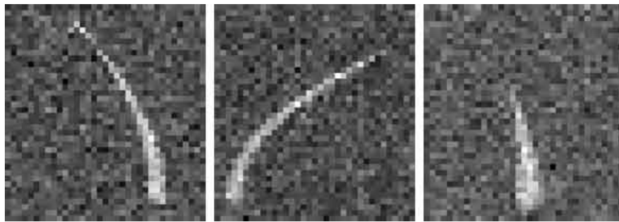
Fig. 7.13. Slices through synthetic 3D images of three different tubes that narrow to a width of zero. The tubes in these three examples have no torsion, but similar images were created of tubes with moderate amounts of torsion. Noise typical of MR data was added to each image.
