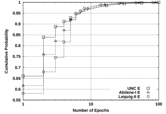
Figure 3.19: Bodies of the E distributions for Abilene-I, Leipzig-II and UNC 1 PM.
