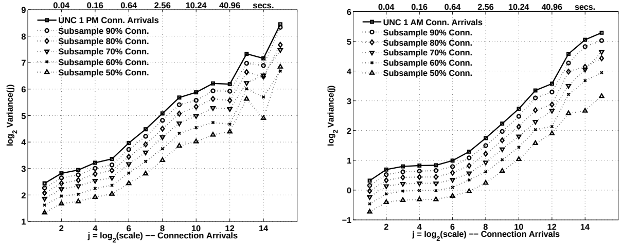
Figure 7.21: Wavelet spectra of several random subsamplings of the connection vectors in UNC 1 PM (left) and 1 AM (right)
