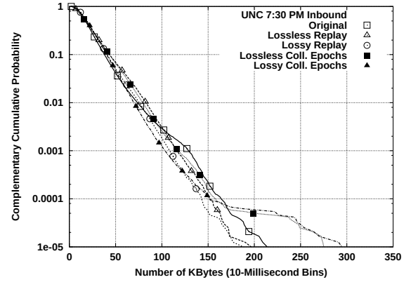
Figure 6.44: Byte throughput marginals for UNC 7:30 PM inbound and its four types of source-level trace replay.
