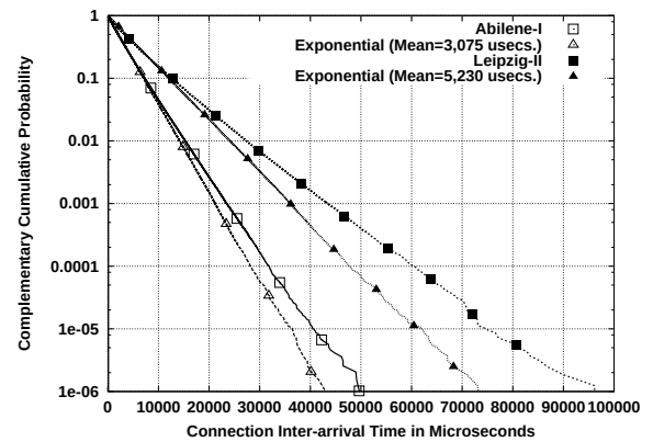
Figure 7.4: Tails of the distributions of connection inter-arrivals for Abilene-I and Leipzig-II, and their exponential fits.
