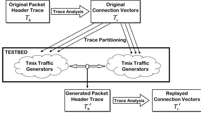
Figure 5.1: Overview of Source-level Trace Replay.
