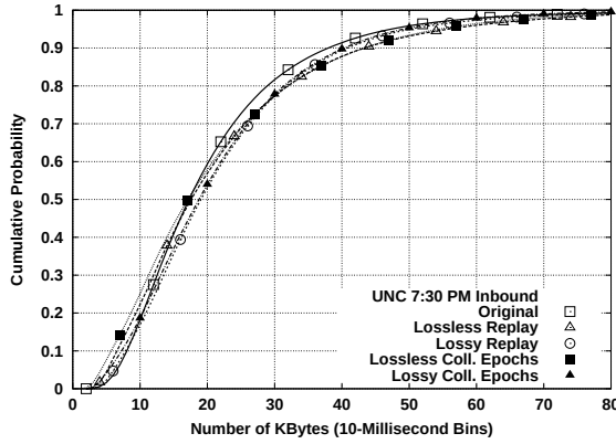
Figure 6.44: Byte throughput marginals for UNC 7:30 PM inbound and its four types of source-level trace replay.
