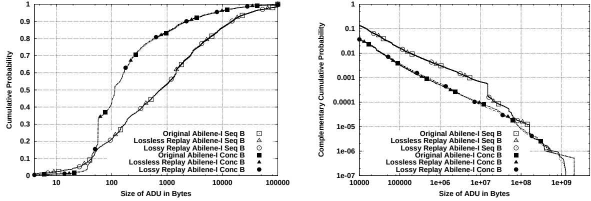
Figure 5.19: Bodies and tails of the B distributions for Abilene-I and its source-level trace replays.
