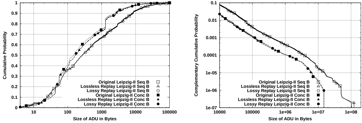
Figure 5.5: Bodies and tails of the B distributions for Leipzig-II and its source-level trace replays.
