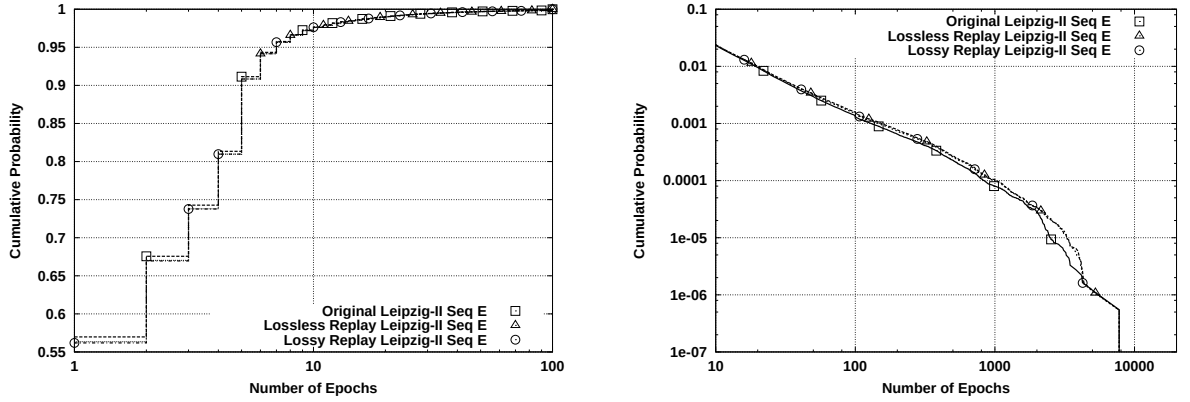
Figure 5.6: Bodies and tails of the E distributions for Leipzig-II and its source-level trace replays.
