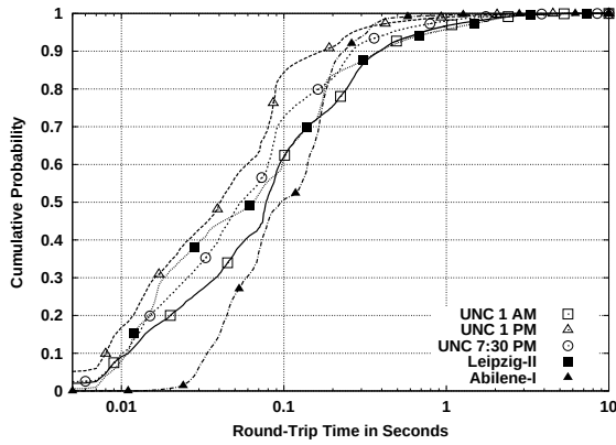
Figure 4.12: Bodies of the RTT distributions for the five traces.
