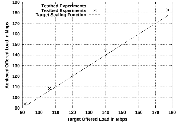
Figure 7.23: Analysis of the accuracy of byte-driven Block Resampling using source-level trace replay: replay of one resampling of UNC 1 AM for each target offered load, illustrating the scaling up of load from the original 91.65 Mbps.
