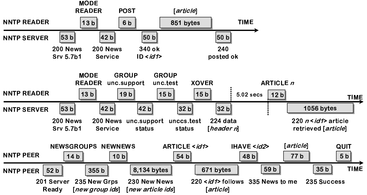
Figure 3.4: Three a-b-t diagrams representing three different types of NNTP interactions.
