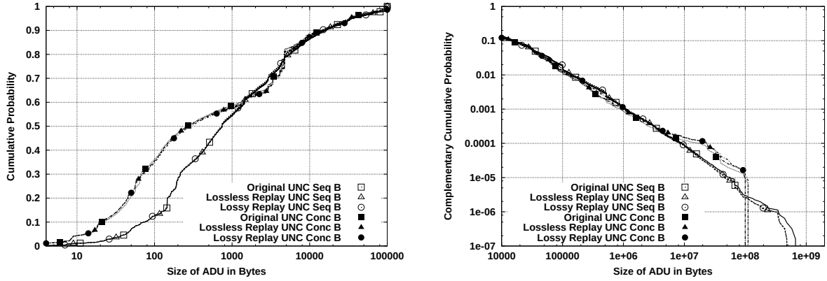
Figure 5.12: Bodies and tails of the B distributions for UNC 1 PM and its source-level trace replays.
