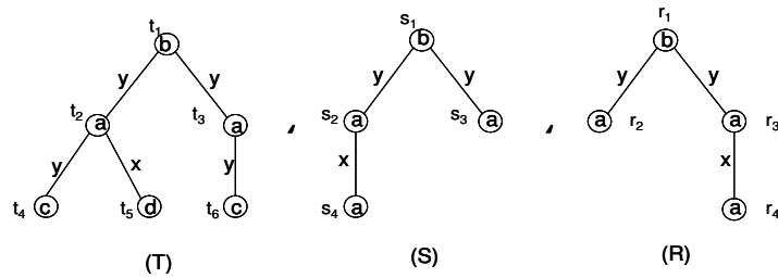
Figure 6.2: Example of three labeled ordered rooted trees and the order \succeq among such trees.
