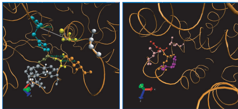
Figure 8.6: Left: Residues included in the patterns from PCP family in protein 1CQD. The residues in catalytic dyad CYS27-HIS161 are connected by a white dotted line and two important surrounding residues ASN181 and SER182 are labeled. Right: Residues included in patterns from the NB family in protein 1OVL. The labeled residue GLN 435 has direct interaction with the cofactor of the protein.
