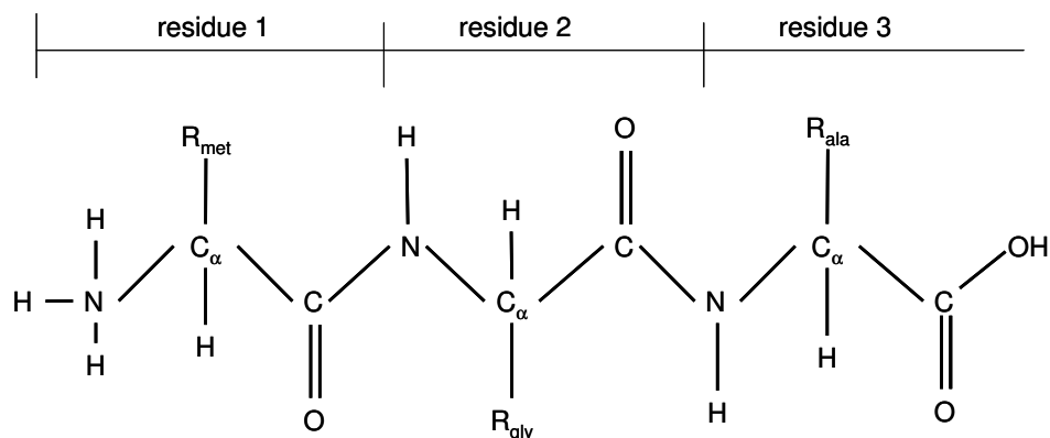
Figure 2.2: A schematic illustration of a polypeptide with three residues: Met, Gly and Ala. The peptide can also be described as the sequence of the three residues: Met-Gly-Ala.
