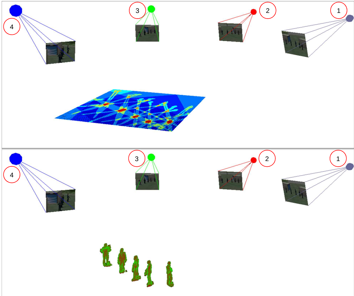
Figure 7.8: 3D reconstruction results using method from [Gua10]. Top: rendering of a single slice of the reconstructed volume showing occupancy probabilities. Bottom: rendering of 3D reconstruction results obtained by thresholding. Also shown are the poses and images of the cameras involved.
