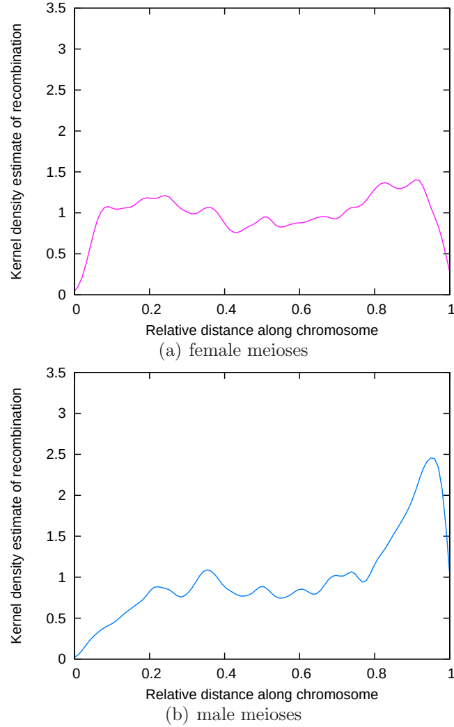
Figure 3.4: Distribution of recombination events along the autosomes in female and male meioses. The x-axis corresponds to the relative position in all autosomes. The y-axis indicates the kernel density estimates of recombinations in each type of meiosis.
