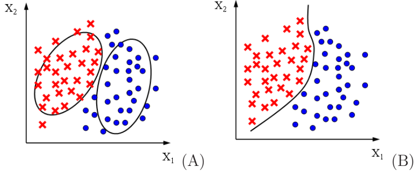
Figure 2.1: Generative learning v.s. discriminative learning for a two-class classification problem. (A) A generative model learns the data distribution of each individual class, where the distributions are represented as ellipses. (B) A discriminative model finds the boundary between the two classes.
