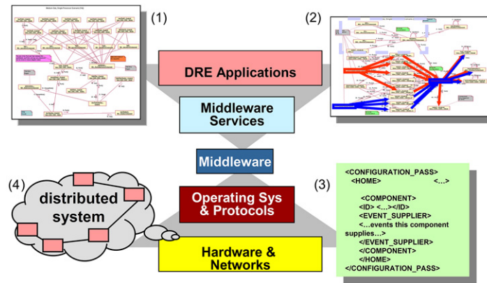
Fig. 7. Model driven middleware process.
