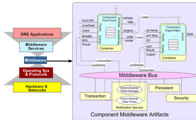
Fig. 2. Component middleware layers and architecture.
