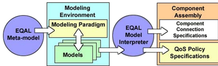
Fig. 12. The event QoS aspect language architecture.
