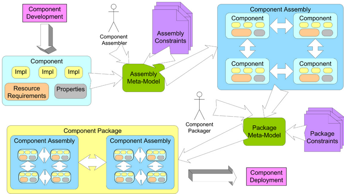
Fig. 10. Component packaging & application assembly.
