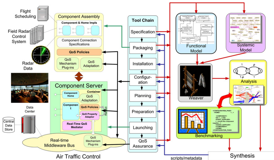
Fig. 8. CoSMIC model driven middleware toolsuite.
