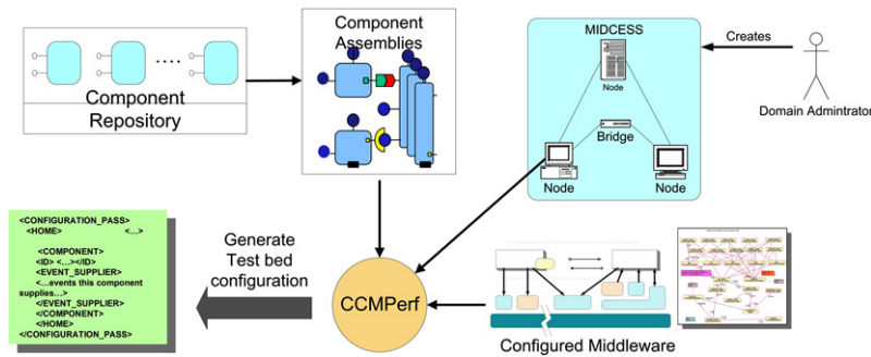
Fig. 13. Deployment planning process.
