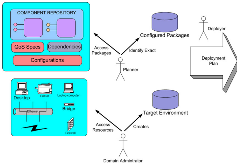
Fig. 6. Planning for deployment.
