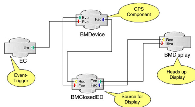
Fig. 14. Modeling component interaction using CCMPerf.
