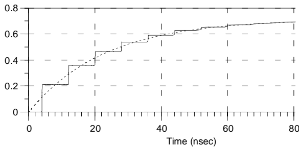
Figure 2: An 8mA CMOS Driver rings up a 4ns line terminated into 1KΩ.
