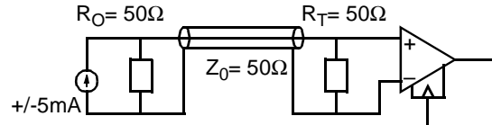
Figure 2: A low-swing, incident-wave signaling system.
