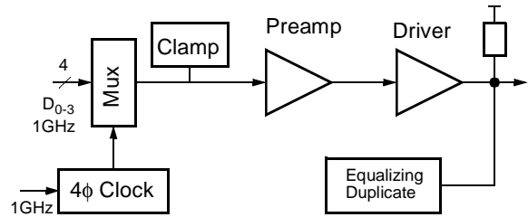
Figure 8: Input-multiplexed transmitter architecture with analog equalization
