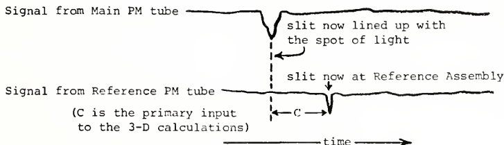
Fig. 3-3: Primary signals from the detector system
