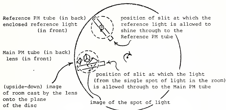
Fig. 3-2: Details of spinning disc detector
