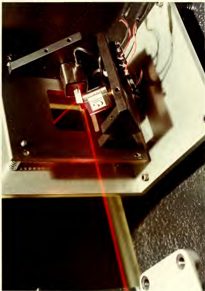
Fig. 3-4: The laser deflection system
