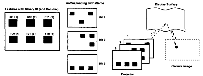
Figure 3: Binary encoded structured light scheme. (Left) Six binary encoded features and the corresponding bit patterns. (Right) Projected features are identified in the camera by their binary ID.
