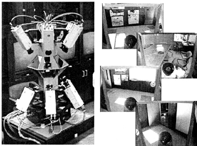
Figure 7: (Left) The Camera-Cluster (Right) Direct outputs of some of its twelve cameras
