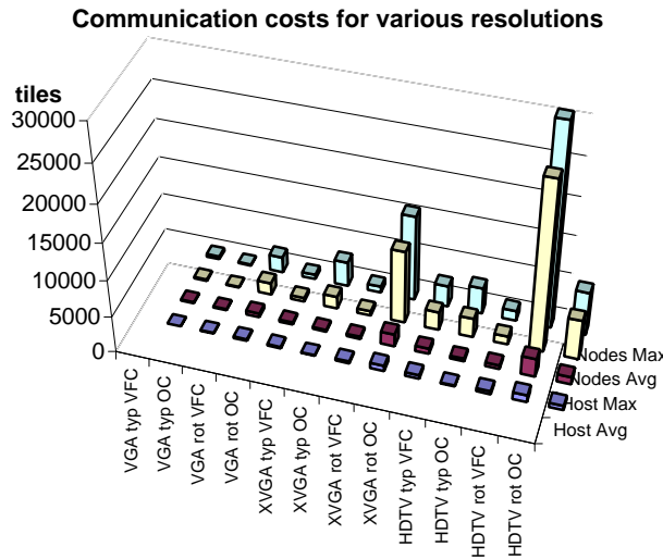
Graph 5.2. Maximum per frame communication volumes for various resolutions
