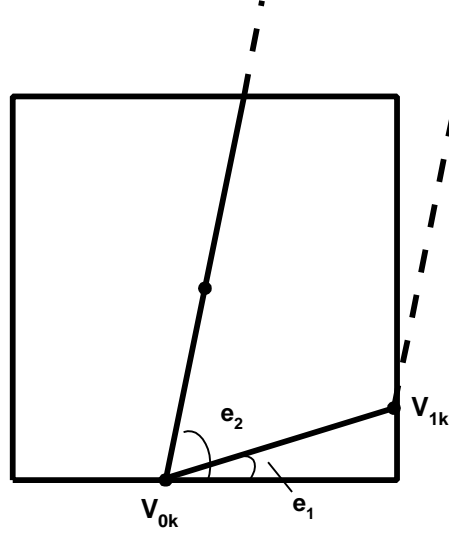
Figure 7.11. Position of sampling parallelogram that determines the maximum length of V_{0k}V_{1k} . V_{0k}V_{2k} is longer than 1 / \sin e_2 .
