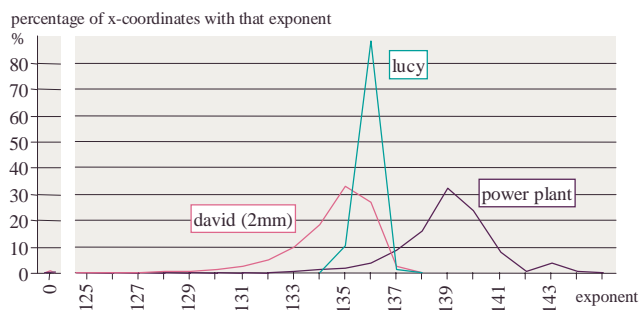
Fig. 5. The distribution of exponents among all x -coordinates for the david (2mm), the lucy, and the power plant model as percentages of the total. The power plant’s exponents of 143 belong to a building situated far from the main complex.
