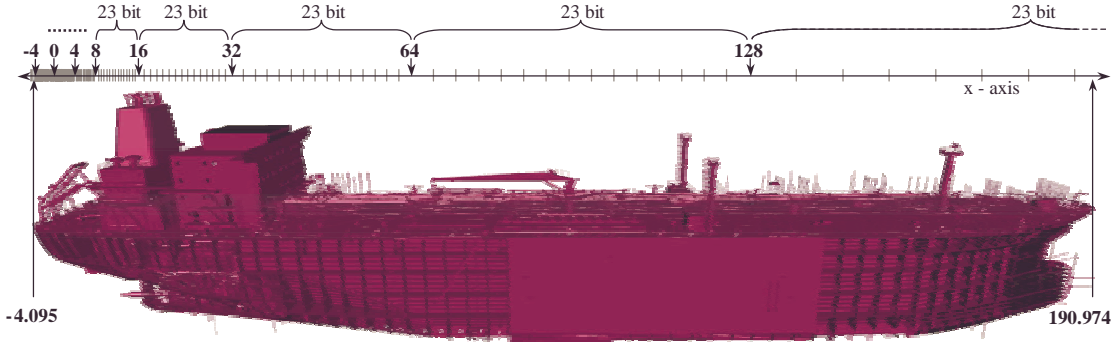
Fig. 1. The x -coordinates of this 75 million vertex Double Eagle tanker range from -4.095 to 190.974 . The coordinates above 128 have the least precision with 23 mantissa bits covering a range of 128. There is sixteen times more precision between 8 and 16, where the same number of mantissa bits only have to cover a range of 8.
