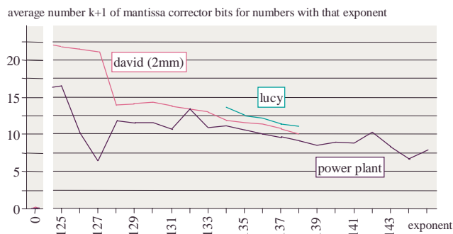
Fig. 6. The average number of significant corrector bits k + 1 that need to be compressed during predictive coding of the mantissas of all x -coordinates with the same exponent. Predictions for numbers with high exponents are evidently better since they result in correctors with fewer significant bits.
