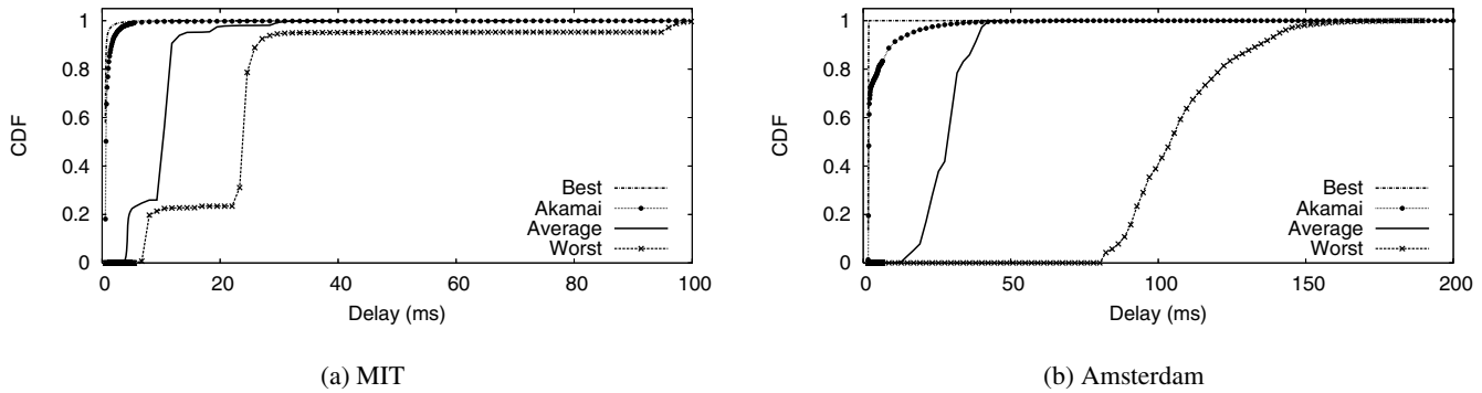
Figure 9: CDF of RTTs for Akamai paths for two PL nodes.
