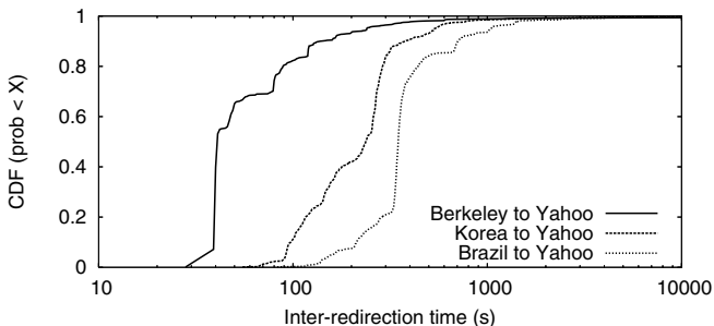
Figure 5: Redirection dynamics from three representative nodes.
