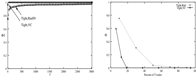
Figure 7: 1997 Internet AS topology. Left: \Phi_3(\tau) . Right: \Theta as a function of |T| .
