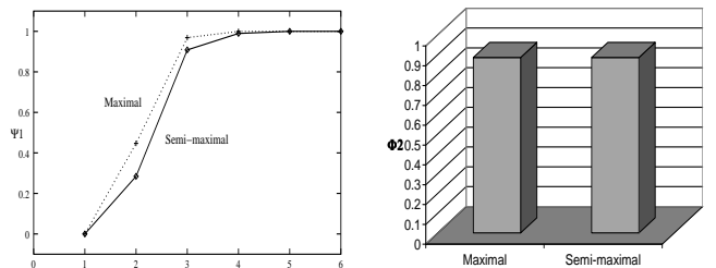
Figure 10: 1997 Internet AS topology. Left: Comparison of \Psi_1(\tau) for maximal and semi-maximal filters. Right: Corresponding comparison of \Phi_2(1) .
