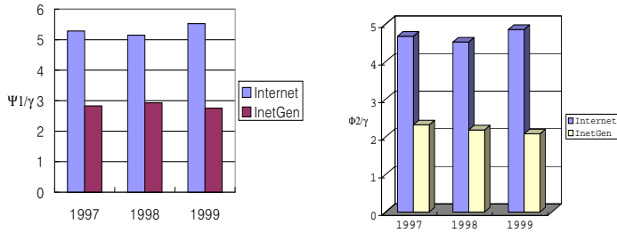
Figure 14: Left: Performance difference between Inet and Internet AS graphs normalized by VC size: \Psi_1(5)/(|VC|/n) . Right: Corresponding comparison of normalized \Phi_2(1) = \Phi_2(1)/\gamma .
