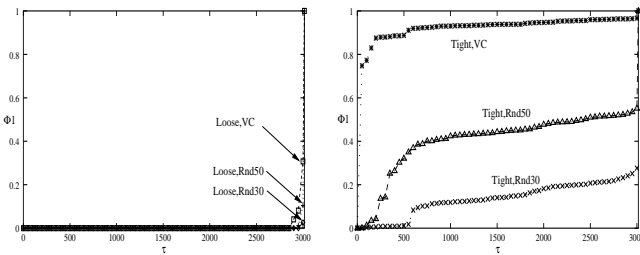
Figure 3: 1997 Internet AS topology. Left: \Phi_1(\tau) for R = loose . Right: \Phi_1(\tau) for R = tight .
