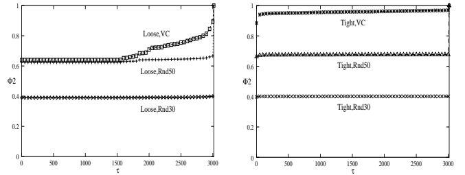
Figure 5: 1997 Internet AS topology. Left: \Phi_2(\tau) as a function of \tau for R = loose . Right: Corresponding graph for R = tight .
