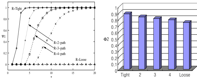
Figure 17: Effect of multi-path routing for 1997 Internet AS topology. Left: \Psi_1(\tau) . Right: \Phi_2(1) for R from tight to loose .
