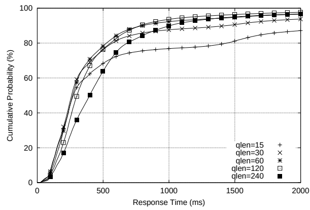
(b) 90% load
