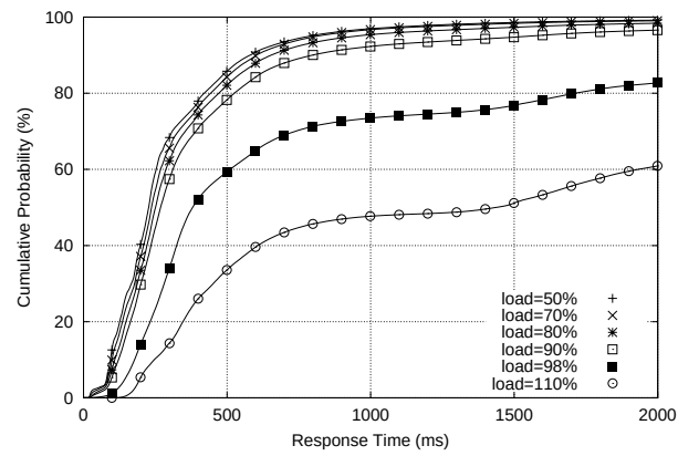
(a) qlen = 60
