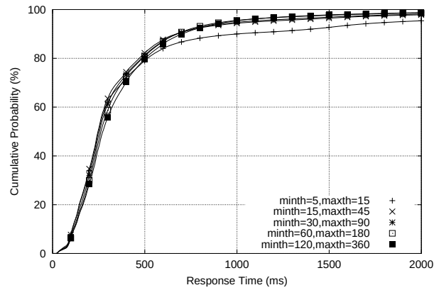
(c) load = 80%
