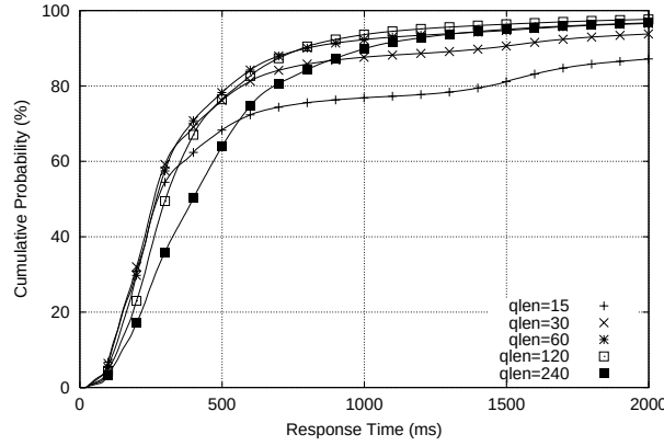
Figure 5.2: Tail-drop performance at 90% load.
