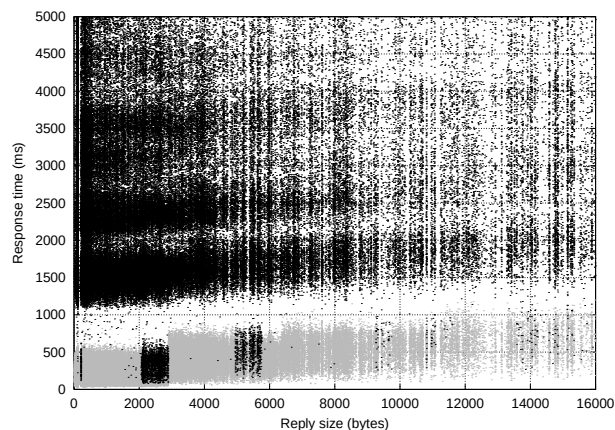
Figure 6.4: Scatter plot of response times versus reply size under RED for (min_{th}, max_{th}) = (5, 15) . Flows with no retransmissions are marked with gray dots, while flows with retransmissions are marked with black dots.
