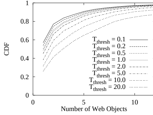
Figure 3.5: Cummulative Distribution Functions (CDFs) of Document Length in Objects, 19 September 1995. Curves correspond to varying of T_{thresh} in seconds [40].
