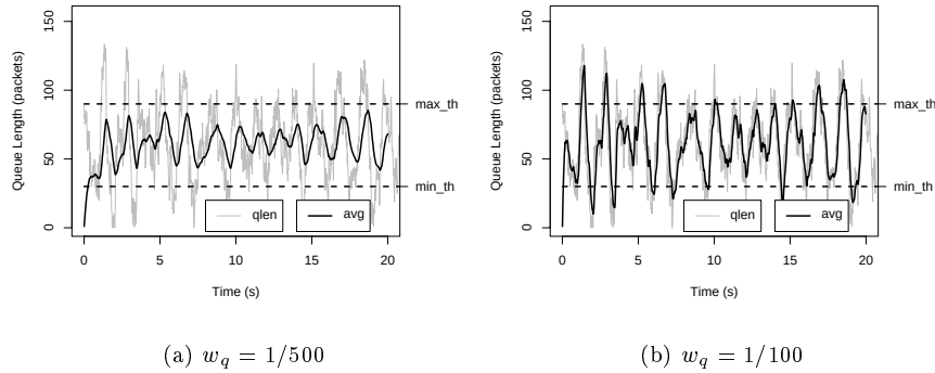
Figure 2.3: Two plots showing the effect of w_q on the weighted average queue length.
