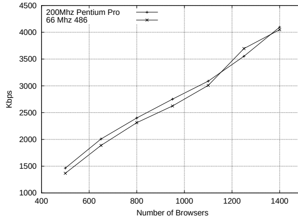
Figure 3.15: Browser program test.
