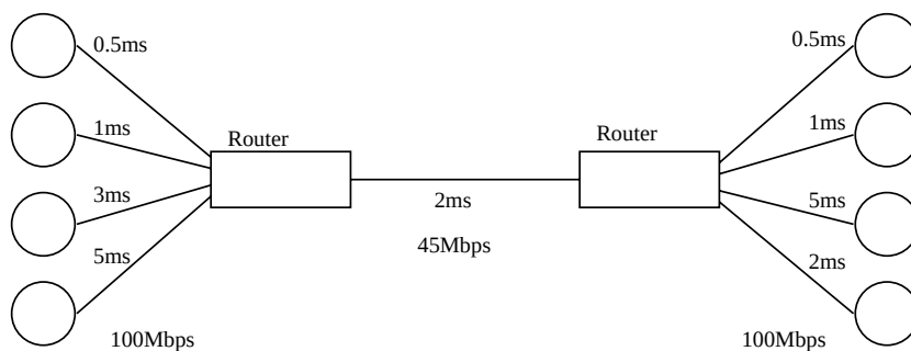
Figure 2.7: Simulation network for studying effects of heavy congestion.
