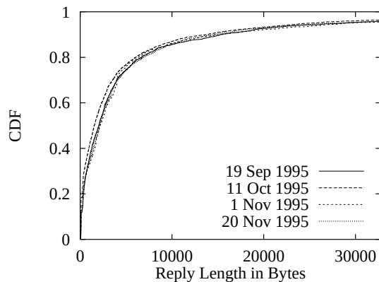
(a) CDFs of HTTP Reply Lengths [40]
