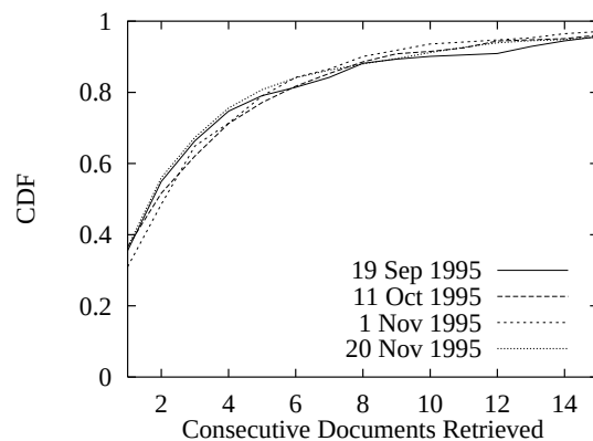
Figure 3.7: CDFs for consecutive document retrievals for all traces [40].
