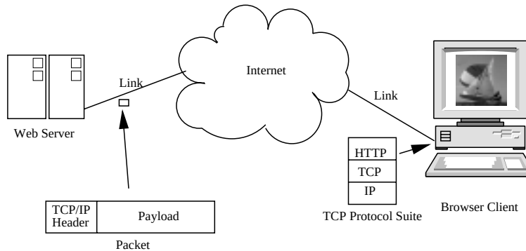
Figure 1.1: Internet Connection: A Web server and a browsing client are connected to the Internet through physical links. Each host has a protocol suite for communicating and data is transmitted as packets.
