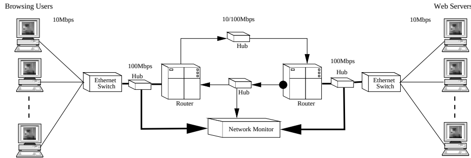
Figure 6.1: Laboratory network with additional instrumentation.
