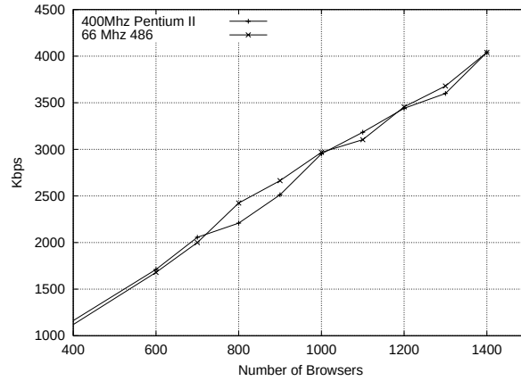
Figure 3.16: Server program test.
