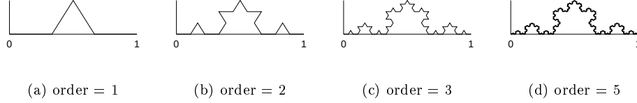
Figure 3.2: von Koch curves from 1 to 5 iterations.
