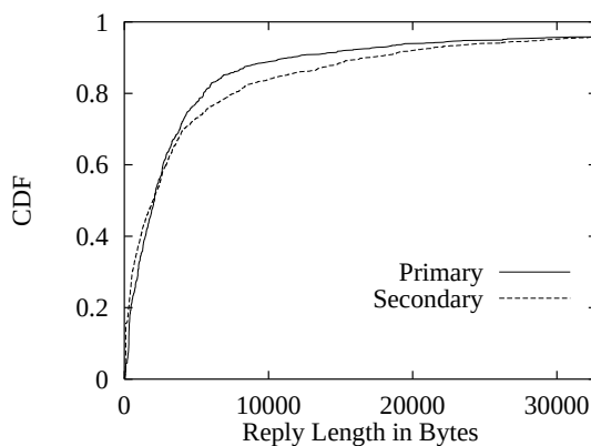
(b) CDF of primary and secondary reply lengths, 19 September 1995 [40]
