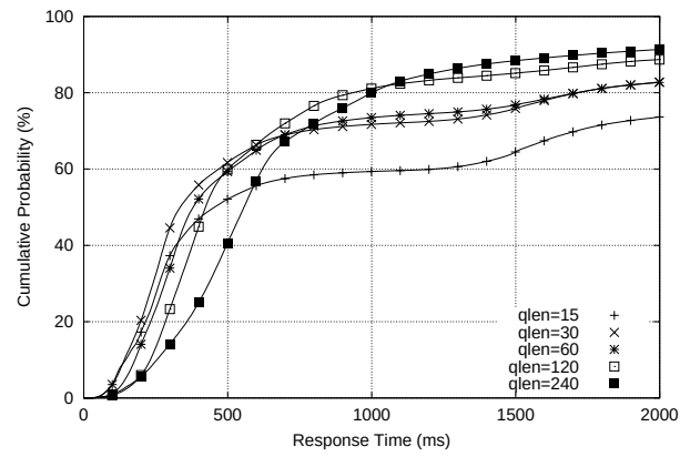
(a) 98% load
