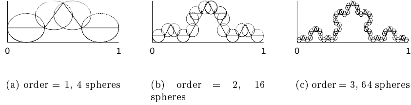
Figure 3.3: Covering von Koch curves with spheres.
