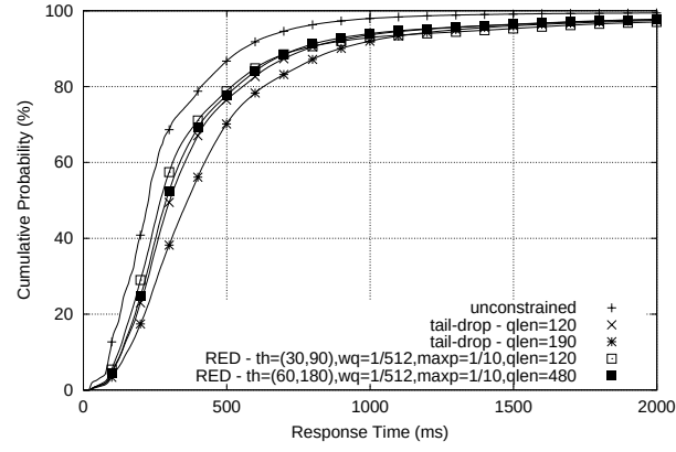
(a) 90% load
