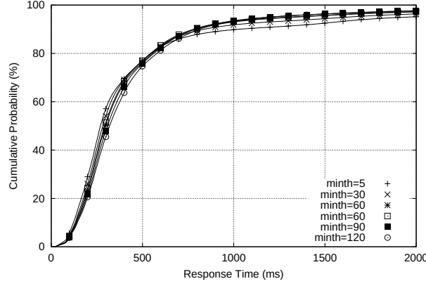
Figure 5.8: The effect of changing min_{th} . Load = 90% and max_{th} = 90 , w_q = 1/512 , max_p = 1/10 , and qlen = 480 .
