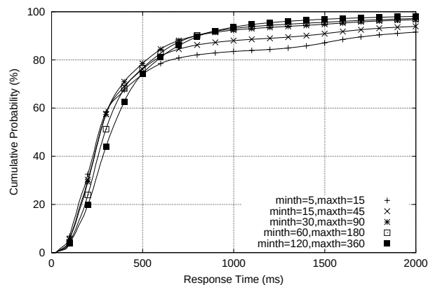
(a) 90%
