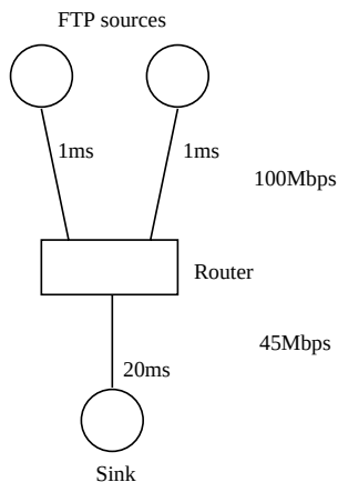
Figure 2.6: Simulation network for the RED and tail-drop comparison: Two FTP sources with equal round trip times, but on separate 100Mbps links send data to a sink through a router. The link from the router to the sink is a 45Mbps link with a 20ms delay.
