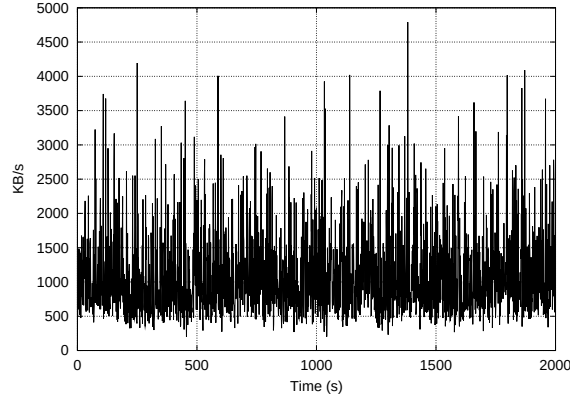
Figure 3.13: Requested KB per second.
