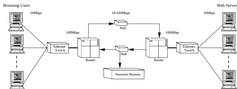
Figure 3.11: Diagram of the laboratory network.
