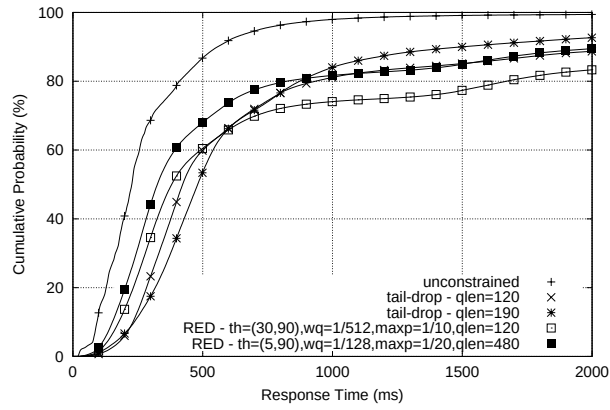
(b) 98% load
