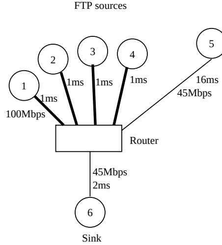
Figure 2.8: Network topology used for fairness testing.
