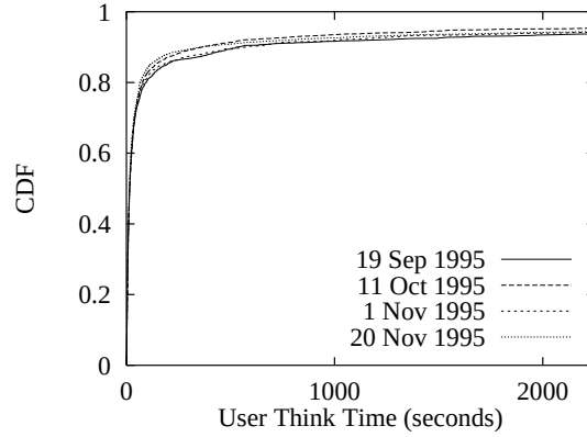
Figure 3.6: CDF of user think times for all traces [40].
