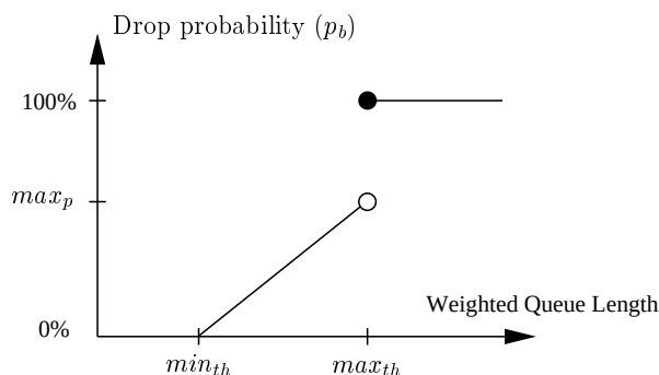
Figure 2.4: RED drop probability dependence on parameters.
