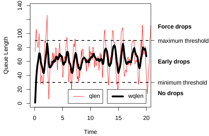
Figure 1.4: Illustration of RED in operation.
