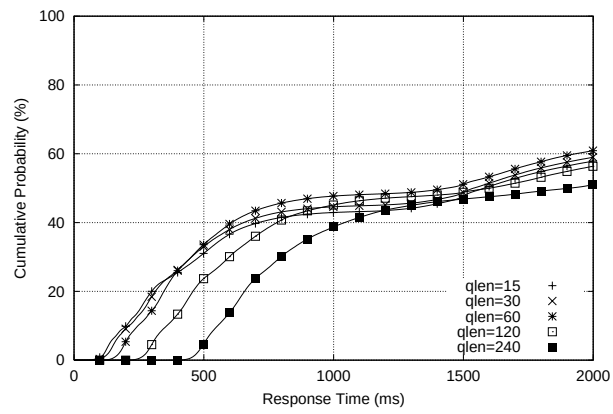
(b) 110% load
