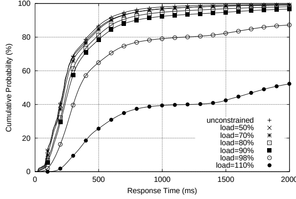
Figure 5.6: The performance of RED at different loads. w_q = 1/512 , max_p = 1/10 , min_{th} = 30 , max_{th} = 90 , and qlen = 480 .
