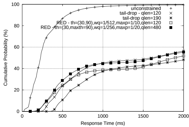
(c) 110% load
