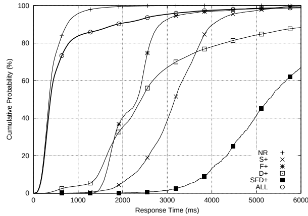
(b) (min_{th}, max_{th}) = (60, 180)
