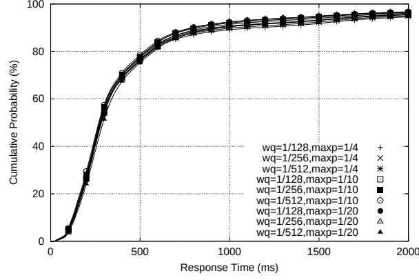
(a) 90% load
