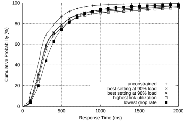
(a) 90% load
