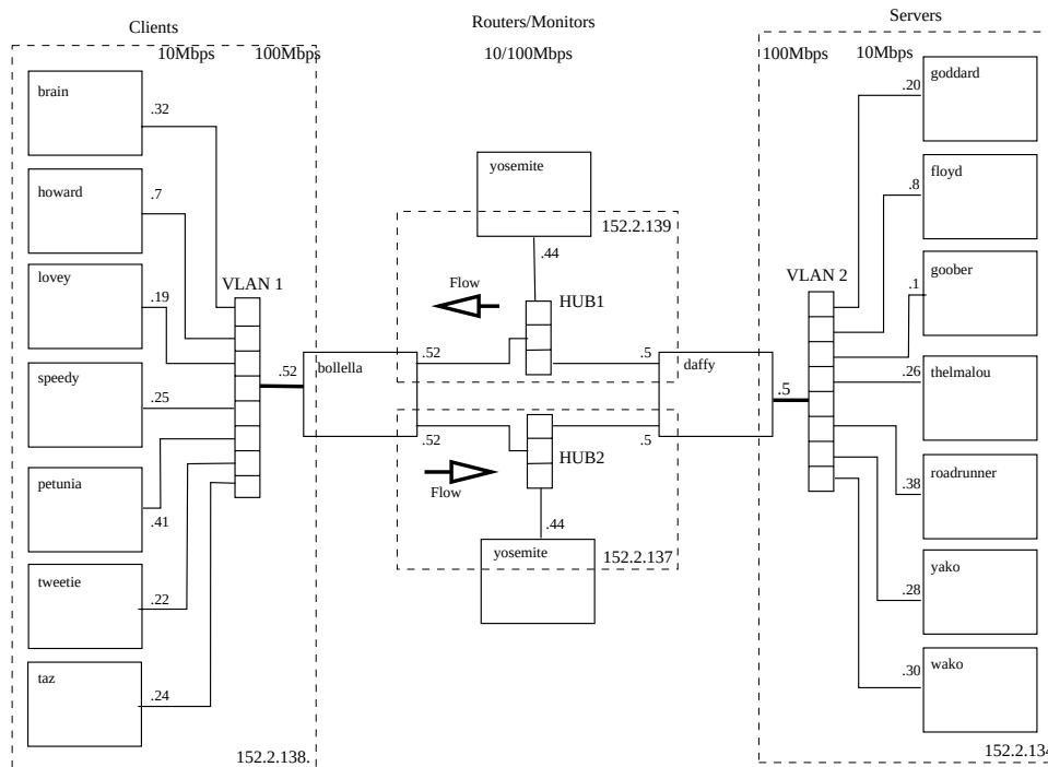
Figure A.1: Detailed diagram of laboratory network.
