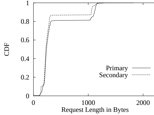
(b) CDF of primary and secondary request lengths, 19 September 1995 [40]
