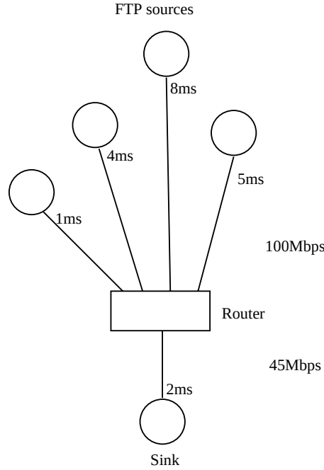
Figure 2.5: Simulation network for the average queue size test: Four FTP sources each on a separate 100Mbps link and with different round trip times send data to a sink through a router. The link from the router to the sink is a 45Mbps link with a 2ms delay.
