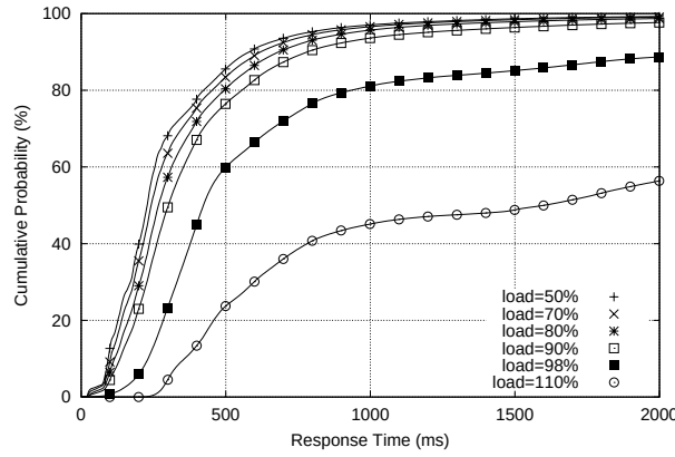
Figure 5.5: Tail-drop performance for different loads with a queue length of 120 elements.
