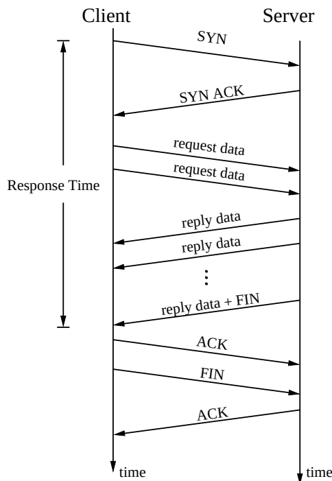
Figure 3.10: Message sequence chart of a Web object request.
