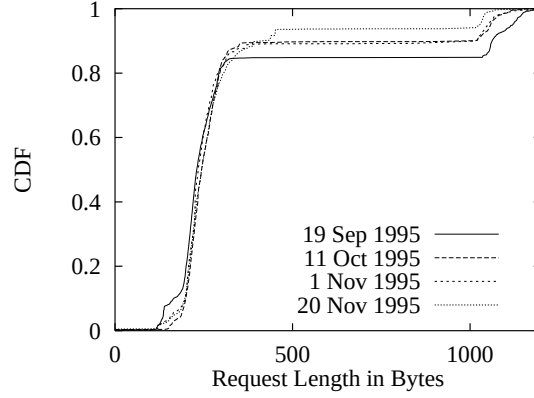
(a) CDFs of HTTP Request Lengths [40]
