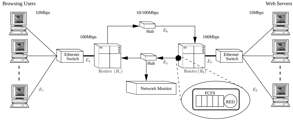
Figure 4.2: Laboratory network. Each Ethernet segment is labeled E_1 to E_6 , and routers are labeled with R_1 and R_2 .
