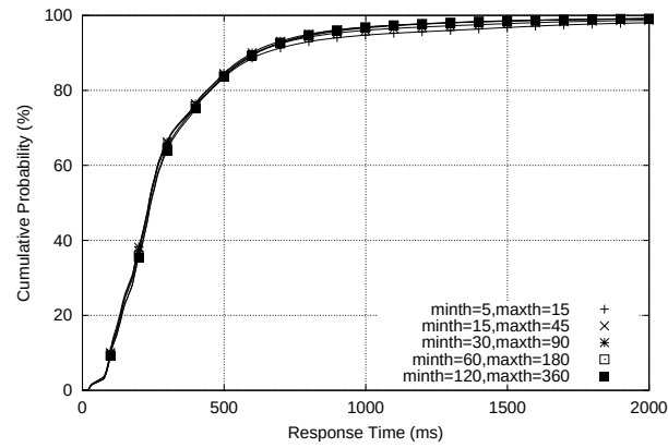
(b) load = 70%
