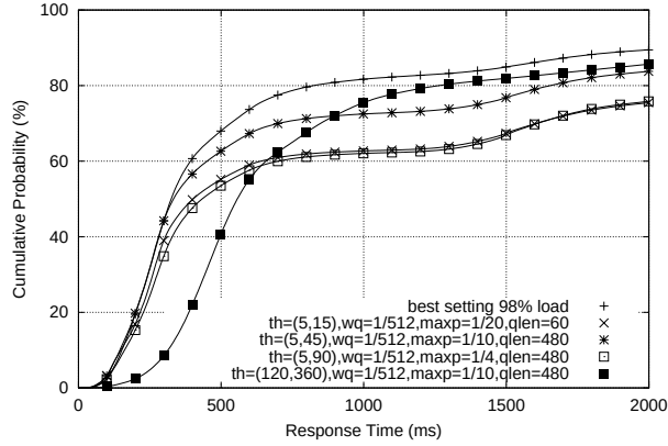
(b) 98% load
