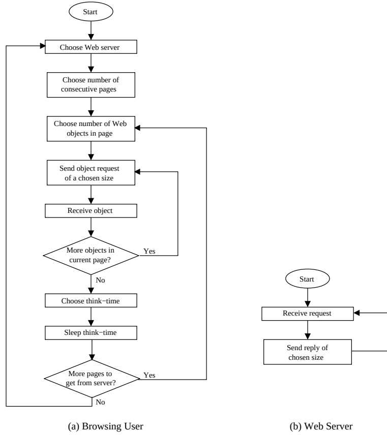
Figure 3.4: Flow diagram of Mah's HTTP traffic model.
