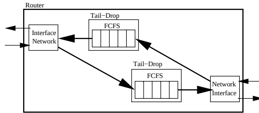
Figure 1.2: An Internet Router.
