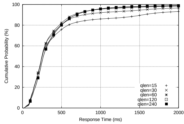
(a) 80% load
