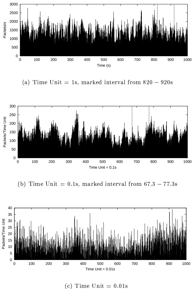
Figure 6.7: Behavior on the unconstrained network at 9.8Mbps load.
