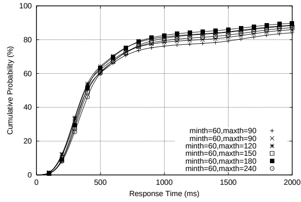
(b) \min_{th} = 60
