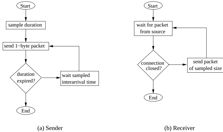
Figure 3.1: Flow chart of a TELNET connection.
