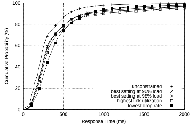
(a) Load = 90%
