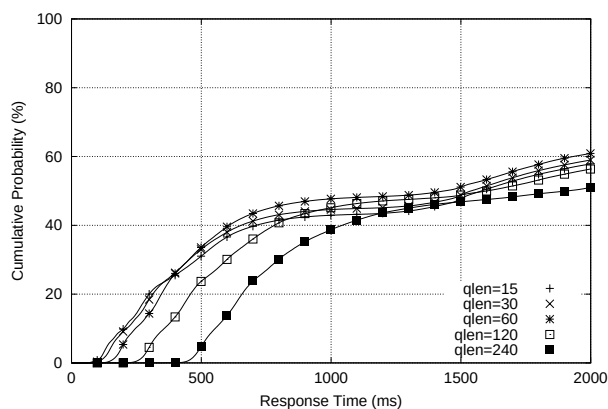
Figure 5.4: Tail-drop performance at 110% load.
