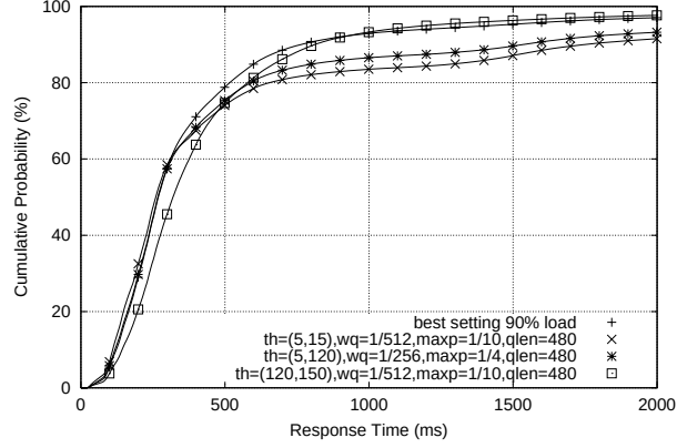
(a) 90% load
