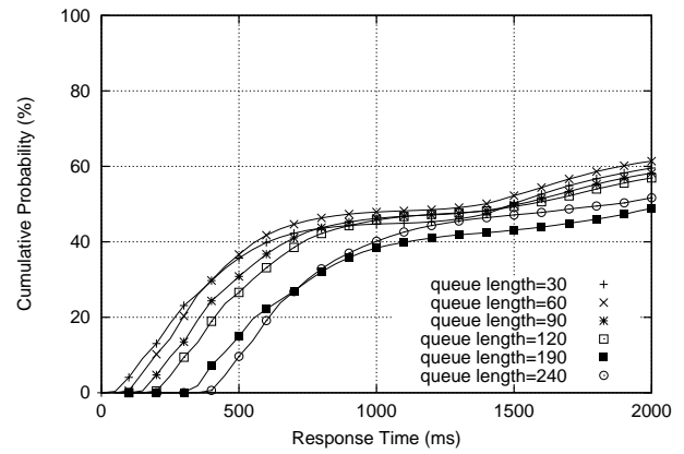
Figure 7d: FIFO performance at 110% load.
