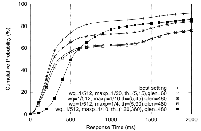
Figure 14b: “Bad” RED parameters settings at 98% load.
