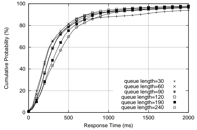
Figure 7b: FIFO performance at 90% load.
