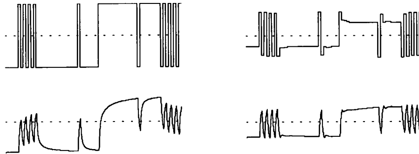
Figure 6: Response of equalizing filter to waveform from Figure 1. The left panel repeats Figure 1 showing the original 4Gb/s signal and the received waveform after a 6m 30AWG line without equalization. The right panel shows the signal after being equalized (top) and the resulting received waveform (bottom).
