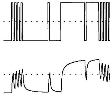
Figure 1: Frequency dependent attenuation causes intersymbol interference. This figure shows a simulation of a 4Gb/s signal passed through a 6m 30AWG line. An isolated high-frequency pulse barely reaches the midpoint of signal swing because of interference from unattenuated low-frequency components of the signal.
