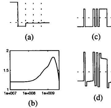
Figure 4: Impulse response (a), frequency response (b), and response (d) to an example sequence (c) of a five-tap FIR equalizing filter matched to 6m of 30AWG 100Ω line.
