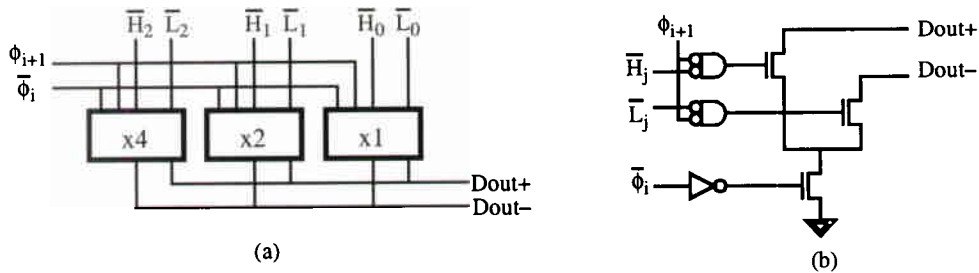
Figure 8: Circuit design for a DAC module – (a) three pulse generators are enabled by the H and L signals and gated by two clocks to generate a precise 250ps pulse with one of 15 selectable current levels, (b) each of the three generators is implemented with a qualifying pre-driver followed by a series final driver that shares a common tail transistor.
