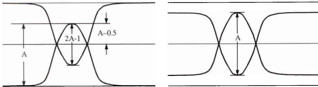
Figure 3: Without equalization (left), attenuating high-frequency components by a factor A reduces the height of the data eye by a factor of 2A-1 and also reduces the width of the eye. With equalization (right) the height of the eye is reduced by a factor of A and the width of the eye is unaffected.
