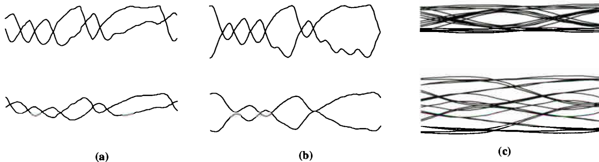
Figure 9: Simulation Results - (a) simulated waveforms with equalization on, top trace is at transmitter, bottom trace is at receiver, (b) waveforms with equalization off, (c) differential eye diagrams of received waveform with equalization (top) and without (bottom).
