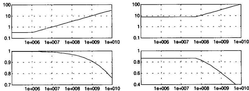
Figure 2: Resistance (top) and attenuation (bottom) curves for 1m of 30AWG 100Ω twisted pair (left) and 1m of 5mil 0.5oz 50Ω stripguide (right).
