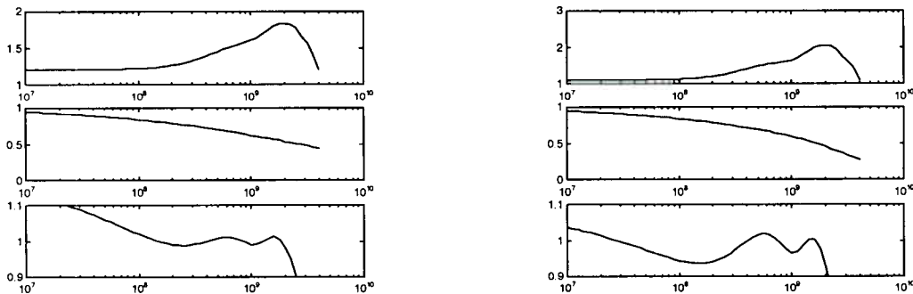
Figure 5: Frequency response of filter (top), line (middle) and combination (bottom) for 6m of 30AWG cable (left) and the same cable followed by a 1pF load resistor (right).
