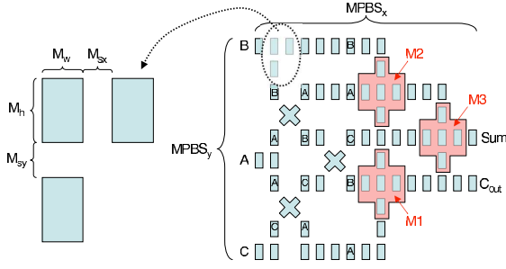
Figure 6: Magnet Adder.
