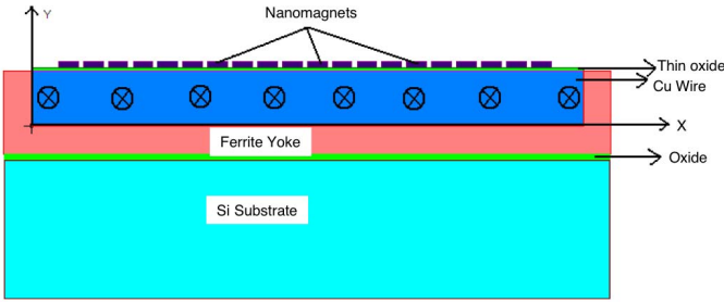
Figure 3: Cross section of the clocking structure.
