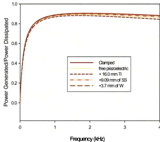
Figure 9. The power transfer efficiency calculated by maximizing the power at 1 kHz for various harvester configurations. The slight drop away from 1 kHz is due to the change in the source impedance with frequency. We have essentially tuned to match at 1 kHz.
