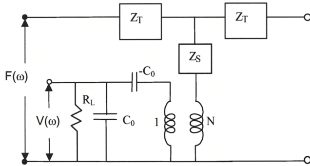
Figure 3. Circuit model of a basic piezoelectric energy harvesting systems. a) A structure applies a harmonic Force F(\omega) to the surface of a piezoelectric material which is clamped on the opposite side.
