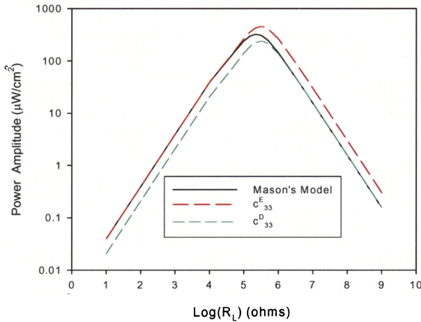
Figure 7. The log of power amplitude as a function of the log of the load resistance R_L for the clamped piezoelectric with material properties and geometry shown in Table 2. The force was 50 N and the frequency 1 kHz.
