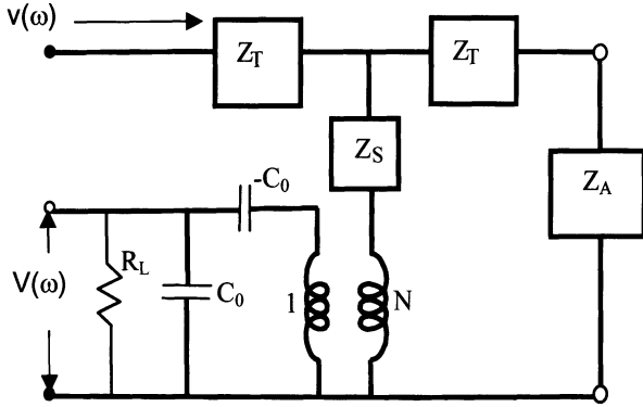
Figure 6. Circuit model of a piezoelectric energy harvesting system. A structure applies a harmonic velocity v(\omega) to the surface of a piezoelectric material which has a reaction mass m on opposite surface.
