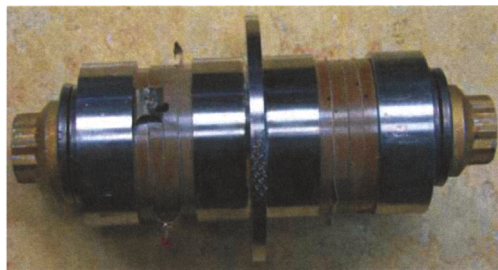
Figure 13. A photograph of a high power acoustic electric feed-through prototype. The final design had six piezoelectric rings.
