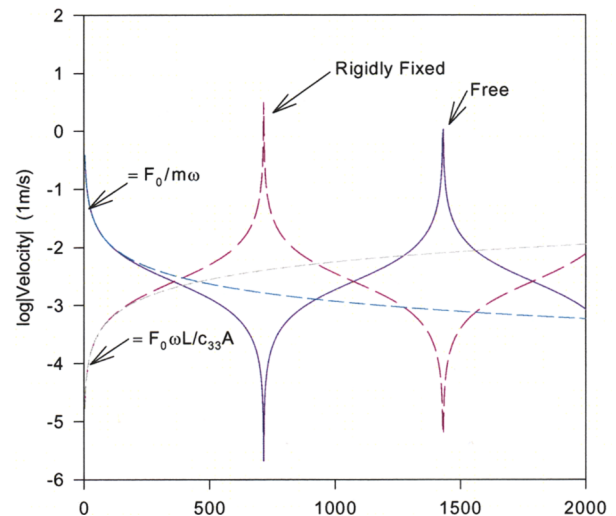
Figure 5. The amplitude of the input velocity for a harmonic force with amplitude F_0 for the acoustic layer shown in figure 4 in the stress free and clamped condition.
