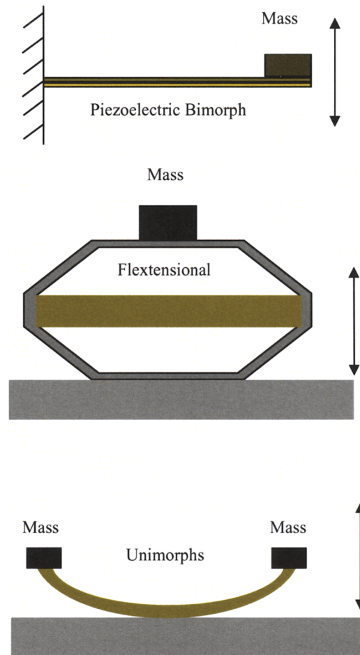
Figure 11. Low resonance frequency piezoelectric transducers.
