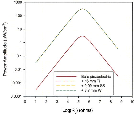
Figure 8. The power density as a function of the load resistance on the electrical port for a bare 2 mm piezoelectric and a piezoelectric with various materials of lengths as shown in Table 3.
