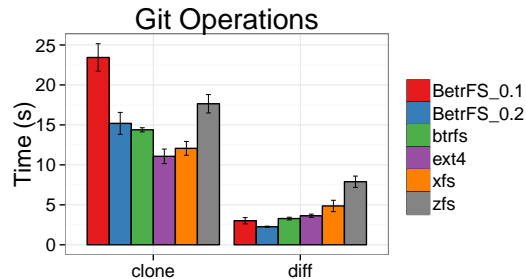
(c) Git operations. The BetrFS source repository was git-cloned locally, and a git-diff was taken between two milestone commits. Lower is better.
