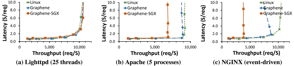
Figure 5: Throughput versus latency of web server workloads, including Lighttpd, Apache, and NGINX, on native Linux, Graphene, and Graphene-SGX. We use an ApacheBench client to gradually increase load, and plot throughput versus latency at each point. Lower and further right is better.
