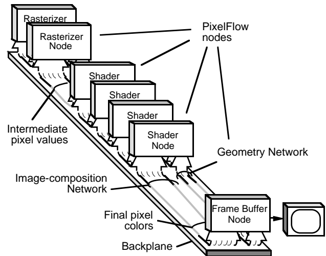
Figure 4: PixelFlow system block diagram.
