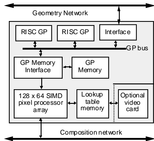
Figure 5: PixelFlow node block diagram
