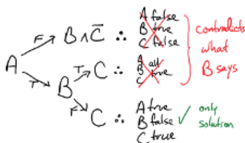
Figure 2.2: A decision tree
