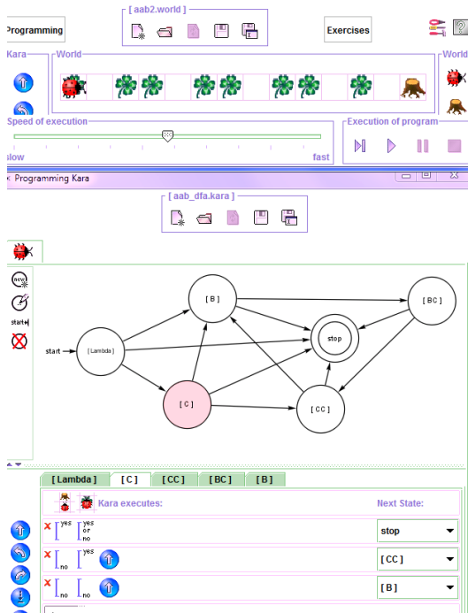
Figure 12.2: Kara program to recognize the language of substrings of \{\text{clover clover blank}\}^* . A string is in the language iff Kara stops without crashing.
