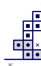
Figure 10.2: Placing zigs along right wall
