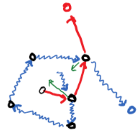
Figure 13.11: Red and blue intersecting twice.
