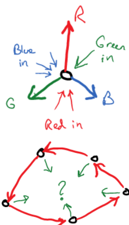
Figure 13.10: Showing that red cycles are impossible
