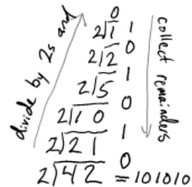
Figure 7.1: Decimal to binary: remainders on dividing by 2.
