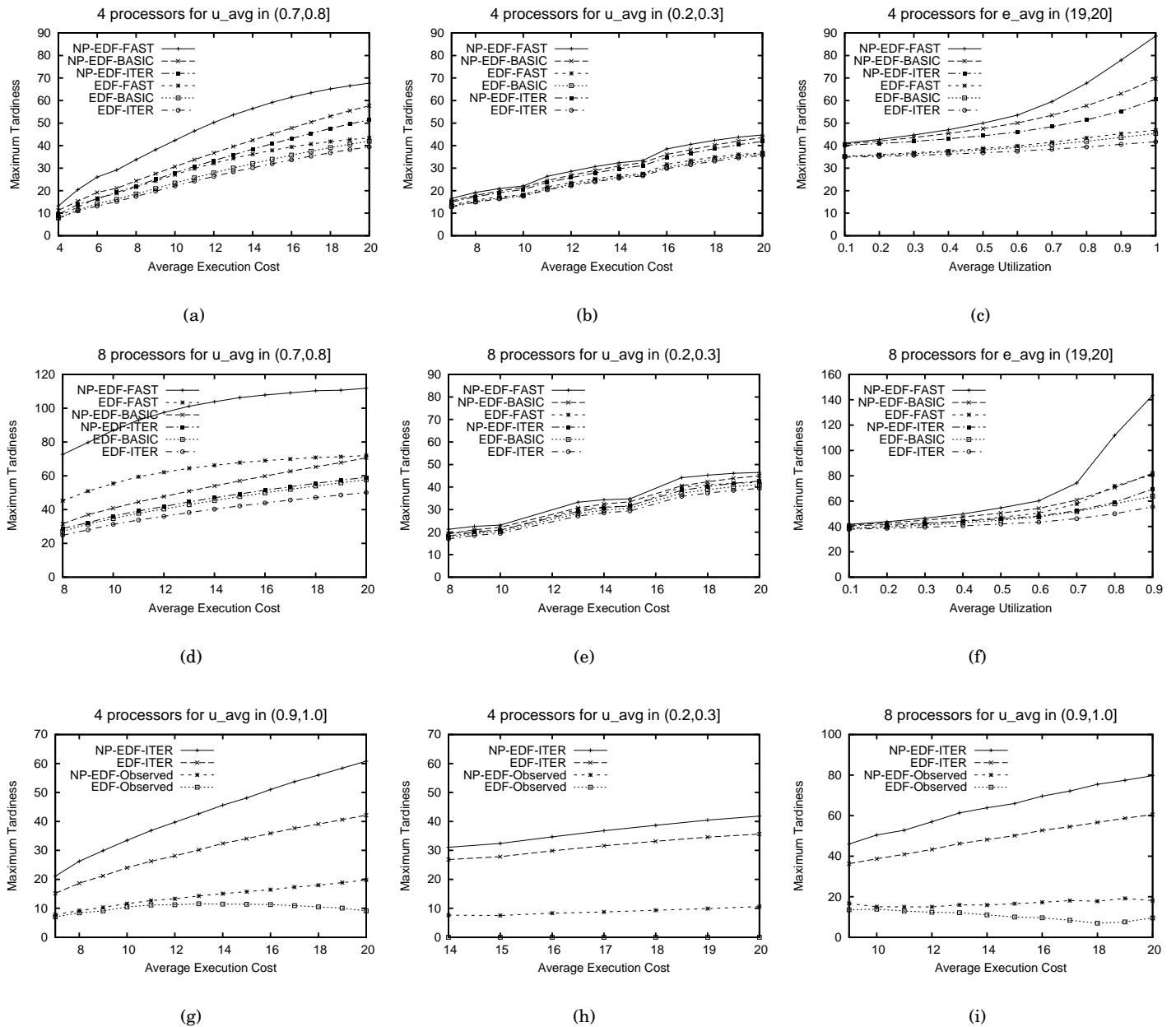
Figure 5: Comparison of the three bounds derived for EDF and NP-EDF for (a)–(c) m = 4 and (d)–(f) m = 8 . Tardiness bounds as a function of e_{avg} for (a) & (d) 0.7 < u_{avg} \leq 0.8 , and for (b) & (e) 0.2 < u_{avg} \leq 0.3 , and as a function of u_{avg} for (c) & (f) 19 < e_{avg} \leq 20 . Comparison of EDF-ITER and NP-EDF-ITER to tardiness observed in actual EDF and NP-EDF schedules for (g) & (h) m = 4 , and for (i) m = 8 . (The order of the legends and curves coincide in all the graphs.)
