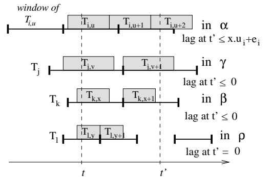
Figure 2: Lemma 3. Partitioning of tasks in \tau . Jobs of a sample task in each subset are shown. In this figure, all jobs except those of T_i , which is in \alpha , complete executing by their deadlines.
