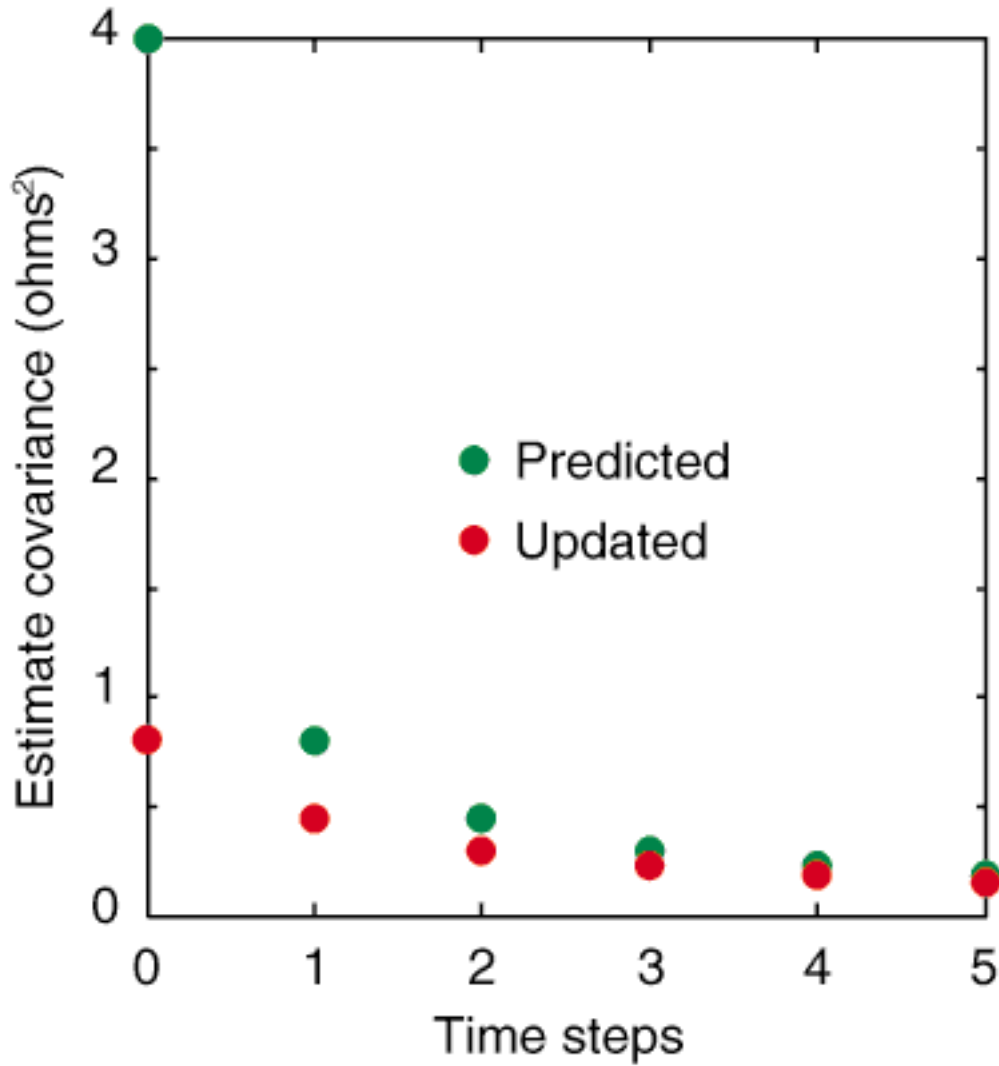
Figure 4. Initially, the predicted uncertainty (variance) of the resistor's value is 4 ohms 2 and is simply based on the manufacturer-provided tolerance value. However, after six measurements, the estimated variance drops to below 0.2 ohms 2 .
