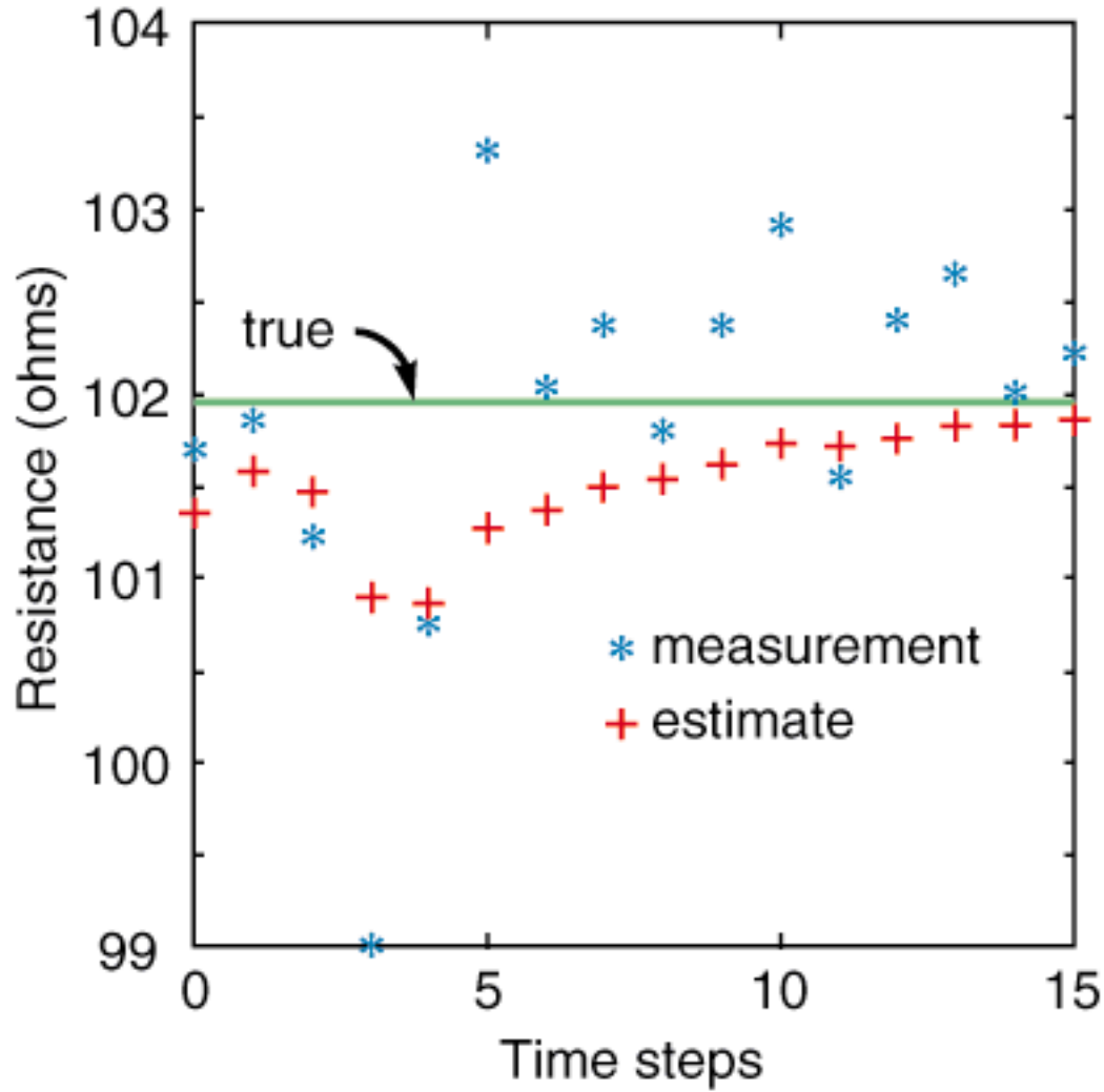
Figure 3. The individual resistance measurements of a nominally 100-ohm resistor are scattered about the true value of slightly less than 102 ohms. The Kalman filter estimate gradually converges to this value.
