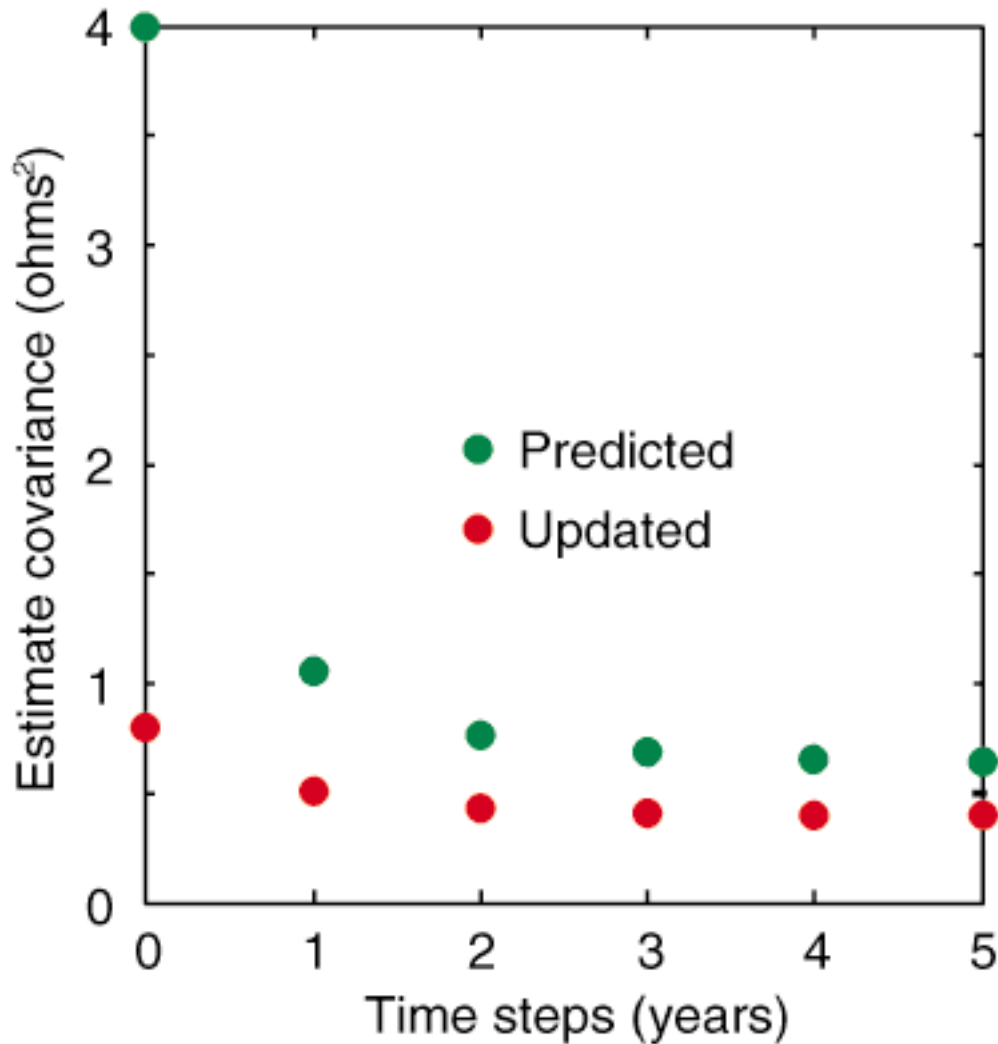
Figure 5. The true resistance of a resistor in an environment with a widely varying temperature is not quite constant. If this is modeled assuming a variation with an average of zero and a variance of 0.25 ohms 2 , the Kalman filter estimate of the resistance variance converges to 0.4 ohms 2 after only a few measurements.
