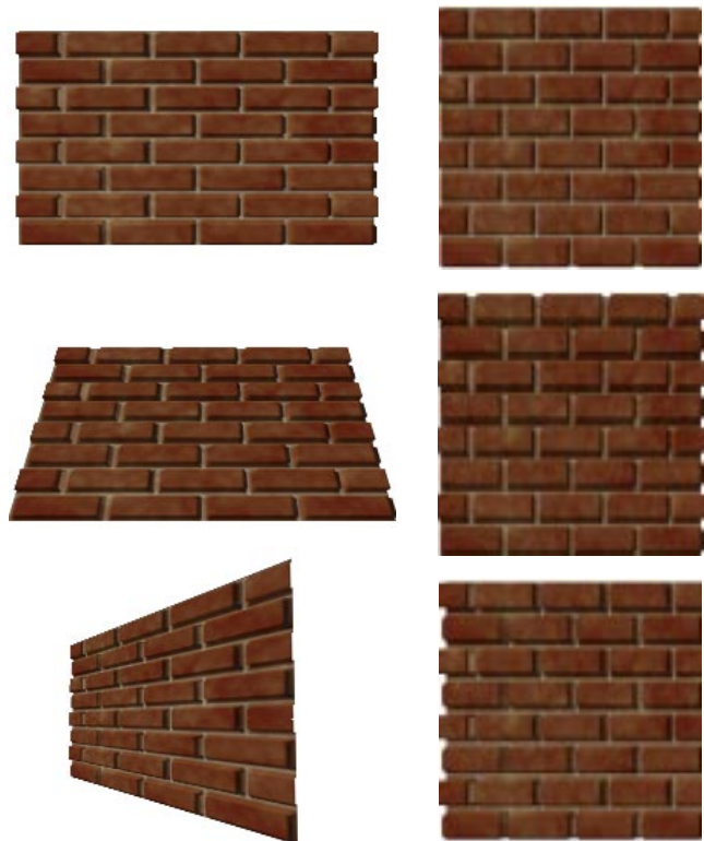
Figure 21. Three views of a relief texture-mapped brick wall. The images on the left show one quadrilateral texture-mapped with the corresponding pre-warped images shown to the right. Brick texels have zero displacement and, therefore, do not move.
