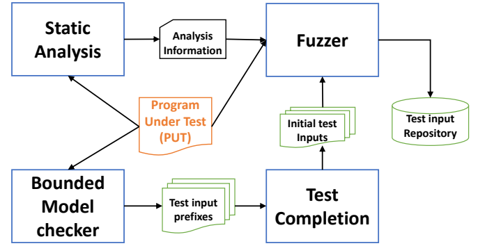
Fig. 3: BMCFuzz Implementation Architecture
