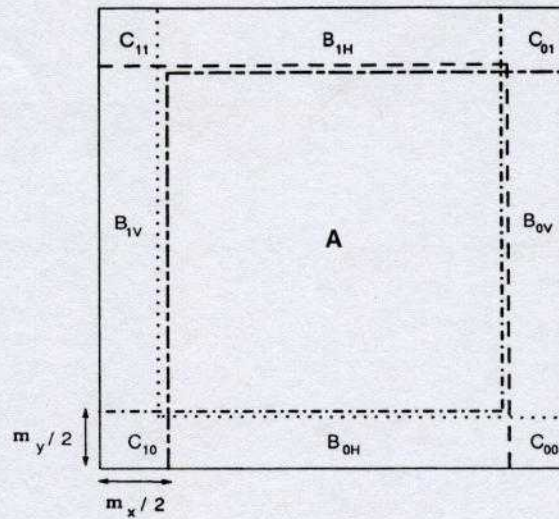
FIG. 5. The image area divided into the mosaic images M_{00} (---), M_{01} (···), M_{10} (—), and M_{11} (---), their common center area A , their border regions, B_{kH} and B_{kV} , and the corner regions C_{kl} .
