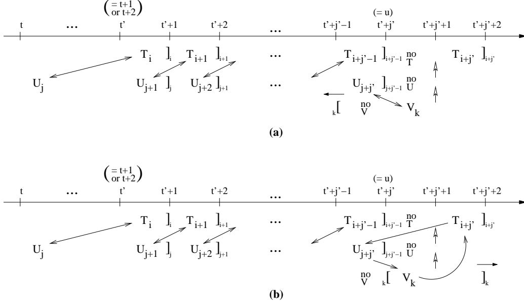
Fig. 16. Case 4 (continued). (a) D(T_i) = D(U_j) and r(V_k) < t' + j' . (b) D(T_i) = D(U_j) , r(V_k) = t' + j' , and V \notin S'_{t'+j'+1} .
