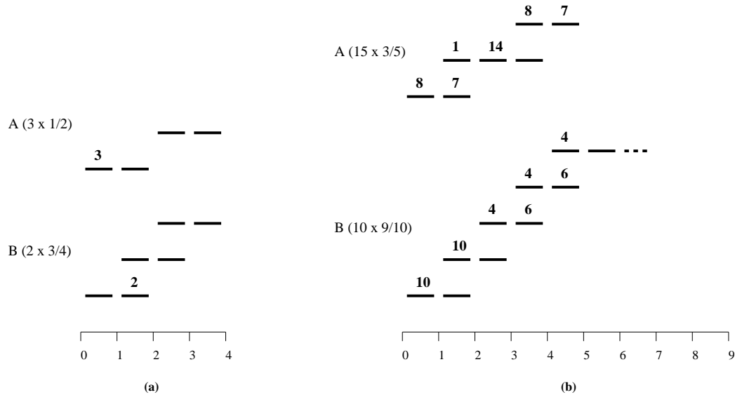
Fig. 8. (a) Theorem 7. (b) Theorem 8.
