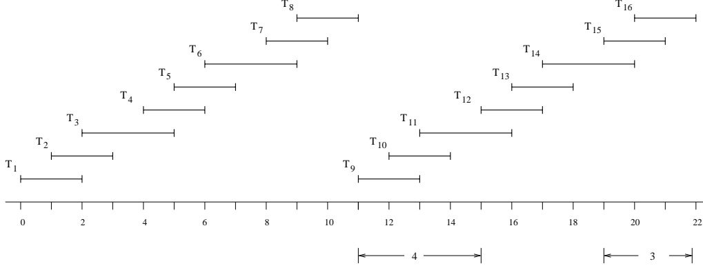
Fig. A.1. Windows of a task T of weight 8/11 are shown. Sample values of t' , t , u , and u' (from Claim 24) are 11, 15, 19, 22.
