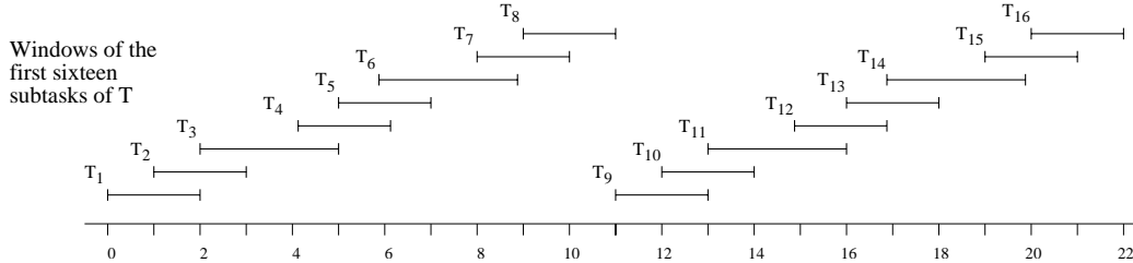
Fig. 2. The Pfair windows of the first two jobs (or sixteen subtasks) of a task T with weight 8/11 in a Pfair-scheduled system. During each job of T , each of the eight units of computation must be allocated processor time during its window, or else a lag-bound violation will result.
