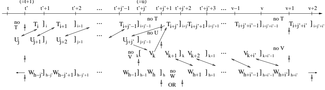
Fig. 21. Subcase 4.B (continued). d(W_h) = u + 1 , W \in S_{u-1} , and W 's most recent group deadline before the one at u + 1 or u + 2 is at or before t + 1 .
