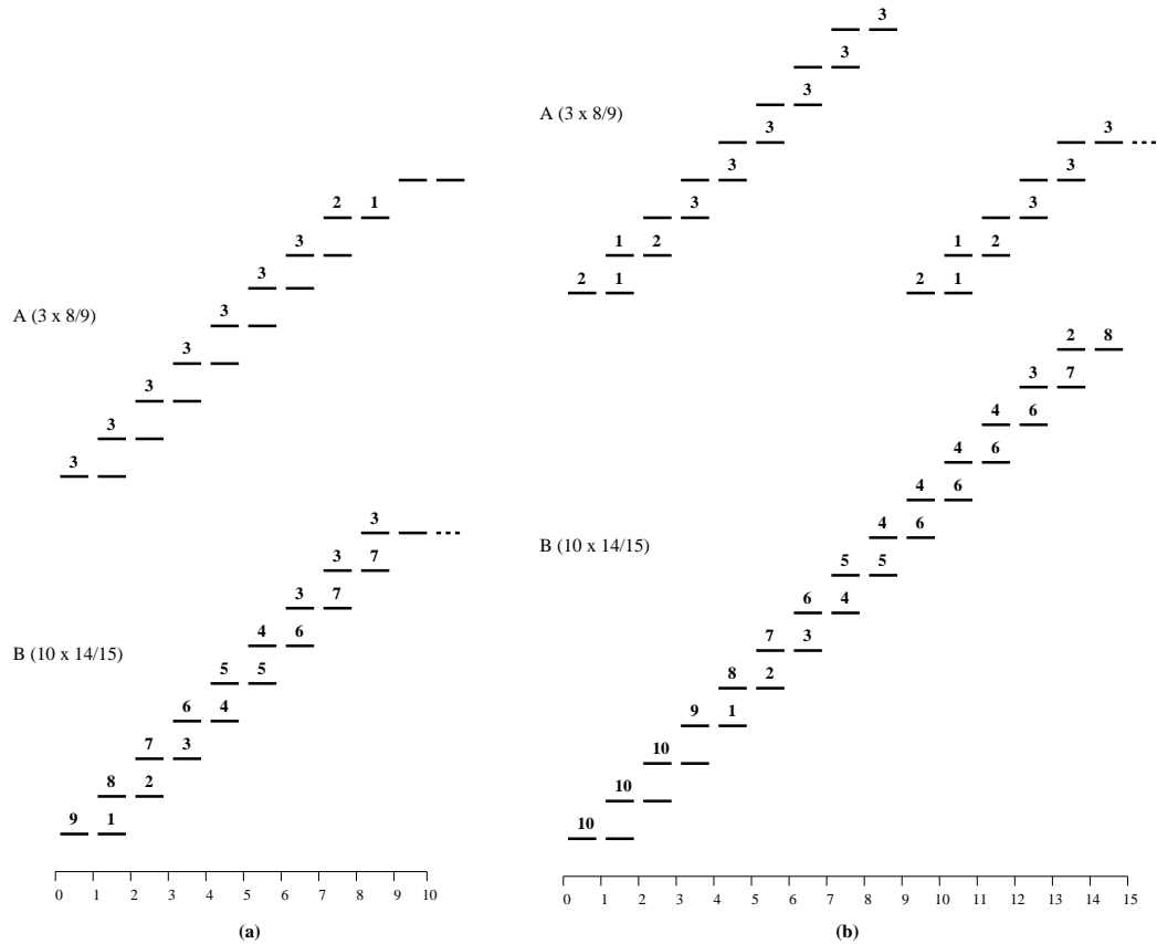
Fig. 6. Theorem 4.
