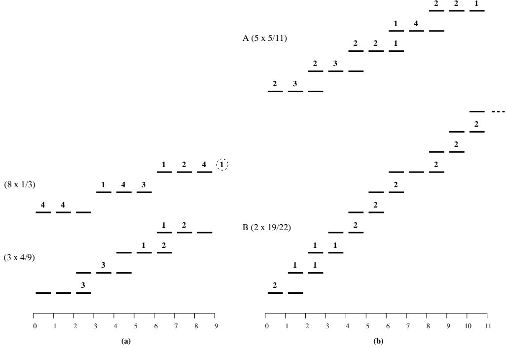
Fig. 4. The notation used here (and in Figures 5, 6, and 8) is the same as in Figure 1. (a) Theorem 1. A deadline is missed at time 9 by a task of weight 1/3 . (We do not illustrate deadline misses in the subsequent figures, and show the schedule only until a slot is reached in which fewer than M tasks are scheduled.) (b) Theorem 2.
