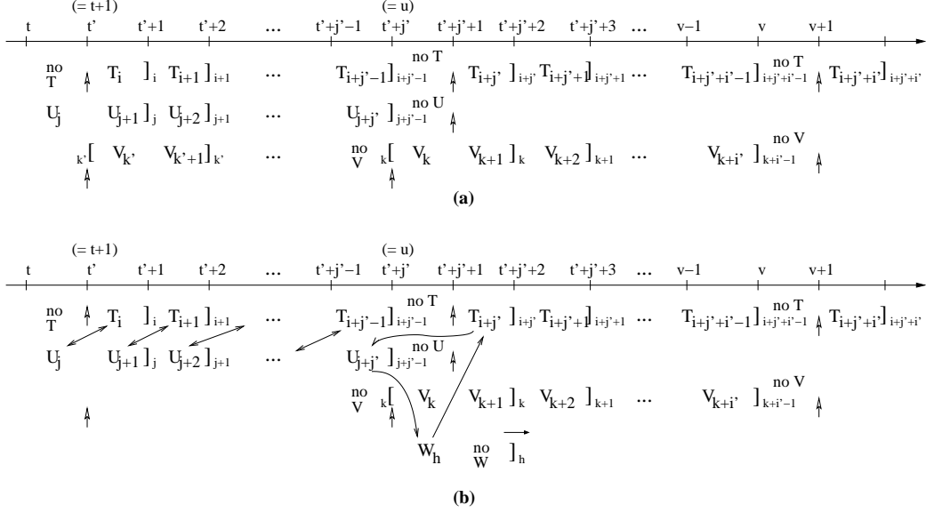
Fig. 19. Subcase 4.B. In each inset of this figure and Figures 20 and 21, t' = t + 1 , D(T_i) = D(U_j) , and D(V_k) = D(T_{i+j'}) . (a) \text{pred}(V, u) = \text{pred}(T, u + 1) . (b) d(W_h) \geq u + 2 .
