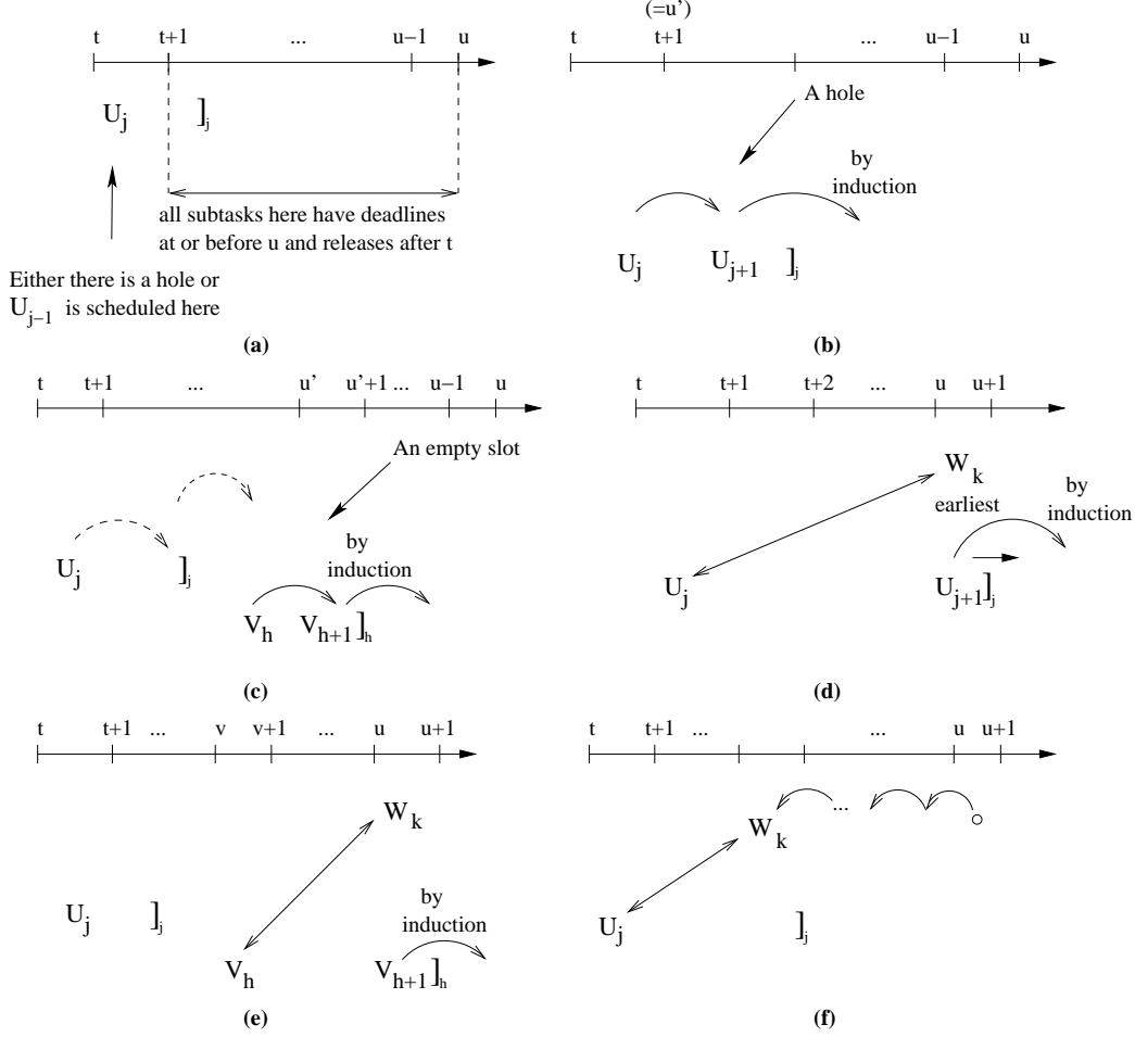
Fig. 23. Cases of Lemma 20. In each inset, d(U_j) > t+1 . (a) Case 1: Smallest interval [t+1, u) such that all subtasks have deadlines and releases inside the interval. (b) Subcase 1.A: u' = t+1 . (c) Subcase 1.B: u' > t+1 . (d) Subcase 2.A: d(U_j) \geq u+1 , and W_k is the earliest subtask with r(W_k) \leq t . (e) Subcase 2.B: d(U_j) < u+1 . (f) Repeated application of Subcase 2.B to finally apply Subcase 2.A.
