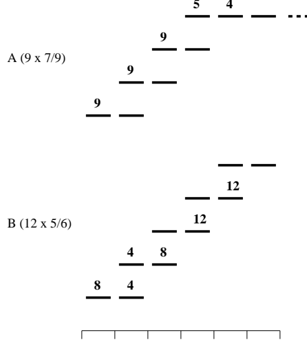
Fig. 7. Theorem 5.
