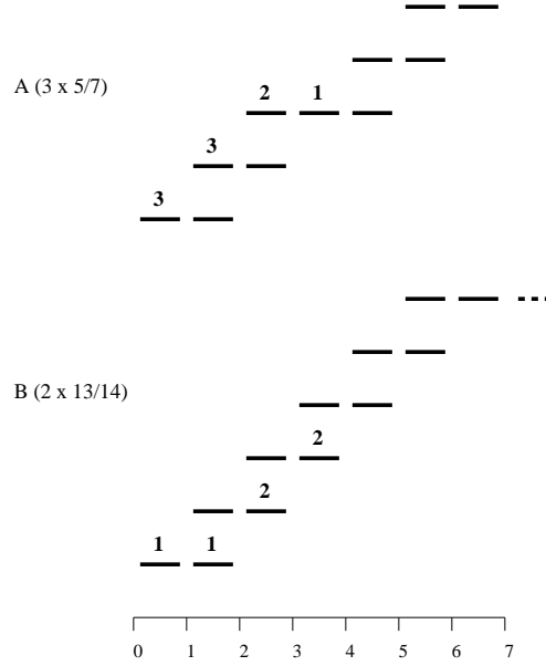
Fig. 5. Theorem 3 and Theorem 6.
