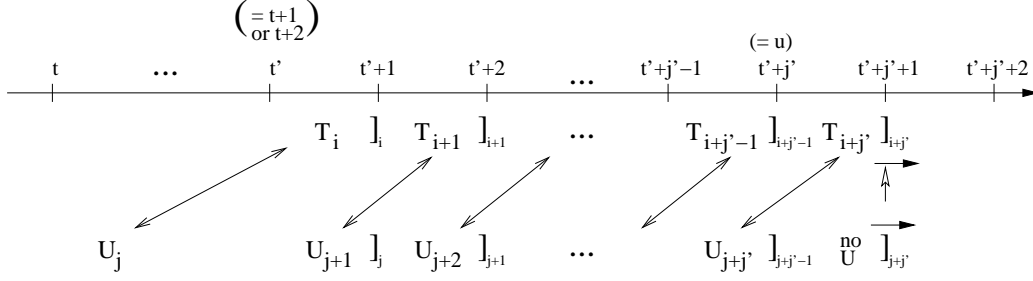
Fig. 15. Case 4. We use the following notation in this figure and Figures 16–21. A group deadline at time t is denoted by an up-arrow that is aligned with time t . A left- or right-pointing arrow over an up-arrow indicates a group deadline that may be anywhere in the direction of the arrow. D(T_i) > D(U_j) or u + 1 = D(T_i) \wedge T \in S_u .
