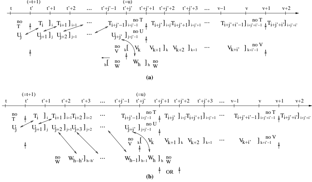
Fig. 20. Subcase 4.B (continued). (a) d(W_h) = u + 1 and W \notin S_{u-1} . (b) d(W_h) = u + 1 , W \in S_{u-1} , and W \notin S_w for some w in [t', u) .
