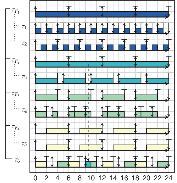
Figure 3: The schedule described in Example 3.1.
