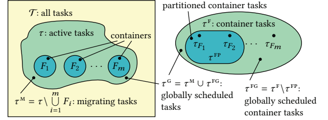
Figure 1: The relationships between the sets used in EDF-sc.
