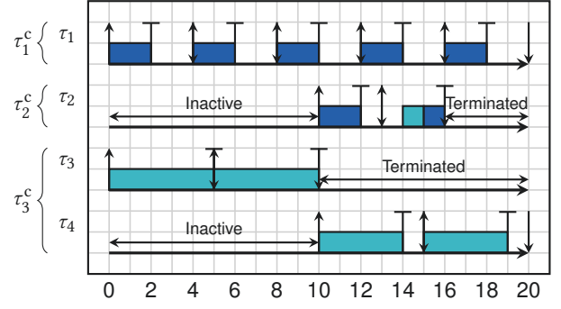
Figure 4: The extended sporadic task system in Example 4.1.
