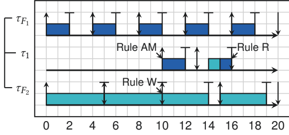
Figure 5: An EDF-sc schedule analogous to the one in Fig. 4.
