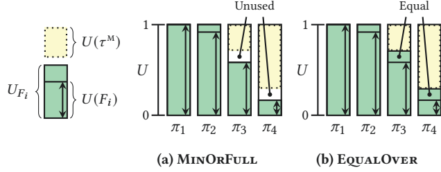
Figure 7: The two container task provisioning techniques discussed. (a) Container tasks \tau_{F_3} and \tau_{F_4} are minimally provisioned ( U_{F_i} = U(F_i) ), and \tau_{F_1} and \tau_{F_2} are fully provisioned ( U_{F_i} = 1 ). (b) Container task utilizations U_{F_3} and U_{F_4} are increased equally to consume the system capacity left unused by MINORFULL.
