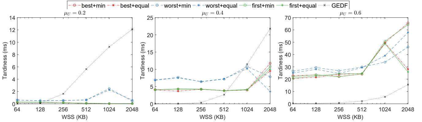
Figure 9: Left to right: observed average tardiness over easy-, moderate-, and hard-to-partition workloads.
