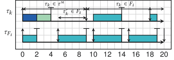
Figure 6: Task \tau_k is eligible to be moved at time 5, since \tau_{k,1} completed at time 4, and d_{k,1} = 9 < d_{F_i,2} = 10 . Its copy \tau'_k is added to F_i at time 5, and at time 9 the move is completed. Such “copy” tasks merely reserve container capacity and are not executed.
