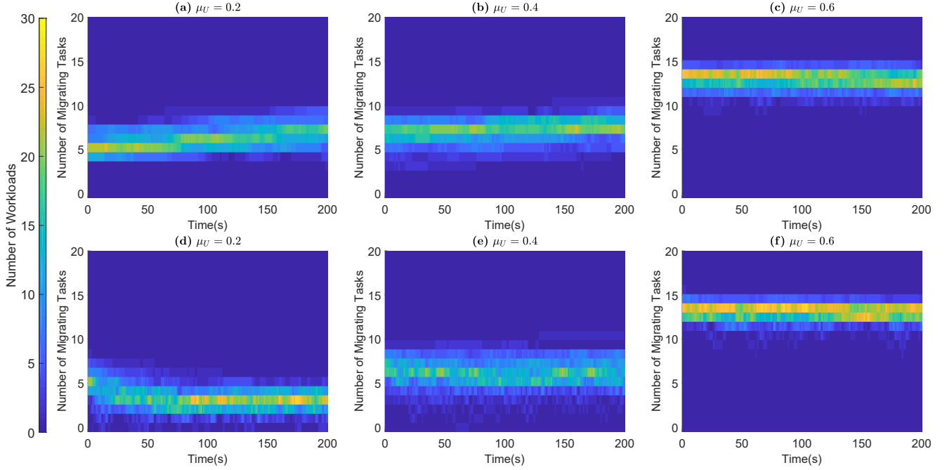
Figure 10: Stabilization heatmaps for WSS of 2048 kB. Insets (a), (b), and (c) (top) show easy-, moderate-, and hard-to-partition workloads with stabilization disabled. Insets (d), (e), and (f) (bottom) show easy-, moderate-, and hard-to-partition workloads with stabilization enabled.
