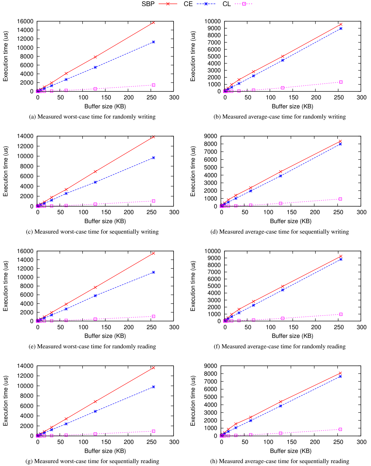
Figure 14: Measured execution data for accessing shared buffers.
