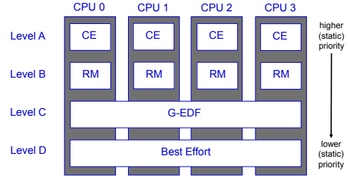
Figure 1: Scheduling in MC^2 on a quad-core machine.
