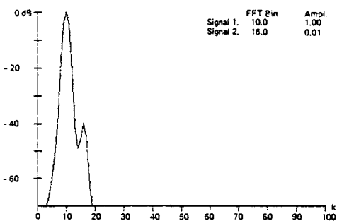
Fig. 63. \text{Cos}^3(n\pi/N) window.
