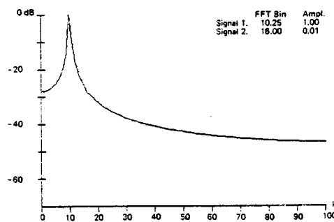
Fig. 59. Rectangle window.
