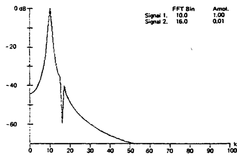
Fig. 71. Riesz window.
