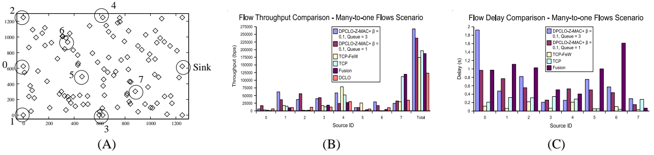
Fig. 6. (A) shows the topology and position of sources for the many-to-one flows scenario. All 8 sources transmit as fast as possible towards the sink node located on the right edge of the topology. (B) and (C) show the average flow throughput and end-to-end delay obtained. Note that on the x-axis, the sources are ordered in terms of their distance to the sink node.
