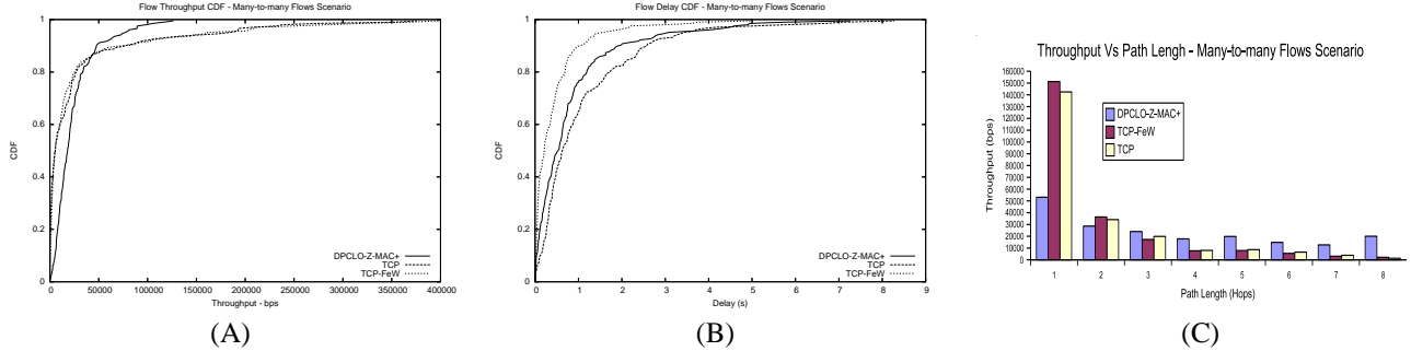
Fig. 7. (A) and (B) show the CDF of the average flow throughput and end-to-end delay for the many-to-many flow scenario. 206 flows are generated during a simulation time of 800s, with source and destination nodes chosen randomly on the topology shown in Figure 6 (A). Flow inter-arrival times and flow durations are picked from a Weibull and Log-normal distribution respectively. (C) shows the distribution of the throughput among flows based on their path lengths in terms of hops.
