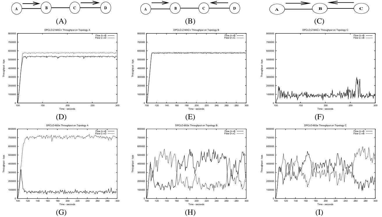
Fig. 5. Throughput of flows in three possible starvation scenarios when using DPCLO with TDMA-based Z-MAC+ and CSMA-based 802.11e. Figure (A) is one instance of the well known Information Asymmetry problem [10] which results in long-term starvation when used with randomized uncoordinated CSMA MAC protocols. Figures (B) and (C) represent symmetric flow scenarios where starvation is short-term.
