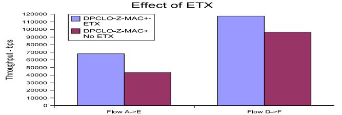
Fig. 4. The effect of ETX when DPCLO-Z-MAC+ is used on a wireless network with lossy links. We use the same topology and flow scenario as Figure 2 (A). Links are assigned loss rates chosen uniformly from the interval [0,0.6].
